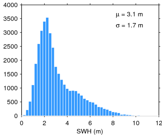
Figure 20. Histogram of science-valid SWH over oceans and lakes for 16/06/2016. The mean ( \mu ) and standard deviation ( \sigma ) are also shown. Note that values larger than 12 m are excluded from the histogram for the sake of readability but not from the computation of \mu and \sigma .
