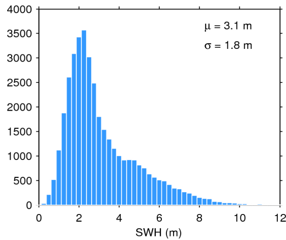
Figure 17. Histogram of flag-valid SWH over oceans and lakes for 16/06/2016. The mean ( \mu ) and standard deviation ( \sigma ) are also shown. Note that values larger than 12 m are excluded from the histogram for the sake of readability but not from the computation of \mu and \sigma .
