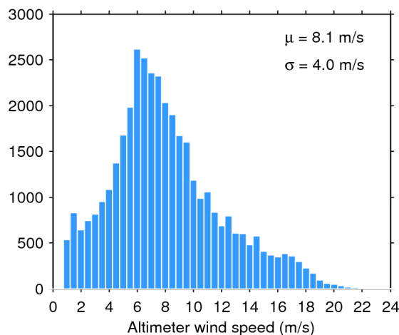
Figure 35. Histogram of science-valid wind over oceans and lakes for 16/06/2016. The mean ( \mu ) and standard deviation ( \sigma ) are also shown. Note that values larger than 24 m/s are excluded from the histogram for the sake of readability but not from the computation of \mu and \sigma .
