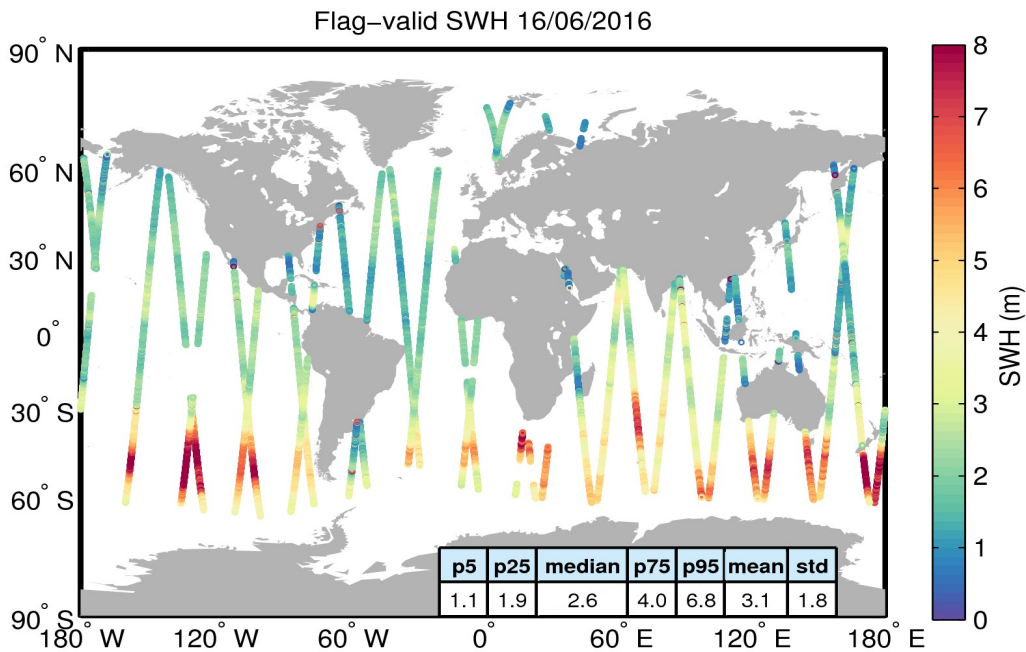
Figure 15. Geographical distribution of flag-valid SWH data over oceans and lakes for 16/06/2016. The statistical values shown in the table refer to the SWH in m and are calculated over all measurements shown in the figure.
