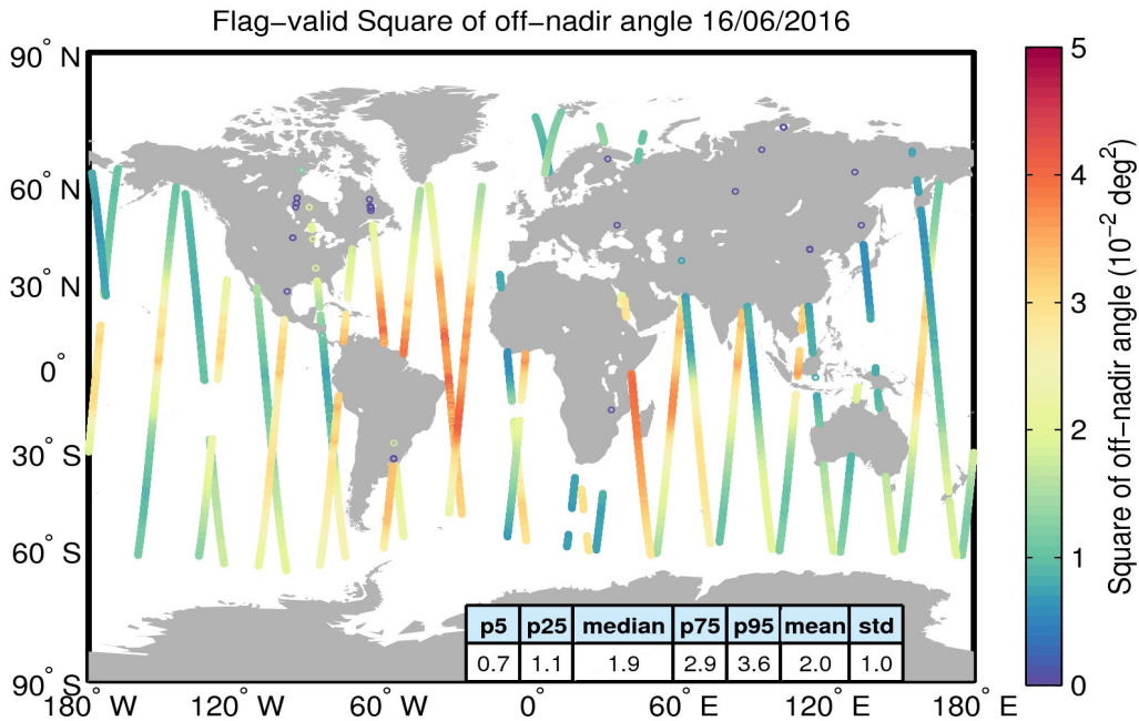
Figure 37. Geographical distribution of flag-valid mispointing data over oceans and lakes for 16/06/2016. The statistical values shown in the table refer to the mispointing in 10^{-2} \text{ deg}^2 and are calculated over all measurements shown in the figure.
