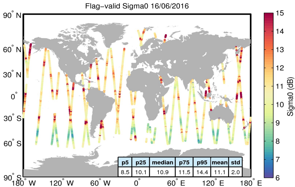
Figure 23. Geographical distribution of flag-valid sigma0 data over oceans and lakes for 16/06/2016. The statistical values shown in the table refer to the sigma0 in dB and are calculated over all measurements shown in the figure.
