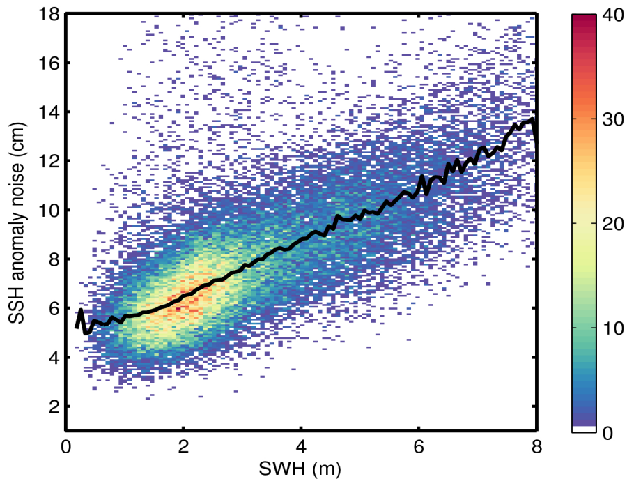
Figure 9. 2D histogram showing flag-valid SSH anomaly noise as a function of SWH for 16/06/2016. The black line denotes the median SSH anomaly noise as a function of SWH.
