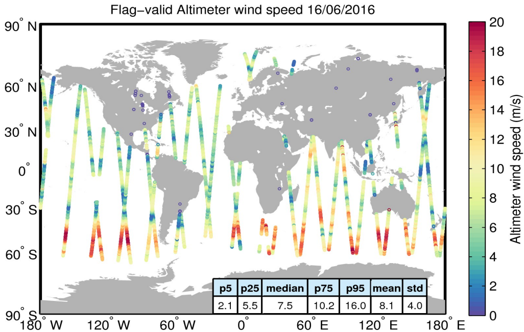
Figure 31. Geographical distribution of flag-valid wind data over oceans and lakes for 16/06/2016. The statistical values shown in the table refer to the wind in m/s and are calculated over all measurements shown in the figure.
