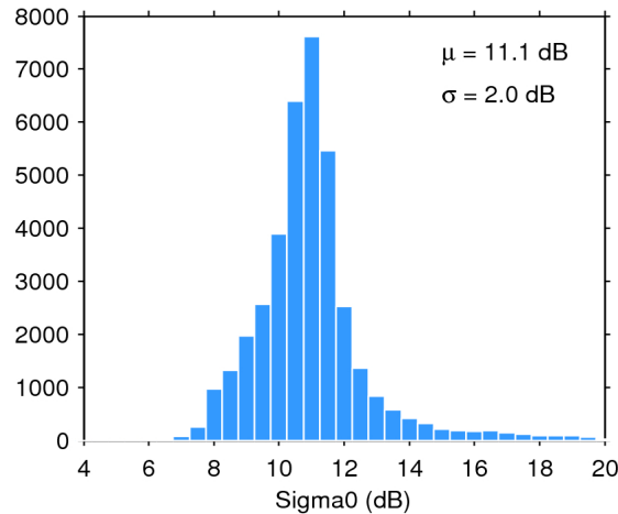
Figure 25. Histogram of flag-valid sigma0 over oceans and lakes for 16/06/2016. The mean ( \mu ) and standard deviation ( \sigma ) are also shown. Note that values outside [4 20] dB are excluded from the histogram for the sake of readability but not from the computation of \mu and \sigma .
