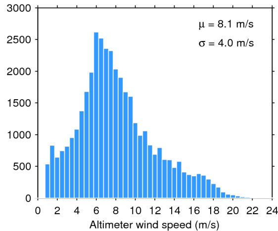
Figure 33. Histogram of flag-valid wind over oceans and lakes for 16/06/2016. The mean ( \mu ) and standard deviation ( \sigma ) are also shown. Note that values larger than 24 m/s are excluded from the histogram for the sake of readability but not from the computation of \mu and \sigma .
