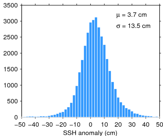
Figure 11. Histogram of science-valid SSH anomaly over oceans and lakes for 16/06/2016. The mean ( \mu ) and standard deviation ( \sigma ) are also shown. Note that values outside [-50 50] cm are excluded from the histogram for the sake of readability but not from the computation of \mu and \sigma .
