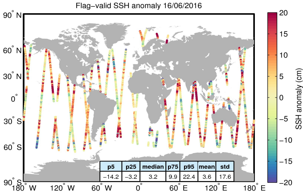
Figure 5. Geographical distribution of flag-valid 1-Hz SSH anomaly data over oceans and lakes for 16/06/2016. The statistical values shown in the table refer to the SSH anomaly in cm and are calculated over all measurements shown in the figure.
