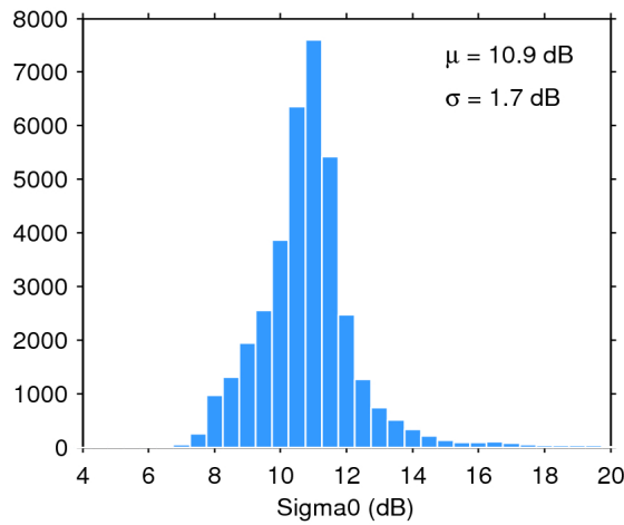
Figure 28. Histogram of science-valid sigma0 over oceans and lakes for 16/06/2016. The mean ( \mu ) and standard deviation ( \sigma ) are also shown. Note that values outside [4 20] dB are excluded from the histogram for the sake of readability but not from the computation of \mu and \sigma .
