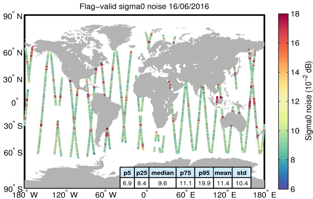
Figure 26. Geographical distribution of flag-valid 20-Hz sigma0 measurement noise over oceans and lakes for 16/06/2016. The statistical values shown in the table refer to the sigma0 noise and are calculated over all measurements shown in the figure.
