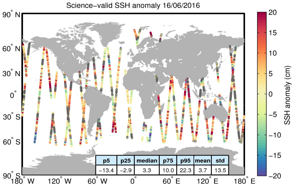
Figure 10. Geographical distribution of science-valid SSH anomaly data over oceans and lakes for 16/06/2016. The statistical values shown in the table refer to the SSH anomaly in cm and are calculated over all measurements shown in the figure. Gray circles denote records that have been rejected based on the editing criteria described in Table 2.
