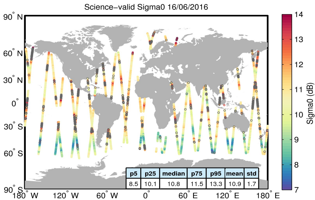
Figure 27. Geographical distribution of science-valid sigma0 data over oceans and lakes for 16/06/2016. The statistical values shown in the table refer to the sigma0 in dB and are calculated over all measurements shown in the figure. Gray circles denote records that have been rejected based on the editing criteria described in Table 4.
