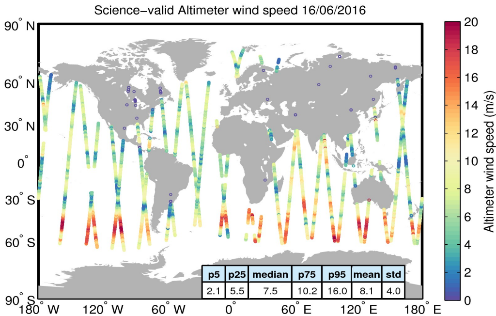
Figure 34. Geographical distribution of science-valid wind data over oceans and lakes for 16/06/2016. The statistical values shown in the table refer to the wind in m/s and are calculated over all measurements shown in the figure. Gray circles denote records that have been rejected based on the editing criteria described in Table 5.
