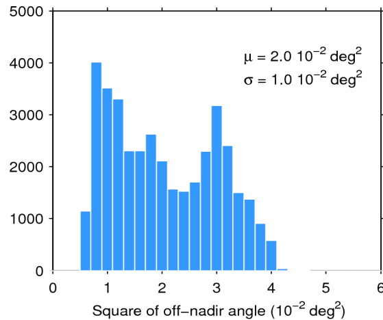
Figure 39. Histogram of flag-valid mispointing over oceans and lakes for 16/06/2016. The mean ( \mu ) and standard deviation ( \sigma ) are also shown. Note that values larger than 6 \cdot 10^{-2} \text{ deg}^2 are excluded from the histogram for the sake of readability but not from the computation of \mu and \sigma .
