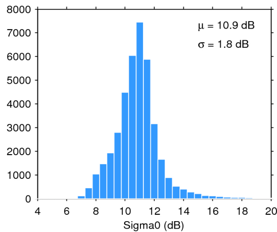
Figure 28. Histogram of science-valid sigma0 over oceans and lakes for 15/06/2016. The mean ( \mu ) and standard deviation ( \sigma ) are also shown. Note that values outside [4 20] dB are excluded from the histogram for the sake of readability but not from the computation of \mu and \sigma .
