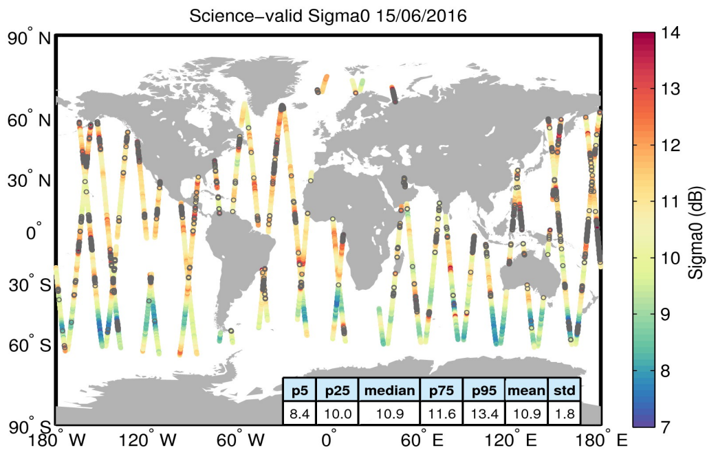
Figure 27. Geographical distribution of science-valid sigma0 data over oceans and lakes for 15/06/2016. The statistical values shown in the table refer to the sigma0 in dB and are calculated over all measurements shown in the figure. Gray circles denote records that have been rejected based on the editing criteria described in Table 4.
