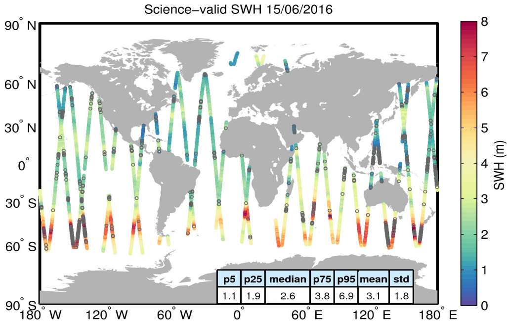
Figure 19. Geographical distribution of science-valid SWH data over oceans and lakes for 15/06/2016. The statistical values shown in the table refer to the SWH in m and are calculated over all measurements shown in the figure. Gray circles denote records that have been rejected based on the editing criteria described in Table 3.
