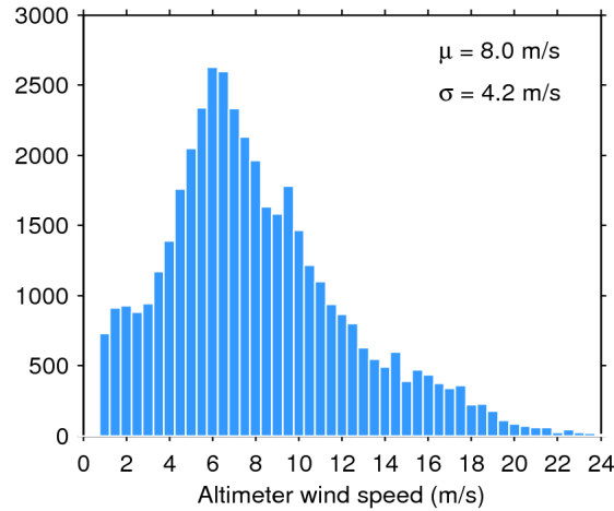
Figure 33. Histogram of flag-valid wind over oceans and lakes for 15/06/2016. The mean ( \mu ) and standard deviation ( \sigma ) are also shown. Note that values larger than 24 m/s are excluded from the histogram for the sake of readability but not from the computation of \mu and \sigma .
