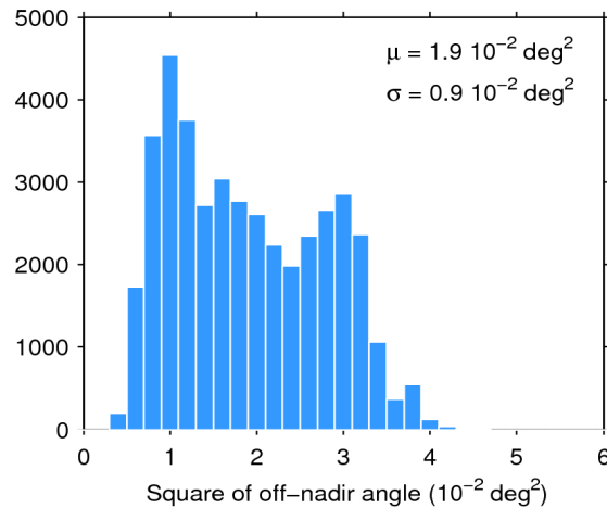
Figure 39. Histogram of flag-valid mispointing over oceans and lakes for 15/06/2016. The mean ( \mu ) and standard deviation ( \sigma ) are also shown. Note that values larger than 6 \cdot 10^{-2} \text{ deg}^2 are excluded from the histogram for the sake of readability but not from the computation of \mu and \sigma .
