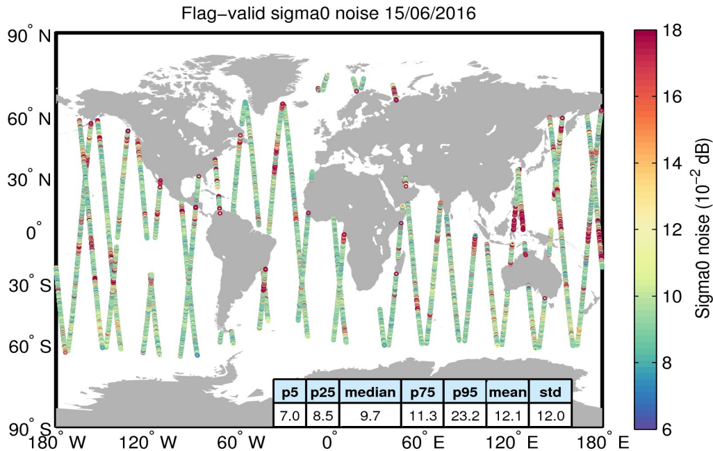
Figure 26. Geographical distribution of flag-valid 20-Hz sigma0 measurement noise over oceans and lakes for 15/06/2016. The statistical values shown in the table refer to the sigma0 noise and are calculated over all measurements shown in the figure.
