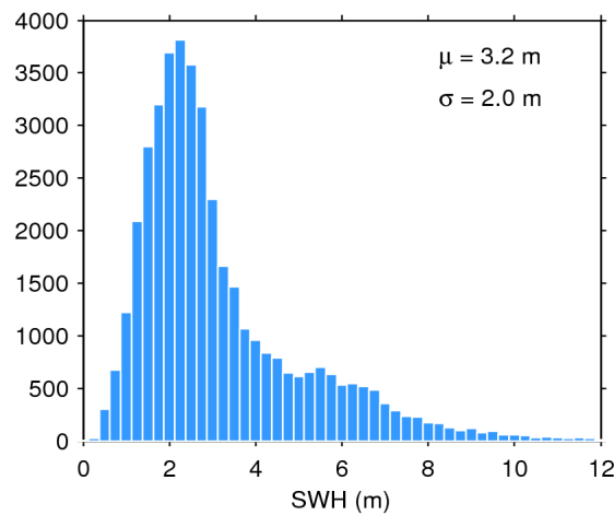
Figure 17. Histogram of flag-valid SWH over oceans and lakes for 15/06/2016. The mean ( \mu ) and standard deviation ( \sigma ) are also shown. Note that values larger than 12 m are excluded from the histogram for the sake of readability but not from the computation of \mu and \sigma .
