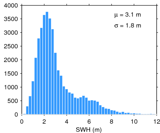
Figure 20. Histogram of science-valid SWH over oceans and lakes for 15/06/2016. The mean ( \mu ) and standard deviation ( \sigma ) are also shown. Note that values larger than 12 m are excluded from the histogram for the sake of readability but not from the computation of \mu and \sigma .
