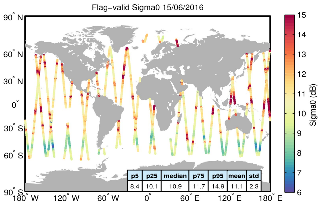
Figure 23. Geographical distribution of flag-valid sigma0 data over oceans and lakes for 15/06/2016. The statistical values shown in the table refer to the sigma0 in dB and are calculated over all measurements shown in the figure.
