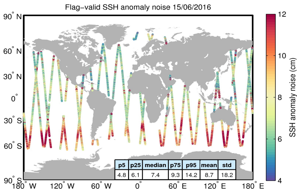
Figure 8. Geographical distribution of flag-valid 20-Hz SSH anomaly measurement noise over oceans and lakes for 15/06/2016. The statistical values shown in the table refer to the SSH anomaly noise and are calculated over all measurements shown in the figure.
