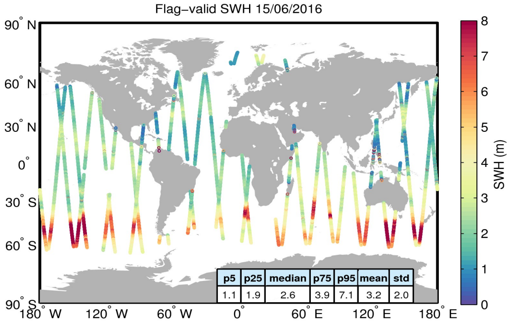
Figure 15. Geographical distribution of flag-valid SWH data over oceans and lakes for 15/06/2016. The statistical values shown in the table refer to the SWH in m and are calculated over all measurements shown in the figure.
