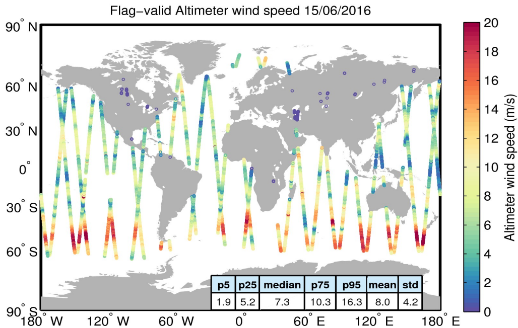
Figure 31. Geographical distribution of flag-valid wind data over oceans and lakes for 15/06/2016. The statistical values shown in the table refer to the wind in m/s and are calculated over all measurements shown in the figure.
