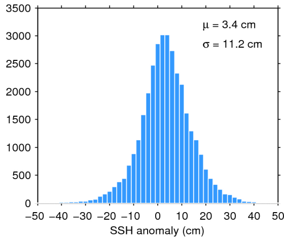
Figure 11. Histogram of science-valid SSH anomaly over oceans and lakes for 15/06/2016. The mean ( \mu ) and standard deviation ( \sigma ) are also shown. Note that values outside [-50 50] cm are excluded from the histogram for the sake of readability but not from the computation of \mu and \sigma .
