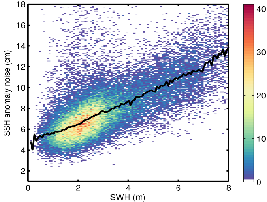
Figure 9. 2D histogram showing flag-valid SSH anomaly noise as a function of SWH for 15/06/2016. The black line denotes the median SSH anomaly noise as a function of SWH.
