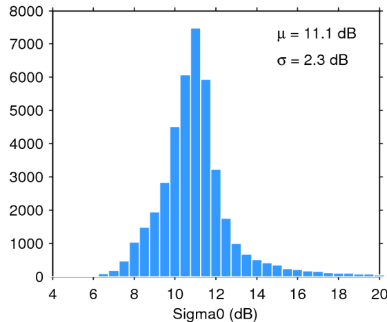
Figure 25. Histogram of flag-valid sigma0 over oceans and lakes for 15/06/2016. The mean ( \mu ) and standard deviation ( \sigma ) are also shown. Note that values outside [4 20] dB are excluded from the histogram for the sake of readability but not from the computation of \mu and \sigma .
