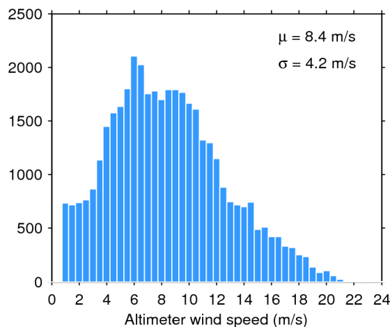
Figure 35. Histogram of science-valid wind over oceans and lakes for 12/06/2016. The mean ( \mu ) and standard deviation ( \sigma ) are also shown. Note that values larger than 24 m/s are excluded from the histogram for the sake of readability but not from the computation of \mu and \sigma .
