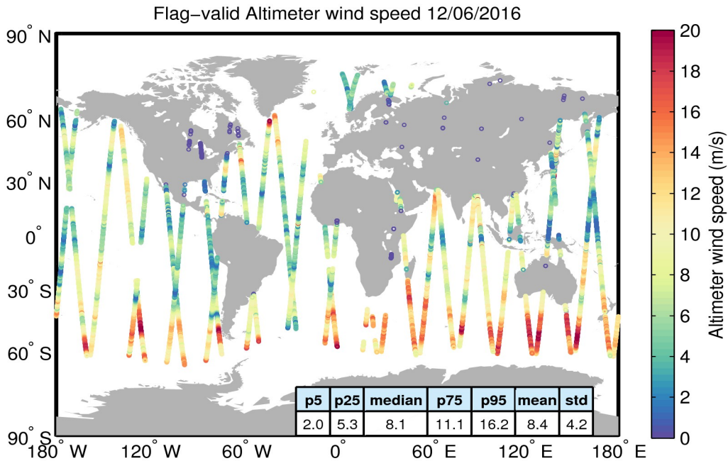
Figure 31. Geographical distribution of flag-valid wind data over oceans and lakes for 12/06/2016. The statistical values shown in the table refer to the wind in m/s and are calculated over all measurements shown in the figure.
