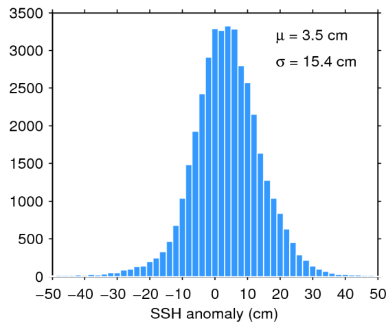
Figure 7. Histogram of flag-valid SSH anomaly over oceans and lakes for 12/06/2016. The mean ( \mu ) and standard deviation ( \sigma ) are also shown. Note that values outside [-50\ 50] cm are excluded from the histogram for the sake of readability but not from the computation of \mu and \sigma .
