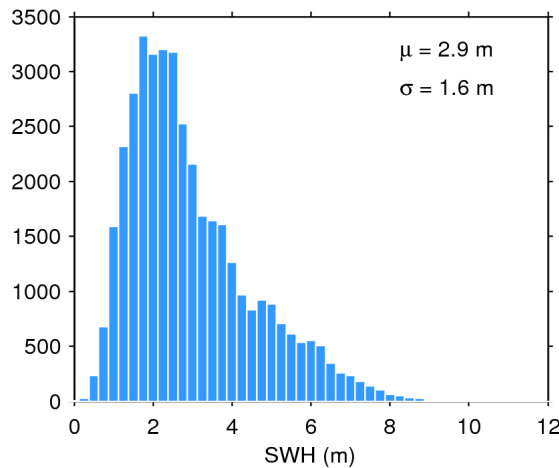
Figure 20. Histogram of science-valid SWH over oceans and lakes for 12/06/2016. The mean ( \mu ) and standard deviation ( \sigma ) are also shown. Note that values larger than 12 m are excluded from the histogram for the sake of readability but not from the computation of \mu and \sigma .
