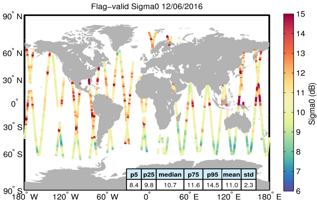
Figure 23. Geographical distribution of flag-valid sigma0 data over oceans and lakes for 12/06/2016. The statistical values shown in the table refer to the sigma0 in dB and are calculated over all measurements shown in the figure.
