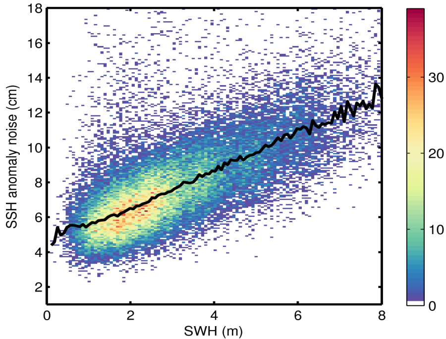
Figure 9. 2D histogram showing flag-valid SSH anomaly noise as a function of SWH for 12/06/2016. The black line denotes the median SSH anomaly noise as a function of SWH.
