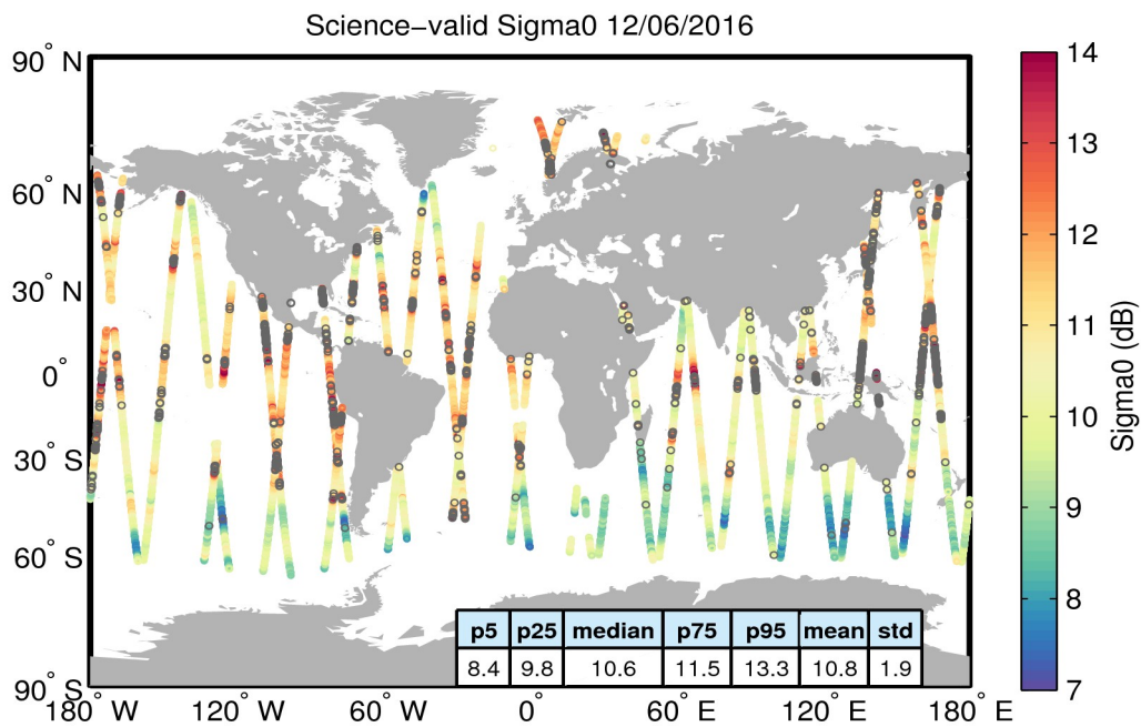
Figure 27. Geographical distribution of science-valid sigma0 data over oceans and lakes for 12/06/2016. The statistical values shown in the table refer to the sigma0 in dB and are calculated over all measurements shown in the figure. Gray circles denote records that have been rejected based on the editing criteria described in Table 4.
