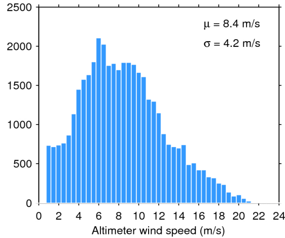
Figure 33. Histogram of flag-valid wind over oceans and lakes for 12/06/2016. The mean ( \mu ) and standard deviation ( \sigma ) are also shown. Note that values larger than 24 m/s are excluded from the histogram for the sake of readability but not from the computation of \mu and \sigma .
