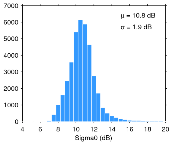
Figure 28. Histogram of science-valid sigma0 over oceans and lakes for 12/06/2016. The mean ( \mu ) and standard deviation ( \sigma ) are also shown. Note that values outside [4 20] dB are excluded from the histogram for the sake of readability but not from the computation of \mu and \sigma .
