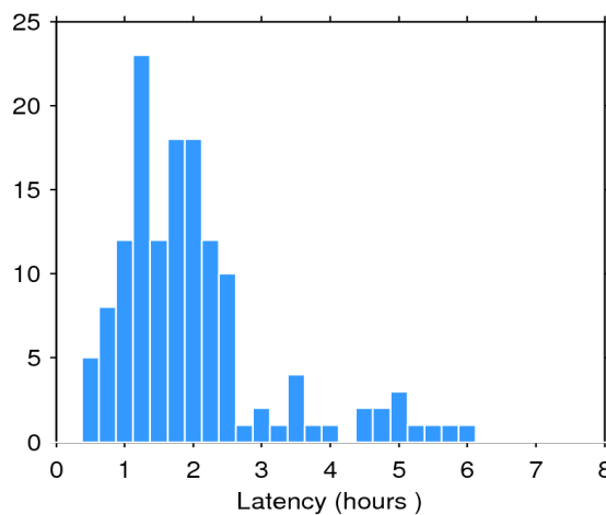
Figure 2. Histogram of the data latency for 12/06/2016. The y-axis denotes the number of files that are made available with a delay of x-hours with respect to the mean time of the records stored in the file.
