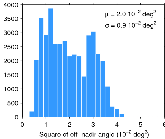
Figure 39. Histogram of flag-valid mispointing over oceans and lakes for 12/06/2016. The mean ( \mu ) and standard deviation ( \sigma ) are also shown. Note that values larger than 6 \cdot 10^{-2} \text{ deg}^2 are excluded from the histogram for the sake of readability but not from the computation of \mu and \sigma .
