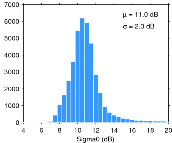
Figure 25. Histogram of flag-valid sigma0 over oceans and lakes for 12/06/2016. The mean ( \mu ) and standard deviation ( \sigma ) are also shown. Note that values outside [4 20] dB are excluded from the histogram for the sake of readability but not from the computation of \mu and \sigma .
