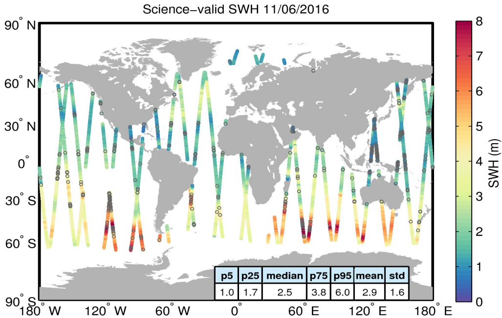
Figure 19. Geographical distribution of science-valid SWH data over oceans and lakes for 11/06/2016. The statistical values shown in the table refer to the SWH in m and are calculated over all measurements shown in the figure. Gray circles denote records that have been rejected based on the editing criteria described in Table 3.
