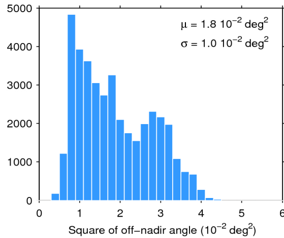
Figure 39. Histogram of flag-valid mispointing over oceans and lakes for 11/06/2016. The mean ( \mu ) and standard deviation ( \sigma ) are also shown. Note that values larger than 6 \cdot 10^{-2} \text{ deg}^2 are excluded from the histogram for the sake of readability but not from the computation of \mu and \sigma .
