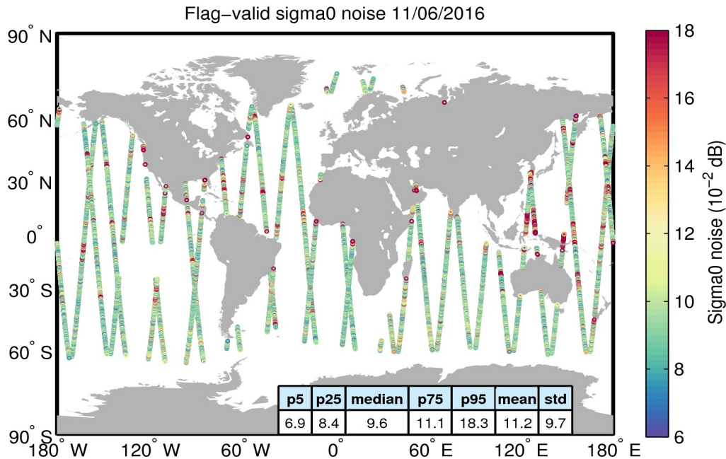
Figure 26. Geographical distribution of flag-valid 20-Hz sigma0 measurement noise over oceans and lakes for 11/06/2016. The statistical values shown in the table refer to the sigma0 noise and are calculated over all measurements shown in the figure.
