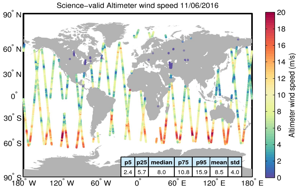
Figure 34. Geographical distribution of science-valid wind data over oceans and lakes for 11/06/2016. The statistical values shown in the table refer to the wind in m/s and are calculated over all measurements shown in the figure. Gray circles denote records that have been rejected based on the editing criteria described in Table 5.
