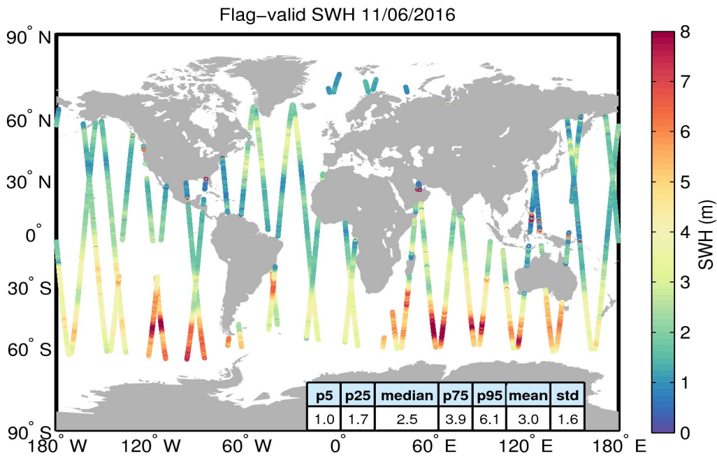
Figure 15. Geographical distribution of flag-valid SWH data over oceans and lakes for 11/06/2016. The statistical values shown in the table refer to the SWH in m and are calculated over all measurements shown in the figure.
