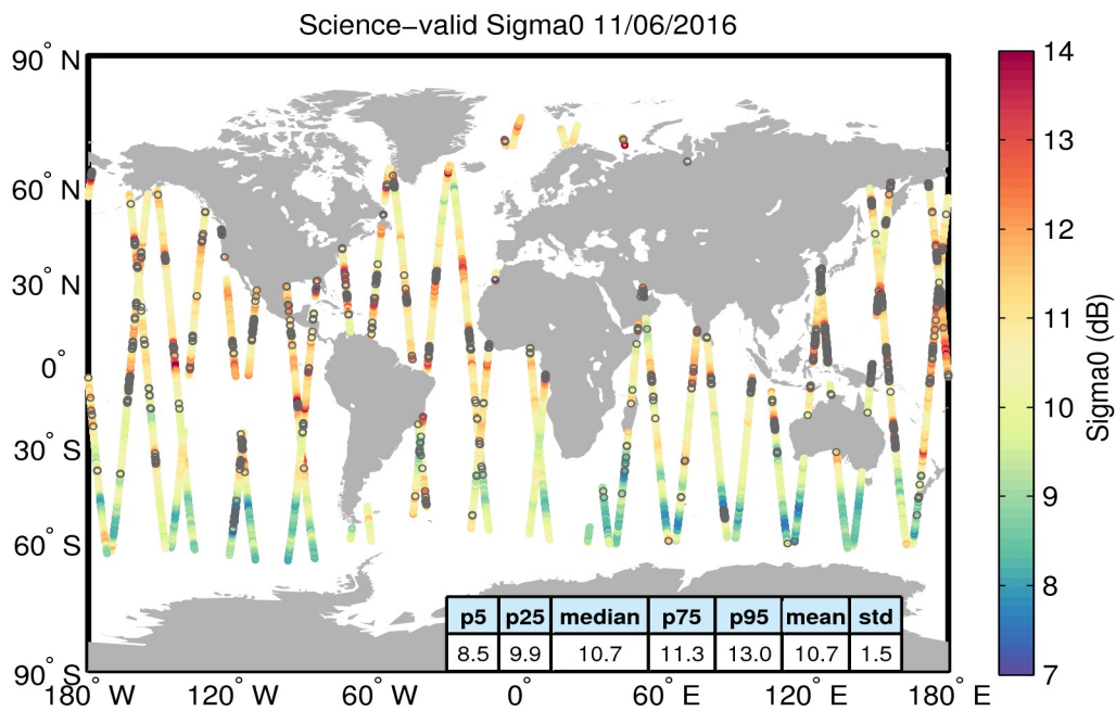
Figure 27. Geographical distribution of science-valid sigma0 data over oceans and lakes for 11/06/2016. The statistical values shown in the table refer to the sigma0 in dB and are calculated over all measurements shown in the figure. Gray circles denote records that have been rejected based on the editing criteria described in Table 4.
