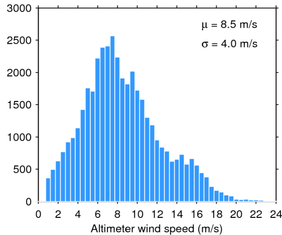
Figure 33. Histogram of flag-valid wind over oceans and lakes for 11/06/2016. The mean ( \mu ) and standard deviation ( \sigma ) are also shown. Note that values larger than 24 m/s are excluded from the histogram for the sake of readability but not from the computation of \mu and \sigma .
