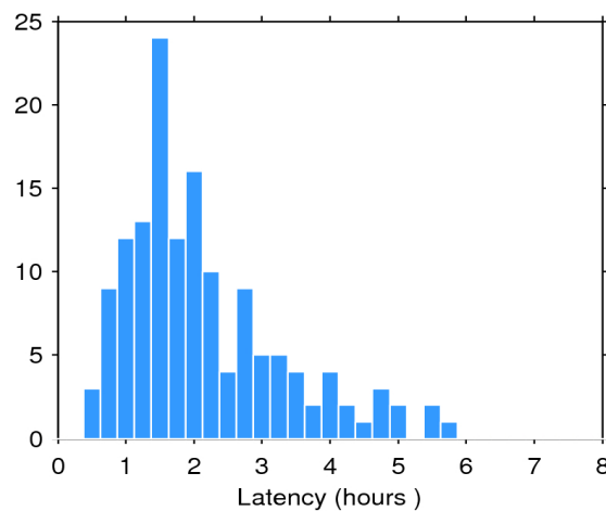
Figure 2. Histogram of the data latency for 11/06/2016. The y-axis denotes the number of files that are made available with a delay of x-hours with respect to the mean time of the records stored in the file.
