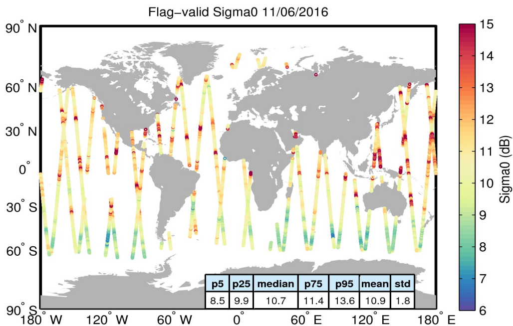
Figure 23. Geographical distribution of flag-valid sigma0 data over oceans and lakes for 11/06/2016. The statistical values shown in the table refer to the sigma0 in dB and are calculated over all measurements shown in the figure.
