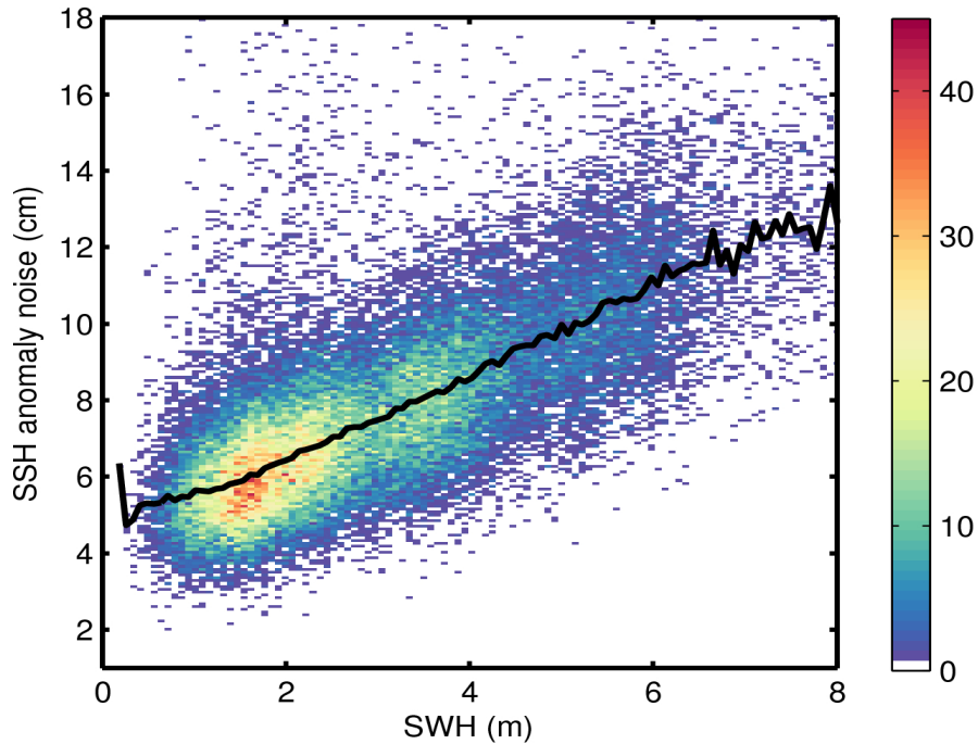
Figure 9. 2D histogram showing flag-valid SSH anomaly noise as a function of SWH for 11/06/2016. The black line denotes the median SSH anomaly noise as a function of SWH.
