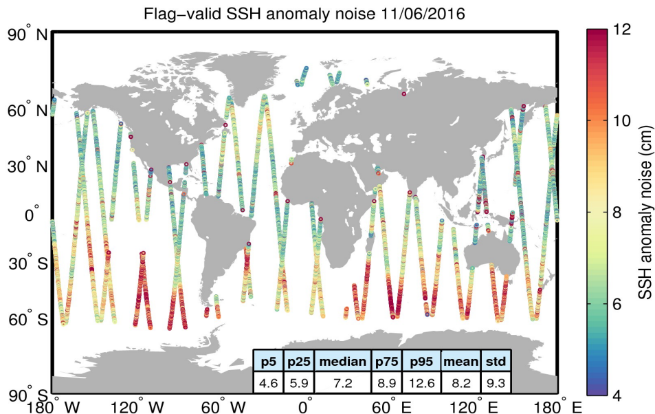
Figure 8. Geographical distribution of flag-valid 20-Hz SSH anomaly measurement noise over oceans and lakes for 11/06/2016. The statistical values shown in the table refer to the SSH anomaly noise and are calculated over all measurements shown in the figure.
