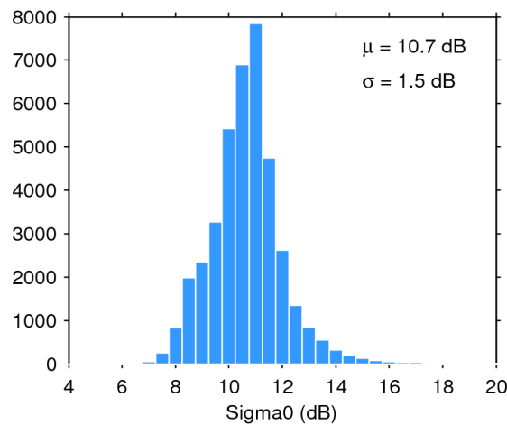
Figure 28. Histogram of science-valid sigma0 over oceans and lakes for 11/06/2016. The mean ( \mu ) and standard deviation ( \sigma ) are also shown. Note that values outside [4 20] dB are excluded from the histogram for the sake of readability but not from the computation of \mu and \sigma .
