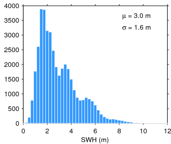
Figure 17. Histogram of flag-valid SWH over oceans and lakes for 11/06/2016. The mean ( \mu ) and standard deviation ( \sigma ) are also shown. Note that values larger than 12 m are excluded from the histogram for the sake of readability but not from the computation of \mu and \sigma .
