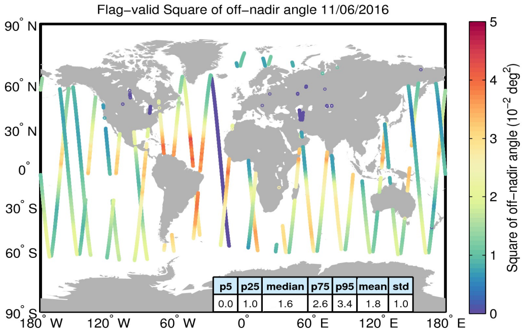
Figure 37. Geographical distribution of flag-valid mispointing data over oceans and lakes for 11/06/2016. The statistical values shown in the table refer to the mispointing in 10^{-2} \text{ deg}^2 and are calculated over all measurements shown in the figure.
