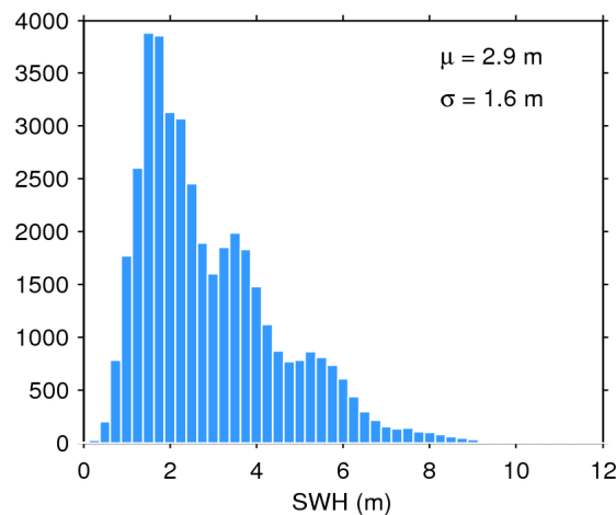
Figure 20. Histogram of science-valid SWH over oceans and lakes for 11/06/2016. The mean ( \mu ) and standard deviation ( \sigma ) are also shown. Note that values larger than 12 m are excluded from the histogram for the sake of readability but not from the computation of \mu and \sigma .
