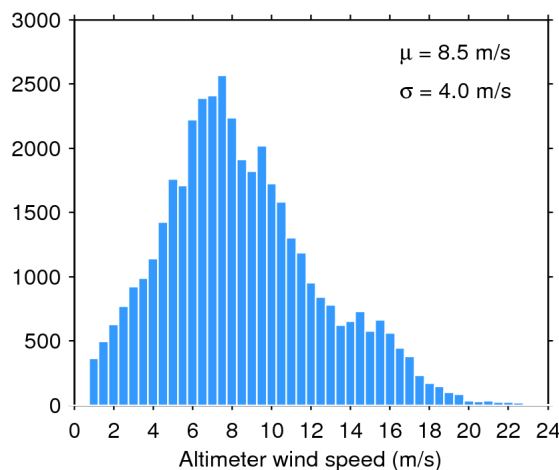
Figure 35. Histogram of science-valid wind over oceans and lakes for 11/06/2016. The mean ( \mu ) and standard deviation ( \sigma ) are also shown. Note that values larger than 24 m/s are excluded from the histogram for the sake of readability but not from the computation of \mu and \sigma .
