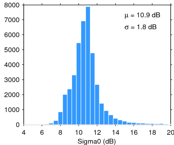
Figure 25. Histogram of flag-valid sigma0 over oceans and lakes for 11/06/2016. The mean ( \mu ) and standard deviation ( \sigma ) are also shown. Note that values outside [4 20] dB are excluded from the histogram for the sake of readability but not from the computation of \mu and \sigma .
