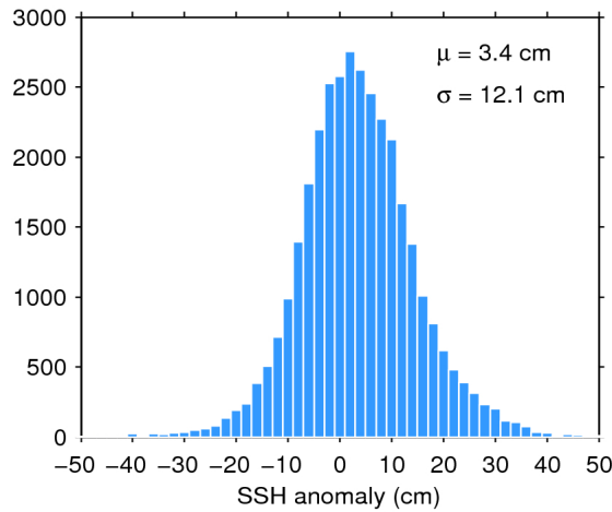
Figure 11. Histogram of science-valid SSH anomaly over oceans and lakes for 11/06/2016. The mean ( \mu ) and standard deviation ( \sigma ) are also shown. Note that values outside [-50 50] cm are excluded from the histogram for the sake of readability but not from the computation of \mu and \sigma .
