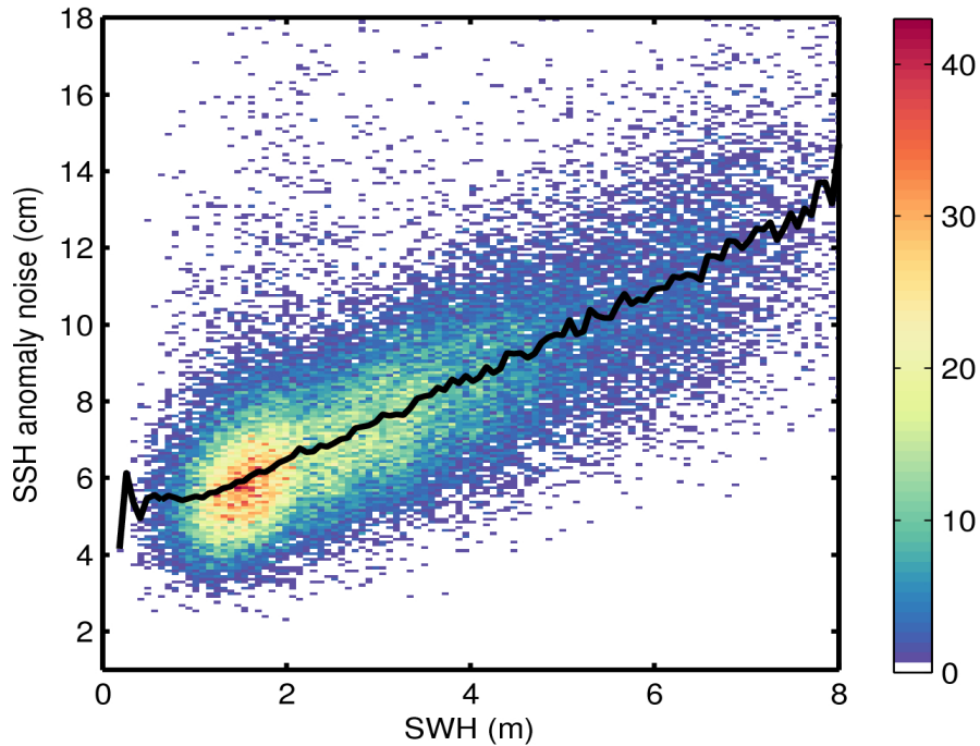
Figure 9. 2D histogram showing flag-valid SSH anomaly noise as a function of SWH for 10/06/2016. The black line denotes the median SSH anomaly noise as a function of SWH.
