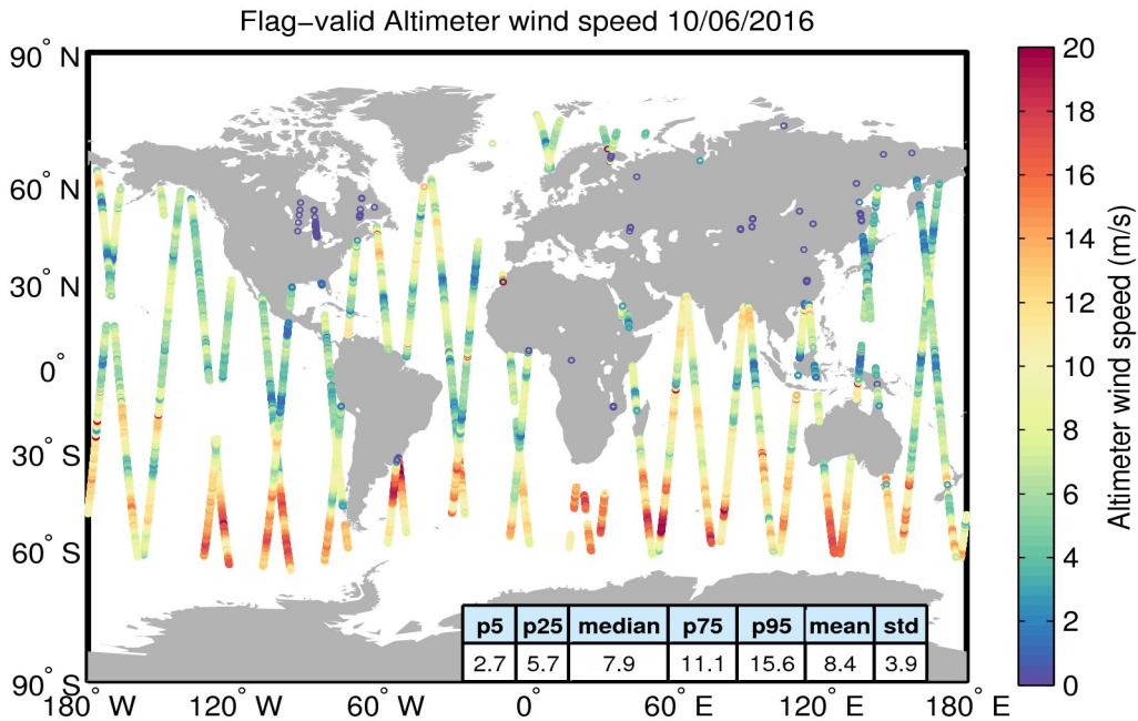
Figure 31. Geographical distribution of flag-valid wind data over oceans and lakes for 10/06/2016. The statistical values shown in the table refer to the wind in m/s and are calculated over all measurements shown in the figure.
