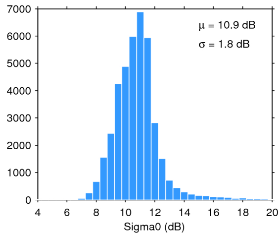
Figure 25. Histogram of flag-valid sigma0 over oceans and lakes for 10/06/2016. The mean ( \mu ) and standard deviation ( \sigma ) are also shown. Note that values outside [4 20] dB are excluded from the histogram for the sake of readability but not from the computation of \mu and \sigma .
