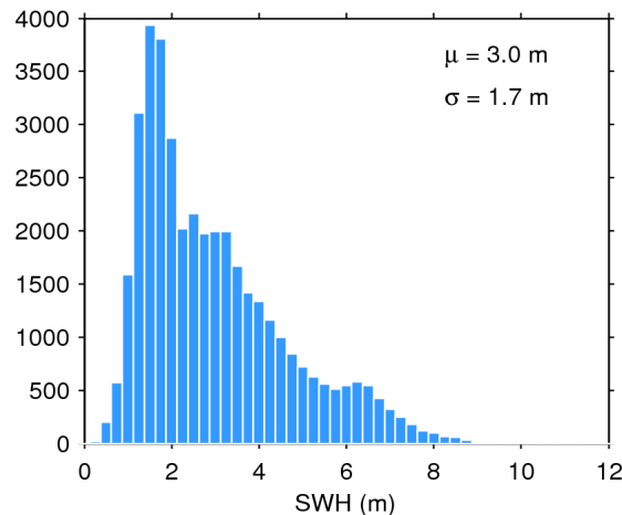
Figure 20. Histogram of science-valid SWH over oceans and lakes for 10/06/2016. The mean ( \mu ) and standard deviation ( \sigma ) are also shown. Note that values larger than 12 m are excluded from the histogram for the sake of readability but not from the computation of \mu and \sigma .
