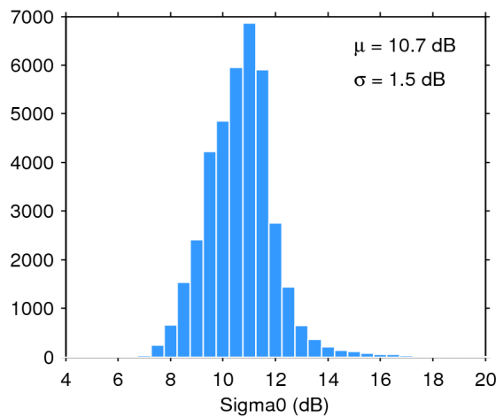
Figure 28. Histogram of science-valid sigma0 over oceans and lakes for 10/06/2016. The mean ( \mu ) and standard deviation ( \sigma ) are also shown. Note that values outside [4 20] dB are excluded from the histogram for the sake of readability but not from the computation of \mu and \sigma .
