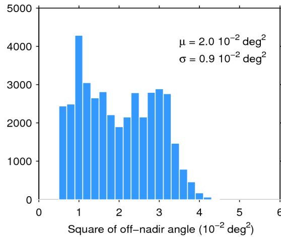
Figure 39. Histogram of flag-valid mispointing over oceans and lakes for 10/06/2016. The mean ( \mu ) and standard deviation ( \sigma ) are also shown. Note that values larger than 6 \cdot 10^{-2} \text{ deg}^2 are excluded from the histogram for the sake of readability but not from the computation of \mu and \sigma .
