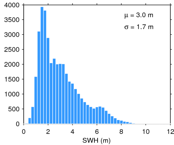
Figure 17. Histogram of flag-valid SWH over oceans and lakes for 10/06/2016. The mean ( \mu ) and standard deviation ( \sigma ) are also shown. Note that values larger than 12 m are excluded from the histogram for the sake of readability but not from the computation of \mu and \sigma .
