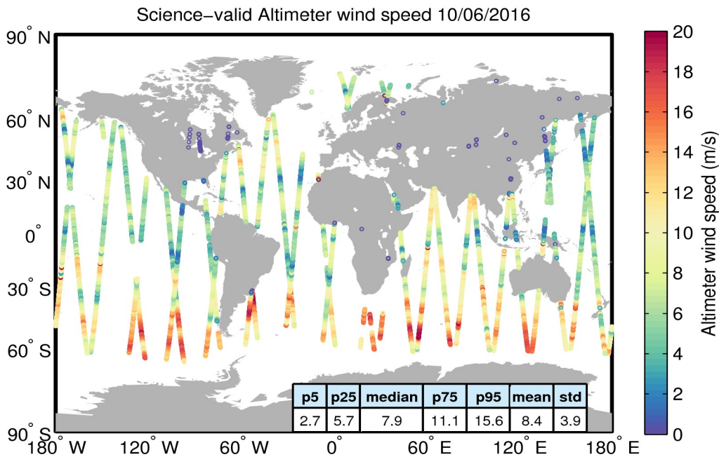
Figure 34. Geographical distribution of science-valid wind data over oceans and lakes for 10/06/2016. The statistical values shown in the table refer to the wind in m/s and are calculated over all measurements shown in the figure. Gray circles denote records that have been rejected based on the editing criteria described in Table 5.
