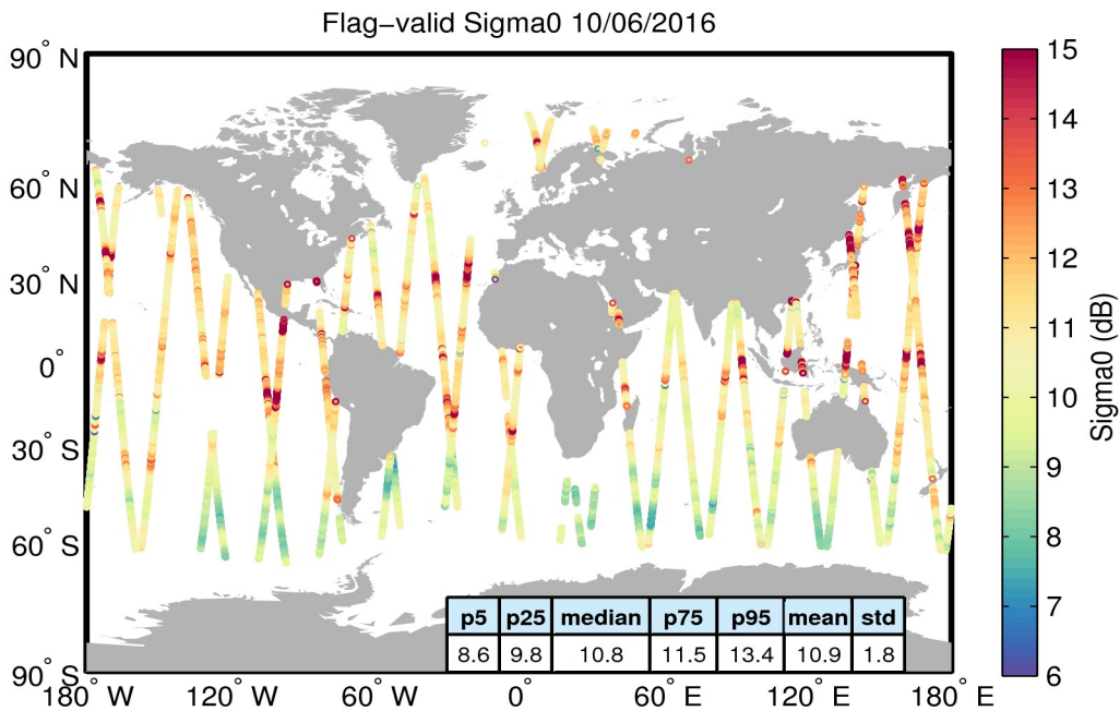
Figure 23. Geographical distribution of flag-valid sigma0 data over oceans and lakes for 10/06/2016. The statistical values shown in the table refer to the sigma0 in dB and are calculated over all measurements shown in the figure.
