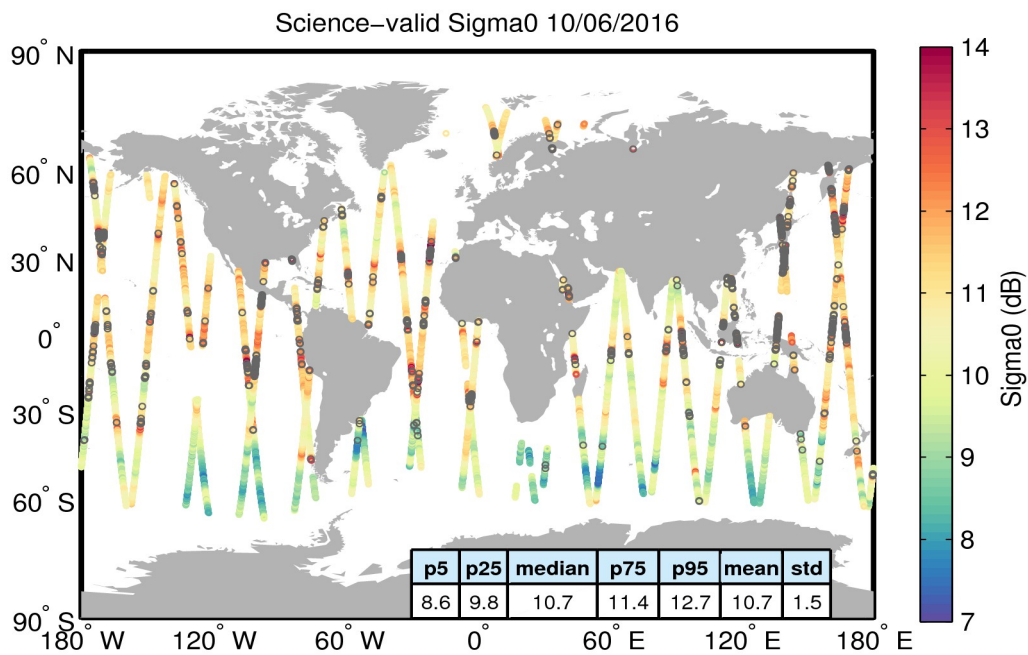
Figure 27. Geographical distribution of science-valid sigma0 data over oceans and lakes for 10/06/2016. The statistical values shown in the table refer to the sigma0 in dB and are calculated over all measurements shown in the figure. Gray circles denote records that have been rejected based on the editing criteria described in Table 4.
