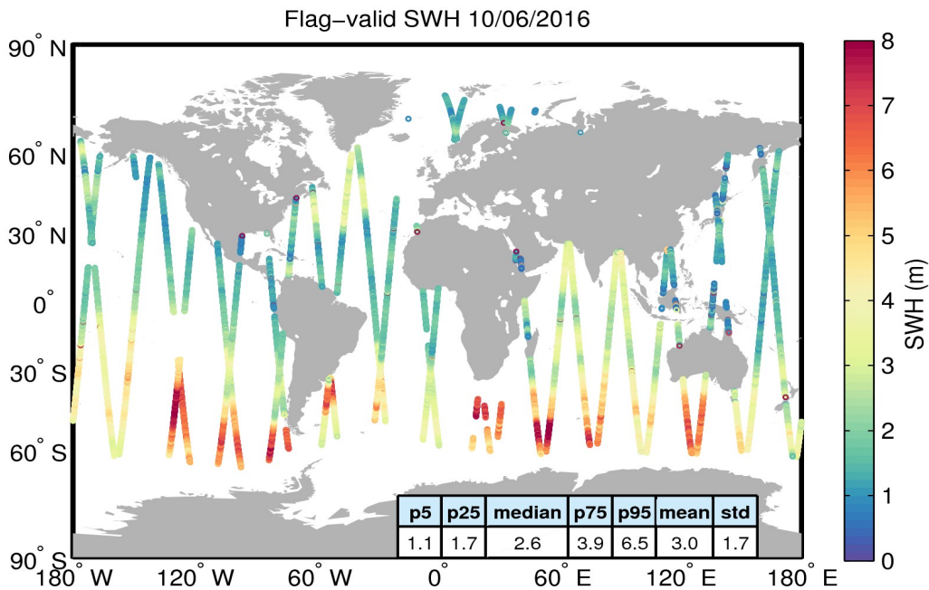
Figure 15. Geographical distribution of flag-valid SWH data over oceans and lakes for 10/06/2016. The statistical values shown in the table refer to the SWH in m and are calculated over all measurements shown in the figure.
