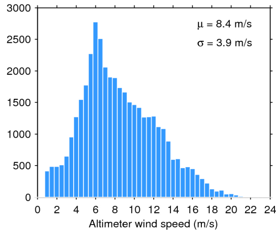
Figure 33. Histogram of flag-valid wind over oceans and lakes for 10/06/2016. The mean ( \mu ) and standard deviation ( \sigma ) are also shown. Note that values larger than 24 m/s are excluded from the histogram for the sake of readability but not from the computation of \mu and \sigma .
