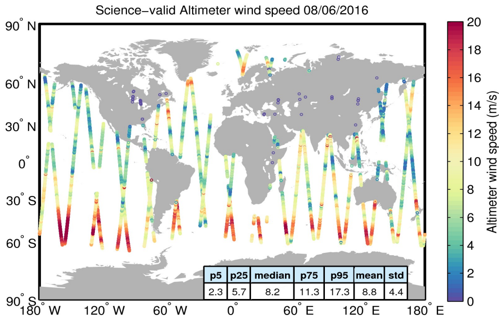
Figure 34. Geographical distribution of science-valid wind data over oceans and lakes for 08/06/2016. The statistical values shown in the table refer to the wind in m/s and are calculated over all measurements shown in the figure. Gray circles denote records that have been rejected based on the editing criteria described in Table 5.
