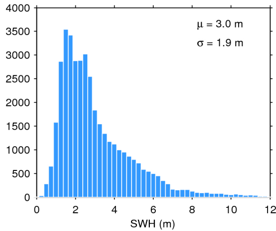
Figure 17. Histogram of flag-valid SWH over oceans and lakes for 08/06/2016. The mean ( \mu ) and standard deviation ( \sigma ) are also shown. Note that values larger than 12 m are excluded from the histogram for the sake of readability but not from the computation of \mu and \sigma .
