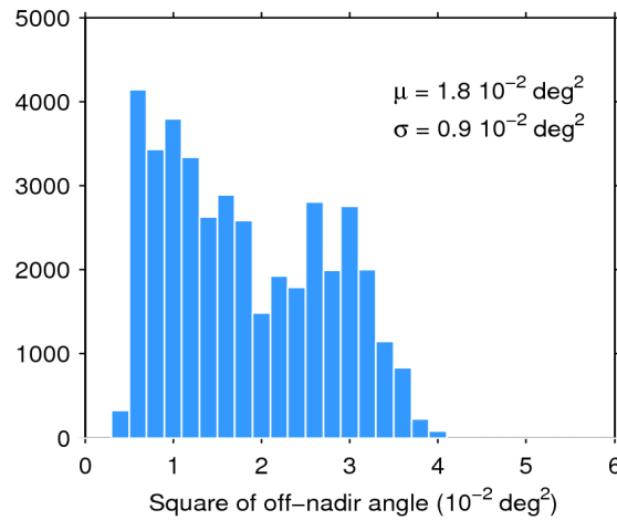
Figure 39. Histogram of flag-valid mispointing over oceans and lakes for 08/06/2016. The mean ( \mu ) and standard deviation ( \sigma ) are also shown. Note that values larger than 6 \cdot 10^{-2} \text{ deg}^2 are excluded from the histogram for the sake of readability but not from the computation of \mu and \sigma .
