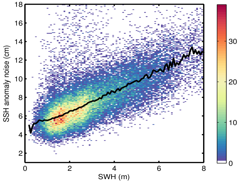
Figure 9. 2D histogram showing flag-valid SSH anomaly noise as a function of SWH for 08/06/2016. The black line denotes the median SSH anomaly noise as a function of SWH.
