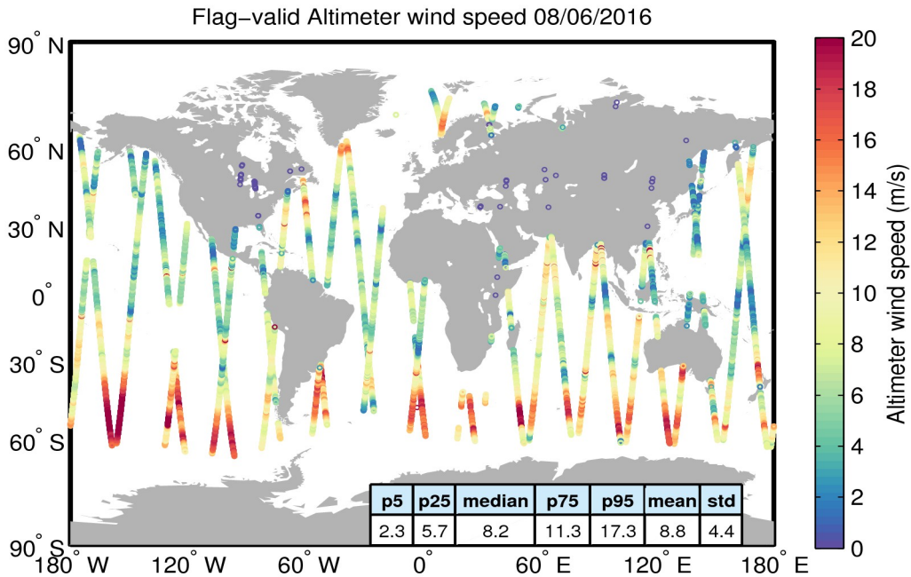
Figure 31. Geographical distribution of flag-valid wind data over oceans and lakes for 08/06/2016. The statistical values shown in the table refer to the wind in m/s and are calculated over all measurements shown in the figure.
