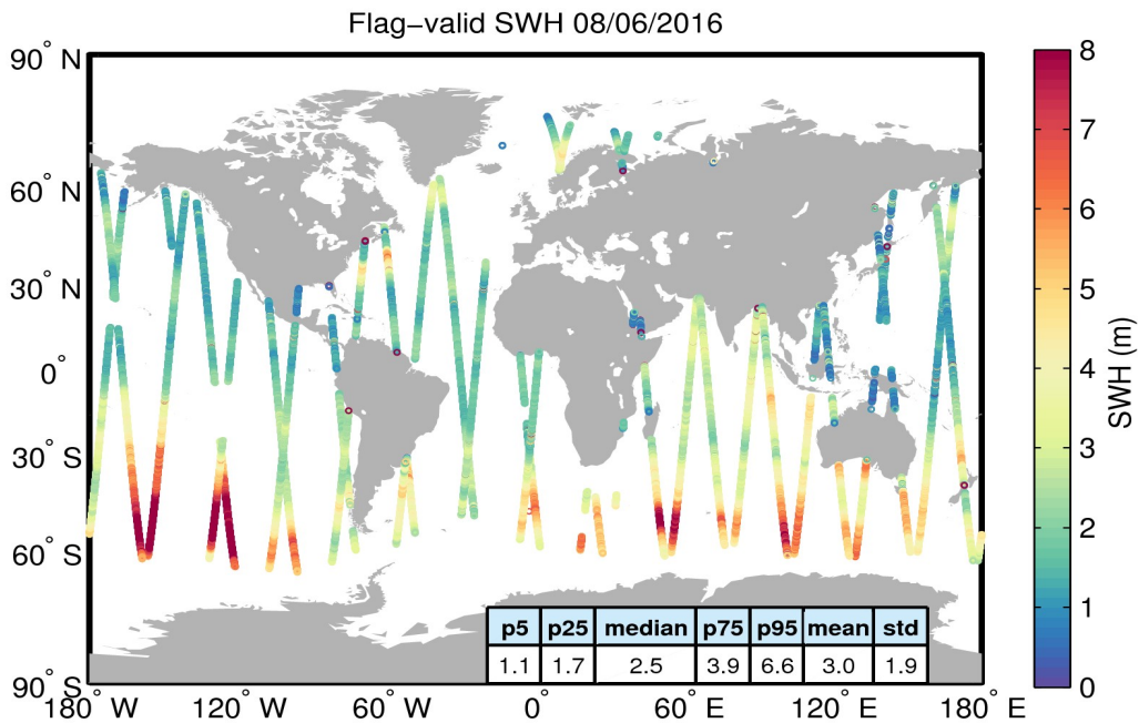
Figure 15. Geographical distribution of flag-valid SWH data over oceans and lakes for 08/06/2016. The statistical values shown in the table refer to the SWH in m and are calculated over all measurements shown in the figure.
