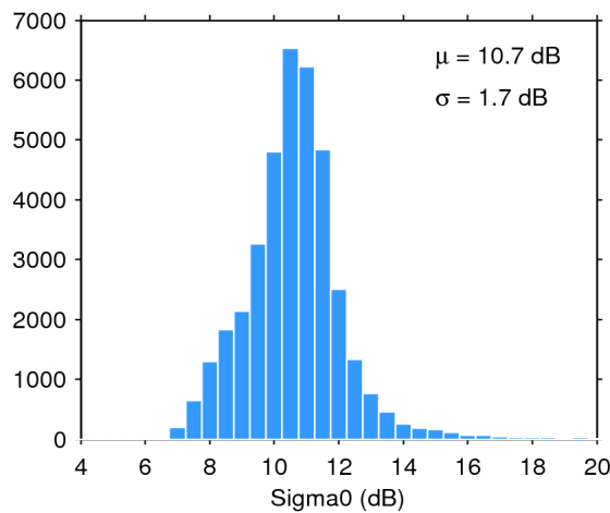
Figure 28. Histogram of science-valid sigma0 over oceans and lakes for 08/06/2016. The mean ( \mu ) and standard deviation ( \sigma ) are also shown. Note that values outside [4 20] dB are excluded from the histogram for the sake of readability but not from the computation of \mu and \sigma .
