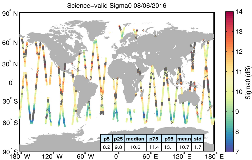
Figure 27. Geographical distribution of science-valid sigma0 data over oceans and lakes for 08/06/2016. The statistical values shown in the table refer to the sigma0 in dB and are calculated over all measurements shown in the figure. Gray circles denote records that have been rejected based on the editing criteria described in Table 4.
