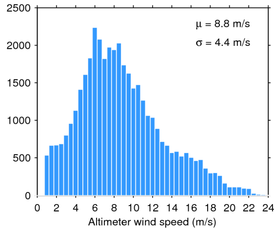
Figure 33. Histogram of flag-valid wind over oceans and lakes for 08/06/2016. The mean ( \mu ) and standard deviation ( \sigma ) are also shown. Note that values larger than 24 m/s are excluded from the histogram for the sake of readability but not from the computation of \mu and \sigma .
