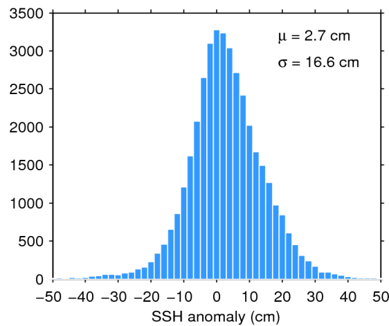
Figure 7. Histogram of flag-valid SSH anomaly over oceans and lakes for 08/06/2016. The mean ( \mu ) and standard deviation ( \sigma ) are also shown. Note that values outside [-50 50] cm are excluded from the histogram for the sake of readability but not from the computation of \mu and \sigma .
