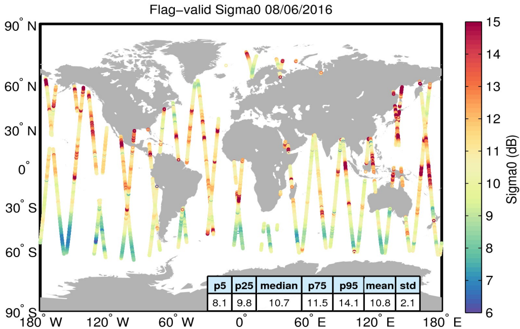
Figure 23. Geographical distribution of flag-valid sigma0 data over oceans and lakes for 08/06/2016. The statistical values shown in the table refer to the sigma0 in dB and are calculated over all measurements shown in the figure.
