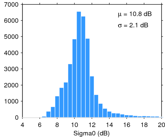
Figure 25. Histogram of flag-valid sigma0 over oceans and lakes for 08/06/2016. The mean ( \mu ) and standard deviation ( \sigma ) are also shown. Note that values outside [4 20] dB are excluded from the histogram for the sake of readability but not from the computation of \mu and \sigma .
