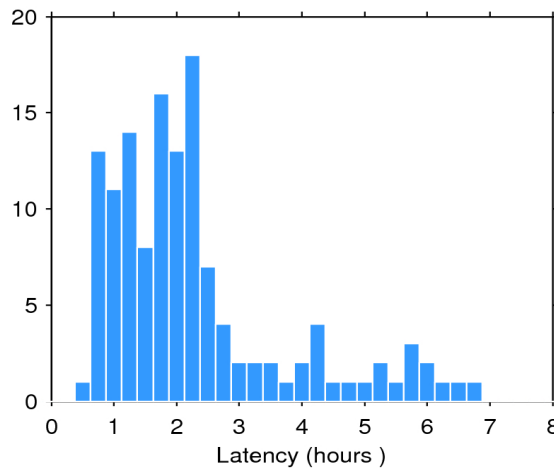
Figure 2. Histogram of the data latency for 08/06/2016. The y-axis denotes the number of files that are made available with a delay of x-hours with respect to the mean time of the records stored in the file.
