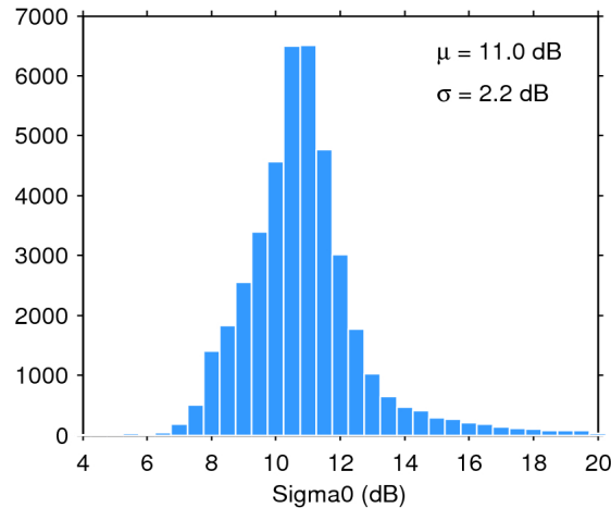
Figure 25. Histogram of flag-valid sigma0 over oceans and lakes for 07/06/2016. The mean ( \mu ) and standard deviation ( \sigma ) are also shown. Note that values outside [4 20] dB are excluded from the histogram for the sake of readability but not from the computation of \mu and \sigma .
