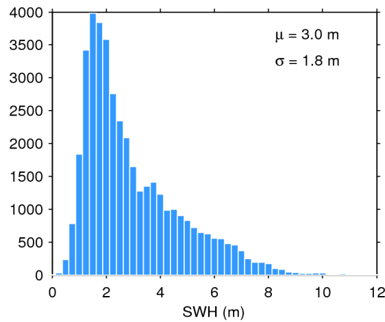
Figure 17. Histogram of flag-valid SWH over oceans and lakes for 07/06/2016. The mean ( \mu ) and standard deviation ( \sigma ) are also shown. Note that values larger than 12 m are excluded from the histogram for the sake of readability but not from the computation of \mu and \sigma .
