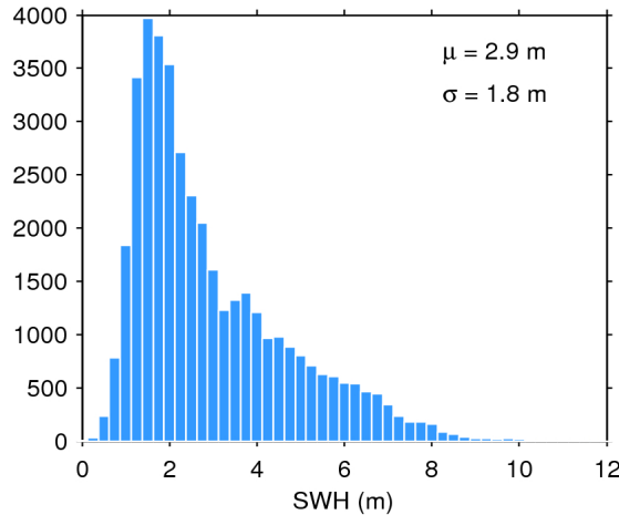
Figure 20. Histogram of science-valid SWH over oceans and lakes for 07/06/2016. The mean ( \mu ) and standard deviation ( \sigma ) are also shown. Note that values larger than 12 m are excluded from the histogram for the sake of readability but not from the computation of \mu and \sigma .
