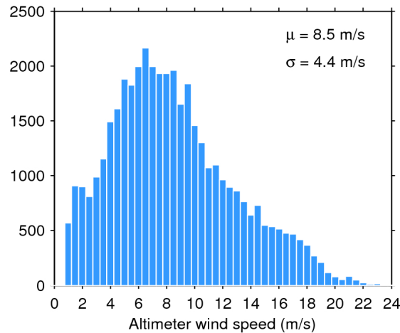
Figure 33. Histogram of flag-valid wind over oceans and lakes for 07/06/2016. The mean ( \mu ) and standard deviation ( \sigma ) are also shown. Note that values larger than 24 m/s are excluded from the histogram for the sake of readability but not from the computation of \mu and \sigma .
