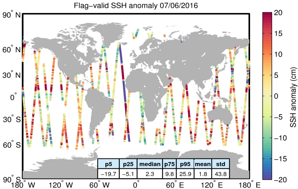
Figure 5. Geographical distribution of flag-valid 1-Hz SSH anomaly data over oceans and lakes for 07/06/2016. The statistical values shown in the table refer to the SSH anomaly in cm and are calculated over all measurements shown in the figure.
