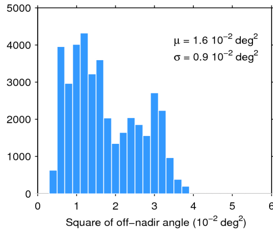
Figure 39. Histogram of flag-valid mispointing over oceans and lakes for 07/06/2016. The mean ( \mu ) and standard deviation ( \sigma ) are also shown. Note that values larger than 6 \cdot 10^{-2} \text{ deg}^2 are excluded from the histogram for the sake of readability but not from the computation of \mu and \sigma .
