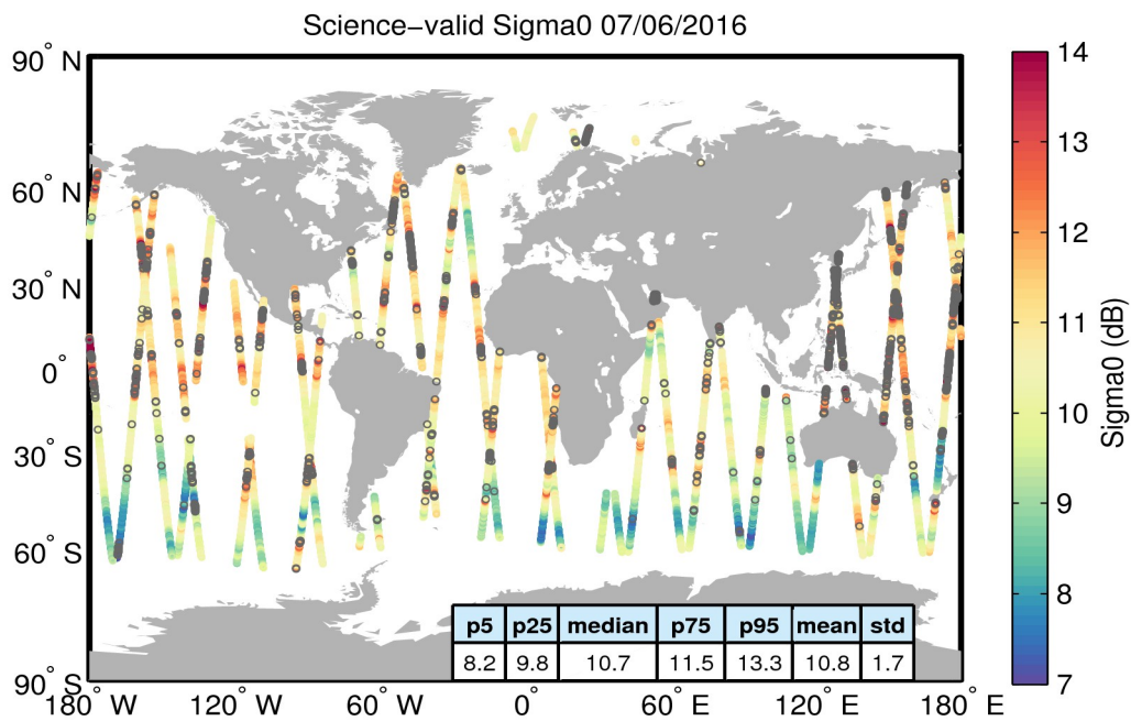
Figure 27. Geographical distribution of science-valid sigma0 data over oceans and lakes for 07/06/2016. The statistical values shown in the table refer to the sigma0 in dB and are calculated over all measurements shown in the figure. Gray circles denote records that have been rejected based on the editing criteria described in Table 4.
