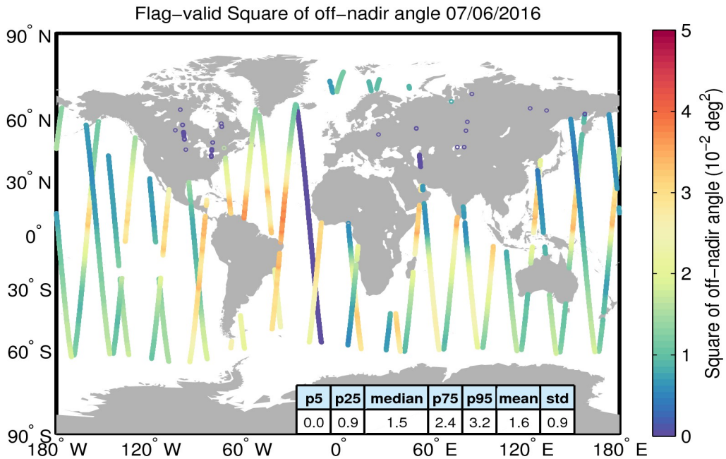
Figure 37. Geographical distribution of flag-valid mispointing data over oceans and lakes for 07/06/2016. The statistical values shown in the table refer to the mispointing in 10^{-2} \text{ deg}^2 and are calculated over all measurements shown in the figure.
