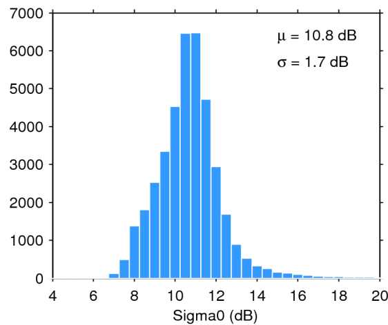
Figure 28. Histogram of science-valid sigma0 over oceans and lakes for 07/06/2016. The mean ( \mu ) and standard deviation ( \sigma ) are also shown. Note that values outside [4 20] dB are excluded from the histogram for the sake of readability but not from the computation of \mu and \sigma .
