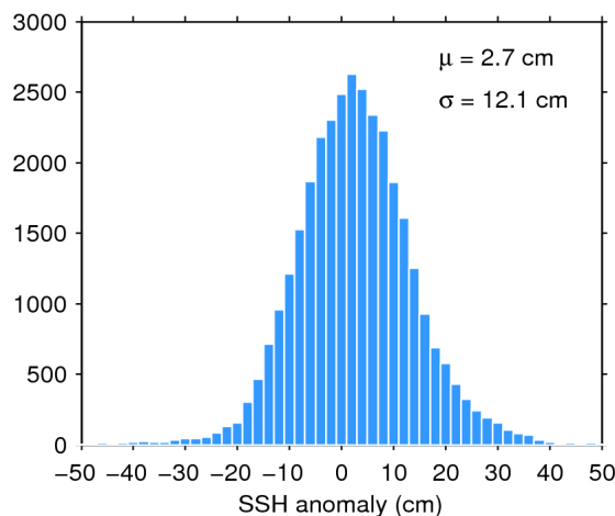
Figure 11. Histogram of science-valid SSH anomaly over oceans and lakes for 07/06/2016. The mean ( \mu ) and standard deviation ( \sigma ) are also shown. Note that values outside [-50 50] cm are excluded from the histogram for the sake of readability but not from the computation of \mu and \sigma .
