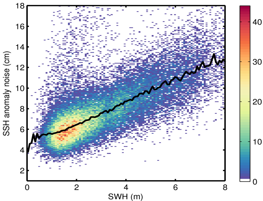
Figure 9. 2D histogram showing flag-valid SSH anomaly noise as a function of SWH for 07/06/2016. The black line denotes the median SSH anomaly noise as a function of SWH.
