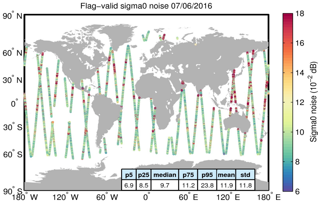
Figure 26. Geographical distribution of flag-valid 20-Hz sigma0 measurement noise over oceans and lakes for 07/06/2016. The statistical values shown in the table refer to the sigma0 noise and are calculated over all measurements shown in the figure.
