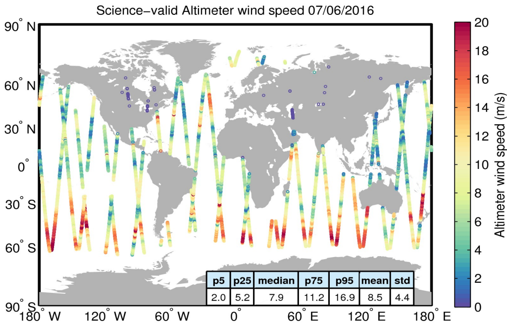
Figure 34. Geographical distribution of science-valid wind data over oceans and lakes for 07/06/2016. The statistical values shown in the table refer to the wind in m/s and are calculated over all measurements shown in the figure. Gray circles denote records that have been rejected based on the editing criteria described in Table 5.
