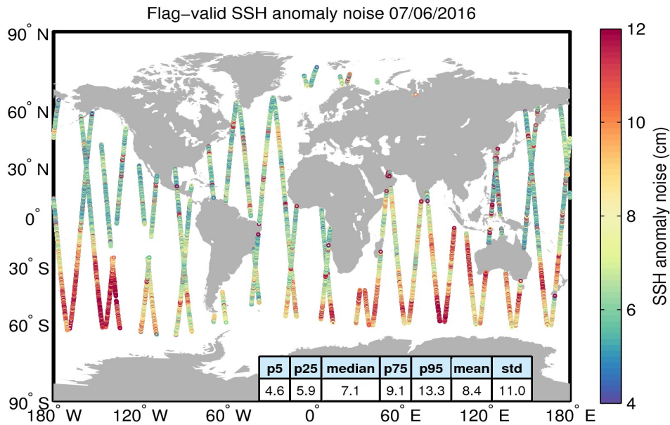
Figure 8. Geographical distribution of flag-valid 20-Hz SSH anomaly measurement noise over oceans and lakes for 07/06/2016. The statistical values shown in the table refer to the SSH anomaly noise and are calculated over all measurements shown in the figure.
