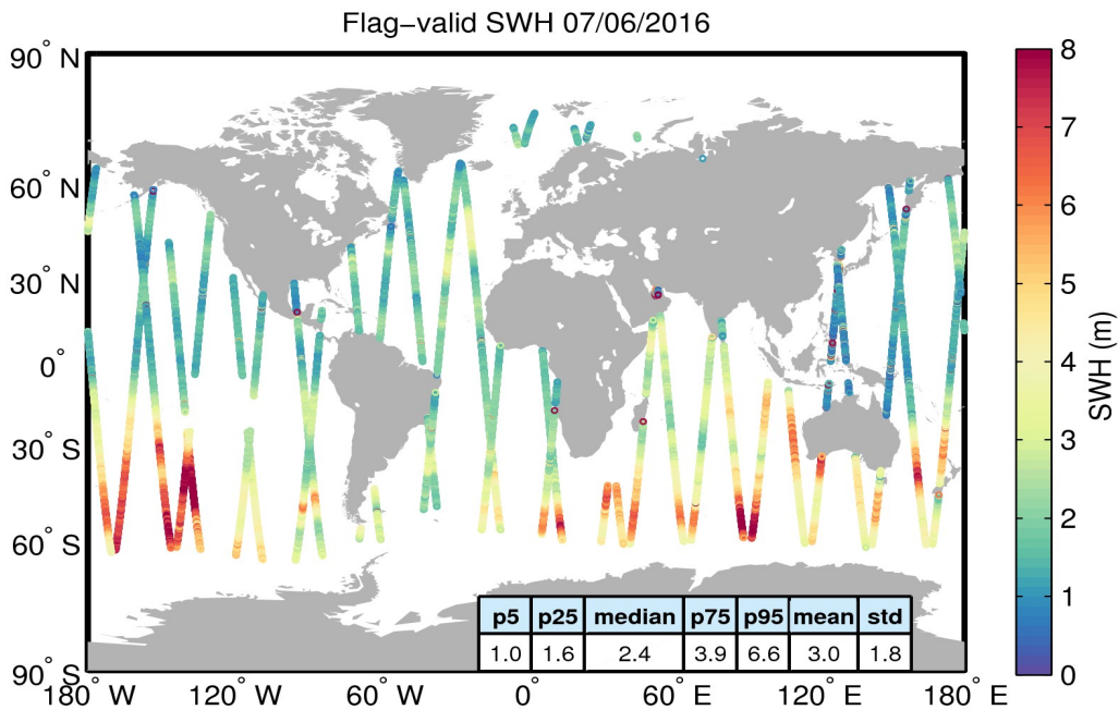
Figure 15. Geographical distribution of flag-valid SWH data over oceans and lakes for 07/06/2016. The statistical values shown in the table refer to the SWH in m and are calculated over all measurements shown in the figure.
