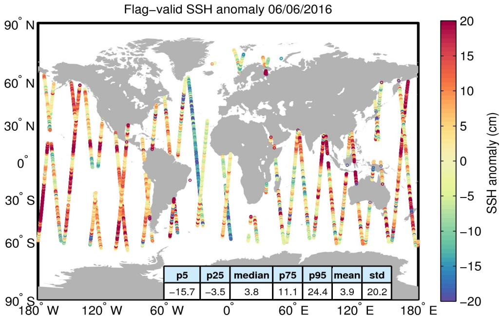
Figure 5. Geographical distribution of flag-valid 1-Hz SSH anomaly data over oceans and lakes for 06/06/2016. The statistical values shown in the table refer to the SSH anomaly in cm and are calculated over all measurements shown in the figure.
