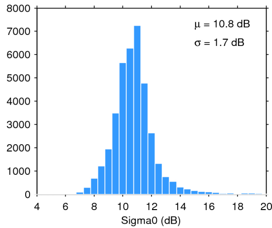
Figure 28. Histogram of science-valid sigma0 over oceans and lakes for 06/06/2016. The mean ( \mu ) and standard deviation ( \sigma ) are also shown. Note that values outside [4 20] dB are excluded from the histogram for the sake of readability but not from the computation of \mu and \sigma .
