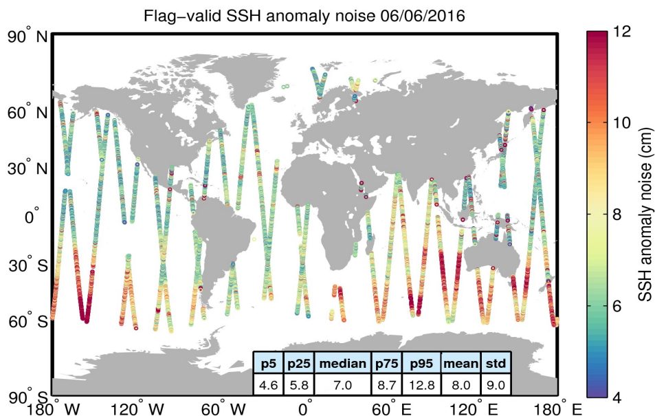
Figure 8. Geographical distribution of flag-valid 20-Hz SSH anomaly measurement noise over oceans and lakes for 06/06/2016. The statistical values shown in the table refer to the SSH anomaly noise and are calculated over all measurements shown in the figure.
