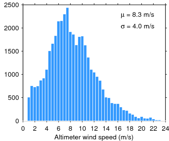
Figure 33. Histogram of flag-valid wind over oceans and lakes for 06/06/2016. The mean ( \mu ) and standard deviation ( \sigma ) are also shown. Note that values larger than 24 m/s are excluded from the histogram for the sake of readability but not from the computation of \mu and \sigma .
