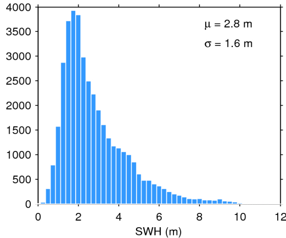
Figure 20. Histogram of science-valid SWH over oceans and lakes for 06/06/2016. The mean ( \mu ) and standard deviation ( \sigma ) are also shown. Note that values larger than 12 m are excluded from the histogram for the sake of readability but not from the computation of \mu and \sigma .
