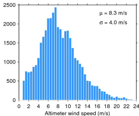
Figure 35. Histogram of science-valid wind over oceans and lakes for 06/06/2016. The mean ( \mu ) and standard deviation ( \sigma ) are also shown. Note that values larger than 24 m/s are excluded from the histogram for the sake of readability but not from the computation of \mu and \sigma .
