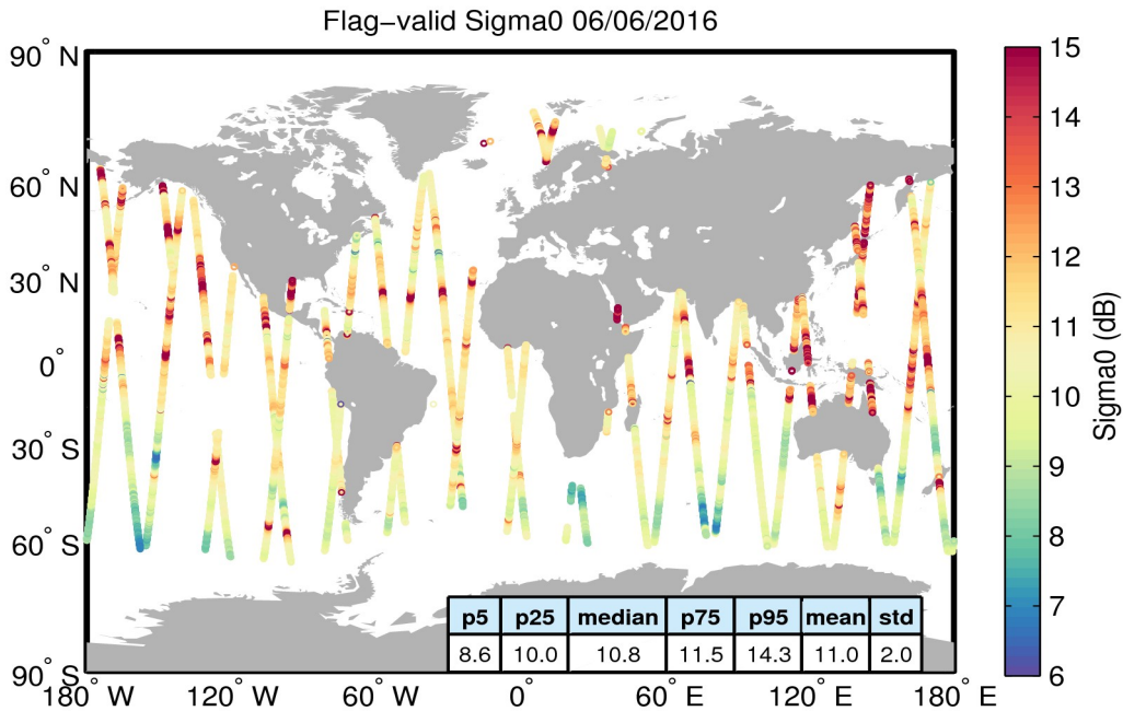
Figure 23. Geographical distribution of flag-valid sigma0 data over oceans and lakes for 06/06/2016. The statistical values shown in the table refer to the sigma0 in dB and are calculated over all measurements shown in the figure.
