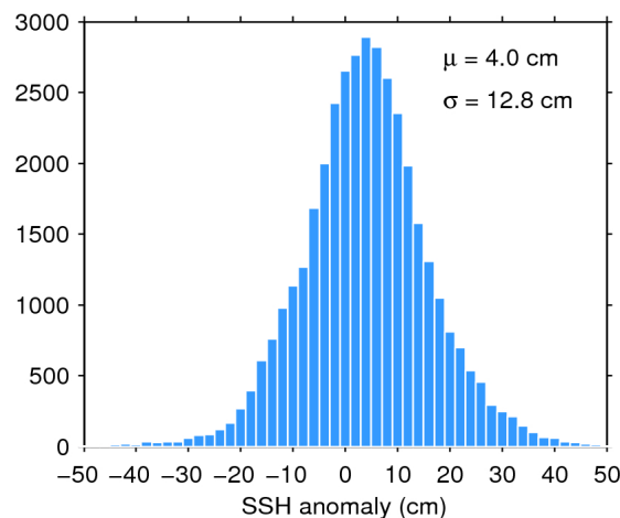
Figure 11. Histogram of science-valid SSH anomaly over oceans and lakes for 06/06/2016. The mean ( \mu ) and standard deviation ( \sigma ) are also shown. Note that values outside [-50 50] cm are excluded from the histogram for the sake of readability but not from the computation of \mu and \sigma .
