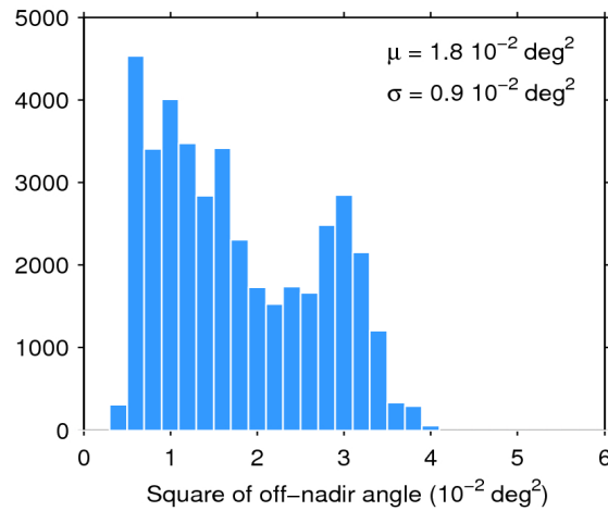
Figure 39. Histogram of flag-valid mispointing over oceans and lakes for 06/06/2016. The mean ( \mu ) and standard deviation ( \sigma ) are also shown. Note that values larger than 6 \cdot 10^{-2} \text{ deg}^2 are excluded from the histogram for the sake of readability but not from the computation of \mu and \sigma .
