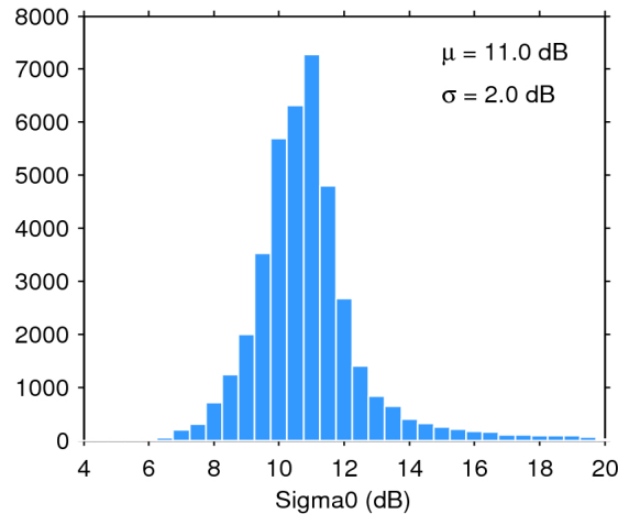
Figure 25. Histogram of flag-valid sigma0 over oceans and lakes for 06/06/2016. The mean ( \mu ) and standard deviation ( \sigma ) are also shown. Note that values outside [4 20] dB are excluded from the histogram for the sake of readability but not from the computation of \mu and \sigma .
