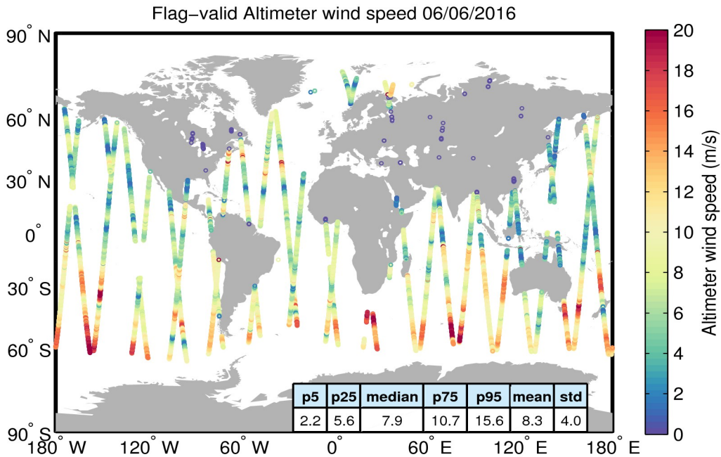
Figure 31. Geographical distribution of flag-valid wind data over oceans and lakes for 06/06/2016. The statistical values shown in the table refer to the wind in m/s and are calculated over all measurements shown in the figure.
