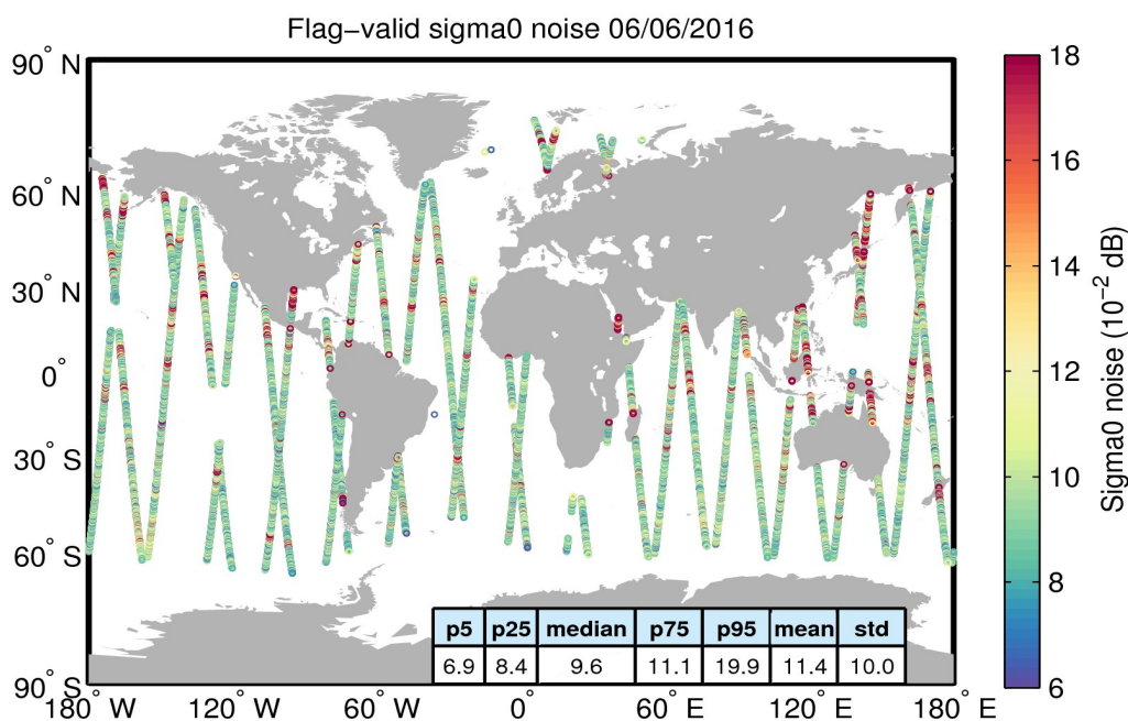
Figure 26. Geographical distribution of flag-valid 20-Hz sigma0 measurement noise over oceans and lakes for 06/06/2016. The statistical values shown in the table refer to the sigma0 noise and are calculated over all measurements shown in the figure.
