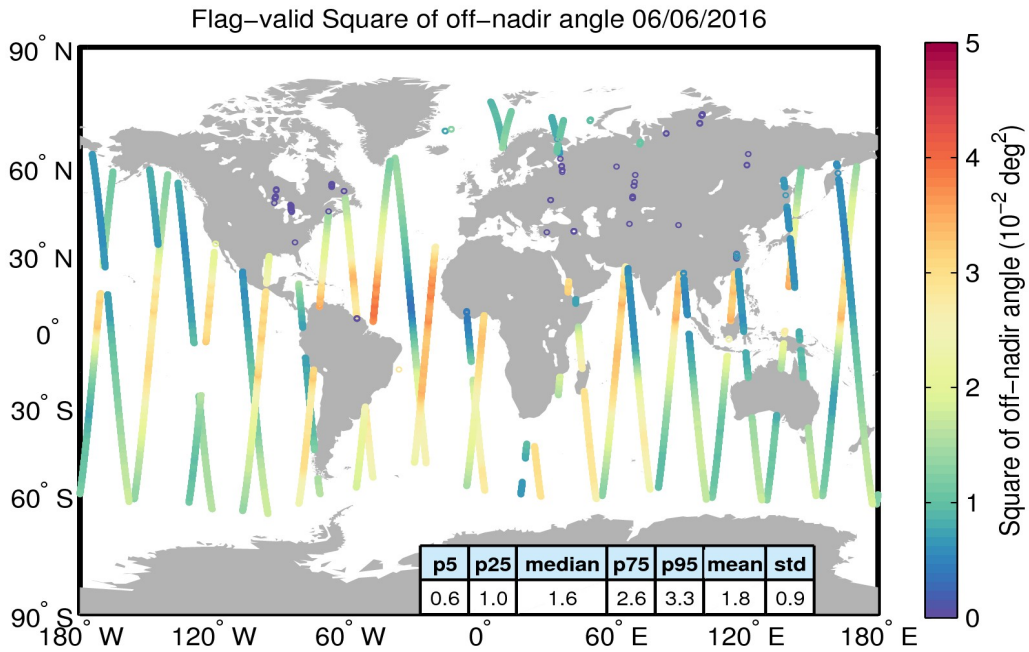
Figure 37. Geographical distribution of flag-valid mispointing data over oceans and lakes for 06/06/2016. The statistical values shown in the table refer to the mispointing in 10^{-2} \text{deg}^2 and are calculated over all measurements shown in the figure.
