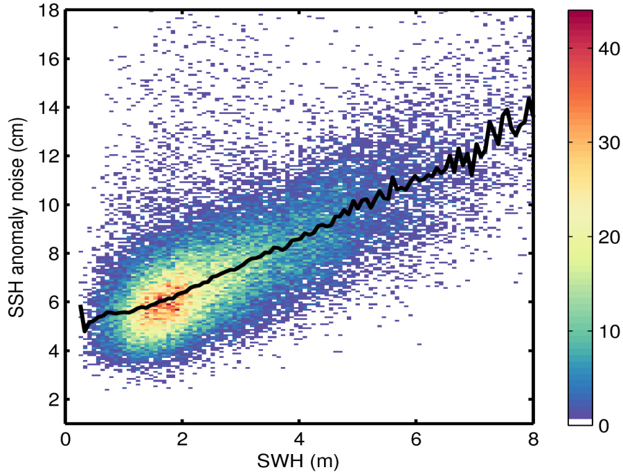
Figure 9. 2D histogram showing flag-valid SSH anomaly noise as a function of SWH for 06/06/2016. The black line denotes the median SSH anomaly noise as a function of SWH.
