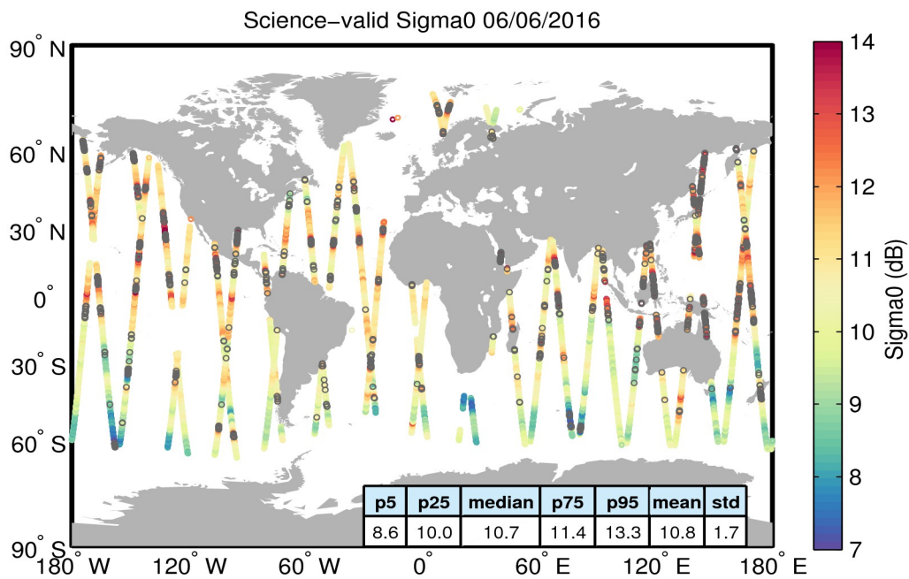
Figure 27. Geographical distribution of science-valid sigma0 data over oceans and lakes for 06/06/2016. The statistical values shown in the table refer to the sigma0 in dB and are calculated over all measurements shown in the figure. Gray circles denote records that have been rejected based on the editing criteria described in Table 4.
