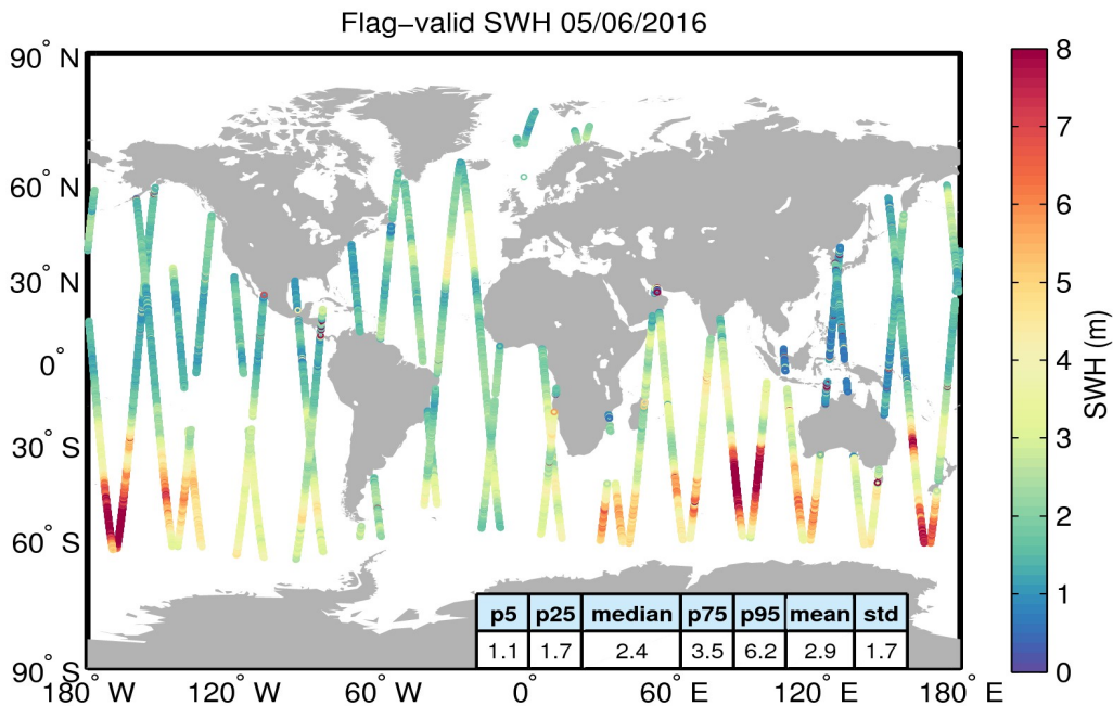
Figure 15. Geographical distribution of flag-valid SWH data over oceans and lakes for 05/06/2016. The statistical values shown in the table refer to the SWH in m and are calculated over all measurements shown in the figure.
