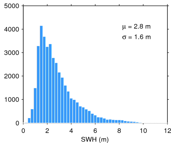
Figure 20. Histogram of science-valid SWH over oceans and lakes for 05/06/2016. The mean ( \mu ) and standard deviation ( \sigma ) are also shown. Note that values larger than 12 m are excluded from the histogram for the sake of readability but not from the computation of \mu and \sigma .
