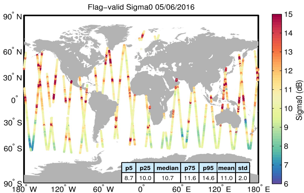
Figure 23. Geographical distribution of flag-valid sigma0 data over oceans and lakes for 05/06/2016. The statistical values shown in the table refer to the sigma0 in dB and are calculated over all measurements shown in the figure.
