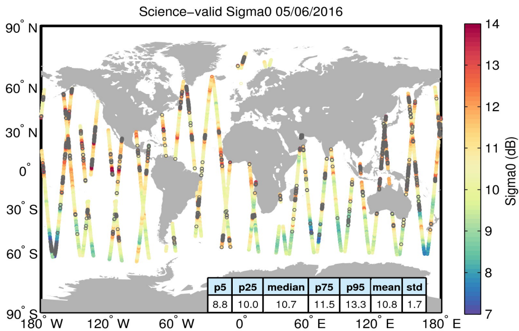
Figure 27. Geographical distribution of science-valid sigma0 data over oceans and lakes for 05/06/2016. The statistical values shown in the table refer to the sigma0 in dB and are calculated over all measurements shown in the figure. Gray circles denote records that have been rejected based on the editing criteria described in Table 4.
