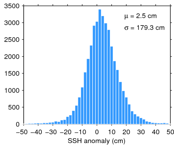
Figure 7. Histogram of flag-valid SSH anomaly over oceans and lakes for 05/06/2016. The mean ( \mu ) and standard deviation ( \sigma ) are also shown. Note that values outside [-50\ 50] cm are excluded from the histogram for the sake of readability but not from the computation of \mu and \sigma .
