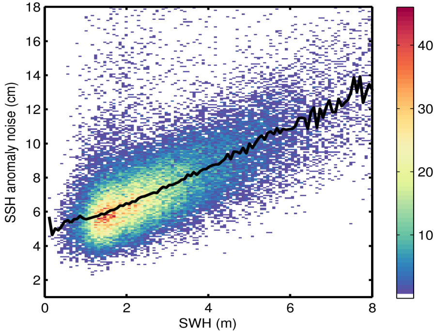
Figure 9. 2D histogram showing flag-valid SSH anomaly noise as a function of SWH for 05/06/2016. The black line denotes the median SSH anomaly noise as a function of SWH.
