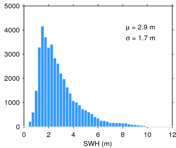
Figure 17. Histogram of flag-valid SWH over oceans and lakes for 05/06/2016. The mean ( \mu ) and standard deviation ( \sigma ) are also shown. Note that values larger than 12 m are excluded from the histogram for the sake of readability but not from the computation of \mu and \sigma .
