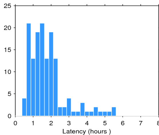
Figure 2. Histogram of the data latency for 05/06/2016. The y-axis denotes the number of files that are made available with a delay of x-hours with respect to the mean time of the records stored in the file.
