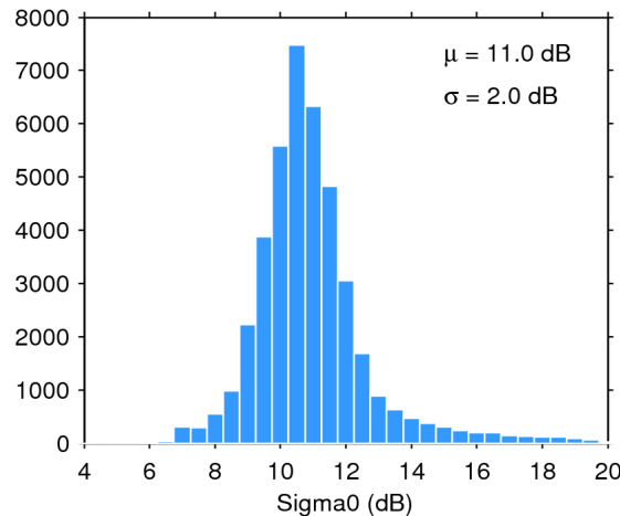
Figure 25. Histogram of flag-valid sigma0 over oceans and lakes for 05/06/2016. The mean ( \mu ) and standard deviation ( \sigma ) are also shown. Note that values outside [4 20] dB are excluded from the histogram for the sake of readability but not from the computation of \mu and \sigma .
