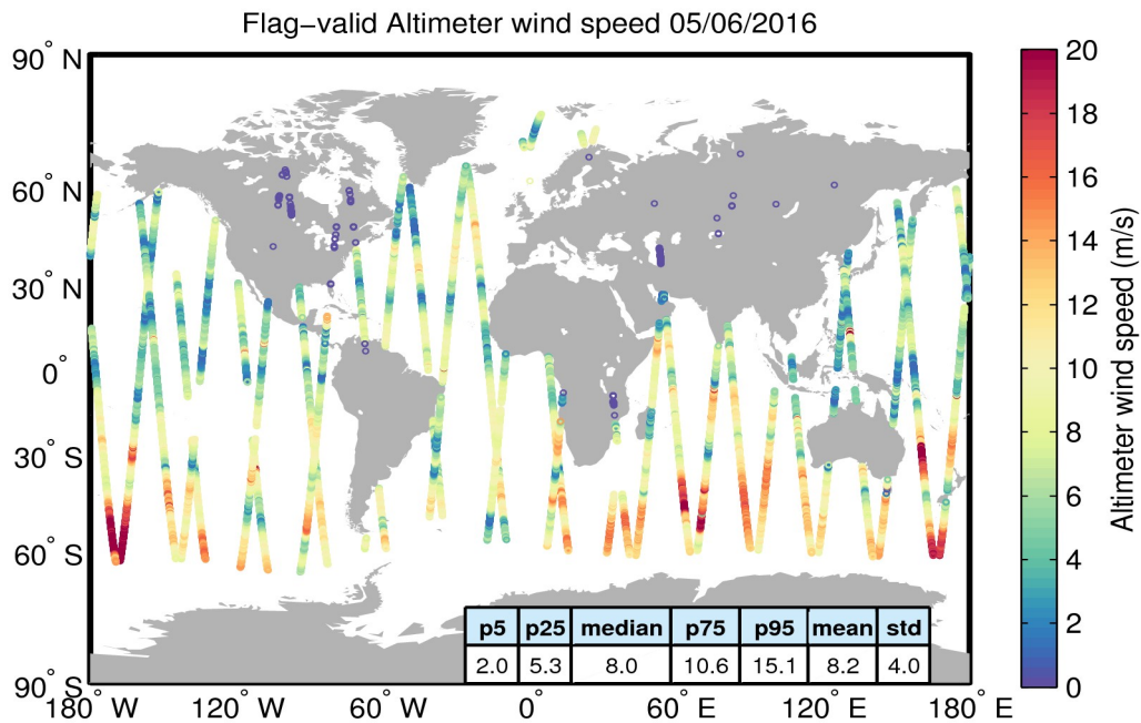
Figure 31. Geographical distribution of flag-valid wind data over oceans and lakes for 05/06/2016. The statistical values shown in the table refer to the wind in m/s and are calculated over all measurements shown in the figure.
