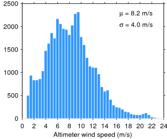
Figure 33. Histogram of flag-valid wind over oceans and lakes for 05/06/2016. The mean ( \mu ) and standard deviation ( \sigma ) are also shown. Note that values larger than 24 m/s are excluded from the histogram for the sake of readability but not from the computation of \mu and \sigma .
