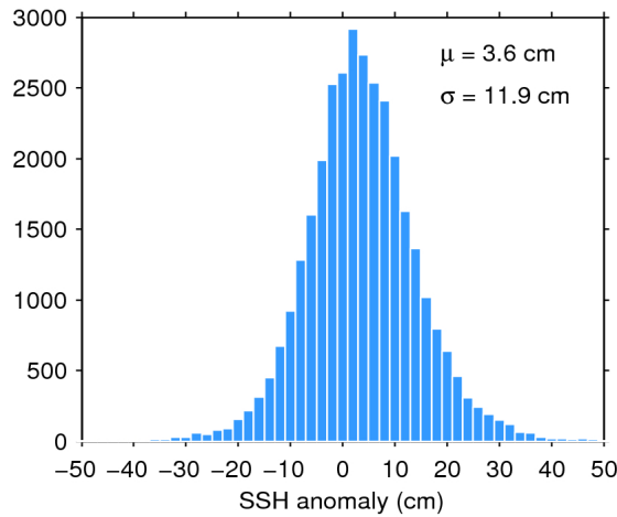
Figure 11. Histogram of science-valid SSH anomaly over oceans and lakes for 05/06/2016. The mean ( \mu ) and standard deviation ( \sigma ) are also shown. Note that values outside [-50 50] cm are excluded from the histogram for the sake of readability but not from the computation of \mu and \sigma .
