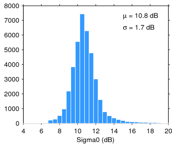
Figure 28. Histogram of science-valid sigma0 over oceans and lakes for 05/06/2016. The mean ( \mu ) and standard deviation ( \sigma ) are also shown. Note that values outside [4 20] dB are excluded from the histogram for the sake of readability but not from the computation of \mu and \sigma .
