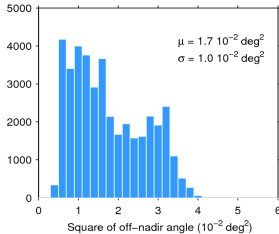
Figure 39. Histogram of flag-valid mispointing over oceans and lakes for 05/06/2016. The mean ( \mu ) and standard deviation ( \sigma ) are also shown. Note that values larger than 6 \cdot 10^{-2} \text{ deg}^2 are excluded from the histogram for the sake of readability but not from the computation of \mu and \sigma .
