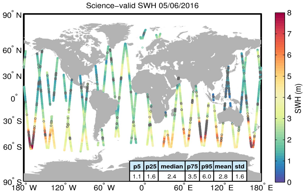
Figure 19. Geographical distribution of science-valid SWH data over oceans and lakes for 05/06/2016. The statistical values shown in the table refer to the SWH in m and are calculated over all measurements shown in the figure. Gray circles denote records that have been rejected based on the editing criteria described in Table 3.
