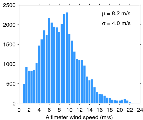
Figure 35. Histogram of science-valid wind over oceans and lakes for 05/06/2016. The mean ( \mu ) and standard deviation ( \sigma ) are also shown. Note that values larger than 24 m/s are excluded from the histogram for the sake of readability but not from the computation of \mu and \sigma .
