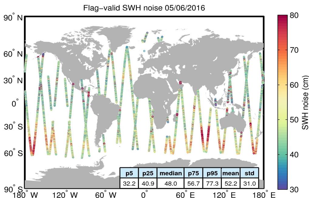
Figure 18. Geographical distribution of flag-valid 20-Hz SWH measurement noise over oceans and lakes for 05/06/2016. The statistical values shown in the figure refer to the SWH noise and are calculated over all measurements shown in the figure.
