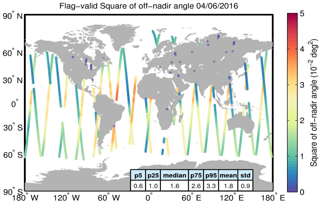
Figure 37. Geographical distribution of flag-valid mispointing data over oceans and lakes for 04/06/2016. The statistical values shown in the table refer to the mispointing in 10^{-2} \text{ deg}^2 and are calculated over all measurements shown in the figure.
