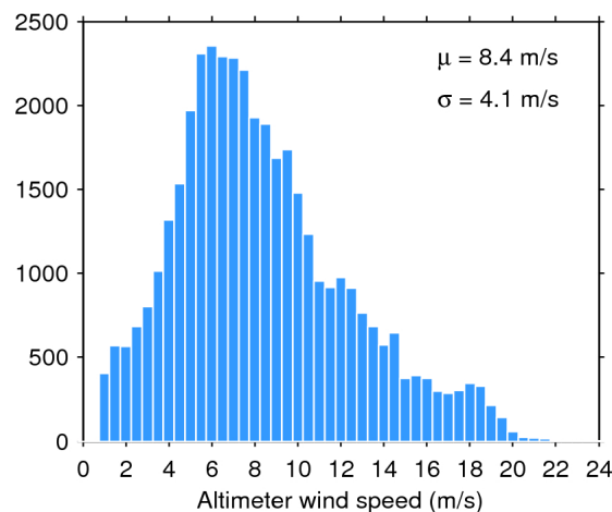
Figure 35. Histogram of science-valid wind over oceans and lakes for 04/06/2016. The mean ( \mu ) and standard deviation ( \sigma ) are also shown. Note that values larger than 24 m/s are excluded from the histogram for the sake of readability but not from the computation of \mu and \sigma .
