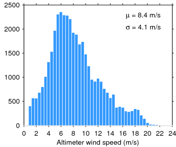
Figure 33. Histogram of flag-valid wind over oceans and lakes for 04/06/2016. The mean ( \mu ) and standard deviation ( \sigma ) are also shown. Note that values larger than 24 m/s are excluded from the histogram for the sake of readability but not from the computation of \mu and \sigma .
