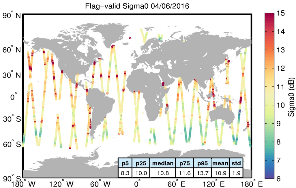
Figure 23. Geographical distribution of flag-valid sigma0 data over oceans and lakes for 04/06/2016. The statistical values shown in the table refer to the sigma0 in dB and are calculated over all measurements shown in the figure.
