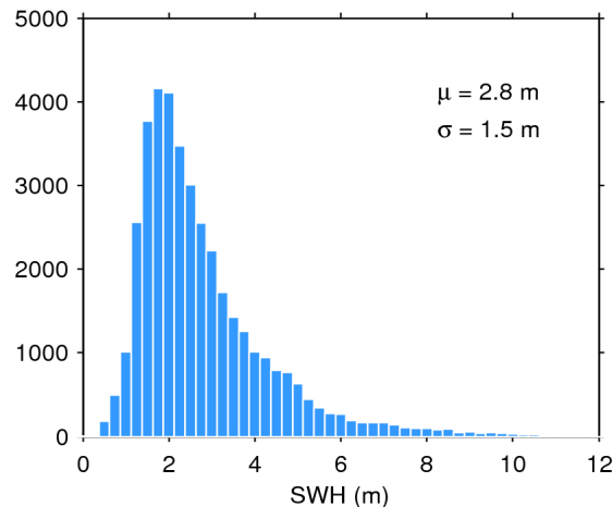
Figure 20. Histogram of science-valid SWH over oceans and lakes for 04/06/2016. The mean ( \mu ) and standard deviation ( \sigma ) are also shown. Note that values larger than 12 m are excluded from the histogram for the sake of readability but not from the computation of \mu and \sigma .
