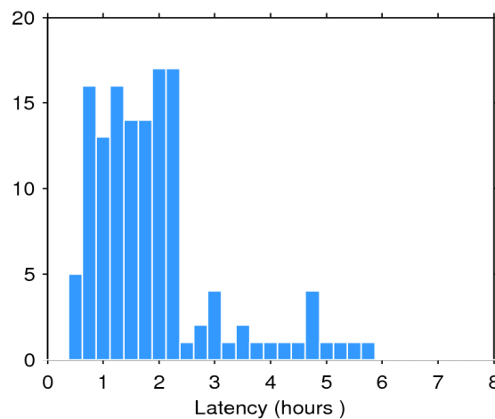
Figure 2. Histogram of the data latency for 04/06/2016. The y-axis denotes the number of files that are made available with a delay of x-hours with respect to the mean time of the records stored in the file.
