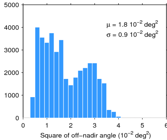
Figure 39. Histogram of flag-valid mispointing over oceans and lakes for 04/06/2016. The mean ( \mu ) and standard deviation ( \sigma ) are also shown. Note that values larger than 6 \cdot 10^{-2} \text{ deg}^2 are excluded from the histogram for the sake of readability but not from the computation of \mu and \sigma .
