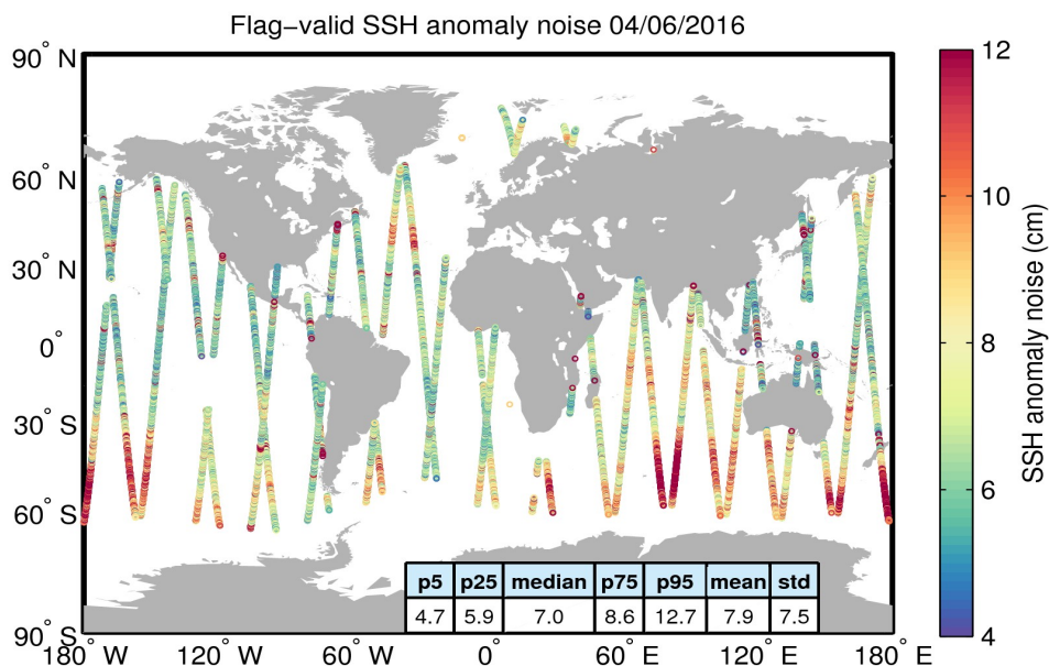
Figure 8. Geographical distribution of flag-valid 20-Hz SSH anomaly measurement noise over oceans and lakes for 04/06/2016. The statistical values shown in the table refer to the SSH anomaly noise and are calculated over all measurements shown in the figure.
