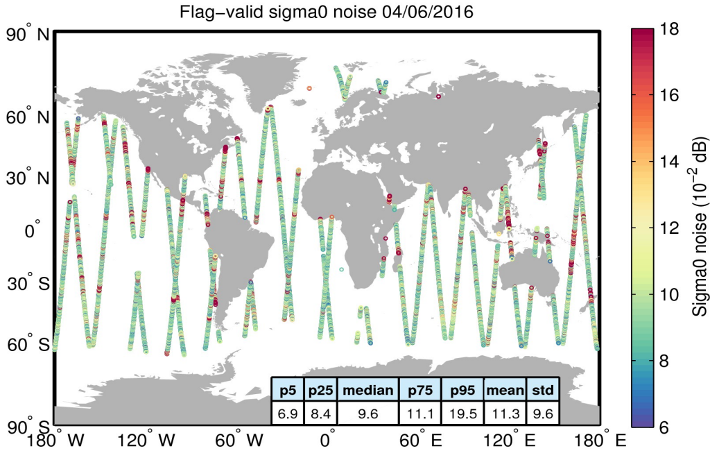
Figure 26. Geographical distribution of flag-valid 20-Hz sigma0 measurement noise over oceans and lakes for 04/06/2016. The statistical values shown in the table refer to the sigma0 noise and are calculated over all measurements shown in the figure.
