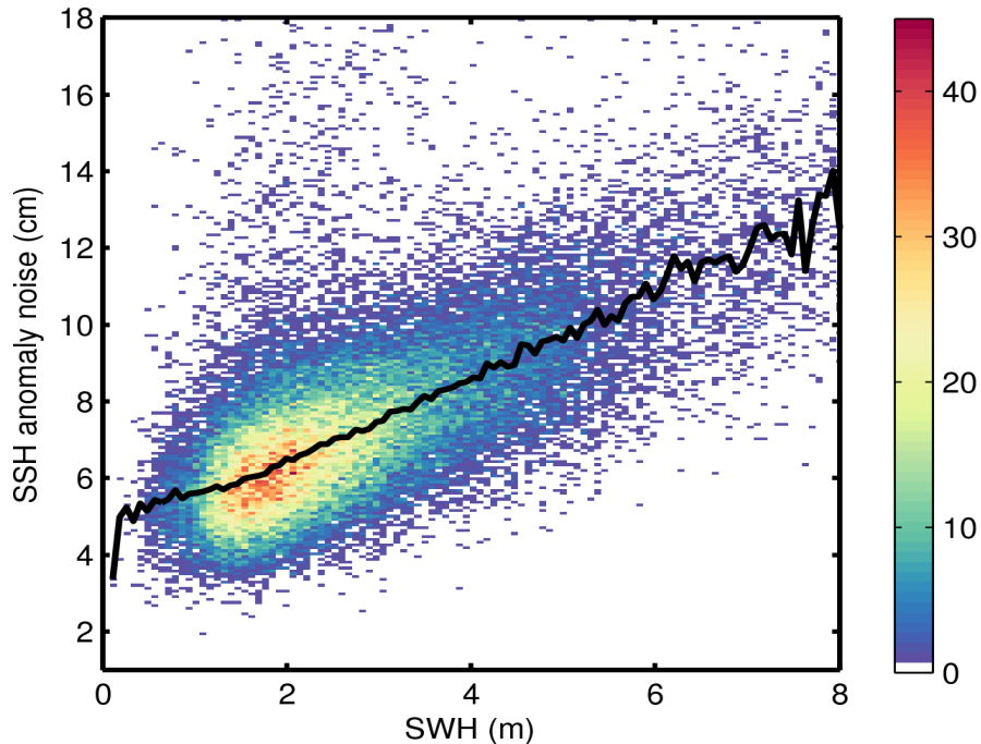
Figure 9. 2D histogram showing flag-valid SSH anomaly noise as a function of SWH for 04/06/2016. The black line denotes the median SSH anomaly noise as a function of SWH.
