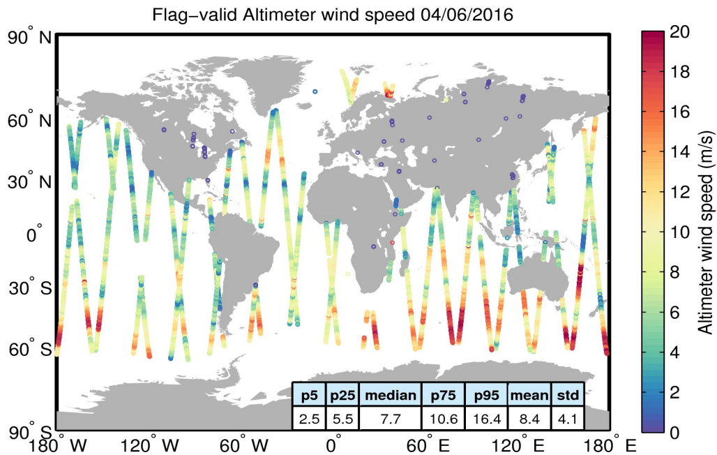
Figure 31. Geographical distribution of flag-valid wind data over oceans and lakes for 04/06/2016. The statistical values shown in the table refer to the wind in m/s and are calculated over all measurements shown in the figure.
