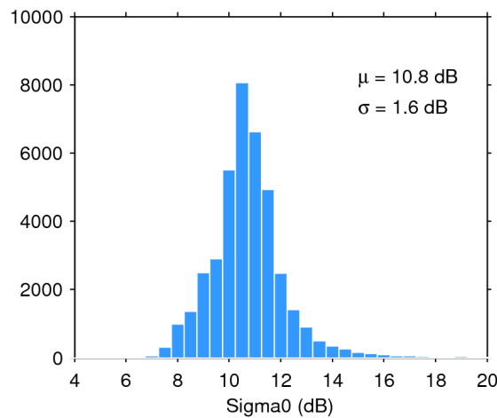
Figure 28. Histogram of science-valid sigma0 over oceans and lakes for 03/06/2016. The mean ( \mu ) and standard deviation ( \sigma ) are also shown. Note that values outside [4 20] dB are excluded from the histogram for the sake of readability but not from the computation of \mu and \sigma .
