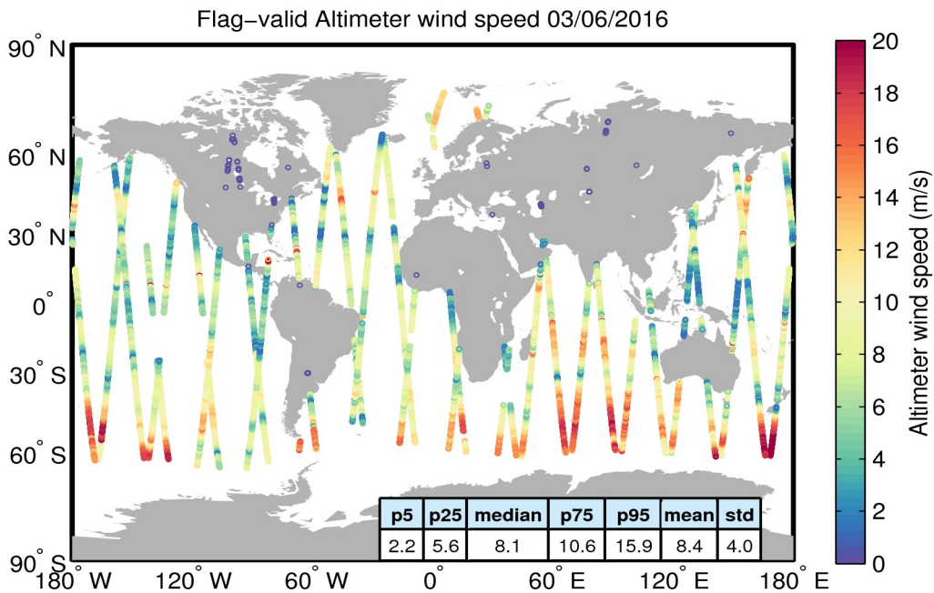
Figure 31. Geographical distribution of flag-valid wind data over oceans and lakes for 03/06/2016. The statistical values shown in the table refer to the wind in m/s and are calculated over all measurements shown in the figure.
