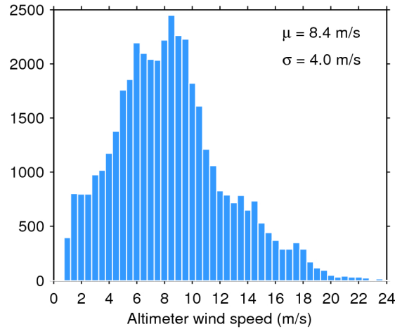
Figure 33. Histogram of flag-valid wind over oceans and lakes for 03/06/2016. The mean ( \mu ) and standard deviation ( \sigma ) are also shown. Note that values larger than 24 m/s are excluded from the histogram for the sake of readability but not from the computation of \mu and \sigma .
