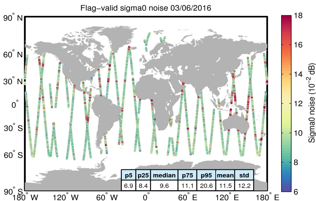
Figure 26. Geographical distribution of flag-valid 20-Hz sigma0 measurement noise over oceans and lakes for 03/06/2016. The statistical values shown in the table refer to the sigma0 noise and are calculated over all measurements shown in the figure.
