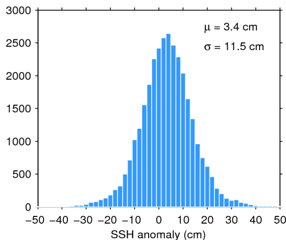
Figure 11. Histogram of science-valid SSH anomaly over oceans and lakes for 03/06/2016. The mean ( \mu ) and standard deviation ( \sigma ) are also shown. Note that values outside [-50 50] cm are excluded from the histogram for the sake of readability but not from the computation of \mu and \sigma .
