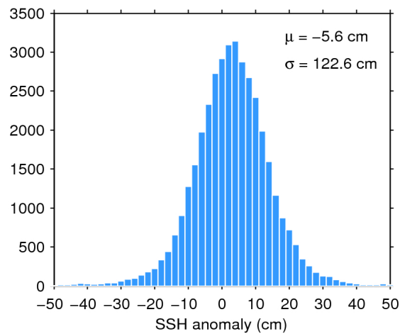
Figure 7. Histogram of flag-valid SSH anomaly over oceans and lakes for 03/06/2016. The mean ( \mu ) and standard deviation ( \sigma ) are also shown. Note that values outside [-50 50] cm are excluded from the histogram for the sake of readability but not from the computation of \mu and \sigma .
