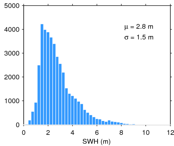
Figure 17. Histogram of flag-valid SWH over oceans and lakes for 03/06/2016. The mean ( \mu ) and standard deviation ( \sigma ) are also shown. Note that values larger than 12 m are excluded from the histogram for the sake of readability but not from the computation of \mu and \sigma .
