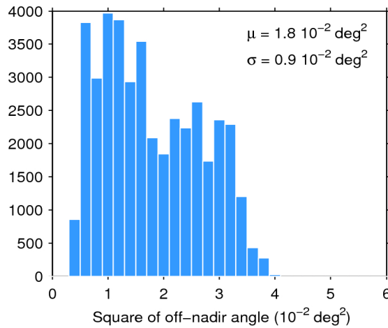
Figure 39. Histogram of flag-valid mispointing over oceans and lakes for 03/06/2016. The mean ( \mu ) and standard deviation ( \sigma ) are also shown. Note that values larger than 6 \cdot 10^{-2} \text{ deg}^2 are excluded from the histogram for the sake of readability but not from the computation of \mu and \sigma .
