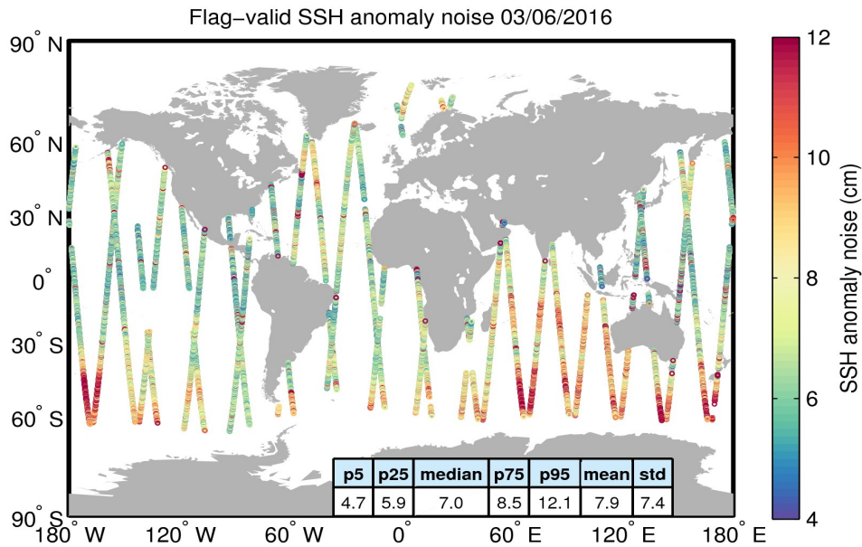
Figure 8. Geographical distribution of flag-valid 20-Hz SSH anomaly measurement noise over oceans and lakes for 03/06/2016. The statistical values shown in the table refer to the SSH anomaly noise and are calculated over all measurements shown in the figure.
