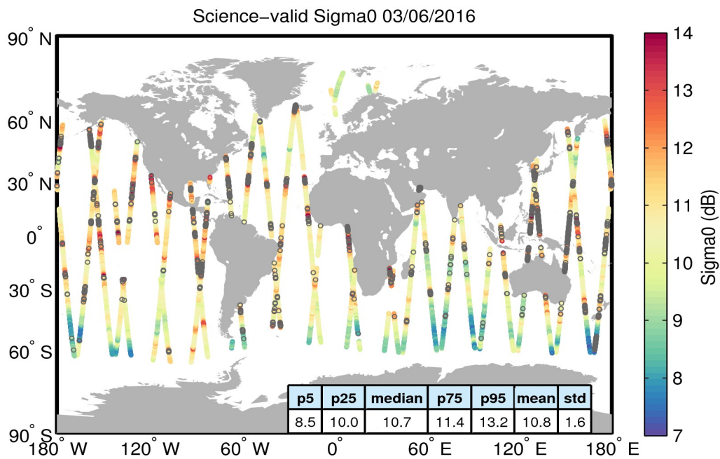
Figure 27. Geographical distribution of science-valid sigma0 data over oceans and lakes for 03/06/2016. The statistical values shown in the table refer to the sigma0 in dB and are calculated over all measurements shown in the figure. Gray circles denote records that have been rejected based on the editing criteria described in Table 4.
