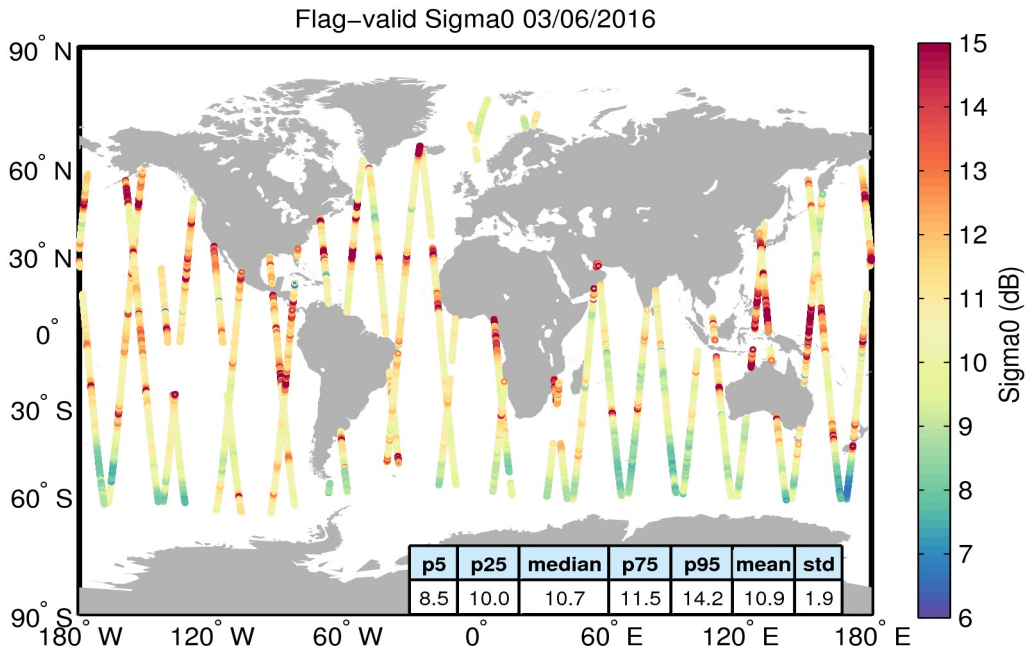
Figure 23. Geographical distribution of flag-valid sigma0 data over oceans and lakes for 03/06/2016. The statistical values shown in the table refer to the sigma0 in dB and are calculated over all measurements shown in the figure.
