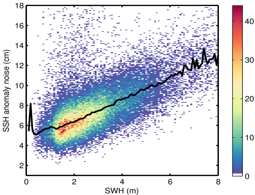
Figure 9. 2D histogram showing flag-valid SSH anomaly noise as a function of SWH for 03/06/2016. The black line denotes the median SSH anomaly noise as a function of SWH.
