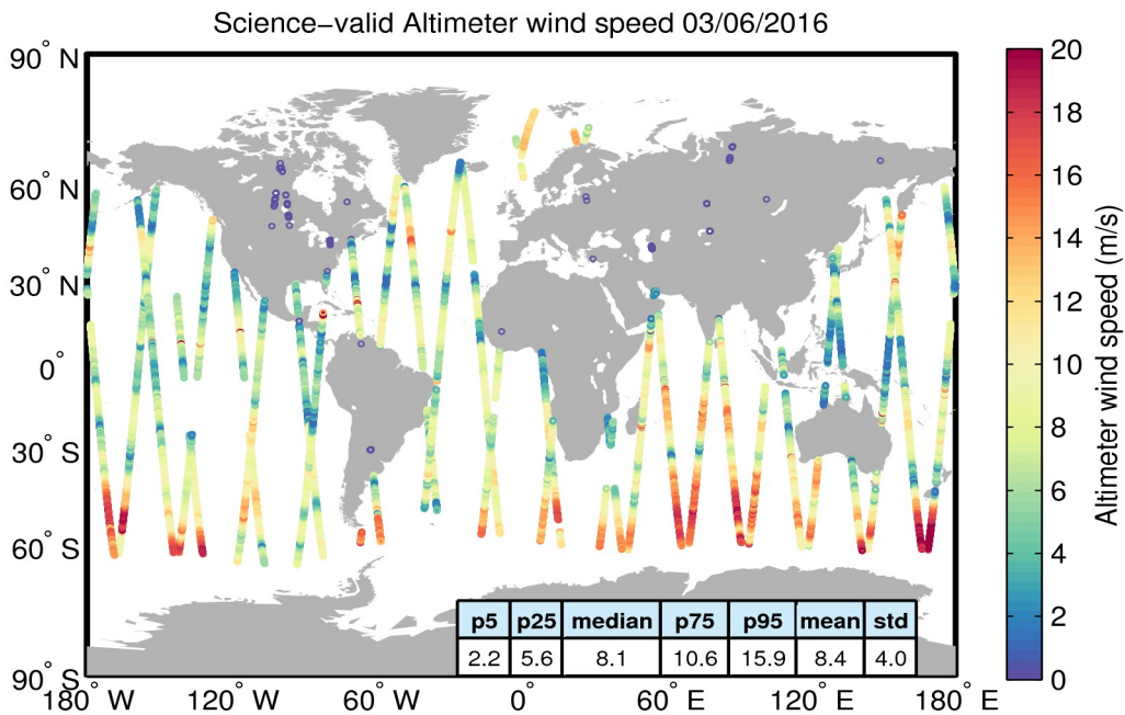
Figure 34. Geographical distribution of science-valid wind data over oceans and lakes for 03/06/2016. The statistical values shown in the table refer to the wind in m/s and are calculated over all measurements shown in the figure. Gray circles denote records that have been rejected based on the editing criteria described in Table 5.
