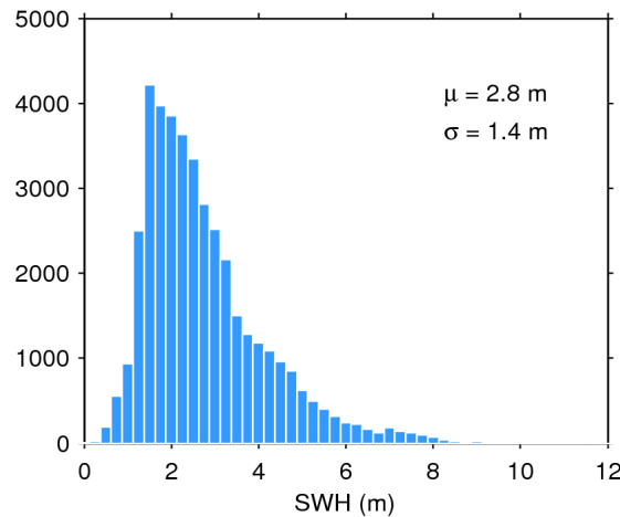
Figure 20. Histogram of science-valid SWH over oceans and lakes for 03/06/2016. The mean ( \mu ) and standard deviation ( \sigma ) are also shown. Note that values larger than 12 m are excluded from the histogram for the sake of readability but not from the computation of \mu and \sigma .
