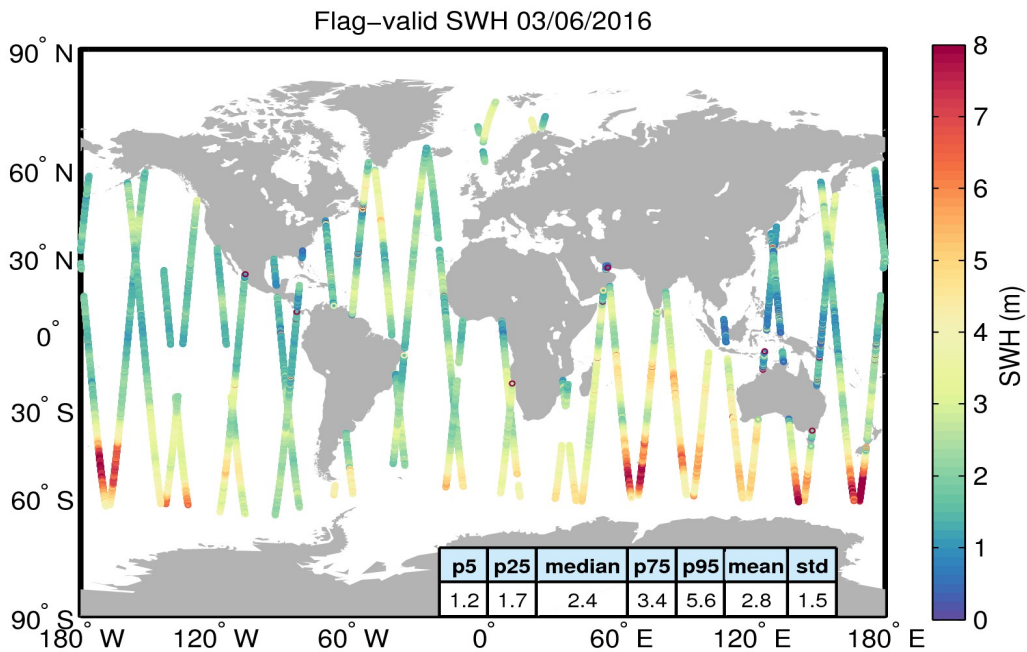
Figure 15. Geographical distribution of flag-valid SWH data over oceans and lakes for 03/06/2016. The statistical values shown in the table refer to the SWH in m and are calculated over all measurements shown in the figure.
