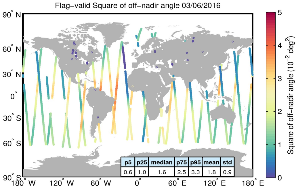
Figure 37. Geographical distribution of flag-valid mispointing data over oceans and lakes for 03/06/2016. The statistical values shown in the table refer to the mispointing in 10^{-2} \text{ deg}^2 and are calculated over all measurements shown in the figure.
