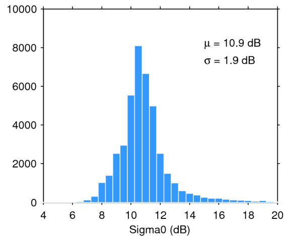
Figure 25. Histogram of flag-valid sigma0 over oceans and lakes for 03/06/2016. The mean ( \mu ) and standard deviation ( \sigma ) are also shown. Note that values outside [4 20] dB are excluded from the histogram for the sake of readability but not from the computation of \mu and \sigma .
