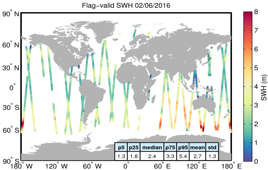
Figure 15. Geographical distribution of flag-valid SWH data over oceans and lakes for 02/06/2016. The statistical values shown in the table refer to the SWH in m and are calculated over all measurements shown in the figure.
