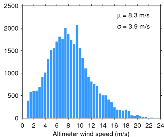
Figure 35. Histogram of science-valid wind over oceans and lakes for 02/06/2016. The mean ( \mu ) and standard deviation ( \sigma ) are also shown. Note that values larger than 24 m/s are excluded from the histogram for the sake of readability but not from the computation of \mu and \sigma .
