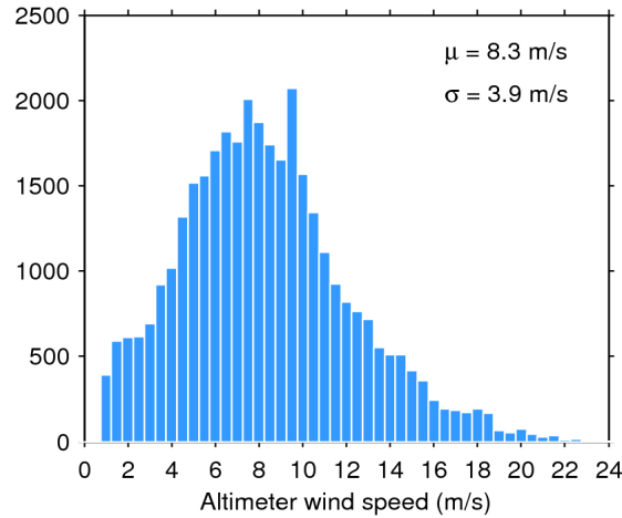
Figure 33. Histogram of flag-valid wind over oceans and lakes for 02/06/2016. The mean ( \mu ) and standard deviation ( \sigma ) are also shown. Note that values larger than 24 m/s are excluded from the histogram for the sake of readability but not from the computation of \mu and \sigma .
