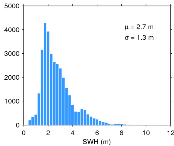
Figure 17. Histogram of flag-valid SWH over oceans and lakes for 02/06/2016. The mean ( \mu ) and standard deviation ( \sigma ) are also shown. Note that values larger than 12 m are excluded from the histogram for the sake of readability but not from the computation of \mu and \sigma .
