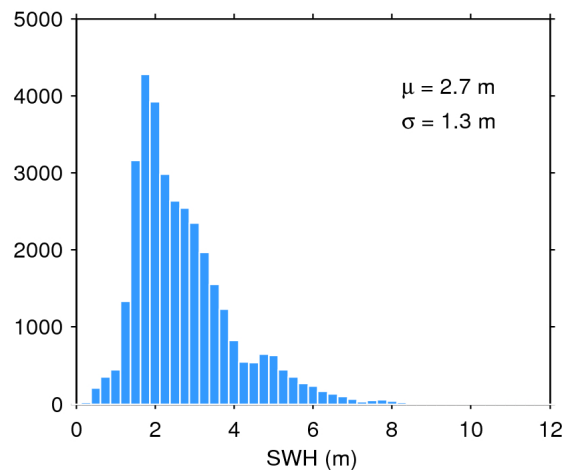
Figure 20. Histogram of science-valid SWH over oceans and lakes for 02/06/2016. The mean ( \mu ) and standard deviation ( \sigma ) are also shown. Note that values larger than 12 m are excluded from the histogram for the sake of readability but not from the computation of \mu and \sigma .
