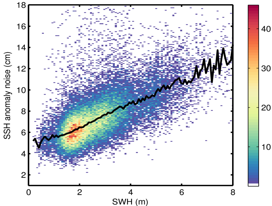
Figure 9. 2D histogram showing flag-valid SSH anomaly noise as a function of SWH for 02/06/2016. The black line denotes the median SSH anomaly noise as a function of SWH.
