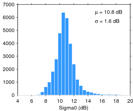
Figure 28. Histogram of science-valid sigma0 over oceans and lakes for 02/06/2016. The mean ( \mu ) and standard deviation ( \sigma ) are also shown. Note that values outside [4 20] dB are excluded from the histogram for the sake of readability but not from the computation of \mu and \sigma .
