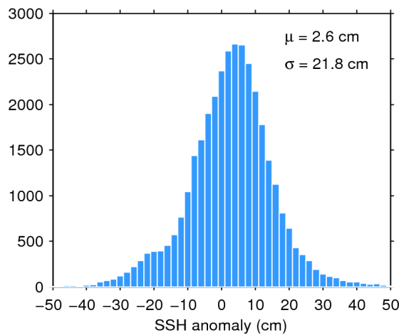
Figure 7. Histogram of flag-valid SSH anomaly over oceans and lakes for 02/06/2016. The mean ( \mu ) and standard deviation ( \sigma ) are also shown. Note that values outside [-50\ 50] cm are excluded from the histogram for the sake of readability but not from the computation of \mu and \sigma .
