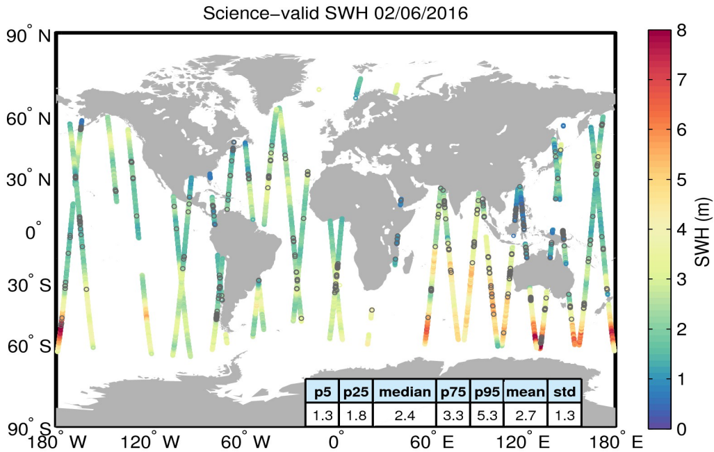
Figure 19. Geographical distribution of science-valid SWH data over oceans and lakes for 02/06/2016. The statistical values shown in the table refer to the SWH in m and are calculated over all measurements shown in the figure. Gray circles denote records that have been rejected based on the editing criteria described in Table 3.
