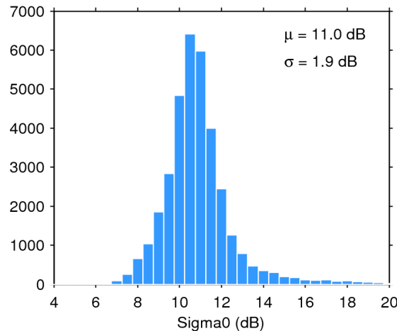
Figure 25. Histogram of flag-valid sigma0 over oceans and lakes for 02/06/2016. The mean ( \mu ) and standard deviation ( \sigma ) are also shown. Note that values outside [4 20] dB are excluded from the histogram for the sake of readability but not from the computation of \mu and \sigma .
