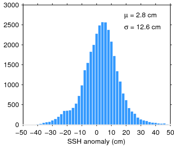
Figure 11. Histogram of science-valid SSH anomaly over oceans and lakes for 02/06/2016. The mean ( \mu ) and standard deviation ( \sigma ) are also shown. Note that values outside [-50 50] cm are excluded from the histogram for the sake of readability but not from the computation of \mu and \sigma .
