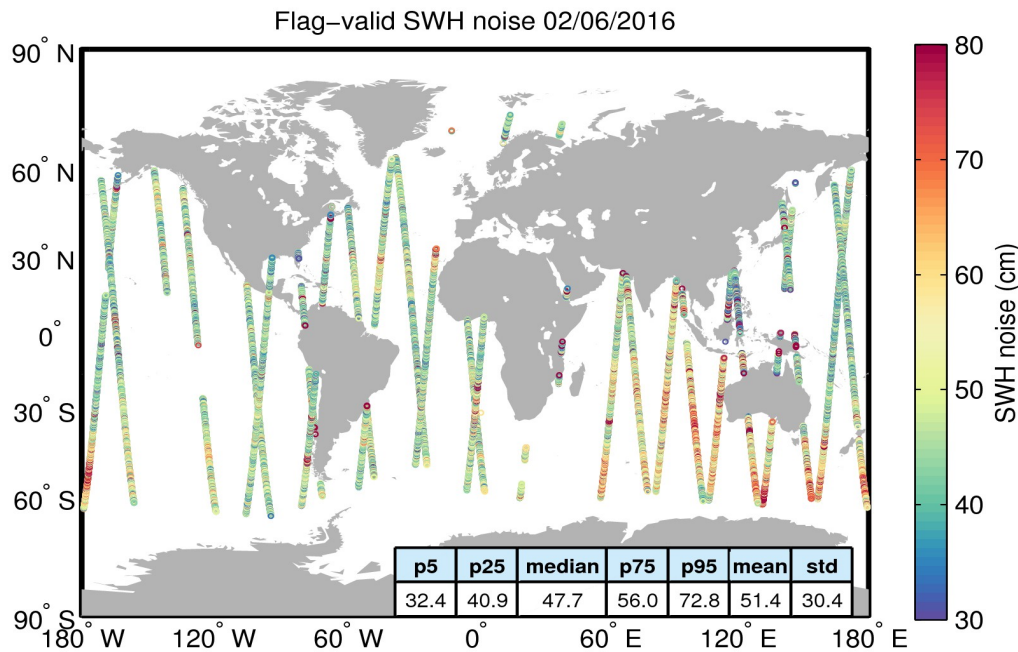
Figure 18. Geographical distribution of flag-valid 20-Hz SWH measurement noise over oceans and lakes for 02/06/2016. The statistical values shown in the figure refer to the SWH noise and are calculated over all measurements shown in the figure.
