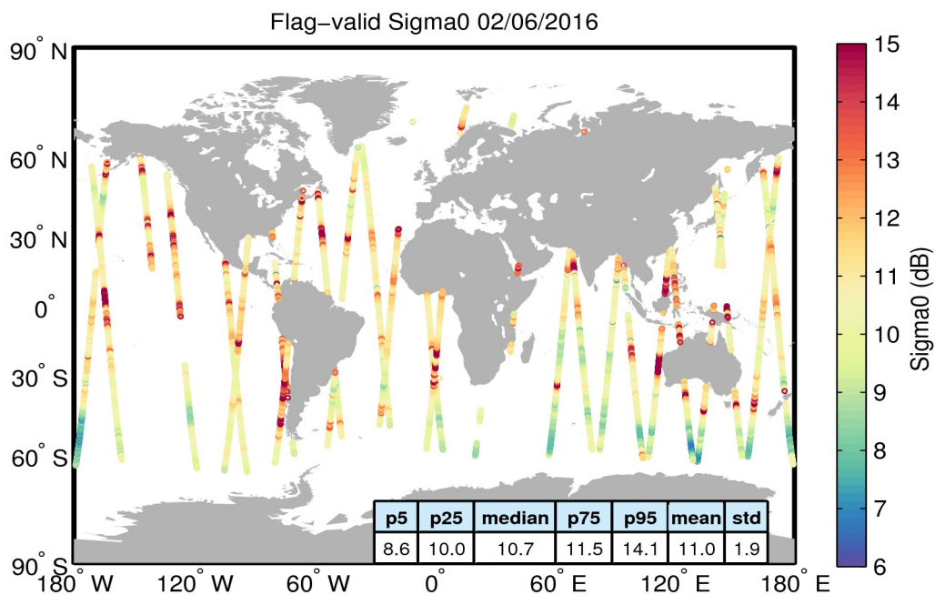
Figure 23. Geographical distribution of flag-valid sigma0 data over oceans and lakes for 02/06/2016. The statistical values shown in the table refer to the sigma0 in dB and are calculated over all measurements shown in the figure.
