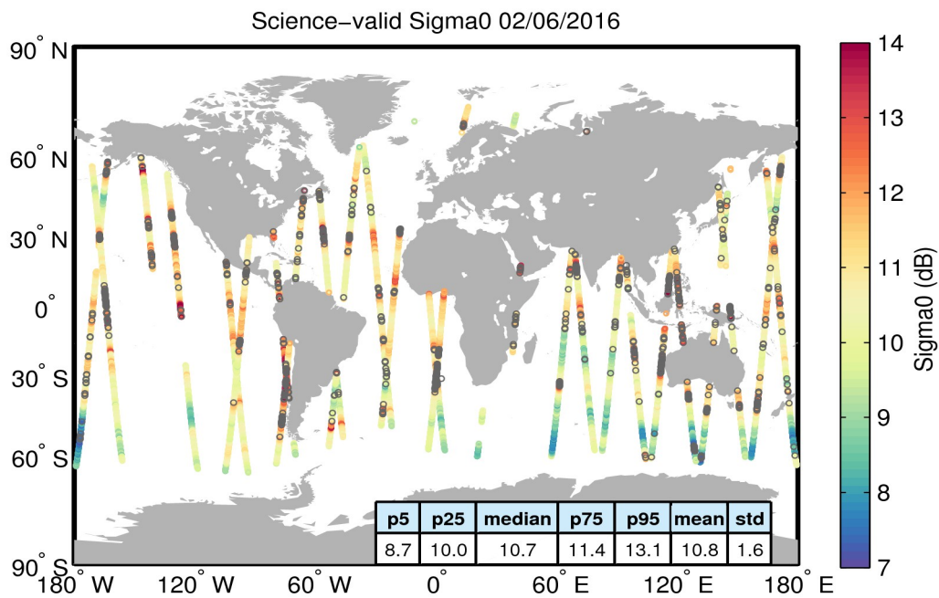
Figure 27. Geographical distribution of science-valid sigma0 data over oceans and lakes for 02/06/2016. The statistical values shown in the table refer to the sigma0 in dB and are calculated over all measurements shown in the figure. Gray circles denote records that have been rejected based on the editing criteria described in Table 4.
