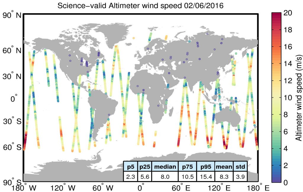
Figure 34. Geographical distribution of science-valid wind data over oceans and lakes for 02/06/2016. The statistical values shown in the table refer to the wind in m/s and are calculated over all measurements shown in the figure. Gray circles denote records that have been rejected based on the editing criteria described in Table 5.
