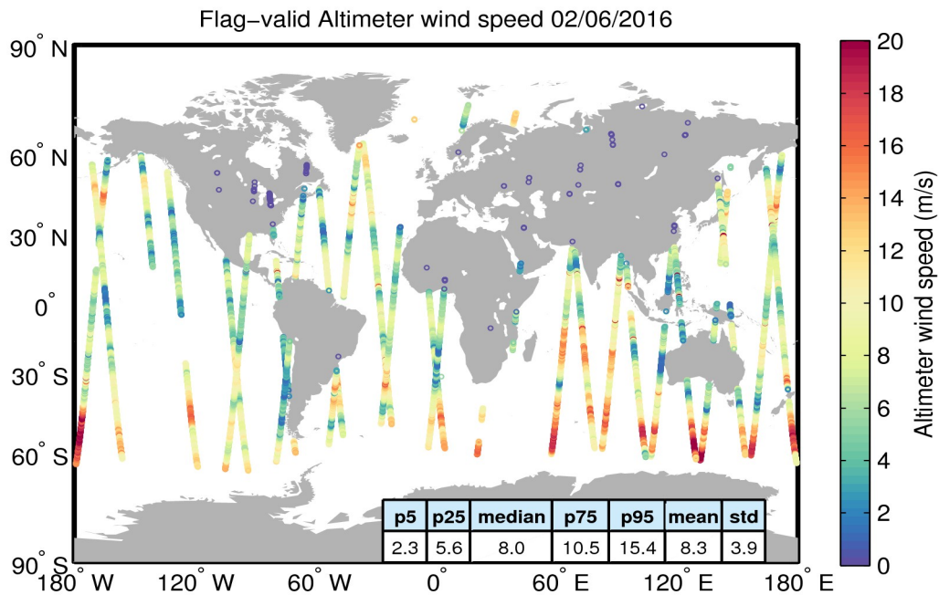
Figure 31. Geographical distribution of flag-valid wind data over oceans and lakes for 02/06/2016. The statistical values shown in the table refer to the wind in m/s and are calculated over all measurements shown in the figure.
