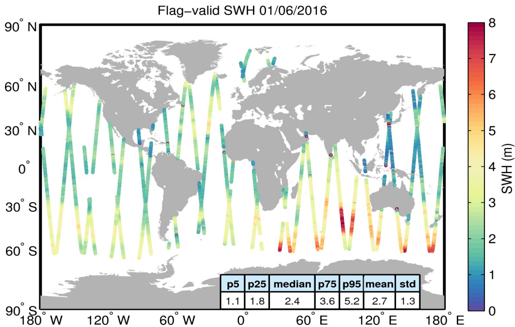
Figure 15. Geographical distribution of flag-valid SWH data over oceans and lakes for 01/06/2016. The statistical values shown in the table refer to the SWH in m and are calculated over all measurements shown in the figure.
