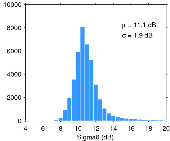
Figure 25. Histogram of flag-valid sigma0 over oceans and lakes for 01/06/2016. The mean ( \mu ) and standard deviation ( \sigma ) are also shown. Note that values outside [4 20] dB are excluded from the histogram for the sake of readability but not from the computation of \mu and \sigma .
