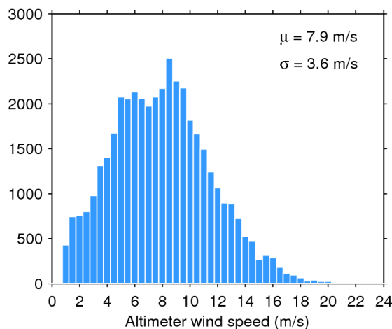
Figure 35. Histogram of science-valid wind over oceans and lakes for 01/06/2016. The mean ( \mu ) and standard deviation ( \sigma ) are also shown. Note that values larger than 24 m/s are excluded from the histogram for the sake of readability but not from the computation of \mu and \sigma .
