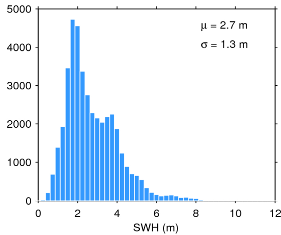
Figure 17. Histogram of flag-valid SWH over oceans and lakes for 01/06/2016. The mean ( \mu ) and standard deviation ( \sigma ) are also shown. Note that values larger than 12 m are excluded from the histogram for the sake of readability but not from the computation of \mu and \sigma .
