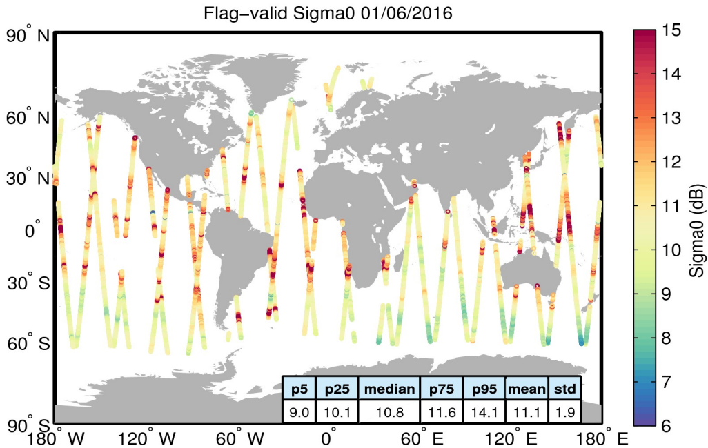
Figure 23. Geographical distribution of flag-valid sigma0 data over oceans and lakes for 01/06/2016. The statistical values shown in the table refer to the sigma0 in dB and are calculated over all measurements shown in the figure.
