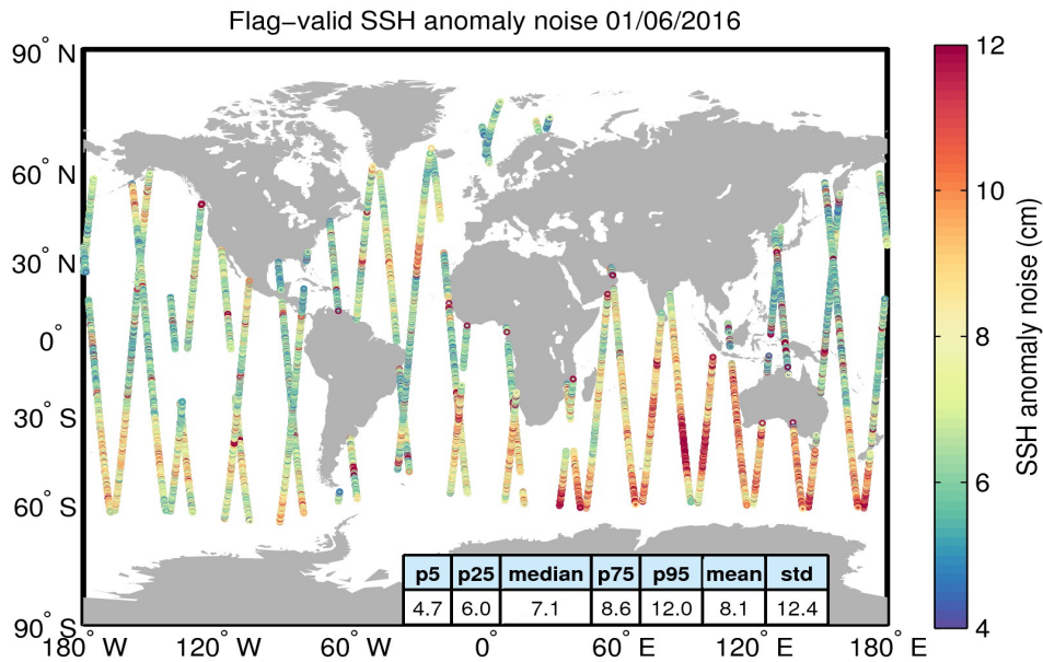
Figure 8. Geographical distribution of flag-valid 20-Hz SSH anomaly measurement noise over oceans and lakes for 01/06/2016. The statistical values shown in the table refer to the SSH anomaly noise and are calculated over all measurements shown in the figure.
