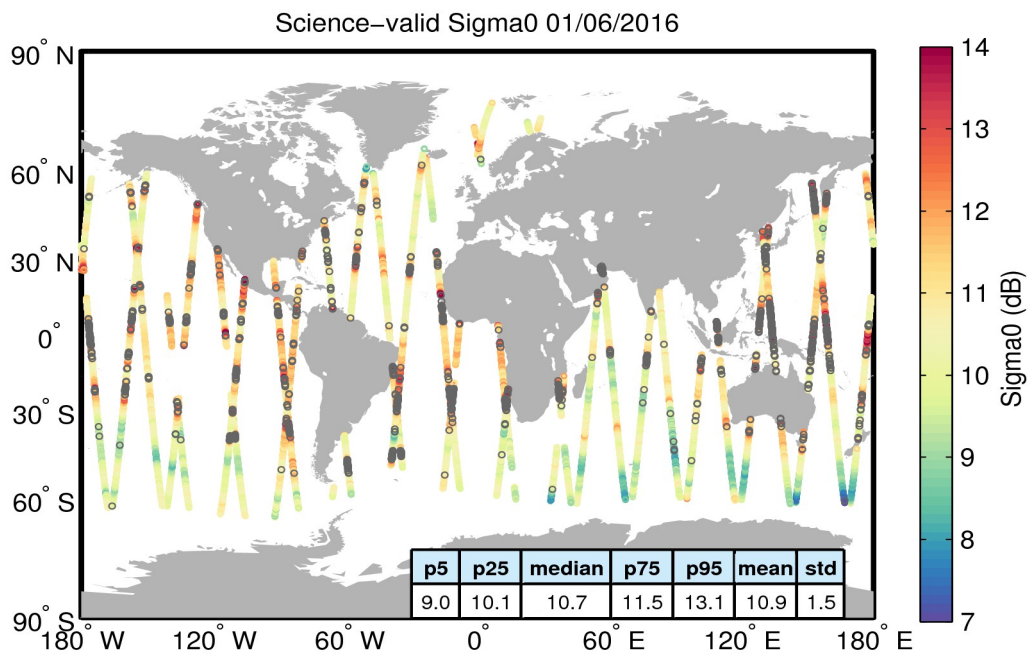
Figure 27. Geographical distribution of science-valid sigma0 data over oceans and lakes for 01/06/2016. The statistical values shown in the table refer to the sigma0 in dB and are calculated over all measurements shown in the figure. Gray circles denote records that have been rejected based on the editing criteria described in Table 4.
