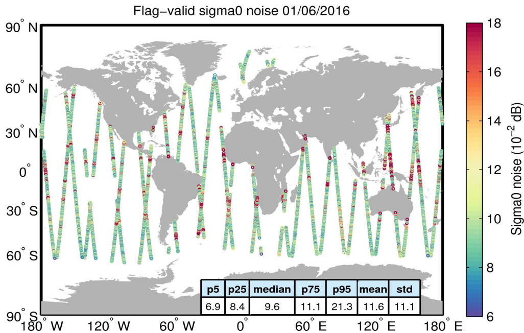
Figure 26. Geographical distribution of flag-valid 20-Hz sigma0 measurement noise over oceans and lakes for 01/06/2016. The statistical values shown in the table refer to the sigma0 noise and are calculated over all measurements shown in the figure.
