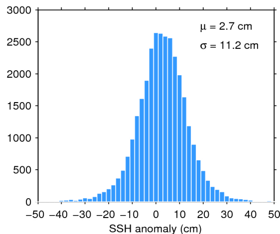
Figure 11. Histogram of science-valid SSH anomaly over oceans and lakes for 01/06/2016. The mean ( \mu ) and standard deviation ( \sigma ) are also shown. Note that values outside [-50 50] cm are excluded from the histogram for the sake of readability but not from the computation of \mu and \sigma .
