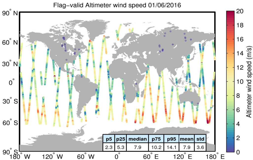
Figure 31. Geographical distribution of flag-valid wind data over oceans and lakes for 01/06/2016. The statistical values shown in the table refer to the wind in m/s and are calculated over all measurements shown in the figure.
