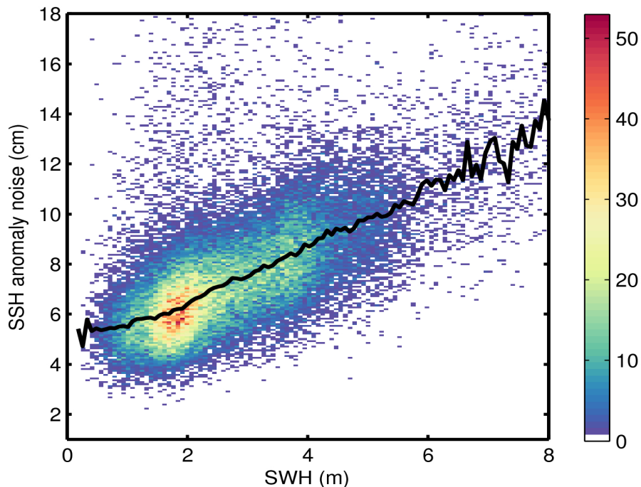
Figure 9. 2D histogram showing flag-valid SSH anomaly noise as a function of SWH for 01/06/2016. The black line denotes the median SSH anomaly noise as a function of SWH.
