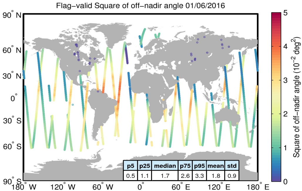
Figure 37. Geographical distribution of flag-valid mispointing data over oceans and lakes for 01/06/2016. The statistical values shown in the table refer to the mispointing in 10^{-2} deg 2 and are calculated over all measurements shown in the figure.
