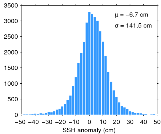
Figure 7. Histogram of flag-valid SSH anomaly over oceans and lakes for 01/06/2016. The mean ( \mu ) and standard deviation ( \sigma ) are also shown. Note that values outside [-50 50] cm are excluded from the histogram for the sake of readability but not from the computation of \mu and \sigma .
