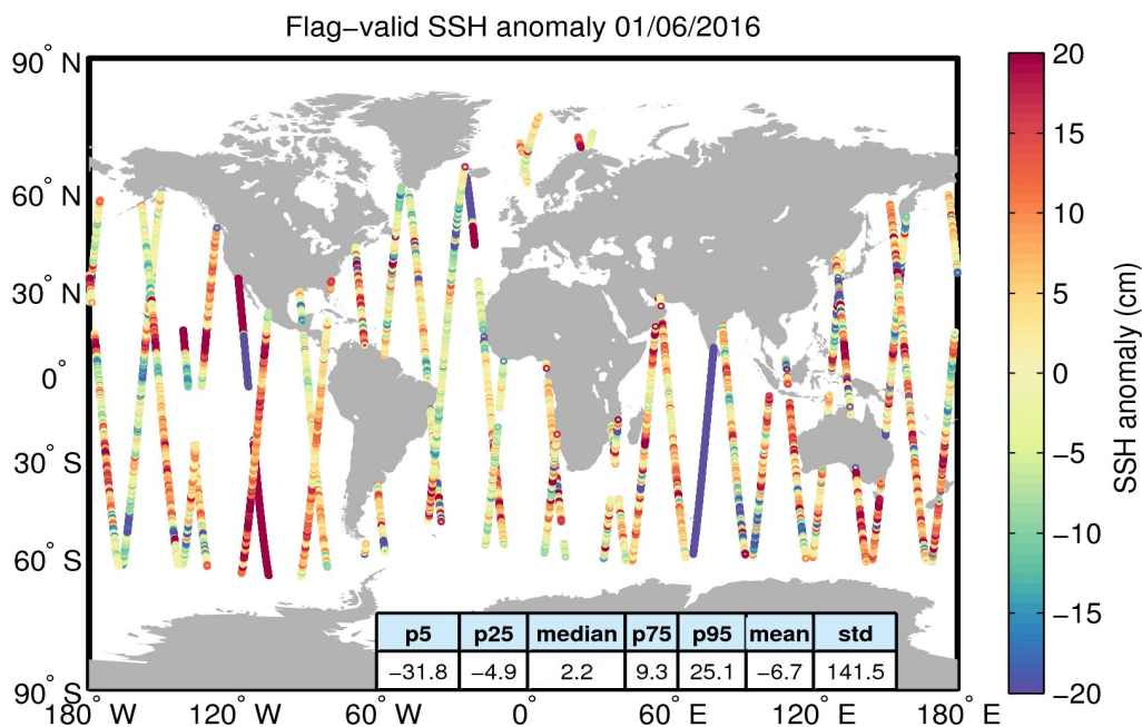
Figure 5. Geographical distribution of flag-valid 1-Hz SSH anomaly data over oceans and lakes for 01/06/2016. The statistical values shown in the table refer to the SSH anomaly in cm and are calculated over all measurements shown in the figure.
