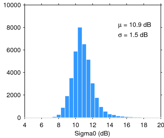
Figure 28. Histogram of science-valid sigma0 over oceans and lakes for 01/06/2016. The mean ( \mu ) and standard deviation ( \sigma ) are also shown. Note that values outside [4 20] dB are excluded from the histogram for the sake of readability but not from the computation of \mu and \sigma .
