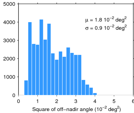
Figure 39. Histogram of flag-valid mispointing over oceans and lakes for 01/06/2016. The mean ( \mu ) and standard deviation ( \sigma ) are also shown. Note that values larger than 6 \cdot 10^{-2} \text{ deg}^2 are excluded from the histogram for the sake of readability but not from the computation of \mu and \sigma .
