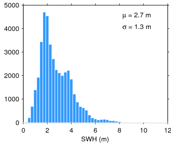
Figure 20. Histogram of science-valid SWH over oceans and lakes for 01/06/2016. The mean ( \mu ) and standard deviation ( \sigma ) are also shown. Note that values larger than 12 m are excluded from the histogram for the sake of readability but not from the computation of \mu and \sigma .
