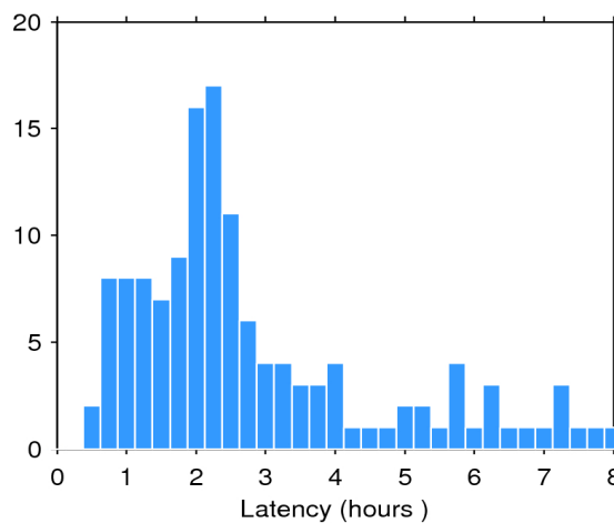
Figure 2. Histogram of the data latency for 01/06/2016. The y-axis denotes the number of files that are made available with a delay of x-hours with respect to the mean time of the records stored in the file.
