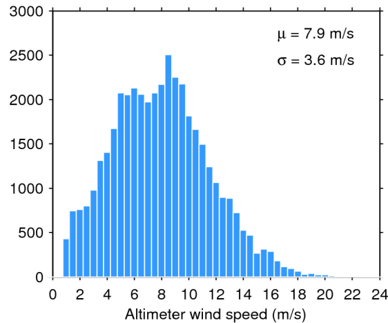
Figure 33. Histogram of flag-valid wind over oceans and lakes for 01/06/2016. The mean ( \mu ) and standard deviation ( \sigma ) are also shown. Note that values larger than 24 m/s are excluded from the histogram for the sake of readability but not from the computation of \mu and \sigma .
