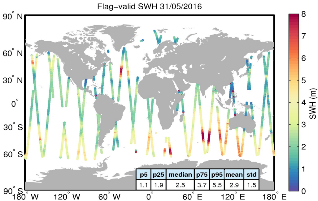
Figure 15. Geographical distribution of flag-valid SWH data over oceans and lakes for 31/05/2016. The statistical values shown in the table refer to the SWH in m and are calculated over all measurements shown in the figure.
