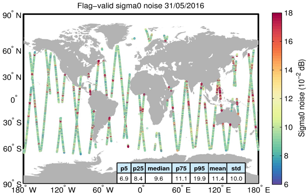
Figure 26. Geographical distribution of flag-valid 20-Hz sigma0 measurement noise over oceans and lakes for 31/05/2016. The statistical values shown in the table refer to the sigma0 noise and are calculated over all measurements shown in the figure.
