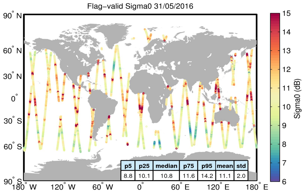
Figure 23. Geographical distribution of flag-valid sigma0 data over oceans and lakes for 31/05/2016. The statistical values shown in the table refer to the sigma0 in dB and are calculated over all measurements shown in the figure.
