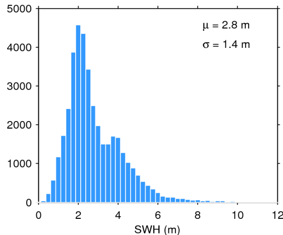
Figure 20. Histogram of science-valid SWH over oceans and lakes for 31/05/2016. The mean ( \mu ) and standard deviation ( \sigma ) are also shown. Note that values larger than 12 m are excluded from the histogram for the sake of readability but not from the computation of \mu and \sigma .
