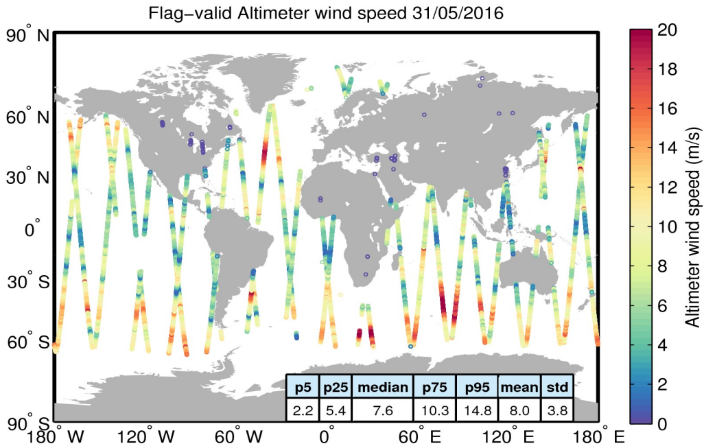
Figure 31. Geographical distribution of flag-valid wind data over oceans and lakes for 31/05/2016. The statistical values shown in the table refer to the wind in m/s and are calculated over all measurements shown in the figure.
