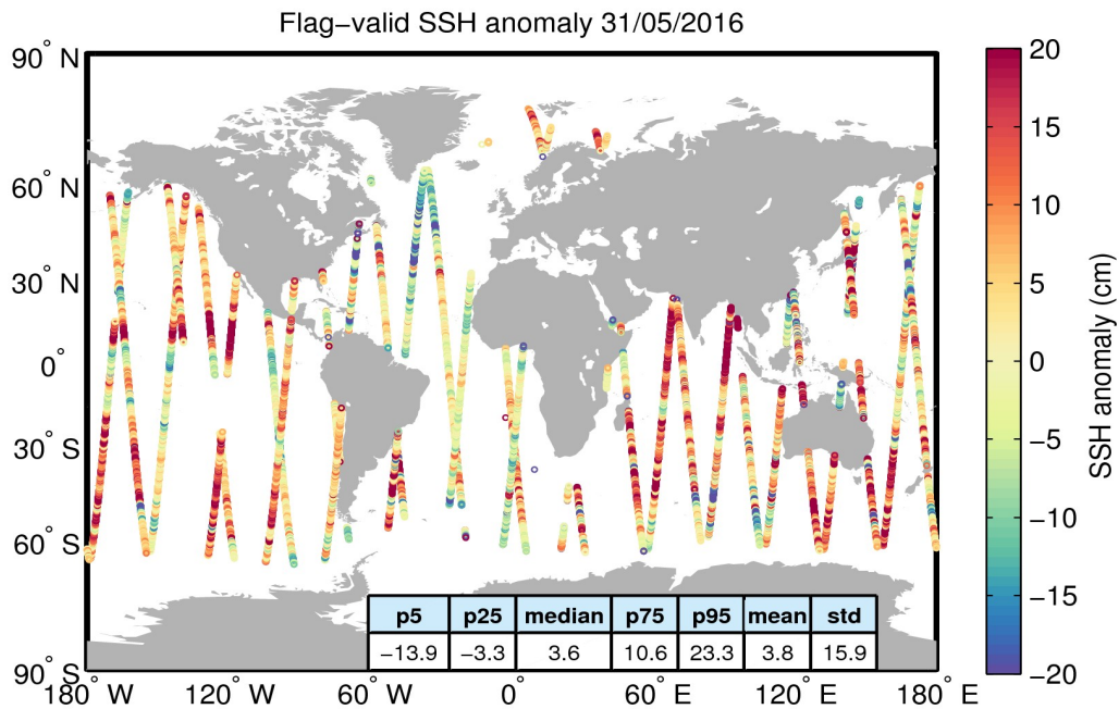
Figure 5. Geographical distribution of flag-valid 1-Hz SSH anomaly data over oceans and lakes for 31/05/2016. The statistical values shown in the table refer to the SSH anomaly in cm and are calculated over all measurements shown in the figure.
