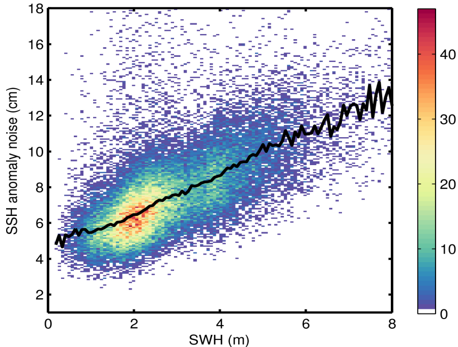
Figure 9. 2D histogram showing flag-valid SSH anomaly noise as a function of SWH for 31/05/2016. The black line denotes the median SSH anomaly noise as a function of SWH.
