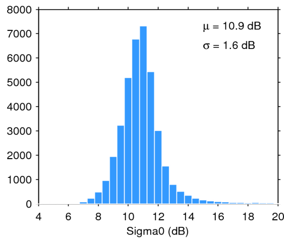
Figure 28. Histogram of science-valid sigma0 over oceans and lakes for 31/05/2016. The mean ( \mu ) and standard deviation ( \sigma ) are also shown. Note that values outside [4 20] dB are excluded from the histogram for the sake of readability but not from the computation of \mu and \sigma .
