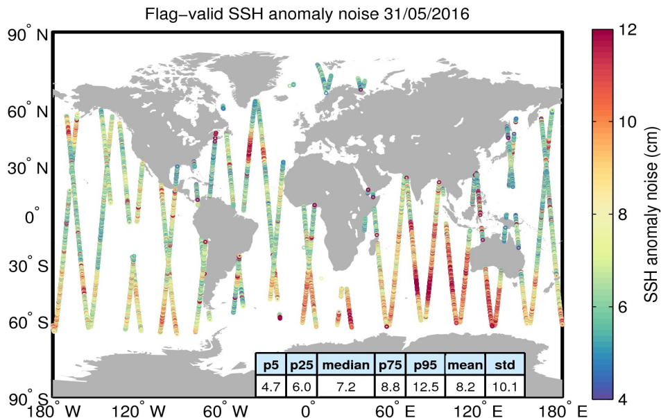
Figure 8. Geographical distribution of flag-valid 20-Hz SSH anomaly measurement noise over oceans and lakes for 31/05/2016. The statistical values shown in the table refer to the SSH anomaly noise and are calculated over all measurements shown in the figure.
