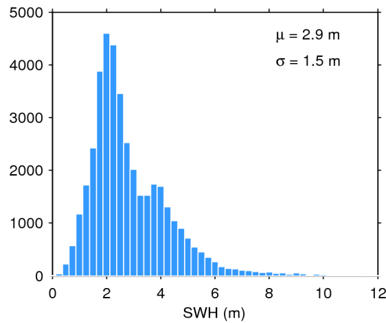
Figure 17. Histogram of flag-valid SWH over oceans and lakes for 31/05/2016. The mean ( \mu ) and standard deviation ( \sigma ) are also shown. Note that values larger than 12 m are excluded from the histogram for the sake of readability but not from the computation of \mu and \sigma .
