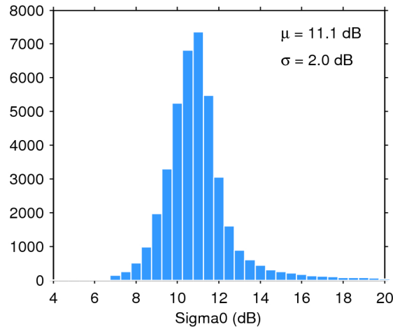
Figure 25. Histogram of flag-valid sigma0 over oceans and lakes for 31/05/2016. The mean ( \mu ) and standard deviation ( \sigma ) are also shown. Note that values outside [4 20] dB are excluded from the histogram for the sake of readability but not from the computation of \mu and \sigma .
