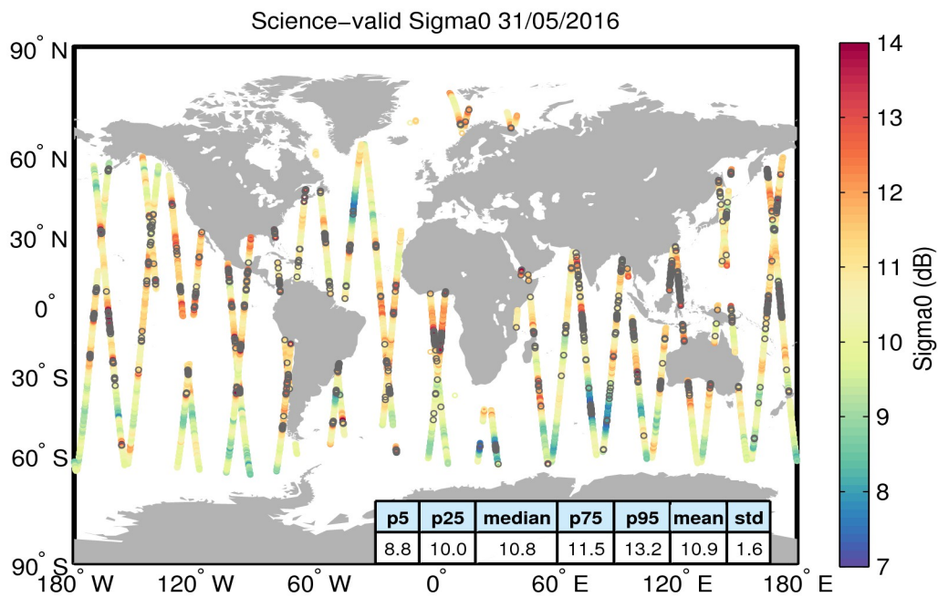
Figure 27. Geographical distribution of science-valid sigma0 data over oceans and lakes for 31/05/2016. The statistical values shown in the table refer to the sigma0 in dB and are calculated over all measurements shown in the figure. Gray circles denote records that have been rejected based on the editing criteria described in Table 4.
