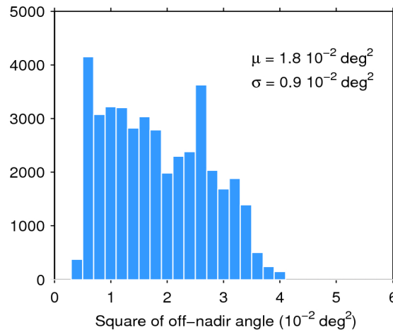
Figure 39. Histogram of flag-valid mispointing over oceans and lakes for 31/05/2016. The mean ( \mu ) and standard deviation ( \sigma ) are also shown. Note that values larger than 6 \cdot 10^{-2} \text{ deg}^2 are excluded from the histogram for the sake of readability but not from the computation of \mu and \sigma .
