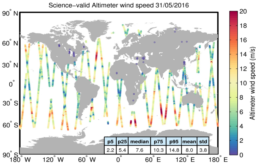
Figure 34. Geographical distribution of science-valid wind data over oceans and lakes for 31/05/2016. The statistical values shown in the table refer to the wind in m/s and are calculated over all measurements shown in the figure. Gray circles denote records that have been rejected based on the editing criteria described in Table 5.
