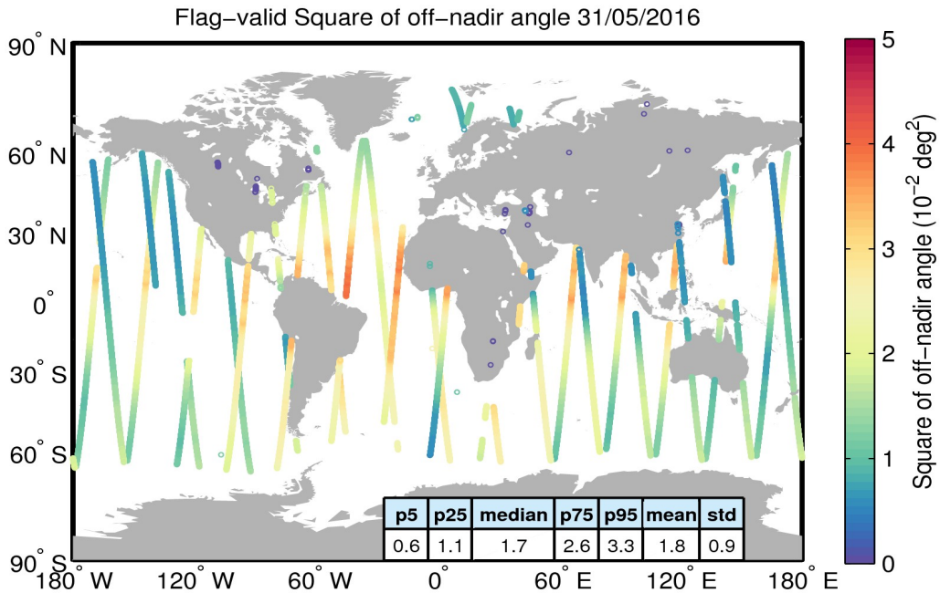
Figure 37. Geographical distribution of flag-valid mispointing data over oceans and lakes for 31/05/2016. The statistical values shown in the table refer to the mispointing in 10^{-2} deg 2 and are calculated over all measurements shown in the figure.
