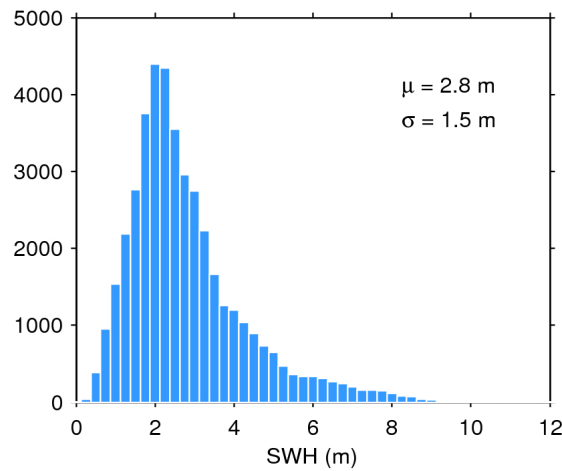
Figure 17. Histogram of flag-valid SWH over oceans and lakes for 30/05/2016. The mean ( \mu ) and standard deviation ( \sigma ) are also shown. Note that values larger than 12 m are excluded from the histogram for the sake of readability but not from the computation of \mu and \sigma .
