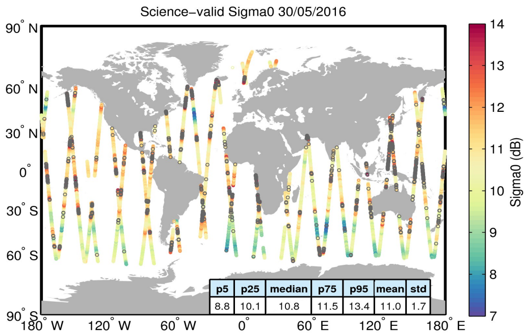
Figure 27. Geographical distribution of science-valid sigma0 data over oceans and lakes for 30/05/2016. The statistical values shown in the table refer to the sigma0 in dB and are calculated over all measurements shown in the figure. Gray circles denote records that have been rejected based on the editing criteria described in Table 4.
