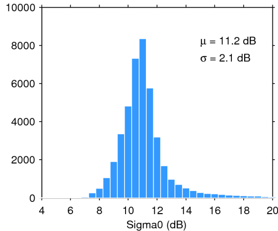
Figure 25. Histogram of flag-valid sigma0 over oceans and lakes for 30/05/2016. The mean ( \mu ) and standard deviation ( \sigma ) are also shown. Note that values outside [4 20] dB are excluded from the histogram for the sake of readability but not from the computation of \mu and \sigma .
