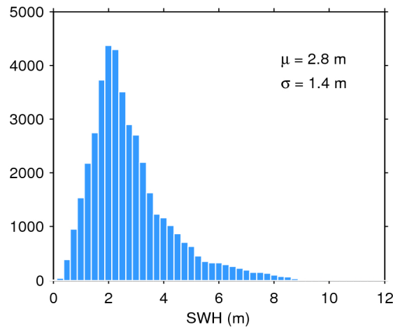
Figure 20. Histogram of science-valid SWH over oceans and lakes for 30/05/2016. The mean ( \mu ) and standard deviation ( \sigma ) are also shown. Note that values larger than 12 m are excluded from the histogram for the sake of readability but not from the computation of \mu and \sigma .
