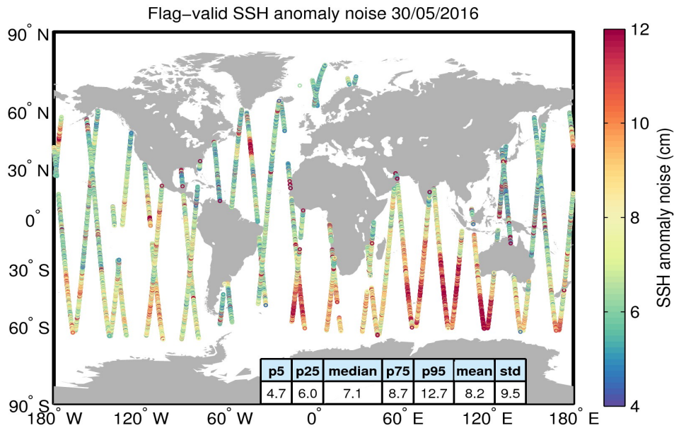
Figure 8. Geographical distribution of flag-valid 20-Hz SSH anomaly measurement noise over oceans and lakes for 30/05/2016. The statistical values shown in the table refer to the SSH anomaly noise and are calculated over all measurements shown in the figure.
