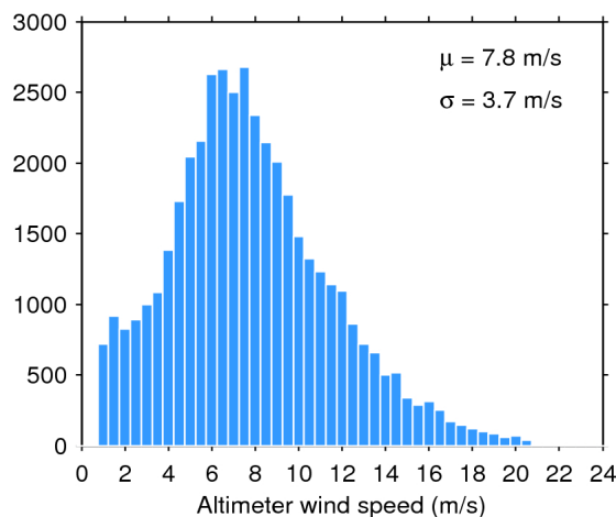
Figure 35. Histogram of science-valid wind over oceans and lakes for 30/05/2016. The mean ( \mu ) and standard deviation ( \sigma ) are also shown. Note that values larger than 24 m/s are excluded from the histogram for the sake of readability but not from the computation of \mu and \sigma .
