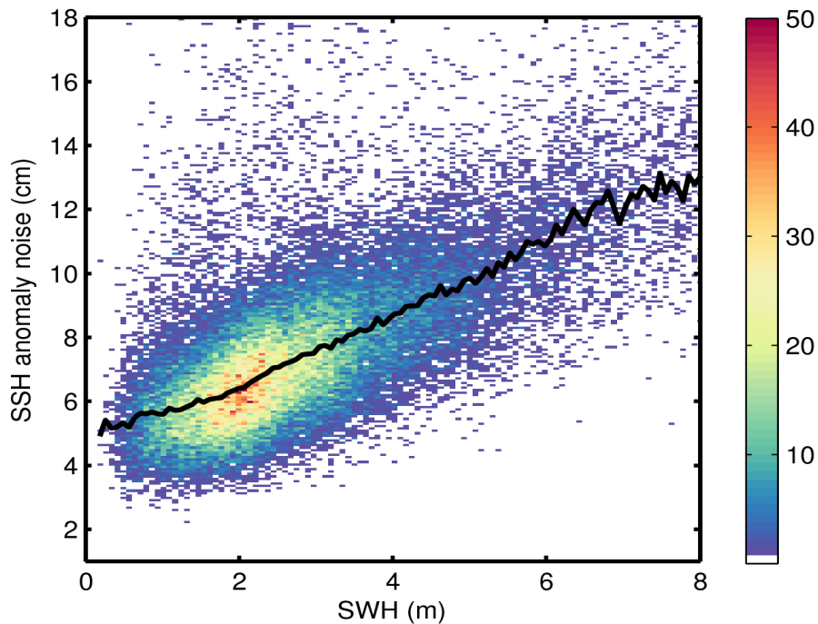
Figure 9. 2D histogram showing flag-valid SSH anomaly noise as a function of SWH for 30/05/2016. The black line denotes the median SSH anomaly noise as a function of SWH.
