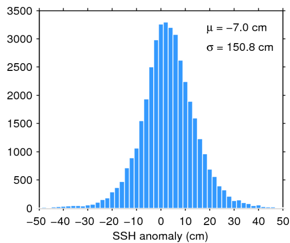
Figure 7. Histogram of flag-valid SSH anomaly over oceans and lakes for 30/05/2016. The mean ( \mu ) and standard deviation ( \sigma ) are also shown. Note that values outside [-50 50] cm are excluded from the histogram for the sake of readability but not from the computation of \mu and \sigma .
