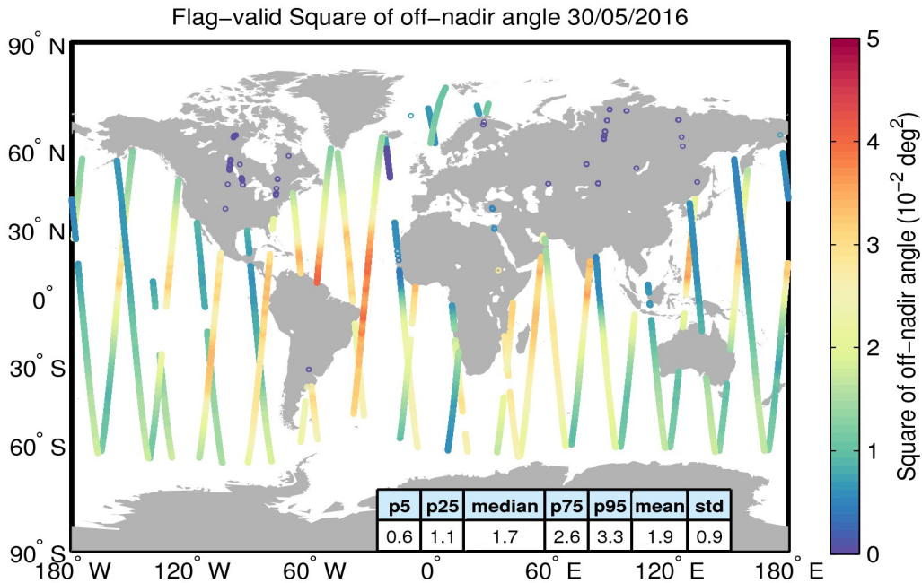
Figure 37. Geographical distribution of flag-valid mispointing data over oceans and lakes for 30/05/2016. The statistical values shown in the table refer to the mispointing in 10^{-2} \text{ deg}^2 and are calculated over all measurements shown in the figure.
