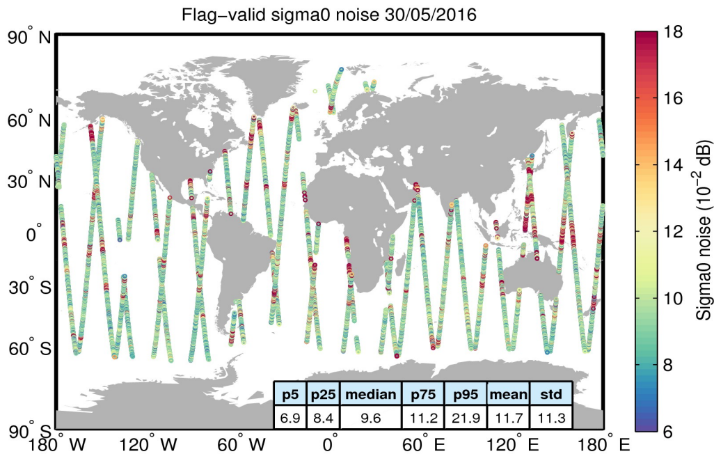
Figure 26. Geographical distribution of flag-valid 20-Hz sigma0 measurement noise over oceans and lakes for 30/05/2016. The statistical values shown in the table refer to the sigma0 noise and are calculated over all measurements shown in the figure.
