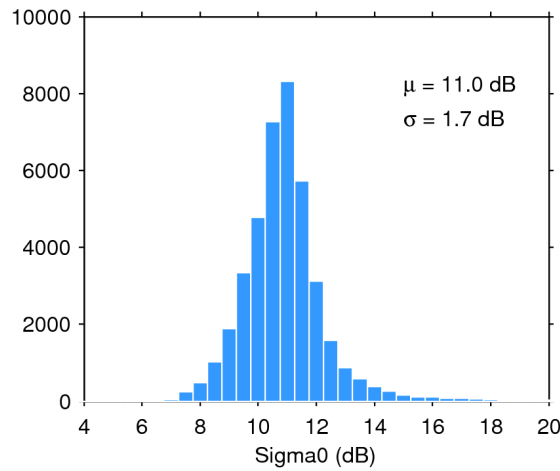
Figure 28. Histogram of science-valid sigma0 over oceans and lakes for 30/05/2016. The mean ( \mu ) and standard deviation ( \sigma ) are also shown. Note that values outside [4 20] dB are excluded from the histogram for the sake of readability but not from the computation of \mu and \sigma .
