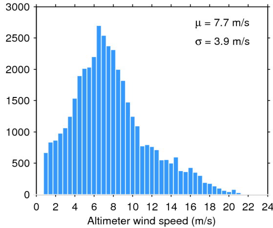
Figure 33. Histogram of flag-valid wind over oceans and lakes for 29/05/2016. The mean ( \mu ) and standard deviation ( \sigma ) are also shown. Note that values larger than 24 m/s are excluded from the histogram for the sake of readability but not from the computation of \mu and \sigma .
