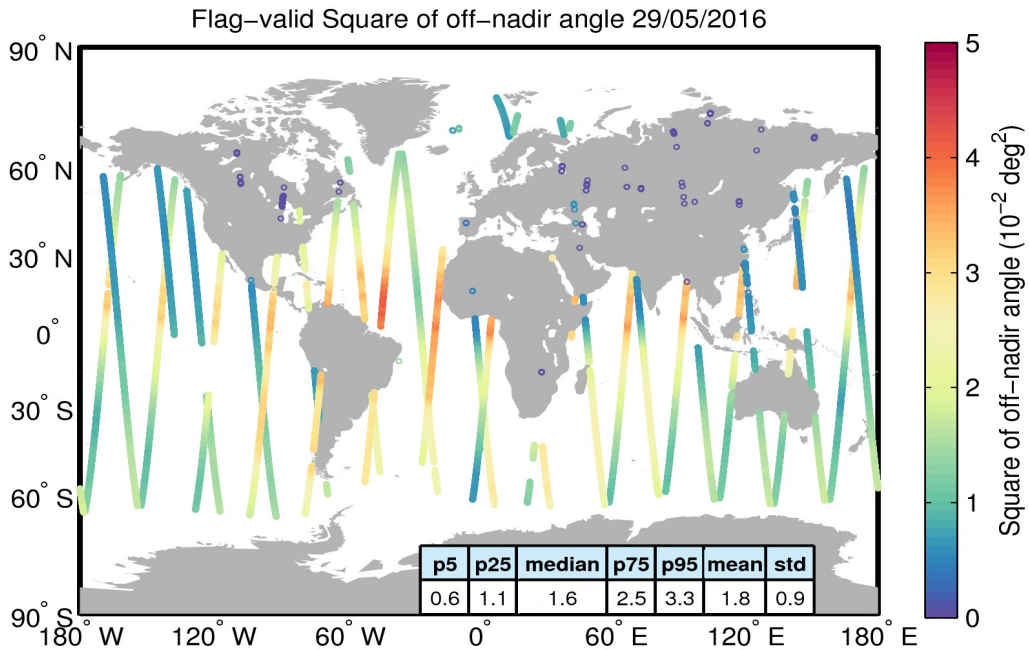
Figure 37. Geographical distribution of flag-valid mispointing data over oceans and lakes for 29/05/2016. The statistical values shown in the table refer to the mispointing in 10^{-2} deg 2 and are calculated over all measurements shown in the figure.
