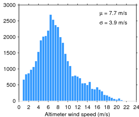
Figure 35. Histogram of science-valid wind over oceans and lakes for 29/05/2016. The mean ( \mu ) and standard deviation ( \sigma ) are also shown. Note that values larger than 24 m/s are excluded from the histogram for the sake of readability but not from the computation of \mu and \sigma .
