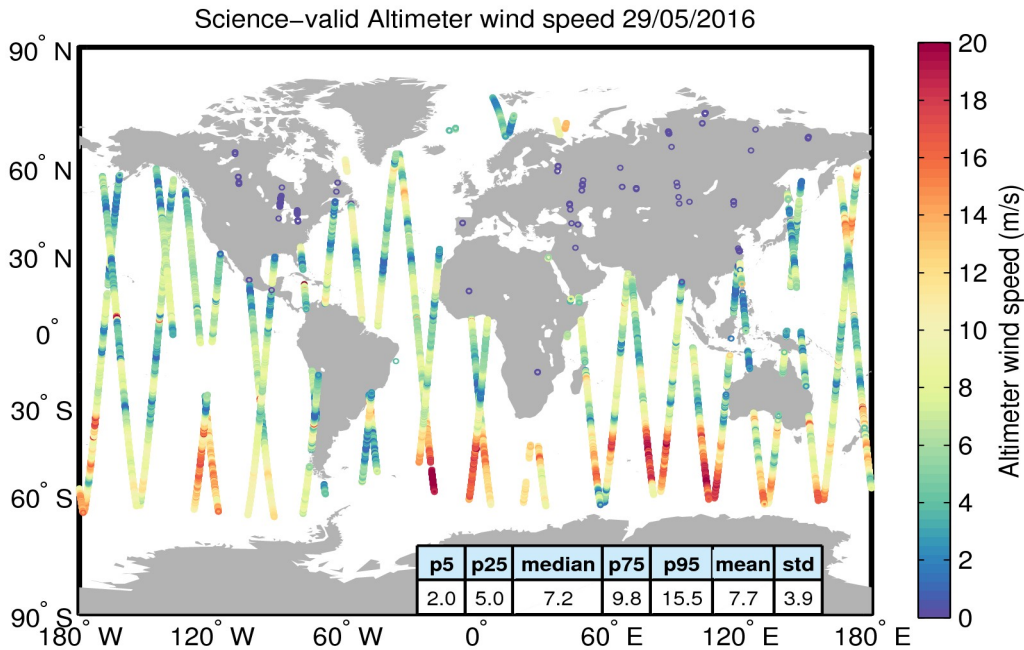
Figure 34. Geographical distribution of science-valid wind data over oceans and lakes for 29/05/2016. The statistical values shown in the table refer to the wind in m/s and are calculated over all measurements shown in the figure. Gray circles denote records that have been rejected based on the editing criteria described in Table 5.
