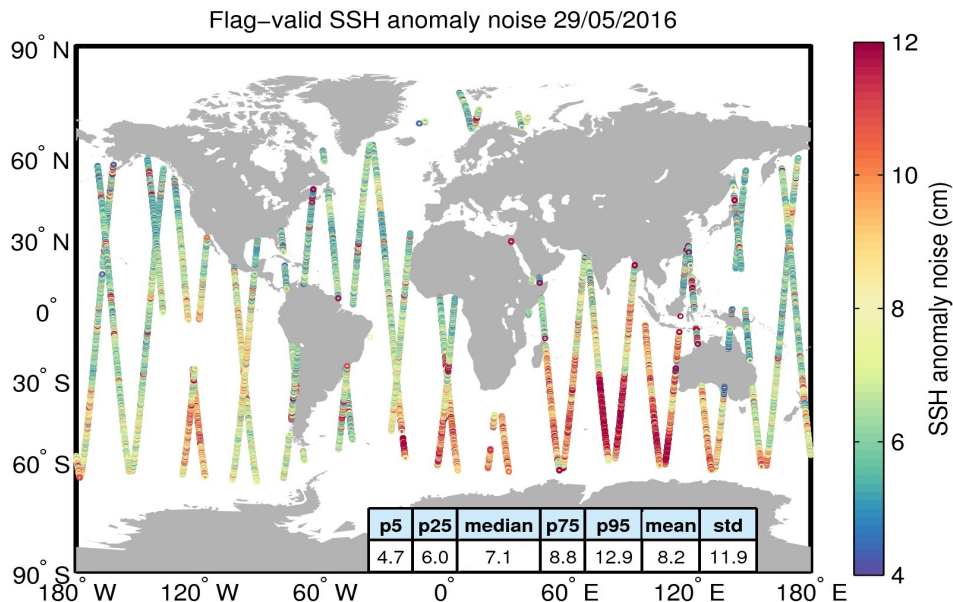
Figure 8. Geographical distribution of flag-valid 20-Hz SSH anomaly measurement noise over oceans and lakes for 29/05/2016. The statistical values shown in the table refer to the SSH anomaly noise and are calculated over all measurements shown in the figure.
