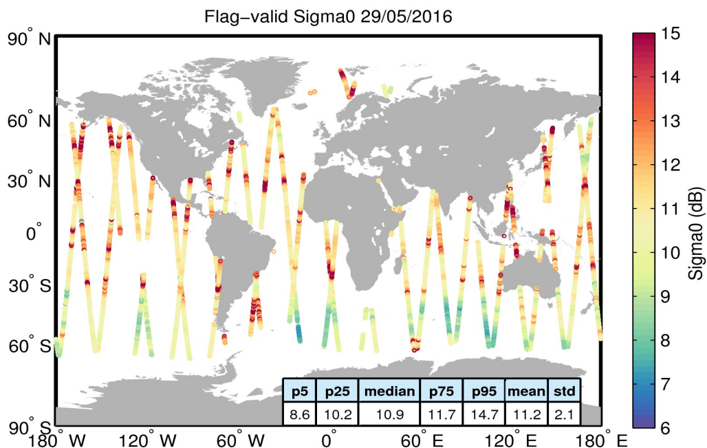
Figure 23. Geographical distribution of flag-valid sigma0 data over oceans and lakes for 29/05/2016. The statistical values shown in the table refer to the sigma0 in dB and are calculated over all measurements shown in the figure.
