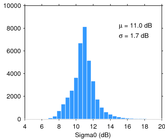
Figure 28. Histogram of science-valid sigma0 over oceans and lakes for 29/05/2016. The mean ( \mu ) and standard deviation ( \sigma ) are also shown. Note that values outside [4 20] dB are excluded from the histogram for the sake of readability but not from the computation of \mu and \sigma .
