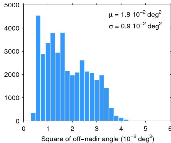
Figure 39. Histogram of flag-valid mispointing over oceans and lakes for 29/05/2016. The mean ( \mu ) and standard deviation ( \sigma ) are also shown. Note that values larger than 6 \cdot 10^{-2} \text{ deg}^2 are excluded from the histogram for the sake of readability but not from the computation of \mu and \sigma .
