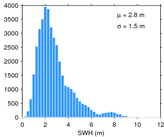
Figure 17. Histogram of flag-valid SWH over oceans and lakes for 29/05/2016. The mean ( \mu ) and standard deviation ( \sigma ) are also shown. Note that values larger than 12 m are excluded from the histogram for the sake of readability but not from the computation of \mu and \sigma .
