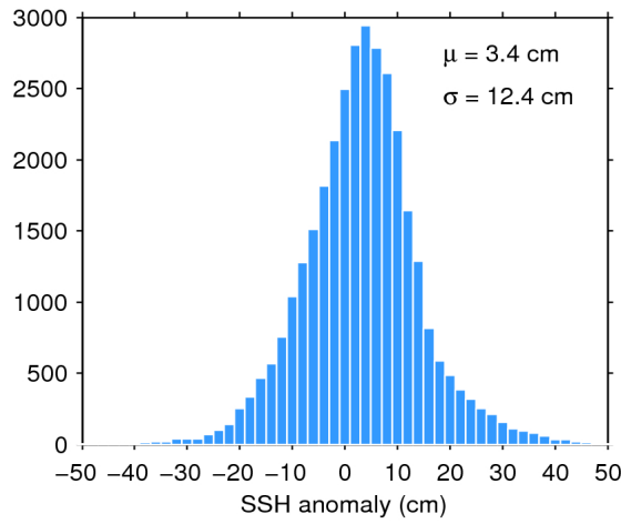
Figure 11. Histogram of science-valid SSH anomaly over oceans and lakes for 29/05/2016. The mean ( \mu ) and standard deviation ( \sigma ) are also shown. Note that values outside [-50 50] cm are excluded from the histogram for the sake of readability but not from the computation of \mu and \sigma .
