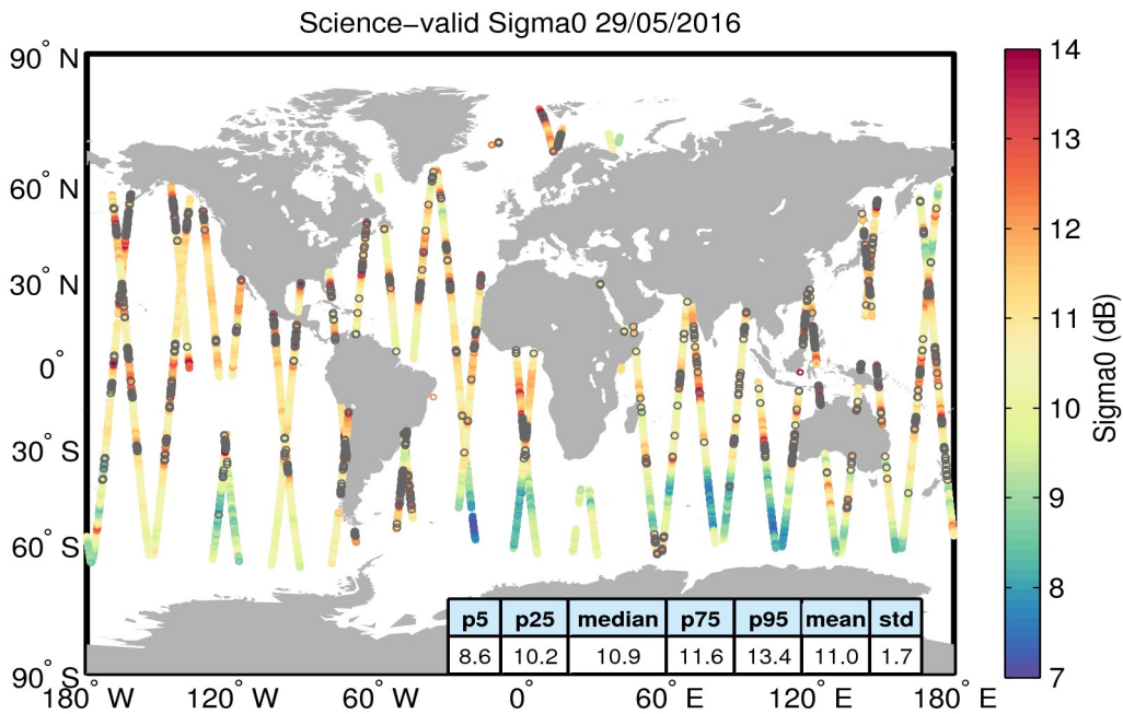
Figure 27. Geographical distribution of science-valid sigma0 data over oceans and lakes for 29/05/2016. The statistical values shown in the table refer to the sigma0 in dB and are calculated over all measurements shown in the figure. Gray circles denote records that have been rejected based on the editing criteria described in Table 4.
