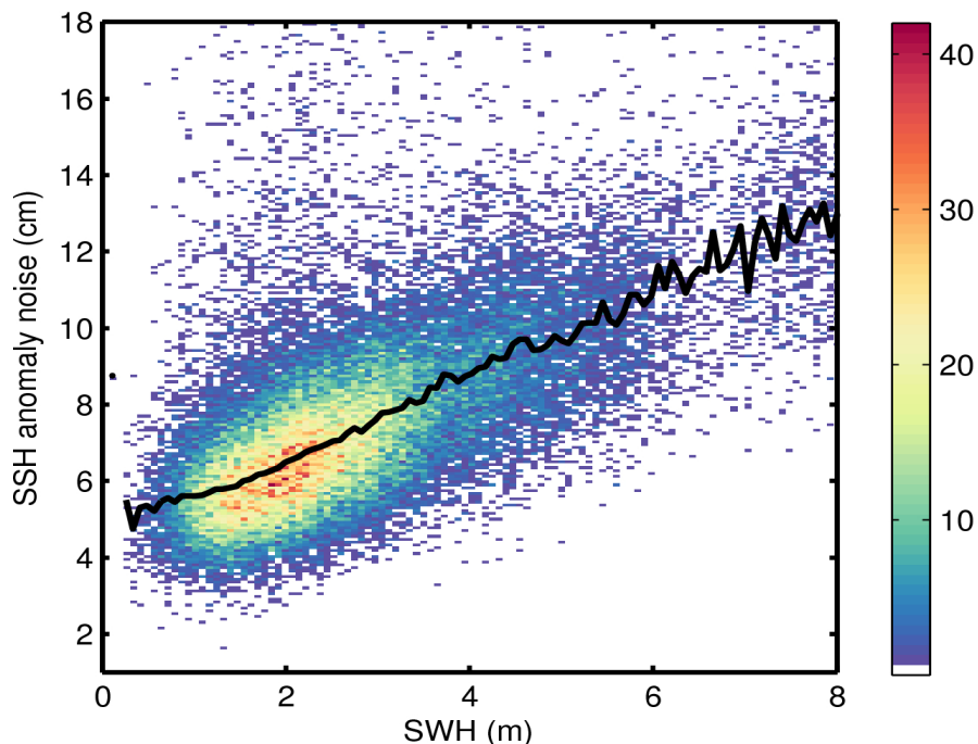
Figure 9. 2D histogram showing flag-valid SSH anomaly noise as a function of SWH for 29/05/2016. The black line denotes the median SSH anomaly noise as a function of SWH.
