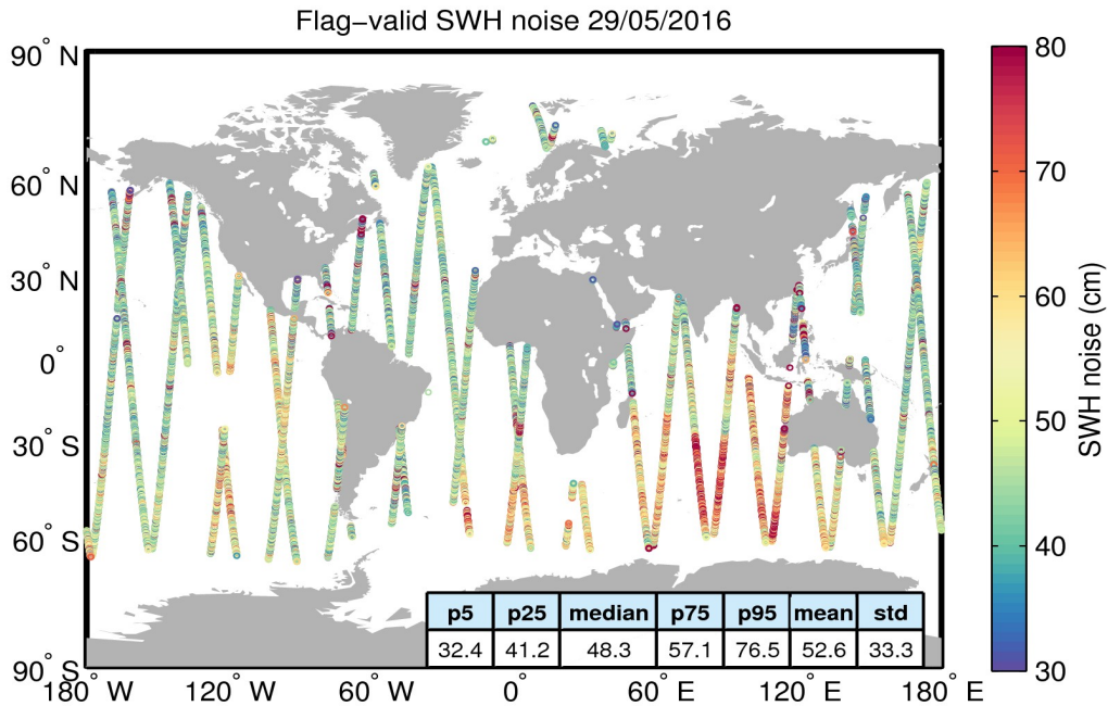
Figure 18. Geographical distribution of flag-valid 20-Hz SWH measurement noise over oceans and lakes for 29/05/2016. The statistical values shown in the table refer to the SWH noise and are calculated over all measurements shown in the figure.
