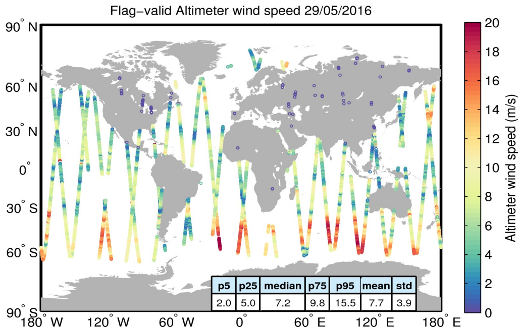
Figure 31. Geographical distribution of flag-valid wind data over oceans and lakes for 29/05/2016. The statistical values shown in the table refer to the wind in m/s and are calculated over all measurements shown in the figure.
