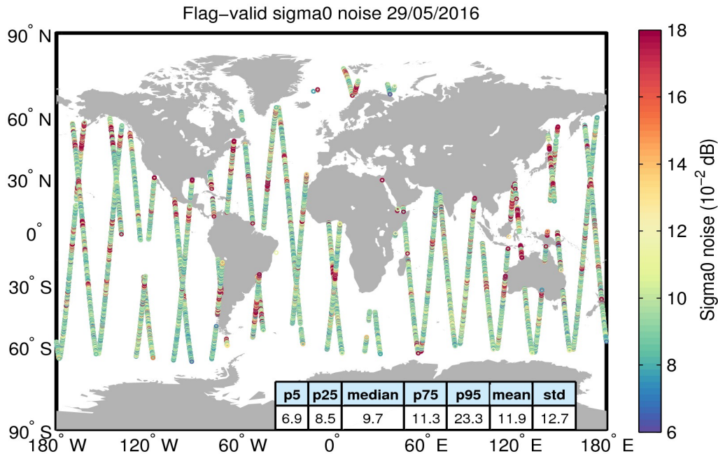
Figure 26. Geographical distribution of flag-valid 20-Hz sigma0 measurement noise over oceans and lakes for 29/05/2016. The statistical values shown in the table refer to the sigma0 noise and are calculated over all measurements shown in the figure.
