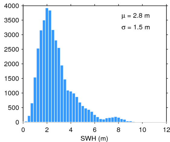
Figure 20. Histogram of science-valid SWH over oceans and lakes for 29/05/2016. The mean ( \mu ) and standard deviation ( \sigma ) are also shown. Note that values larger than 12 m are excluded from the histogram for the sake of readability but not from the computation of \mu and \sigma .
