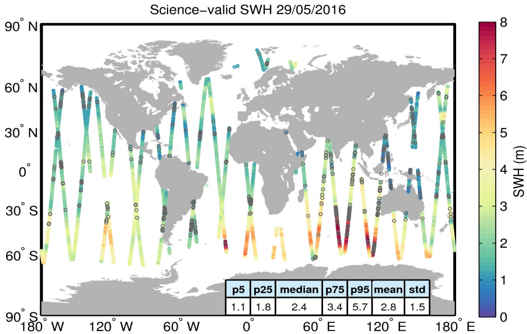
Figure 19. Geographical distribution of science-valid SWH data over oceans and lakes for 29/05/2016. The statistical values shown in the table refer to the SWH in m and are calculated over all measurements shown in the figure. Gray circles denote records that have been rejected based on the editing criteria described in Table 3.
