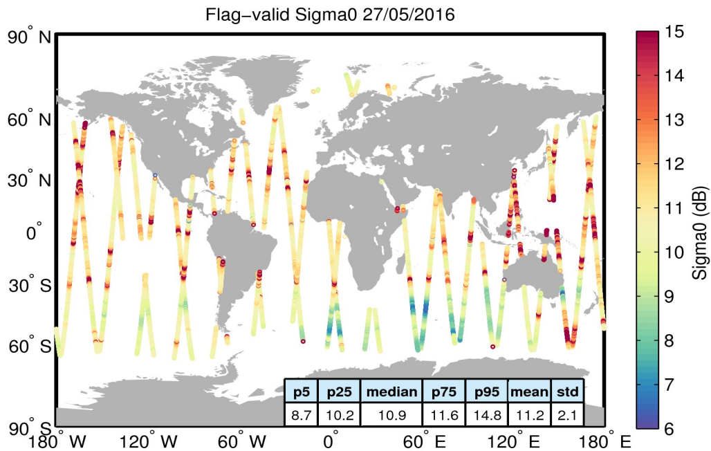
Figure 23. Geographical distribution of flag-valid sigma0 data over oceans and lakes for 27/05/2016. The statistical values shown in the table refer to the sigma0 in dB and are calculated over all measurements shown in the figure.
