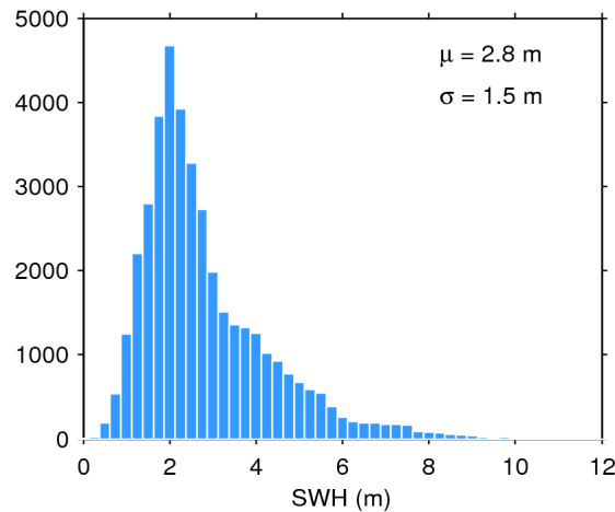
Figure 20. Histogram of science-valid SWH over oceans and lakes for 27/05/2016. The mean ( \mu ) and standard deviation ( \sigma ) are also shown. Note that values larger than 12 m are excluded from the histogram for the sake of readability but not from the computation of \mu and \sigma .
