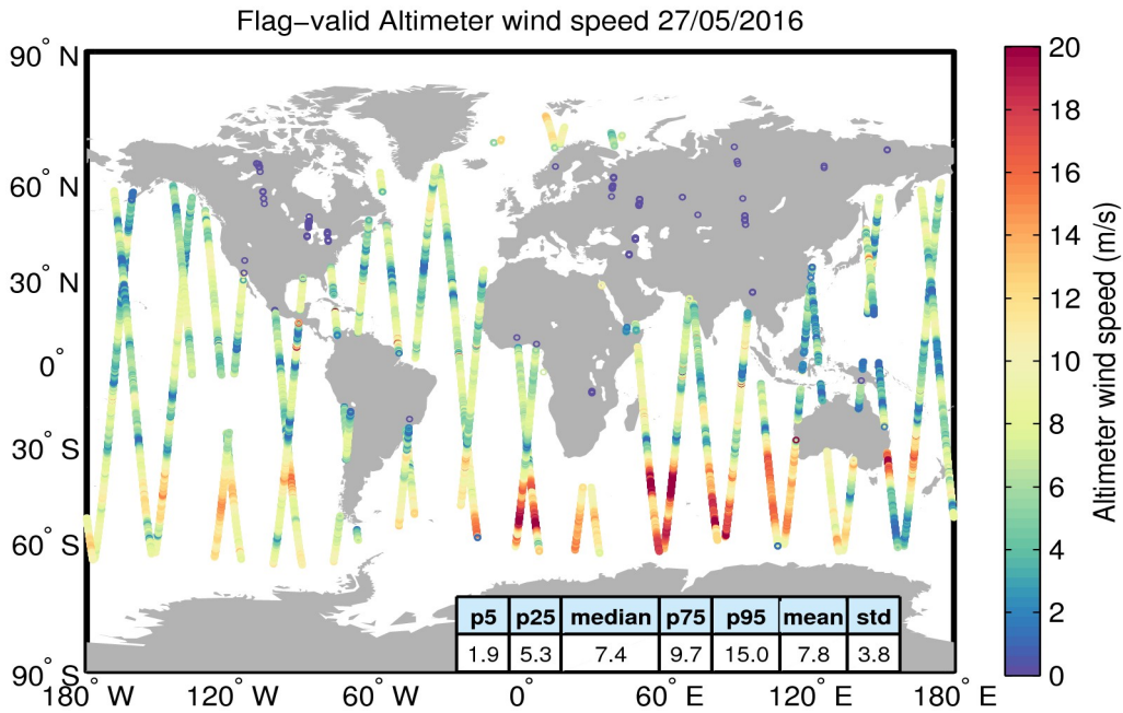
Figure 31. Geographical distribution of flag-valid wind data over oceans and lakes for 27/05/2016. The statistical values shown in the table refer to the wind in m/s and are calculated over all measurements shown in the figure.
