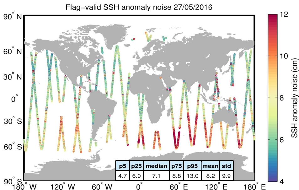
Figure 8. Geographical distribution of flag-valid 20-Hz SSH anomaly measurement noise over oceans and lakes for 27/05/2016. The statistical values shown in the table refer to the SSH anomaly noise and are calculated over all measurements shown in the figure.
