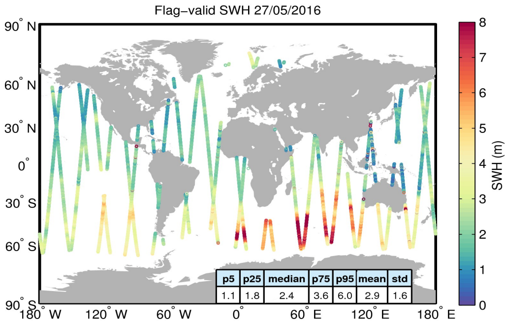
Figure 15. Geographical distribution of flag-valid SWH data over oceans and lakes for 27/05/2016. The statistical values shown in the table refer to the SWH in m and are calculated over all measurements shown in the figure.
