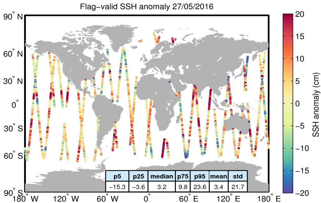
Figure 5. Geographical distribution of flag-valid 1-Hz SSH anomaly data over oceans and lakes for 27/05/2016. The statistical values shown in the table refer to the SSH anomaly in cm and are calculated over all measurements shown in the figure.
