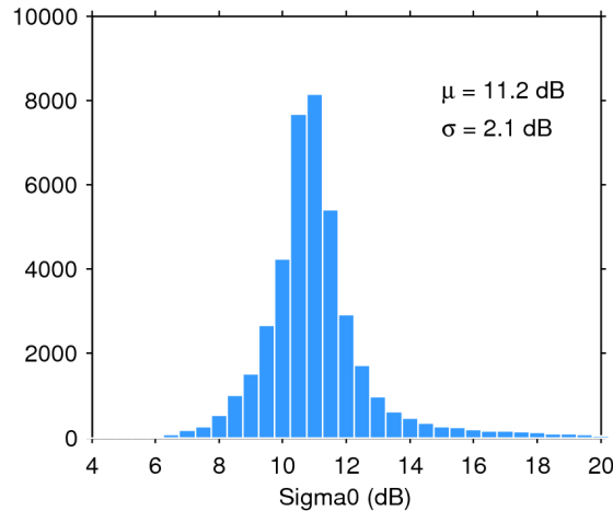
Figure 25. Histogram of flag-valid sigma0 over oceans and lakes for 27/05/2016. The mean ( \mu ) and standard deviation ( \sigma ) are also shown. Note that values outside [4 20] dB are excluded from the histogram for the sake of readability but not from the computation of \mu and \sigma .
