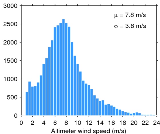
Figure 35. Histogram of science-valid wind over oceans and lakes for 27/05/2016. The mean ( \mu ) and standard deviation ( \sigma ) are also shown. Note that values larger than 24 m/s are excluded from the histogram for the sake of readability but not from the computation of \mu and \sigma .
