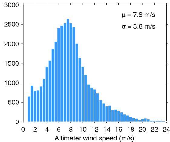
Figure 33. Histogram of flag-valid wind over oceans and lakes for 27/05/2016. The mean ( \mu ) and standard deviation ( \sigma ) are also shown. Note that values larger than 24 m/s are excluded from the histogram for the sake of readability but not from the computation of \mu and \sigma .
