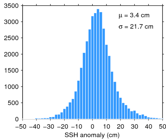
Figure 7. Histogram of flag-valid SSH anomaly over oceans and lakes for 27/05/2016. The mean ( \mu ) and standard deviation ( \sigma ) are also shown. Note that values outside [-50\ 50] cm are excluded from the histogram for the sake of readability but not from the computation of \mu and \sigma .
