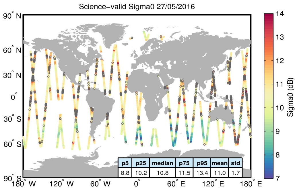
Figure 27. Geographical distribution of science-valid sigma0 data over oceans and lakes for 27/05/2016. The statistical values shown in the table refer to the sigma0 in dB and are calculated over all measurements shown in the figure. Gray circles denote records that have been rejected based on the editing criteria described in Table 4.
