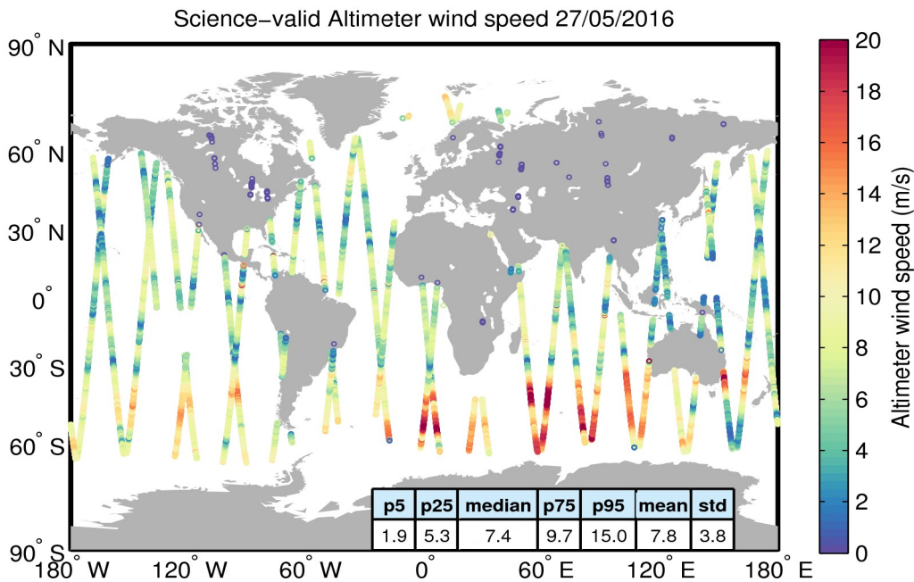
Figure 34. Geographical distribution of science-valid wind data over oceans and lakes for 27/05/2016. The statistical values shown in the table refer to the wind in m/s and are calculated over all measurements shown in the figure. Gray circles denote records that have been rejected based on the editing criteria described in Table 5.
