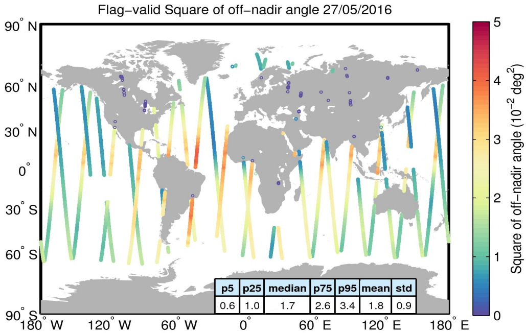
Figure 37. Geographical distribution of flag-valid mispointing data over oceans and lakes for 27/05/2016. The statistical values shown in the table refer to the mispointing in 10^{-2} deg 2 and are calculated over all measurements shown in the figure.
