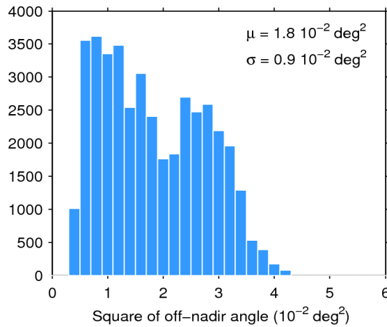
Figure 39. Histogram of flag-valid mispointing over oceans and lakes for 27/05/2016. The mean ( \mu ) and standard deviation ( \sigma ) are also shown. Note that values larger than 6 \cdot 10^{-2} \text{ deg}^2 are excluded from the histogram for the sake of readability but not from the computation of \mu and \sigma .
