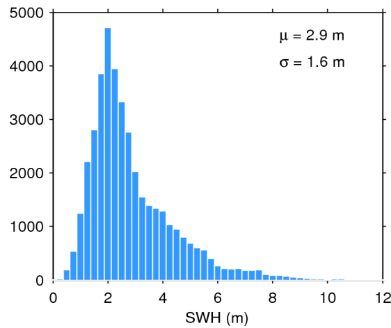
Figure 17. Histogram of flag-valid SWH over oceans and lakes for 27/05/2016. The mean ( \mu ) and standard deviation ( \sigma ) are also shown. Note that values larger than 12 m are excluded from the histogram for the sake of readability but not from the computation of \mu and \sigma .
