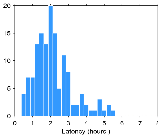
Figure 2. Histogram of the data latency for 27/05/2016. The y-axis denotes the number of files that are made available with a delay of x-hours with respect to the mean time of the records stored in the file.
