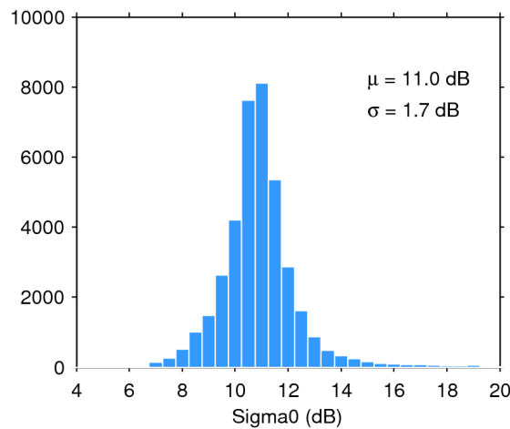
Figure 28. Histogram of science-valid sigma0 over oceans and lakes for 27/05/2016. The mean ( \mu ) and standard deviation ( \sigma ) are also shown. Note that values outside [4 20] dB are excluded from the histogram for the sake of readability but not from the computation of \mu and \sigma .
