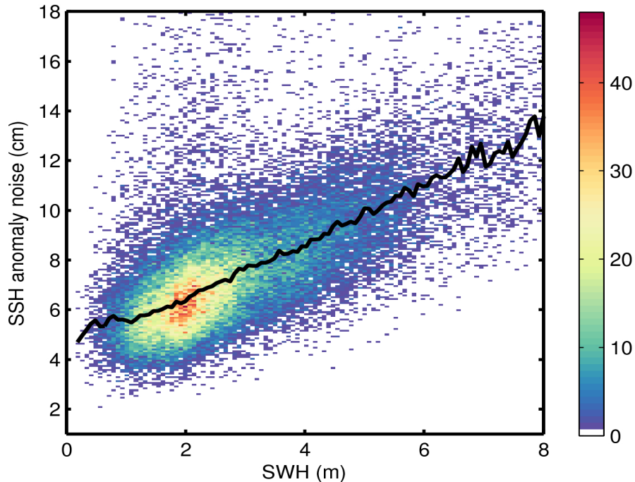
Figure 9. 2D histogram showing flag-valid SSH anomaly noise as a function of SWH for 27/05/2016. The black line denotes the median SSH anomaly noise as a function of SWH.
