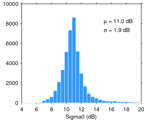
Figure 25. Histogram of flag-valid sigma0 over oceans and lakes for 26/05/2016. The mean ( \mu ) and standard deviation ( \sigma ) are also shown. Note that values outside [4 20] dB are excluded from the histogram for the sake of readability but not from the computation of \mu and \sigma .
