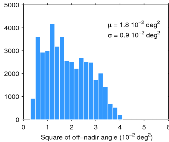
Figure 39. Histogram of flag-valid mispointing over oceans and lakes for 26/05/2016. The mean ( \mu ) and standard deviation ( \sigma ) are also shown. Note that values larger than 6 \cdot 10^{-2} \text{ deg}^2 are excluded from the histogram for the sake of readability but not from the computation of \mu and \sigma .
