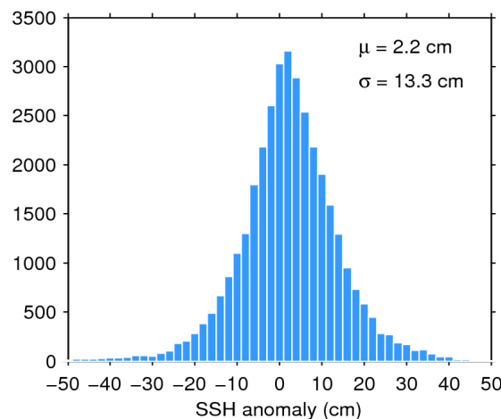
Figure 11. Histogram of science-valid SSH anomaly over oceans and lakes for 26/05/2016. The mean ( \mu ) and standard deviation ( \sigma ) are also shown. Note that values outside [-50 50] cm are excluded from the histogram for the sake of readability but not from the computation of \mu and \sigma .
