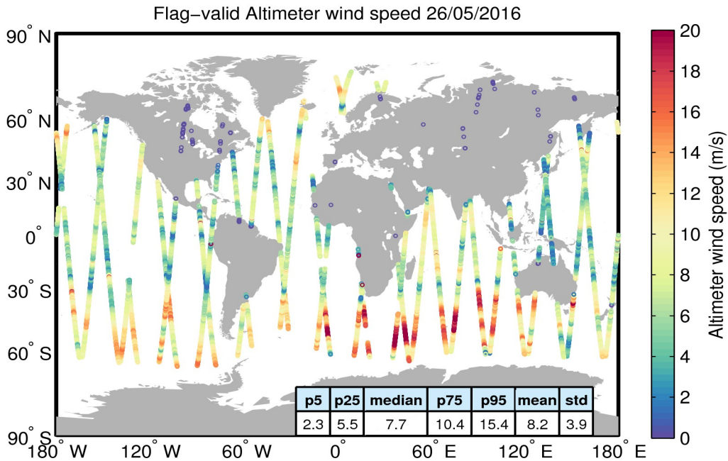
Figure 31. Geographical distribution of flag-valid wind data over oceans and lakes for 26/05/2016. The statistical values shown in the table refer to the wind in m/s and are calculated over all measurements shown in the figure.
