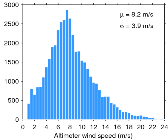
Figure 33. Histogram of flag-valid wind over oceans and lakes for 26/05/2016. The mean ( \mu ) and standard deviation ( \sigma ) are also shown. Note that values larger than 24 m/s are excluded from the histogram for the sake of readability but not from the computation of \mu and \sigma .
