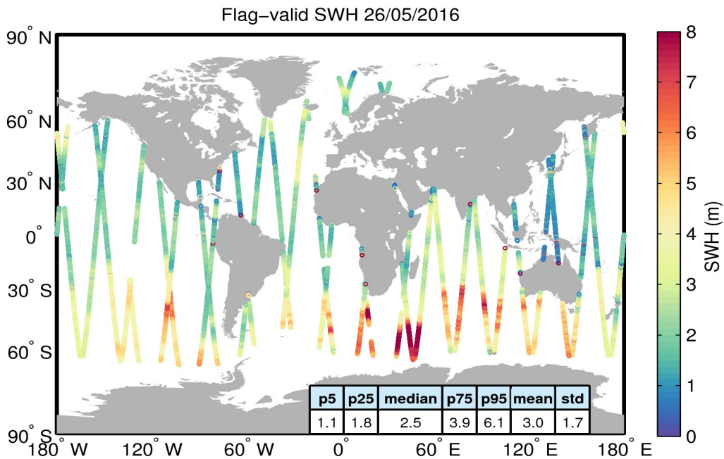
Figure 15. Geographical distribution of flag-valid SWH data over oceans and lakes for 26/05/2016. The statistical values shown in the table refer to the SWH in m and are calculated over all measurements shown in the figure.
