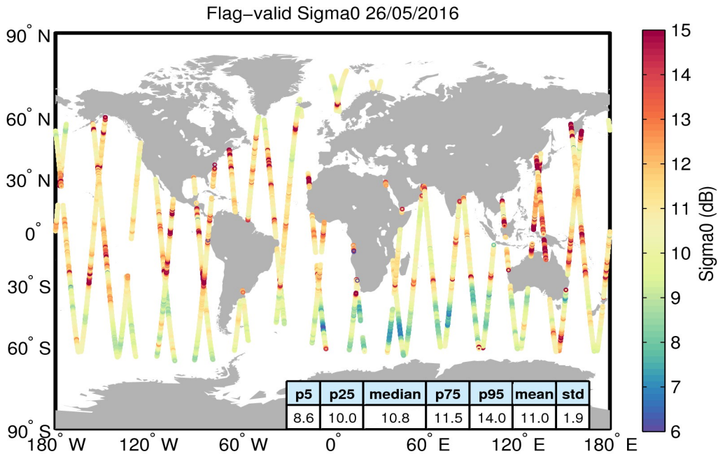
Figure 23. Geographical distribution of flag-valid sigma0 data over oceans and lakes for 26/05/2016. The statistical values shown in the table refer to the sigma0 in dB and are calculated over all measurements shown in the figure.
