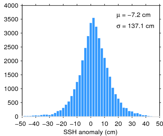
Figure 7. Histogram of flag-valid SSH anomaly over oceans and lakes for 26/05/2016. The mean ( \mu ) and standard deviation ( \sigma ) are also shown. Note that values outside [-50 50] cm are excluded from the histogram for the sake of readability but not from the computation of \mu and \sigma .
