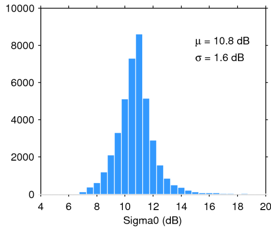
Figure 28. Histogram of science-valid sigma0 over oceans and lakes for 26/05/2016. The mean ( \mu ) and standard deviation ( \sigma ) are also shown. Note that values outside [4 20] dB are excluded from the histogram for the sake of readability but not from the computation of \mu and \sigma .
