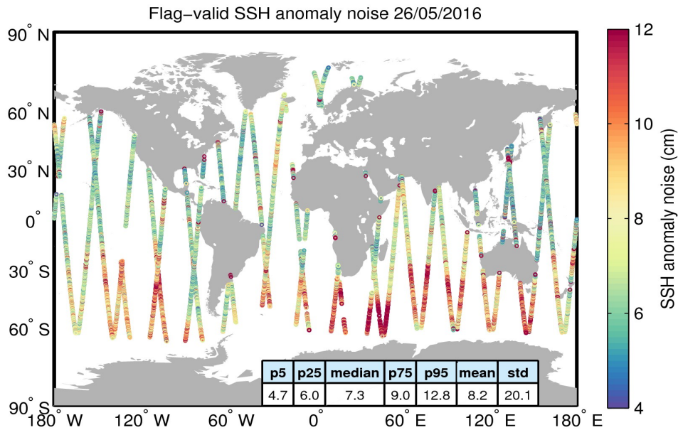
Figure 8. Geographical distribution of flag-valid 20-Hz SSH anomaly measurement noise over oceans and lakes for 26/05/2016. The statistical values shown in the table refer to the SSH anomaly noise and are calculated over all measurements shown in the figure.
