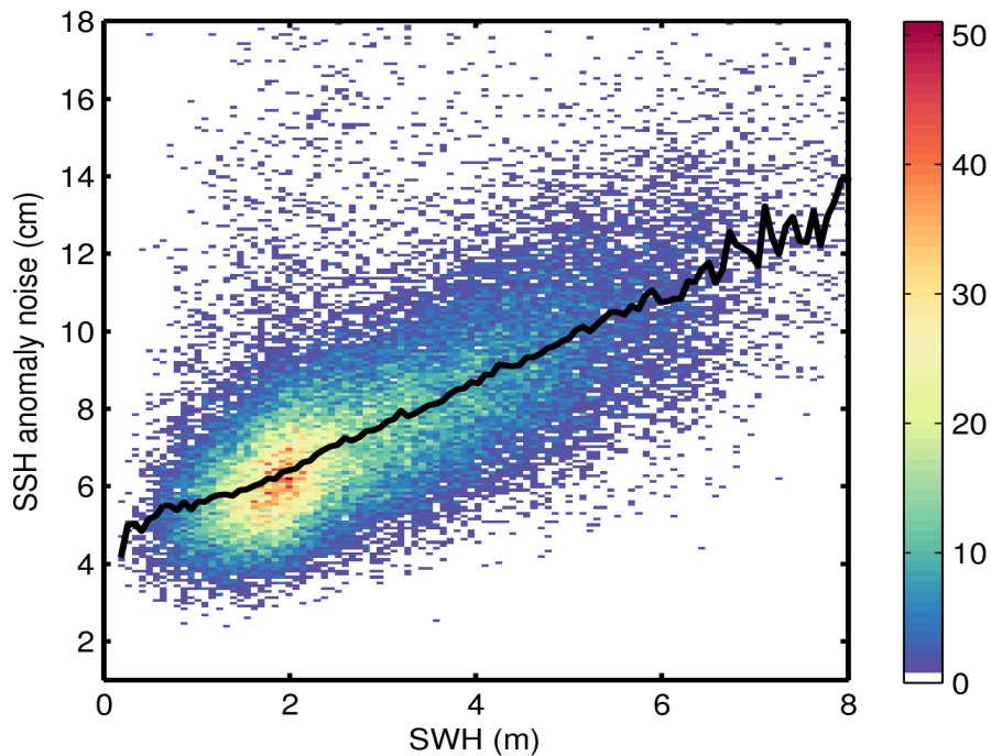
Figure 9. 2D histogram showing flag-valid SSH anomaly noise as a function of SWH for 26/05/2016. The black line denotes the median SSH anomaly noise as a function of SWH.
