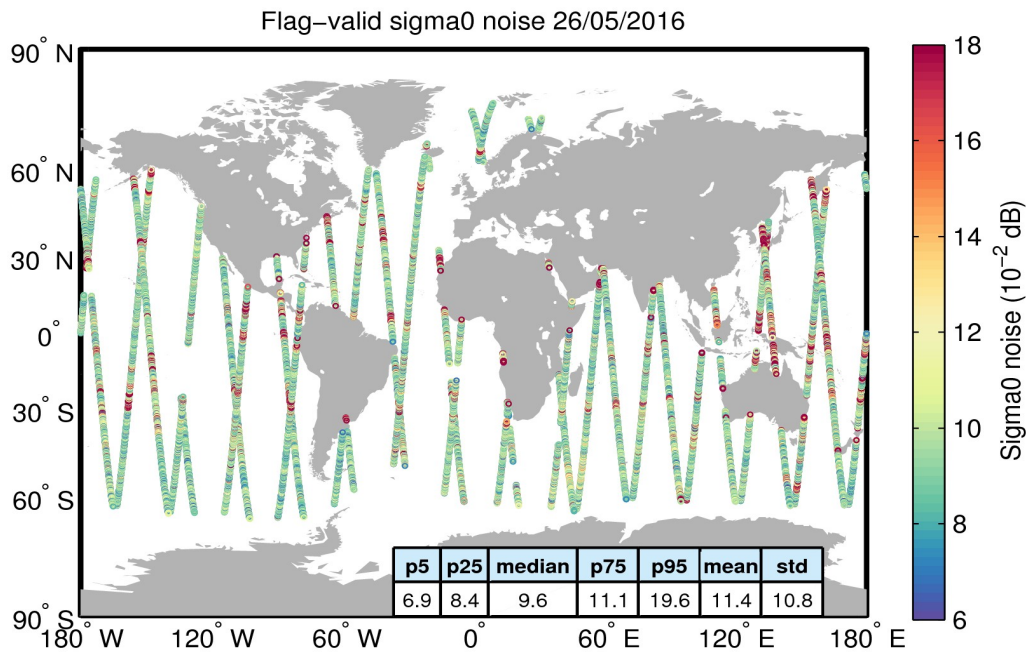
Figure 26. Geographical distribution of flag-valid 20-Hz sigma0 measurement noise over oceans and lakes for 26/05/2016. The statistical values shown in the table refer to the sigma0 noise and are calculated over all measurements shown in the figure.
