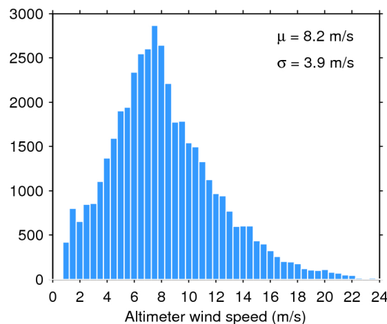
Figure 35. Histogram of science-valid wind over oceans and lakes for 26/05/2016. The mean ( \mu ) and standard deviation ( \sigma ) are also shown. Note that values larger than 24 m/s are excluded from the histogram for the sake of readability but not from the computation of \mu and \sigma .
