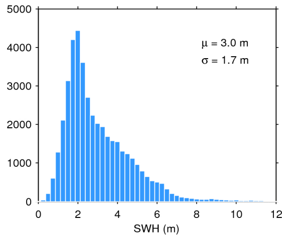
Figure 17. Histogram of flag-valid SWH over oceans and lakes for 26/05/2016. The mean ( \mu ) and standard deviation ( \sigma ) are also shown. Note that values larger than 12 m are excluded from the histogram for the sake of readability but not from the computation of \mu and \sigma .
