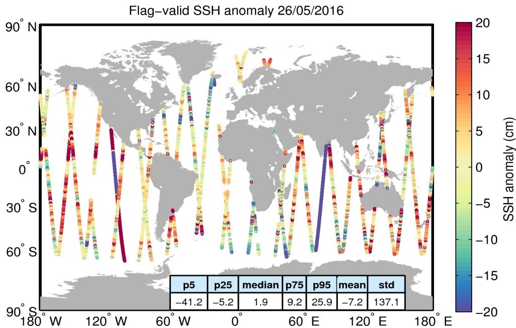
Figure 5. Geographical distribution of flag-valid 1-Hz SSH anomaly data over oceans and lakes for 26/05/2016. The statistical values shown in the table refer to the SSH anomaly in cm and are calculated over all measurements shown in the figure.
