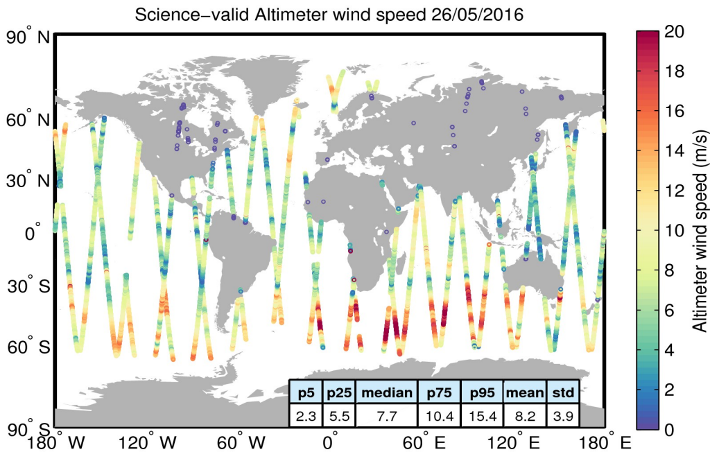
Figure 34. Geographical distribution of science-valid wind data over oceans and lakes for 26/05/2016. The statistical values shown in the table refer to the wind in m/s and are calculated over all measurements shown in the figure. Gray circles denote records that have been rejected based on the editing criteria described in Table 5.
