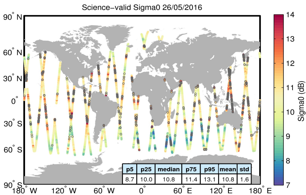
Figure 27. Geographical distribution of science-valid sigma0 data over oceans and lakes for 26/05/2016. The statistical values shown in the table refer to the sigma0 in dB and are calculated over all measurements shown in the figure. Gray circles denote records that have been rejected based on the editing criteria described in Table 4.
