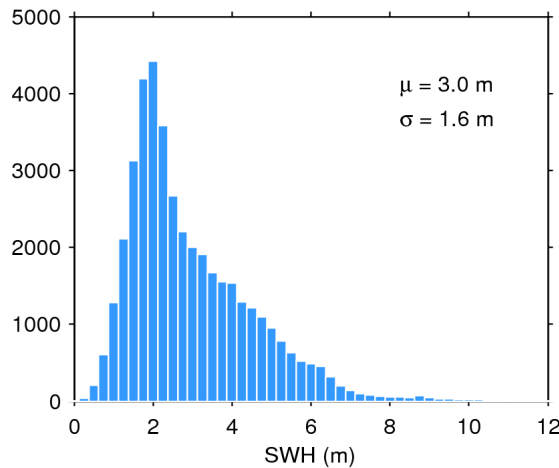
Figure 20. Histogram of science-valid SWH over oceans and lakes for 26/05/2016. The mean ( \mu ) and standard deviation ( \sigma ) are also shown. Note that values larger than 12 m are excluded from the histogram for the sake of readability but not from the computation of \mu and \sigma .
