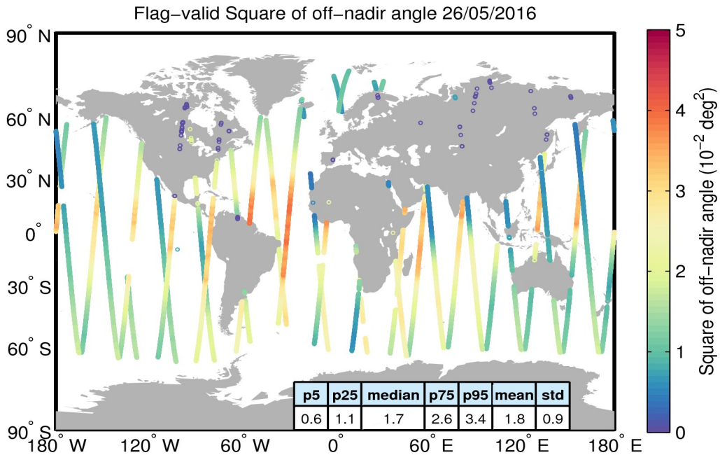
Figure 37. Geographical distribution of flag-valid mispointing data over oceans and lakes for 26/05/2016. The statistical values shown in the table refer to the mispointing in 10^{-2} deg 2 and are calculated over all measurements shown in the figure.
