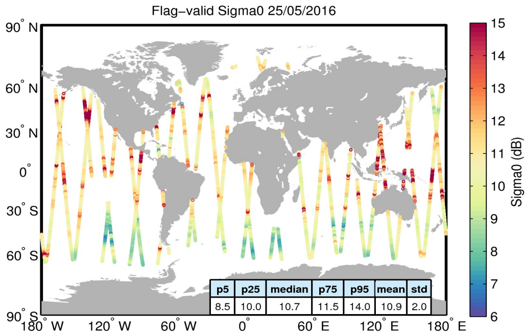
Figure 23. Geographical distribution of flag-valid sigma0 data over oceans and lakes for 25/05/2016. The statistical values shown in the table refer to the sigma0 in dB and are calculated over all measurements shown in the figure.
