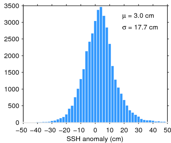
Figure 7. Histogram of flag-valid SSH anomaly over oceans and lakes for 25/05/2016. The mean ( \mu ) and standard deviation ( \sigma ) are also shown. Note that values outside [-50 50] cm are excluded from the histogram for the sake of readability but not from the computation of \mu and \sigma .
