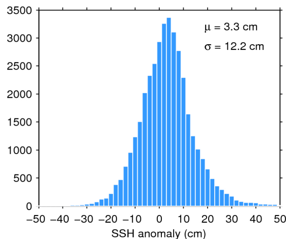
Figure 11. Histogram of science-valid SSH anomaly over oceans and lakes for 25/05/2016. The mean ( \mu ) and standard deviation ( \sigma ) are also shown. Note that values outside [-50 50] cm are excluded from the histogram for the sake of readability but not from the computation of \mu and \sigma .
