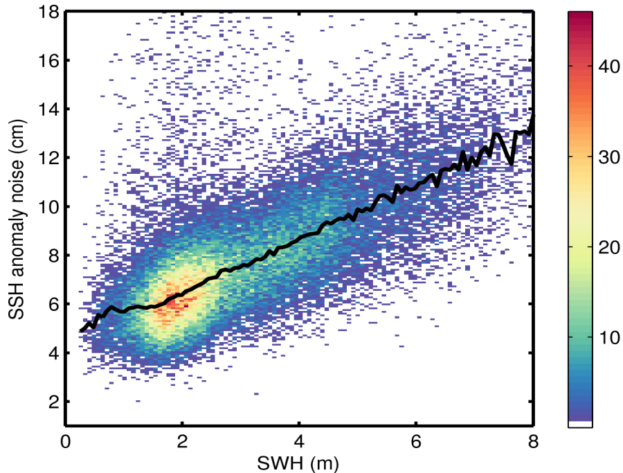
Figure 9. 2D histogram showing flag-valid SSH anomaly noise as a function of SWH for 25/05/2016. The black line denotes the median SSH anomaly noise as a function of SWH.
