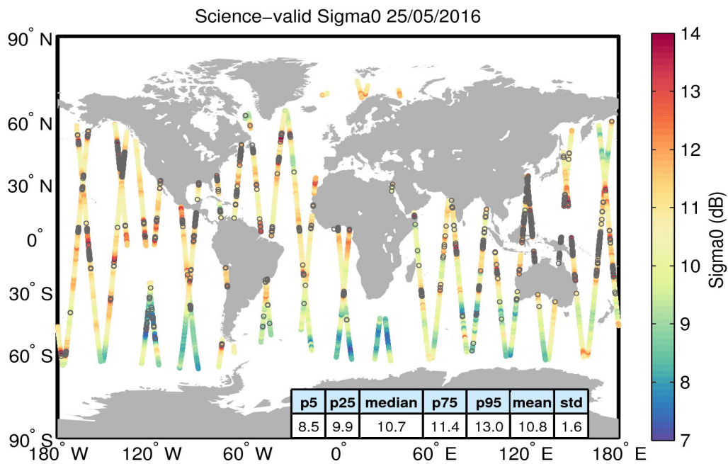
Figure 27. Geographical distribution of science-valid sigma0 data over oceans and lakes for 25/05/2016. The statistical values shown in the table refer to the sigma0 in dB and are calculated over all measurements shown in the figure. Gray circles denote records that have been rejected based on the editing criteria described in Table 4.
