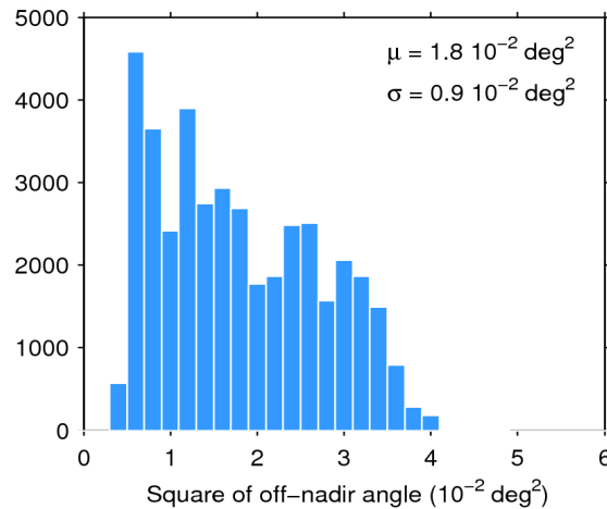
Figure 39. Histogram of flag-valid mispointing over oceans and lakes for 25/05/2016. The mean ( \mu ) and standard deviation ( \sigma ) are also shown. Note that values larger than 6 \cdot 10^{-2} \text{ deg}^2 are excluded from the histogram for the sake of readability but not from the computation of \mu and \sigma .
