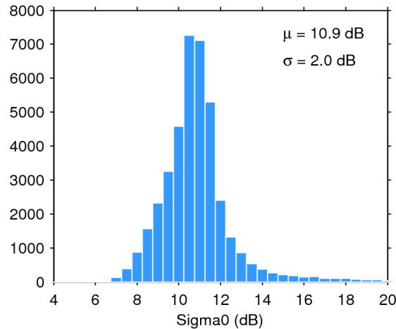
Figure 25. Histogram of flag-valid sigma0 over oceans and lakes for 25/05/2016. The mean ( \mu ) and standard deviation ( \sigma ) are also shown. Note that values outside [4 20] dB are excluded from the histogram for the sake of readability but not from the computation of \mu and \sigma .
