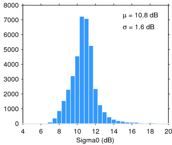
Figure 28. Histogram of science-valid sigma0 over oceans and lakes for 25/05/2016. The mean ( \mu ) and standard deviation ( \sigma ) are also shown. Note that values outside [4 20] dB are excluded from the histogram for the sake of readability but not from the computation of \mu and \sigma .
