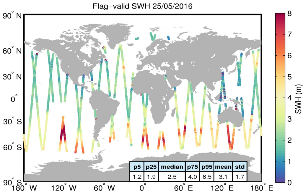
Figure 15. Geographical distribution of flag-valid SWH data over oceans and lakes for 25/05/2016. The statistical values shown in the table refer to the SWH in m and are calculated over all measurements shown in the figure.
