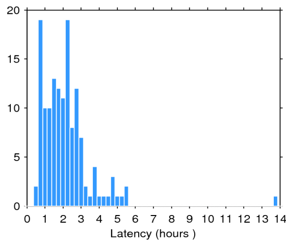
Figure 2. Histogram of the data latency for 25/05/2016. The y-axis denotes the number of files that are made available with a delay of x-hours with respect to the mean time of the records stored in the file.
