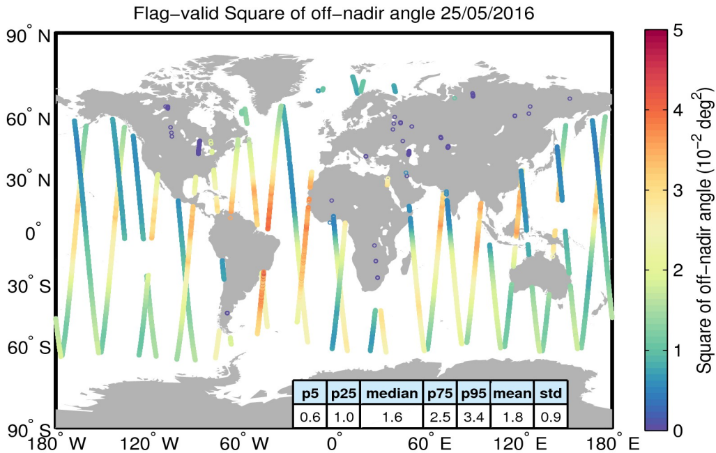
Figure 37. Geographical distribution of flag-valid mispointing data over oceans and lakes for 25/05/2016. The statistical values shown in the table refer to the mispointing in 10^{-2} \text{ deg}^2 and are calculated over all measurements shown in the figure.
