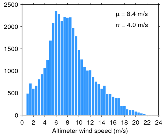
Figure 33. Histogram of flag-valid wind over oceans and lakes for 25/05/2016. The mean ( \mu ) and standard deviation ( \sigma ) are also shown. Note that values larger than 24 m/s are excluded from the histogram for the sake of readability but not from the computation of \mu and \sigma .
