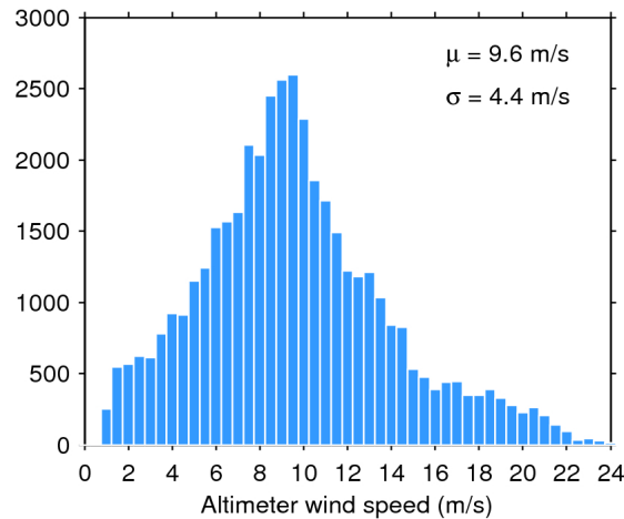
Figure 33. Histogram of flag-valid wind over oceans and lakes for 24/05/2016. The mean ( \mu ) and standard deviation ( \sigma ) are also shown. Note that values larger than 24 m/s are excluded from the histogram for the sake of readability but not from the computation of \mu and \sigma .
