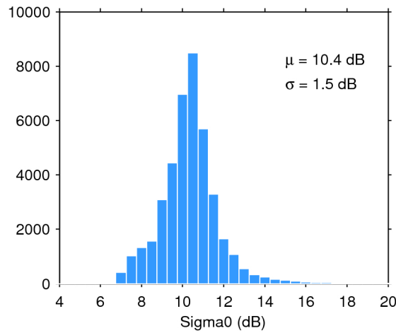
Figure 28. Histogram of science-valid sigma0 over oceans and lakes for 24/05/2016. The mean ( \mu ) and standard deviation ( \sigma ) are also shown. Note that values outside [4 20] dB are excluded from the histogram for the sake of readability but not from the computation of \mu and \sigma .
