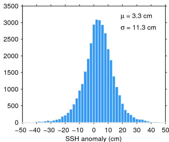
Figure 11. Histogram of science-valid SSH anomaly over oceans and lakes for 24/05/2016. The mean ( \mu ) and standard deviation ( \sigma ) are also shown. Note that values outside [-50 50] cm are excluded from the histogram for the sake of readability but not from the computation of \mu and \sigma .
