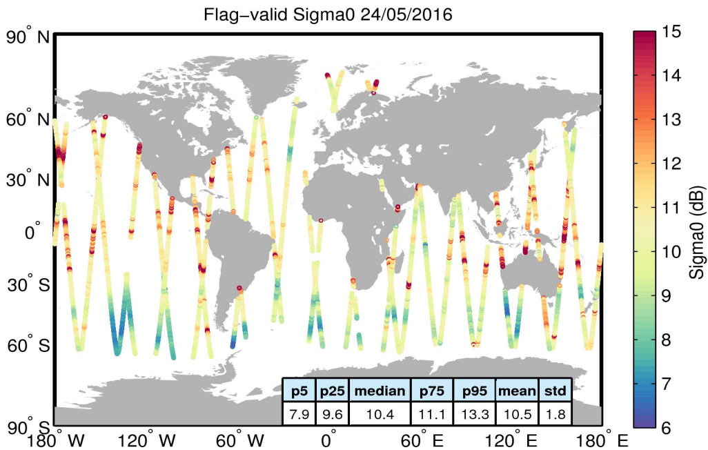
Figure 23. Geographical distribution of flag-valid sigma0 data over oceans and lakes for 24/05/2016. The statistical values shown in the table refer to the sigma0 in dB and are calculated over all measurements shown in the figure.
