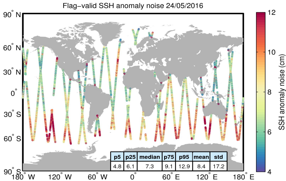
Figure 8. Geographical distribution of flag-valid 20-Hz SSH anomaly measurement noise over oceans and lakes for 24/05/2016. The statistical values shown in the table refer to the SSH anomaly noise and are calculated over all measurements shown in the figure.
