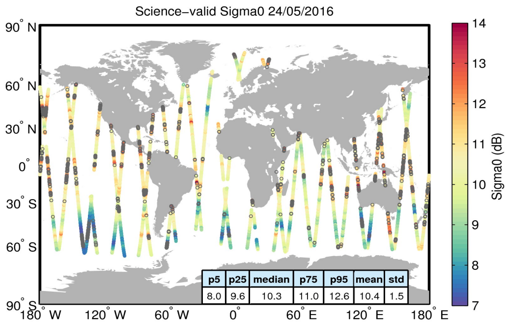
Figure 27. Geographical distribution of science-valid sigma0 data over oceans and lakes for 24/05/2016. The statistical values shown in the table refer to the sigma0 in dB and are calculated over all measurements shown in the figure. Gray circles denote records that have been rejected based on the editing criteria described in Table 4.
