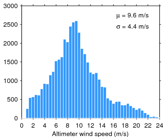
Figure 35. Histogram of science-valid wind over oceans and lakes for 24/05/2016. The mean ( \mu ) and standard deviation ( \sigma ) are also shown. Note that values larger than 24 m/s are excluded from the histogram for the sake of readability but not from the computation of \mu and \sigma .
