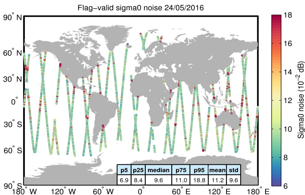
Figure 26. Geographical distribution of flag-valid 20-Hz sigma0 measurement noise over oceans and lakes for 24/05/2016. The statistical values shown in the table refer to the sigma0 noise and are calculated over all measurements shown in the figure.
