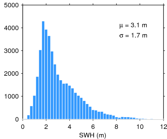
Figure 20. Histogram of science-valid SWH over oceans and lakes for 24/05/2016. The mean ( \mu ) and standard deviation ( \sigma ) are also shown. Note that values larger than 12 m are excluded from the histogram for the sake of readability but not from the computation of \mu and \sigma .
