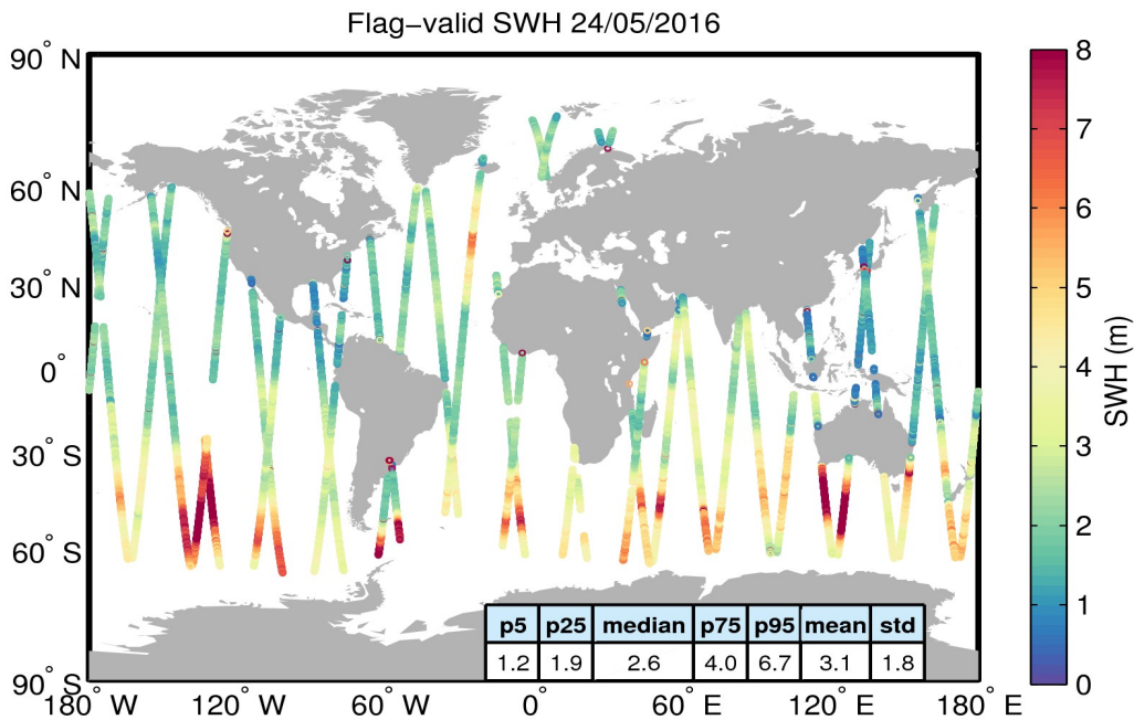
Figure 15. Geographical distribution of flag-valid SWH data over oceans and lakes for 24/05/2016. The statistical values shown in the table refer to the SWH in m and are calculated over all measurements shown in the figure.
