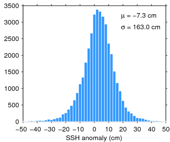
Figure 7. Histogram of flag-valid SSH anomaly over oceans and lakes for 24/05/2016. The mean ( \mu ) and standard deviation ( \sigma ) are also shown. Note that values outside [-50 50] cm are excluded from the histogram for the sake of readability but not from the computation of \mu and \sigma .
