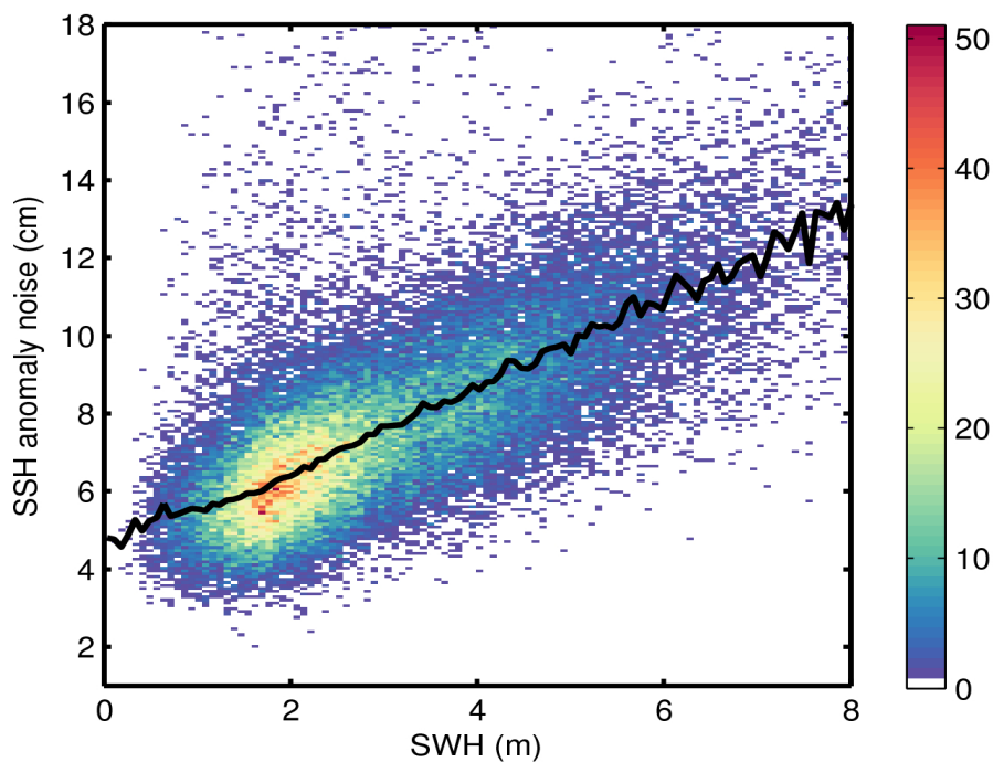
Figure 9. 2D histogram showing flag-valid SSH anomaly noise as a function of SWH for 24/05/2016. The black line denotes the median SSH anomaly noise as a function of SWH.
