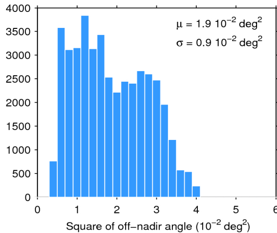
Figure 39. Histogram of flag-valid mispointing over oceans and lakes for 24/05/2016. The mean ( \mu ) and standard deviation ( \sigma ) are also shown. Note that values larger than 6 \cdot 10^{-2} \text{ deg}^2 are excluded from the histogram for the sake of readability but not from the computation of \mu and \sigma .
