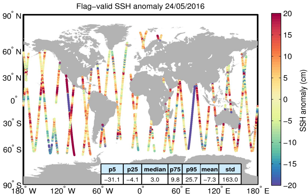
Figure 5. Geographical distribution of flag-valid 1-Hz SSH anomaly data over oceans and lakes for 24/05/2016. The statistical values shown in the table refer to the SSH anomaly in cm and are calculated over all measurements shown in the figure.
