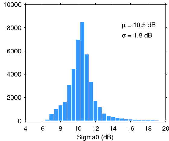
Figure 25. Histogram of flag-valid sigma0 over oceans and lakes for 24/05/2016. The mean ( \mu ) and standard deviation ( \sigma ) are also shown. Note that values outside [4 20] dB are excluded from the histogram for the sake of readability but not from the computation of \mu and \sigma .
