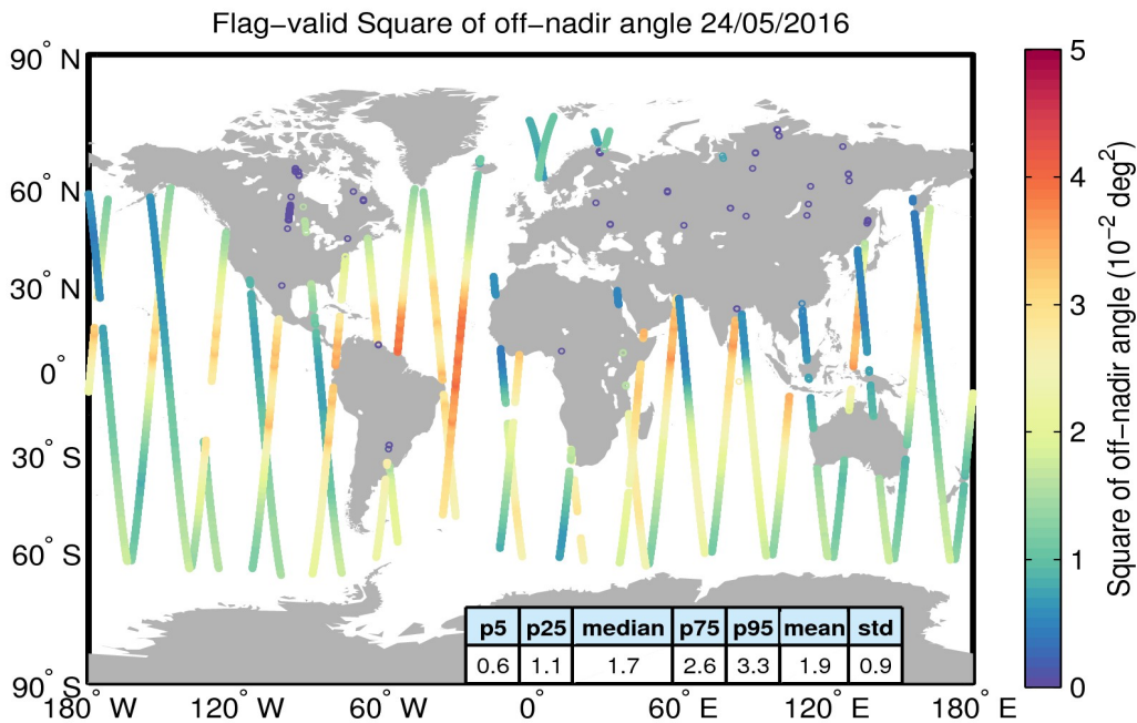
Figure 37. Geographical distribution of flag-valid mispointing data over oceans and lakes for 24/05/2016. The statistical values shown in the table refer to the mispointing in 10^{-2} deg 2 and are calculated over all measurements shown in the figure.
