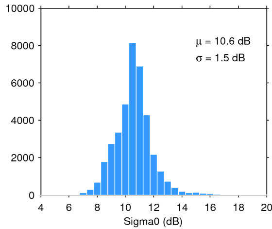
Figure 28. Histogram of science-valid sigma0 over oceans and lakes for 23/05/2016. The mean ( \mu ) and standard deviation ( \sigma ) are also shown. Note that values outside [4 20] dB are excluded from the histogram for the sake of readability but not from the computation of \mu and \sigma .
