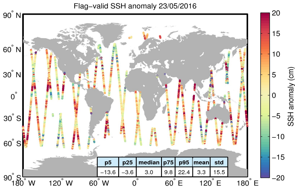
Figure 5. Geographical distribution of flag-valid 1-Hz SSH anomaly data over oceans and lakes for 23/05/2016. The statistical values shown in the table refer to the SSH anomaly in cm and are calculated over all measurements shown in the figure.
