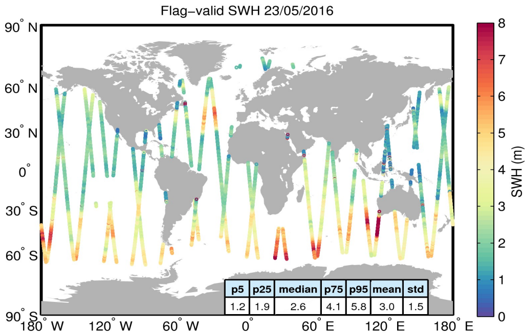
Figure 15. Geographical distribution of flag-valid SWH data over oceans and lakes for 23/05/2016. The statistical values shown in the table refer to the SWH in m and are calculated over all measurements shown in the figure.
