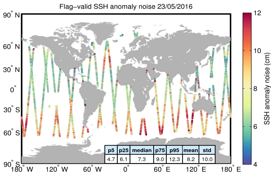
Figure 8. Geographical distribution of flag-valid 20-Hz SSH anomaly measurement noise over oceans and lakes for 23/05/2016. The statistical values shown in the table refer to the SSH anomaly noise and are calculated over all measurements shown in the figure.
