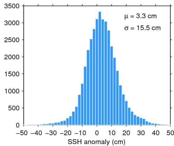
Figure 7. Histogram of flag-valid SSH anomaly over oceans and lakes for 23/05/2016. The mean ( \mu ) and standard deviation ( \sigma ) are also shown. Note that values outside [-50\ 50] cm are excluded from the histogram for the sake of readability but not from the computation of \mu and \sigma .
