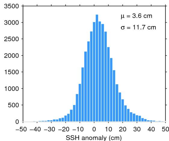
Figure 11. Histogram of science-valid SSH anomaly over oceans and lakes for 23/05/2016. The mean ( \mu ) and standard deviation ( \sigma ) are also shown. Note that values outside [-50 50] cm are excluded from the histogram for the sake of readability but not from the computation of \mu and \sigma .
