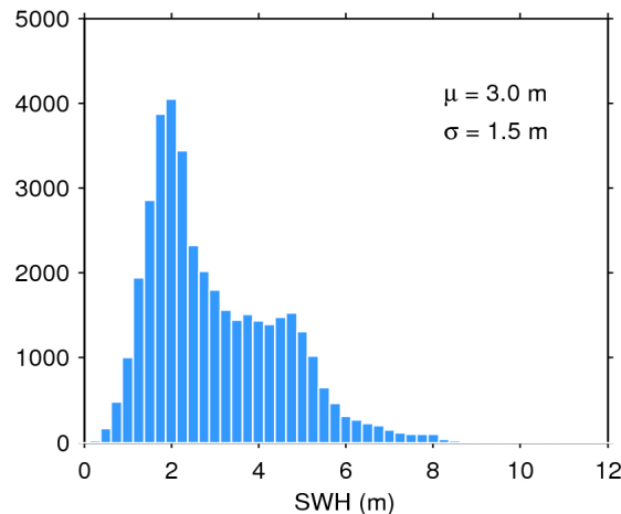
Figure 20. Histogram of science-valid SWH over oceans and lakes for 23/05/2016. The mean ( \mu ) and standard deviation ( \sigma ) are also shown. Note that values larger than 12 m are excluded from the histogram for the sake of readability but not from the computation of \mu and \sigma .
