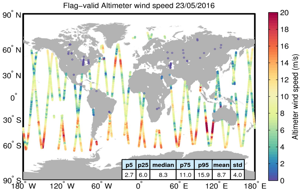
Figure 31. Geographical distribution of flag-valid wind data over oceans and lakes for 23/05/2016. The statistical values shown in the table refer to the wind in m/s and are calculated over all measurements shown in the figure.
