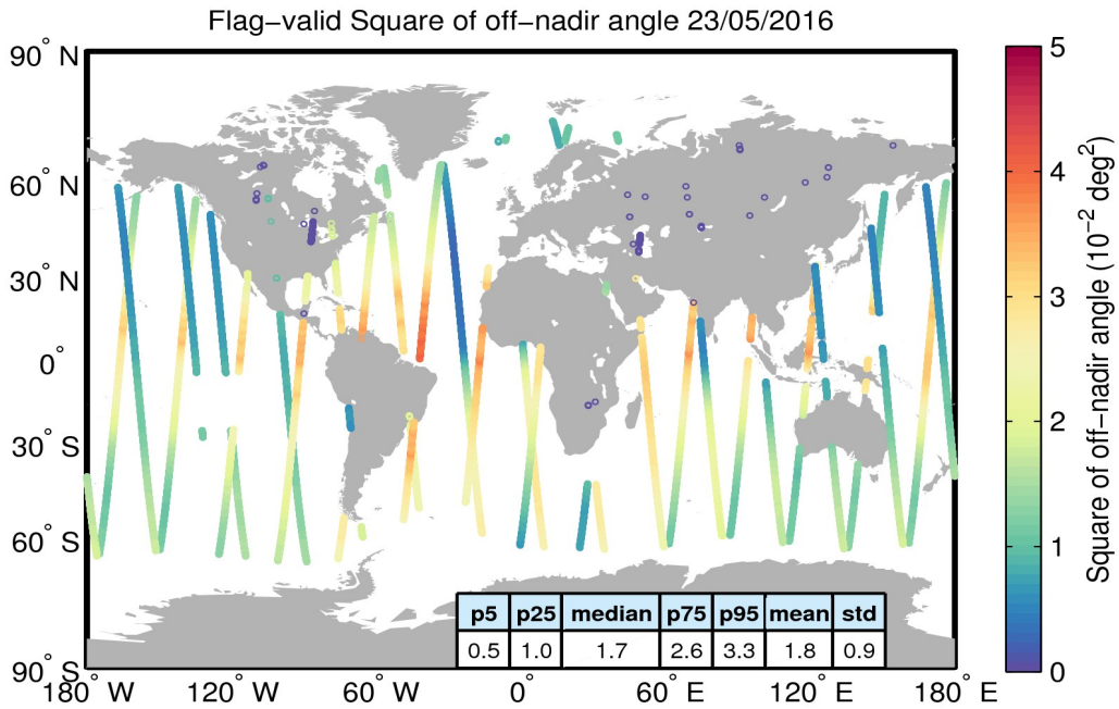
Figure 37. Geographical distribution of flag-valid mispointing data over oceans and lakes for 23/05/2016. The statistical values shown in the table refer to the mispointing in 10^{-2} \text{ deg}^2 and are calculated over all measurements shown in the figure.
