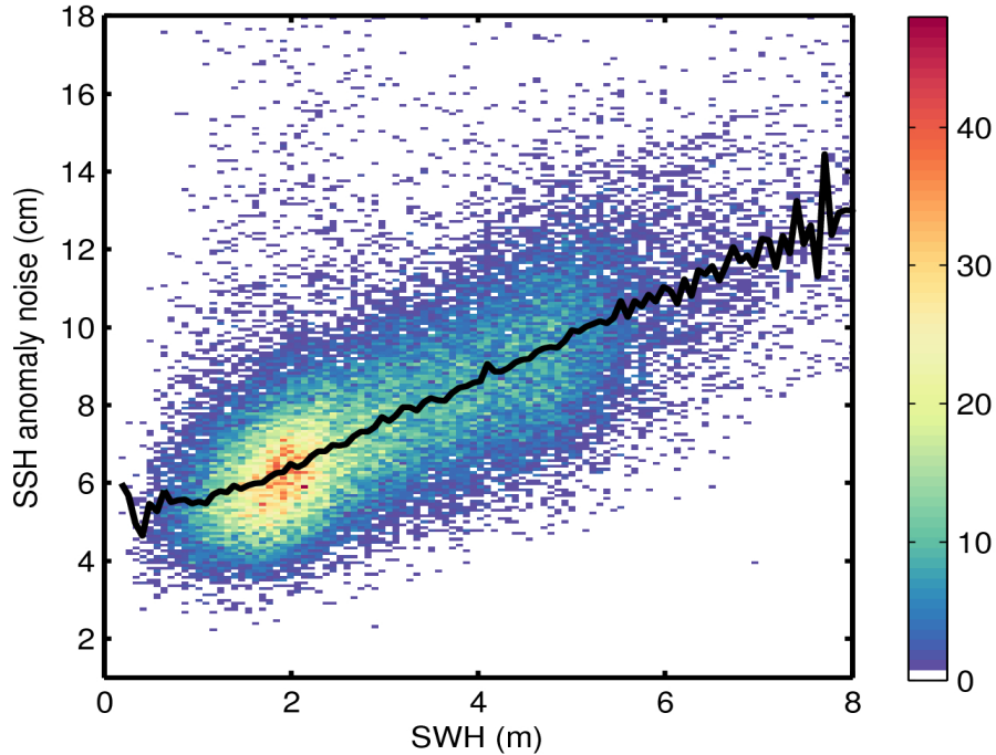
Figure 9. 2D histogram showing flag-valid SSH anomaly noise as a function of SWH for 23/05/2016. The black line denotes the median SSH anomaly noise as a function of SWH.
