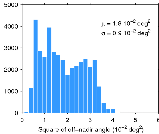
Figure 39. Histogram of flag-valid mispointing over oceans and lakes for 23/05/2016. The mean ( \mu ) and standard deviation ( \sigma ) are also shown. Note that values larger than 6 \cdot 10^{-2} \text{ deg}^2 are excluded from the histogram for the sake of readability but not from the computation of \mu and \sigma .
