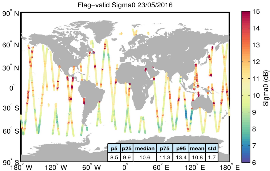
Figure 23. Geographical distribution of flag-valid sigma0 data over oceans and lakes for 23/05/2016. The statistical values shown in the table refer to the sigma0 in dB and are calculated over all measurements shown in the figure.
