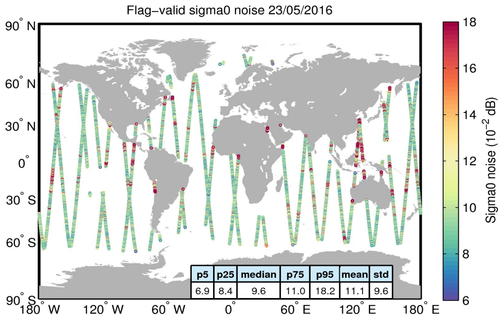
Figure 26. Geographical distribution of flag-valid 20-Hz sigma0 measurement noise over oceans and lakes for 23/05/2016. The statistical values shown in the table refer to the sigma0 noise and are calculated over all measurements shown in the figure.
