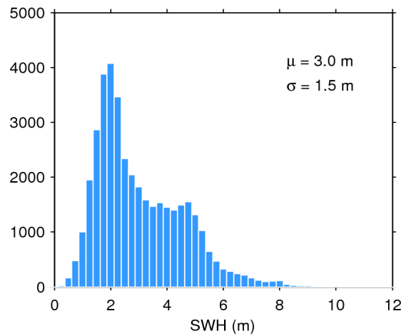
Figure 17. Histogram of flag-valid SWH over oceans and lakes for 23/05/2016. The mean ( \mu ) and standard deviation ( \sigma ) are also shown. Note that values larger than 12 m are excluded from the histogram for the sake of readability but not from the computation of \mu and \sigma .
