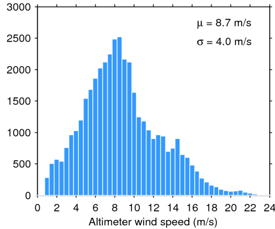
Figure 33. Histogram of flag-valid wind over oceans and lakes for 23/05/2016. The mean ( \mu ) and standard deviation ( \sigma ) are also shown. Note that values larger than 24 m/s are excluded from the histogram for the sake of readability but not from the computation of \mu and \sigma .
