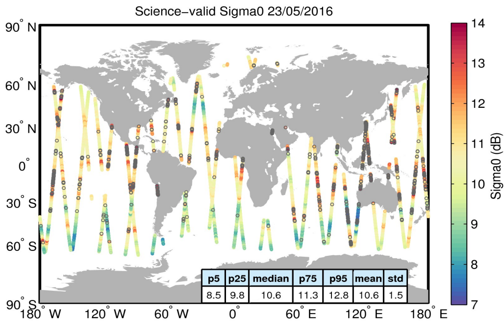
Figure 27. Geographical distribution of science-valid sigma0 data over oceans and lakes for 23/05/2016. The statistical values shown in the table refer to the sigma0 in dB and are calculated over all measurements shown in the figure. Gray circles denote records that have been rejected based on the editing criteria described in Table 4.
