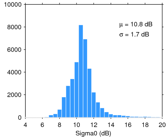
Figure 25. Histogram of flag-valid sigma0 over oceans and lakes for 23/05/2016. The mean ( \mu ) and standard deviation ( \sigma ) are also shown. Note that values outside [4 20] dB are excluded from the histogram for the sake of readability but not from the computation of \mu and \sigma .
