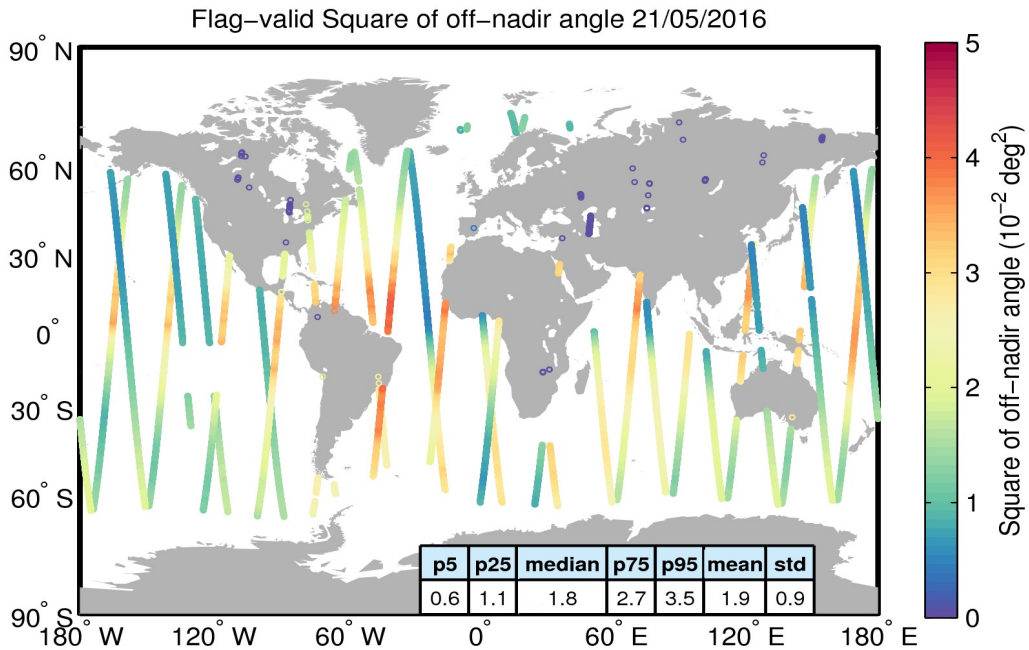
Figure 37. Geographical distribution of flag-valid mispointing data over oceans and lakes for 21/05/2016. The statistical values shown in the table refer to the mispointing in 10^{-2} deg 2 and are calculated over all measurements shown in the figure.
