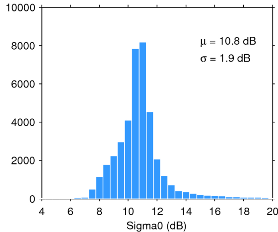
Figure 25. Histogram of flag-valid sigma0 over oceans and lakes for 21/05/2016. The mean ( \mu ) and standard deviation ( \sigma ) are also shown. Note that values outside [4 20] dB are excluded from the histogram for the sake of readability but not from the computation of \mu and \sigma .
