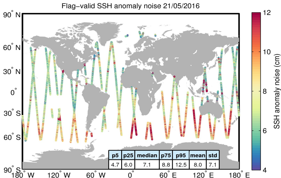
Figure 8. Geographical distribution of flag-valid 20-Hz SSH anomaly measurement noise over oceans and lakes for 21/05/2016. The statistical values shown in the table refer to the SSH anomaly noise and are calculated over all measurements shown in the figure.
