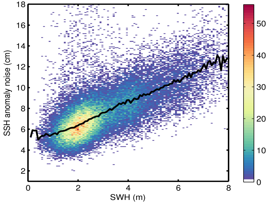
Figure 9. 2D histogram showing flag-valid SSH anomaly noise as a function of SWH for 21/05/2016. The black line denotes the median SSH anomaly noise as a function of SWH.
