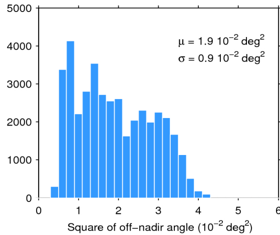
Figure 39. Histogram of flag-valid mispointing over oceans and lakes for 21/05/2016. The mean ( \mu ) and standard deviation ( \sigma ) are also shown. Note that values larger than 6 \cdot 10^{-2} \text{ deg}^2 are excluded from the histogram for the sake of readability but not from the computation of \mu and \sigma .
