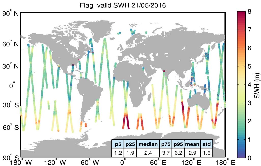
Figure 15. Geographical distribution of flag-valid SWH data over oceans and lakes for 21/05/2016. The statistical values shown in the table refer to the SWH in m and are calculated over all measurements shown in the figure.
