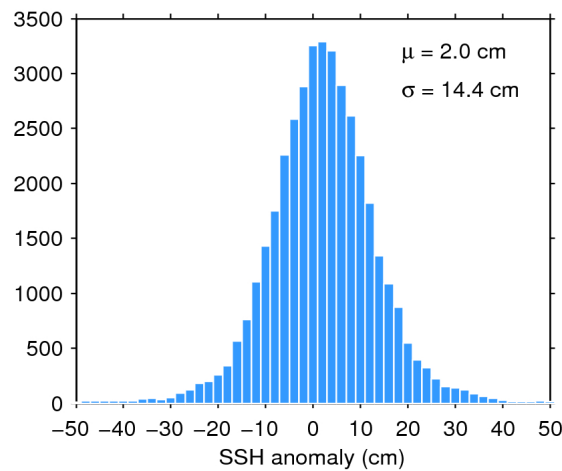
Figure 7. Histogram of flag-valid SSH anomaly over oceans and lakes for 21/05/2016. The mean ( \mu ) and standard deviation ( \sigma ) are also shown. Note that values outside [-50 50] cm are excluded from the histogram for the sake of readability but not from the computation of \mu and \sigma .
