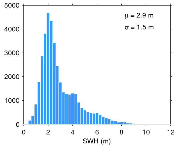
Figure 20. Histogram of science-valid SWH over oceans and lakes for 21/05/2016. The mean ( \mu ) and standard deviation ( \sigma ) are also shown. Note that values larger than 12 m are excluded from the histogram for the sake of readability but not from the computation of \mu and \sigma .
