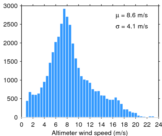
Figure 35. Histogram of science-valid wind over oceans and lakes for 21/05/2016. The mean ( \mu ) and standard deviation ( \sigma ) are also shown. Note that values larger than 24 m/s are excluded from the histogram for the sake of readability but not from the computation of \mu and \sigma .
