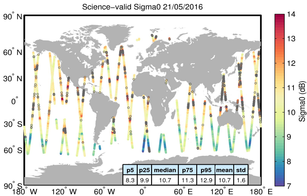
Figure 27. Geographical distribution of science-valid sigma0 data over oceans and lakes for 21/05/2016. The statistical values shown in the table refer to the sigma0 in dB and are calculated over all measurements shown in the figure. Gray circles denote records that have been rejected based on the editing criteria described in Table 4.
