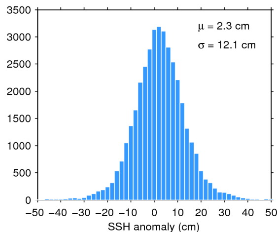
Figure 11. Histogram of science-valid SSH anomaly over oceans and lakes for 21/05/2016. The mean ( \mu ) and standard deviation ( \sigma ) are also shown. Note that values outside [-50 50] cm are excluded from the histogram for the sake of readability but not from the computation of \mu and \sigma .
