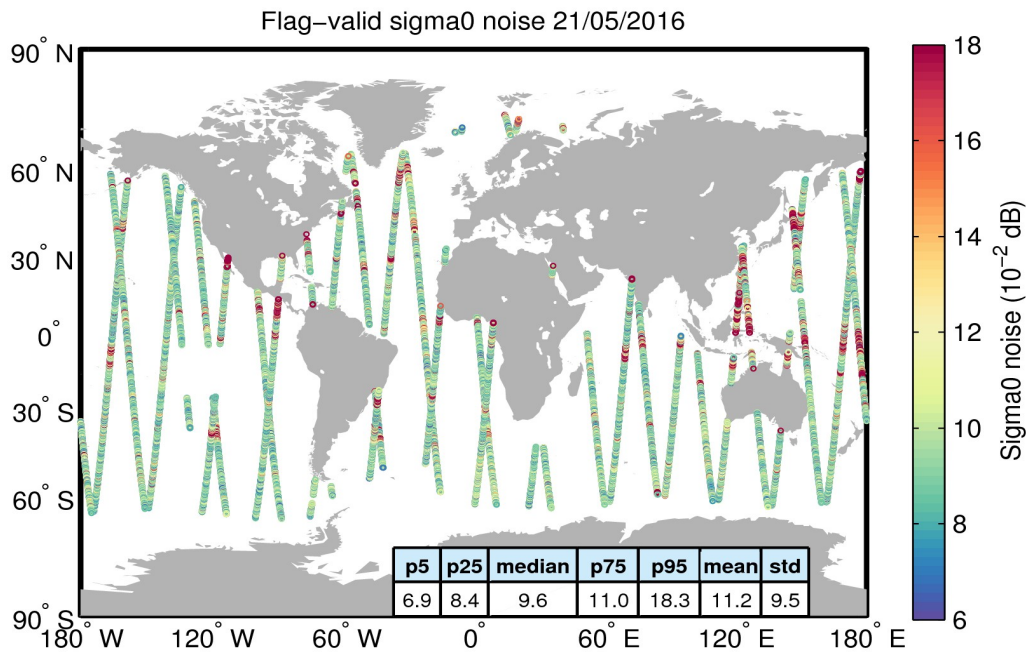
Figure 26. Geographical distribution of flag-valid 20-Hz sigma0 measurement noise over oceans and lakes for 21/05/2016. The statistical values shown in the table refer to the sigma0 noise and are calculated over all measurements shown in the figure.
