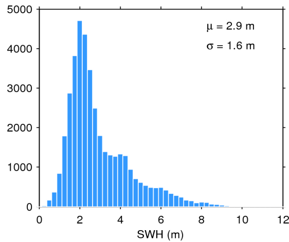
Figure 17. Histogram of flag-valid SWH over oceans and lakes for 21/05/2016. The mean ( \mu ) and standard deviation ( \sigma ) are also shown. Note that values larger than 12 m are excluded from the histogram for the sake of readability but not from the computation of \mu and \sigma .
