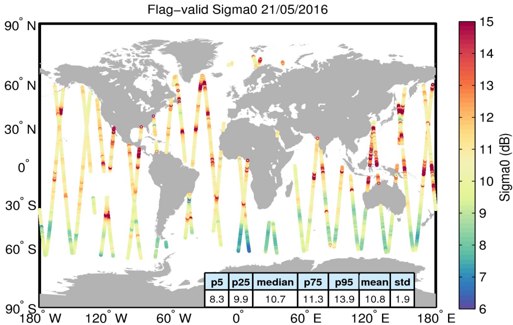
Figure 23. Geographical distribution of flag-valid sigma0 data over oceans and lakes for 21/05/2016. The statistical values shown in the table refer to the sigma0 in dB and are calculated over all measurements shown in the figure.
