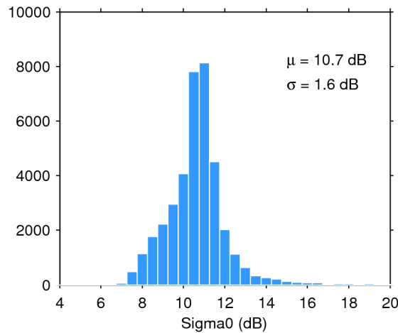
Figure 28. Histogram of science-valid sigma0 over oceans and lakes for 21/05/2016. The mean ( \mu ) and standard deviation ( \sigma ) are also shown. Note that values outside [4 20] dB are excluded from the histogram for the sake of readability but not from the computation of \mu and \sigma .
