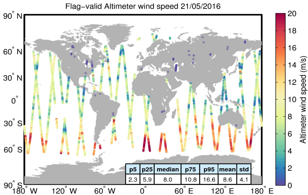
Figure 31. Geographical distribution of flag-valid wind data over oceans and lakes for 21/05/2016. The statistical values shown in the table refer to the wind in m/s and are calculated over all measurements shown in the figure.
