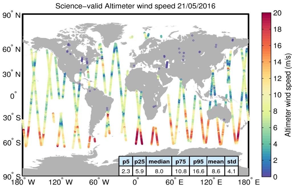
Figure 34. Geographical distribution of science-valid wind data over oceans and lakes for 21/05/2016. The statistical values shown in the table refer to the wind in m/s and are calculated over all measurements shown in the figure. Gray circles denote records that have been rejected based on the editing criteria described in Table 5.
