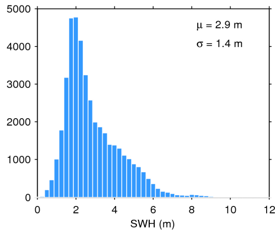
Figure 17. Histogram of flag-valid SWH over oceans and lakes for 20/05/2016. The mean ( \mu ) and standard deviation ( \sigma ) are also shown. Note that values larger than 12 m are excluded from the histogram for the sake of readability but not from the computation of \mu and \sigma .
