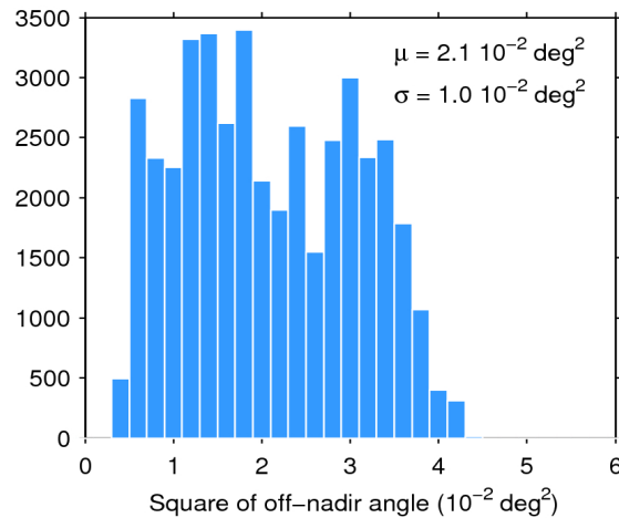
Figure 39. Histogram of flag-valid mispointing over oceans and lakes for 20/05/2016. The mean ( \mu ) and standard deviation ( \sigma ) are also shown. Note that values larger than 6 \cdot 10^{-2} \text{ deg}^2 are excluded from the histogram for the sake of readability but not from the computation of \mu and \sigma .
