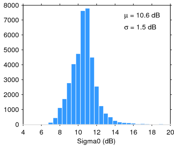
Figure 28. Histogram of science-valid sigma0 over oceans and lakes for 20/05/2016. The mean ( \mu ) and standard deviation ( \sigma ) are also shown. Note that values outside [4 20] dB are excluded from the histogram for the sake of readability but not from the computation of \mu and \sigma .
