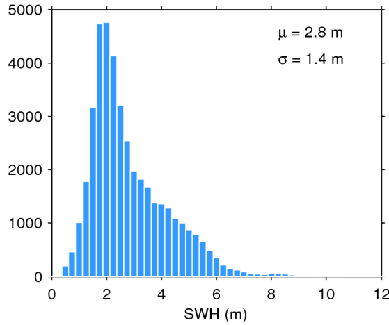
Figure 20. Histogram of science-valid SWH over oceans and lakes for 20/05/2016. The mean ( \mu ) and standard deviation ( \sigma ) are also shown. Note that values larger than 12 m are excluded from the histogram for the sake of readability but not from the computation of \mu and \sigma .
