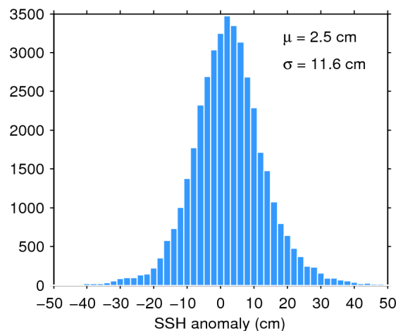
Figure 11. Histogram of science-valid SSH anomaly over oceans and lakes for 20/05/2016. The mean ( \mu ) and standard deviation ( \sigma ) are also shown. Note that values outside [-50 50] cm are excluded from the histogram for the sake of readability but not from the computation of \mu and \sigma .
