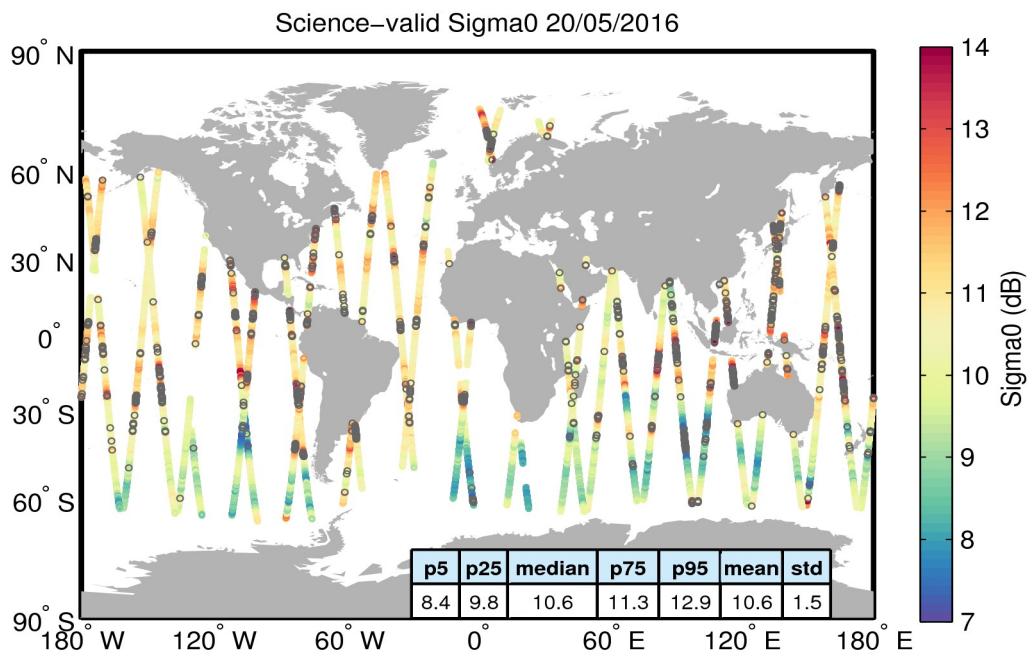
Figure 27. Geographical distribution of science-valid sigma0 data over oceans and lakes for 20/05/2016. The statistical values shown in the table refer to the sigma0 in dB and are calculated over all measurements shown in the figure. Gray circles denote records that have been rejected based on the editing criteria described in Table 4.
