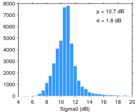
Figure 25. Histogram of flag-valid sigma0 over oceans and lakes for 20/05/2016. The mean ( \mu ) and standard deviation ( \sigma ) are also shown. Note that values outside [4 20] dB are excluded from the histogram for the sake of readability but not from the computation of \mu and \sigma .
