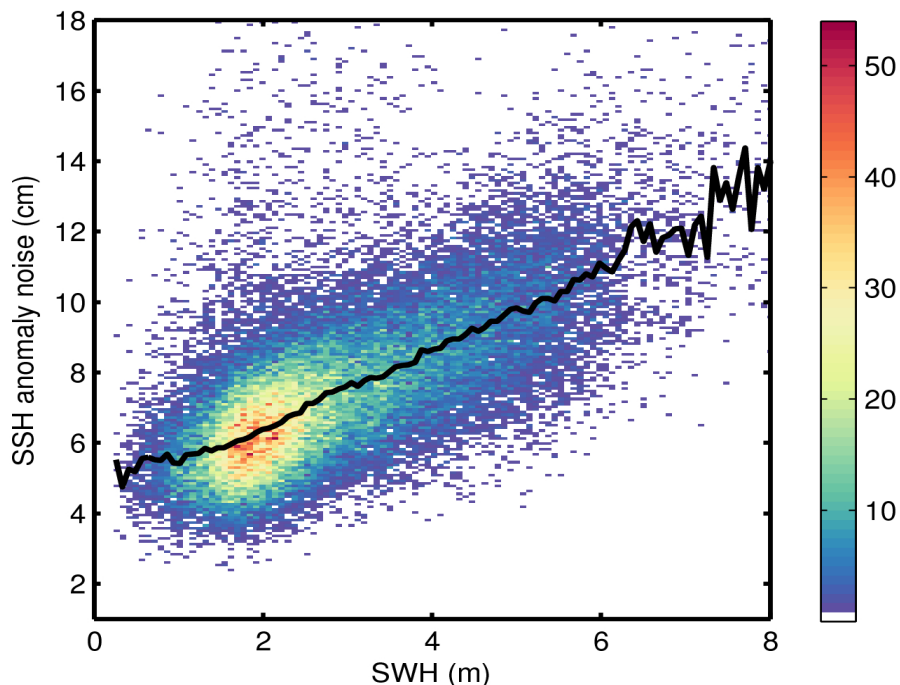
Figure 9. 2D histogram showing flag-valid SSH anomaly noise as a function of SWH for 20/05/2016. The black line denotes the median SSH anomaly noise as a function of SWH.
