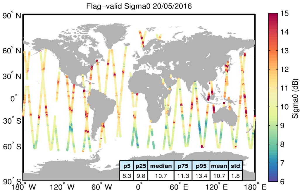
Figure 23. Geographical distribution of flag-valid sigma0 data over oceans and lakes for 20/05/2016. The statistical values shown in the table refer to the sigma0 in dB and are calculated over all measurements shown in the figure.
