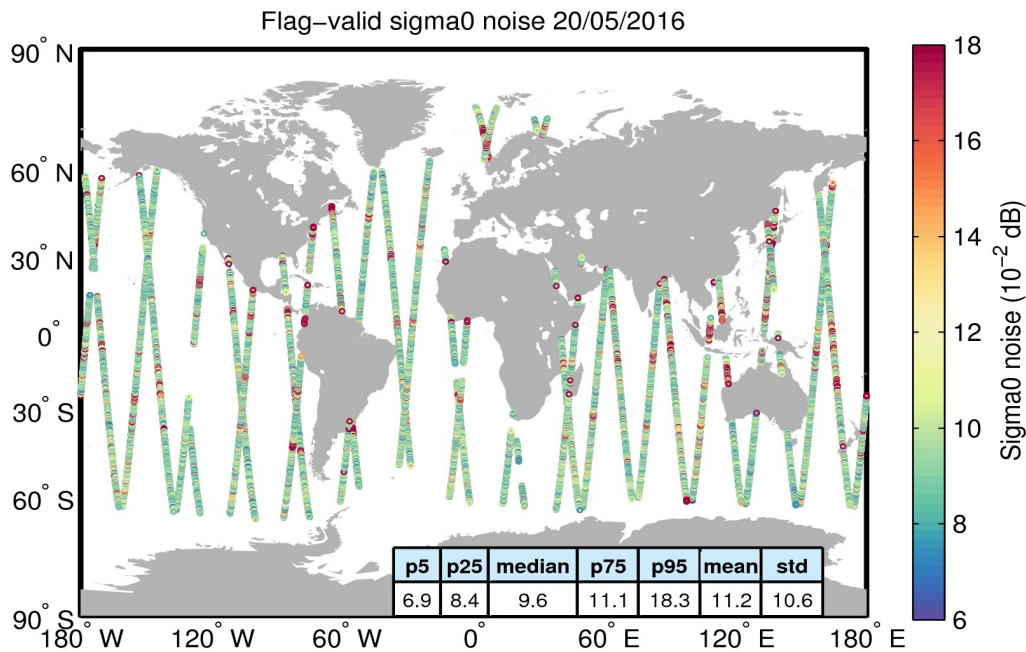
Figure 26. Geographical distribution of flag-valid 20-Hz sigma0 measurement noise over oceans and lakes for 20/05/2016. The statistical values shown in the table refer to the sigma0 noise and are calculated over all measurements shown in the figure.
