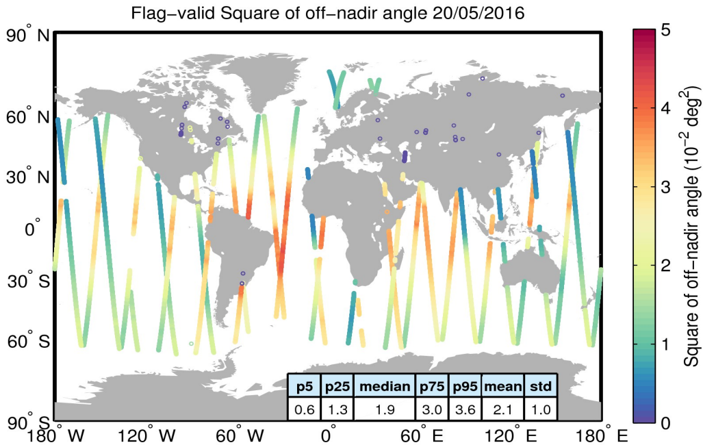
Figure 37. Geographical distribution of flag-valid mispointing data over oceans and lakes for 20/05/2016. The statistical values shown in the table refer to the mispointing in 10^{-2} deg 2 and are calculated over all measurements shown in the figure.
