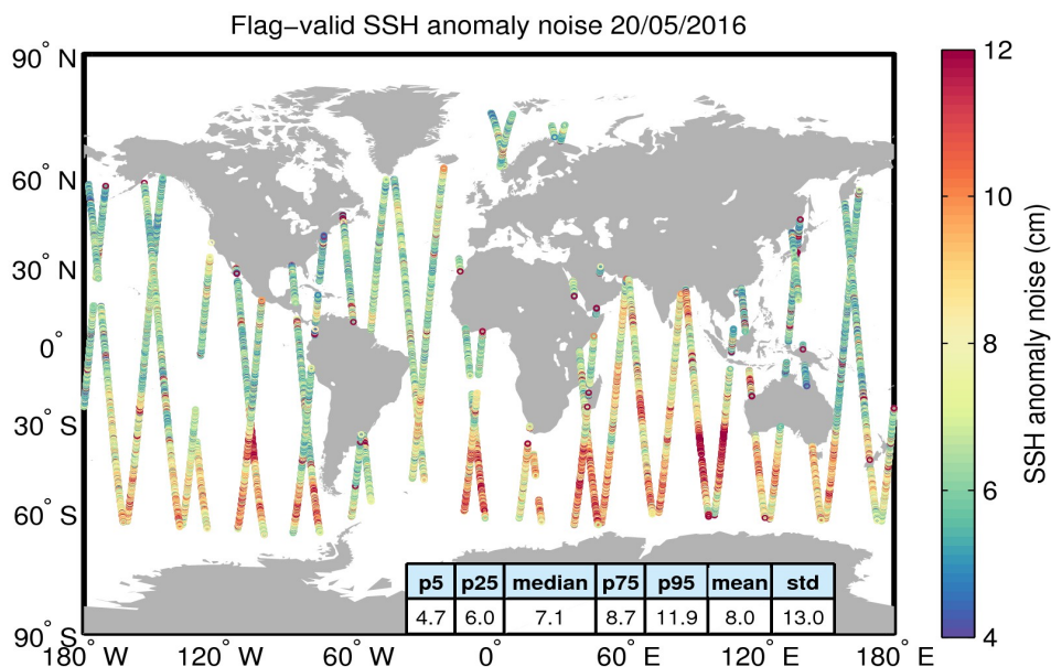
Figure 8. Geographical distribution of flag-valid 20-Hz SSH anomaly measurement noise over oceans and lakes for 20/05/2016. The statistical values shown in the table refer to the SSH anomaly noise and are calculated over all measurements shown in the figure.
