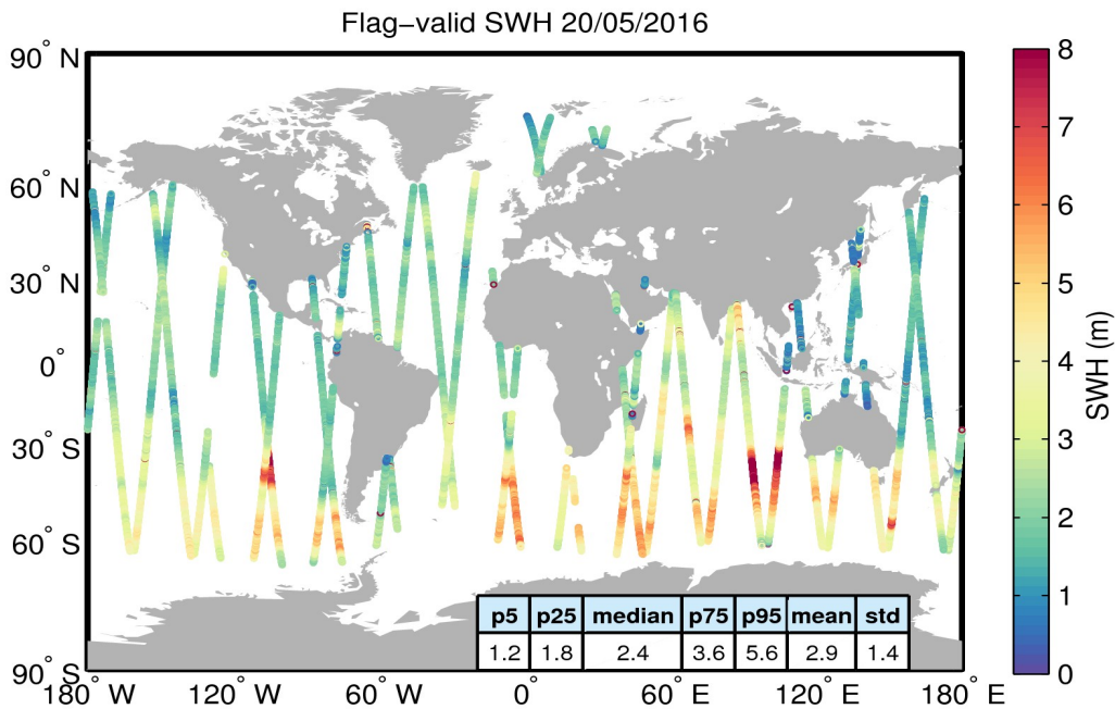
Figure 15. Geographical distribution of flag-valid SWH data over oceans and lakes for 20/05/2016. The statistical values shown in the table refer to the SWH in m and are calculated over all measurements shown in the figure.
