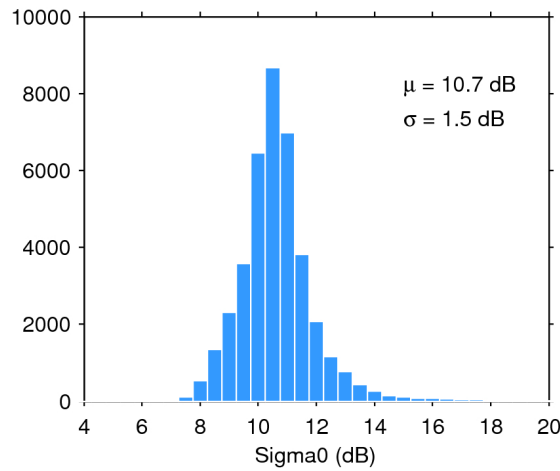
Figure 28. Histogram of science-valid sigma0 over oceans and lakes for 19/05/2016. The mean ( \mu ) and standard deviation ( \sigma ) are also shown. Note that values outside [4 20] dB are excluded from the histogram for the sake of readability but not from the computation of \mu and \sigma .
