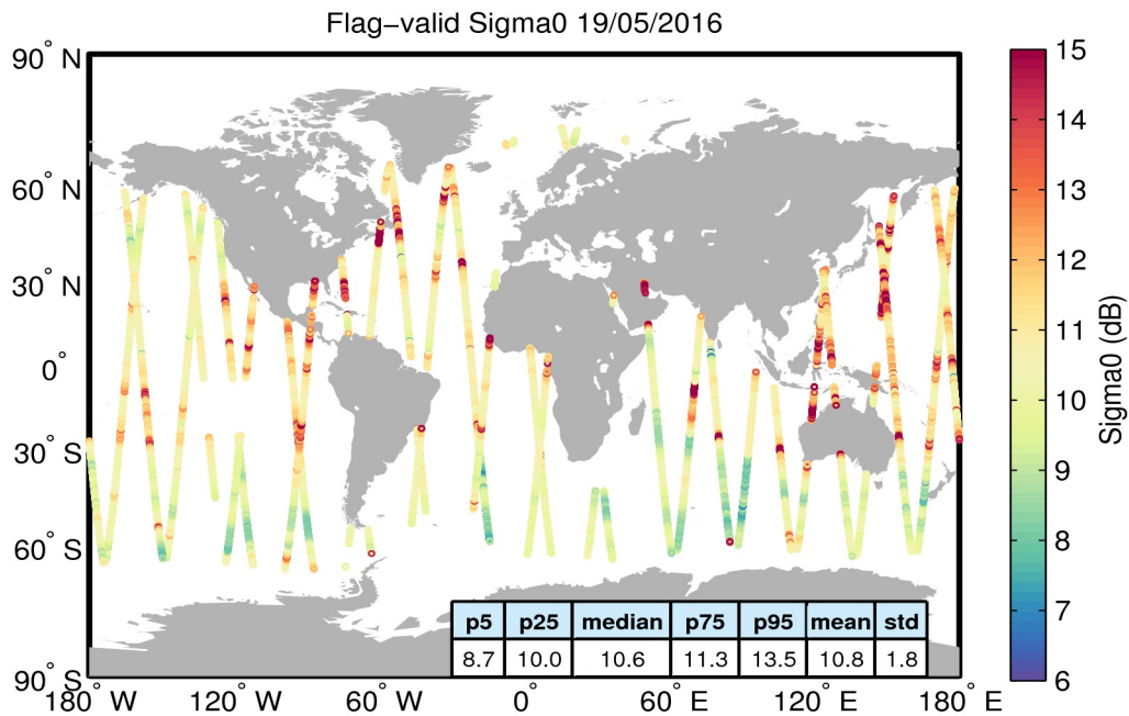
Figure 23. Geographical distribution of flag-valid sigma0 data over oceans and lakes for 19/05/2016. The statistical values shown in the table refer to the sigma0 in dB and are calculated over all measurements shown in the figure.
