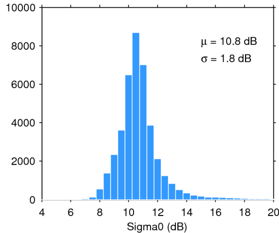
Figure 25. Histogram of flag-valid sigma0 over oceans and lakes for 19/05/2016. The mean ( \mu ) and standard deviation ( \sigma ) are also shown. Note that values outside [4 20] dB are excluded from the histogram for the sake of readability but not from the computation of \mu and \sigma .
