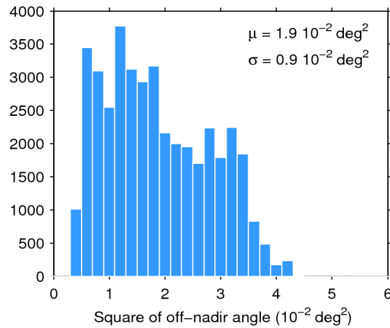
Figure 39. Histogram of flag-valid mispointing over oceans and lakes for 19/05/2016. The mean ( \mu ) and standard deviation ( \sigma ) are also shown. Note that values larger than 6 \cdot 10^{-2} \text{ deg}^2 are excluded from the histogram for the sake of readability but not from the computation of \mu and \sigma .
