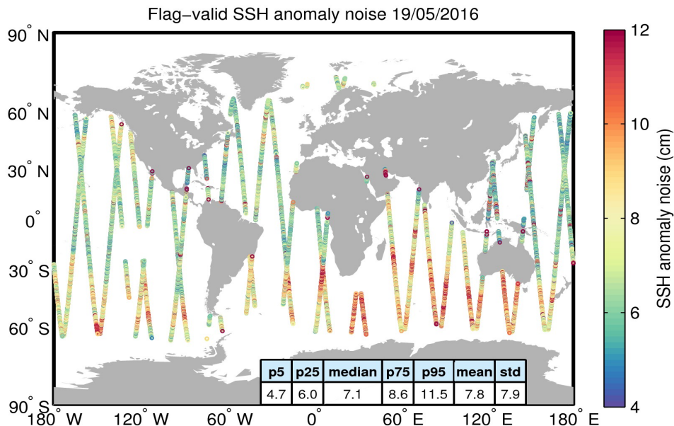
Figure 8. Geographical distribution of flag-valid 20-Hz SSH anomaly measurement noise over oceans and lakes for 19/05/2016. The statistical values shown in the table refer to the SSH anomaly noise and are calculated over all measurements shown in the figure.
