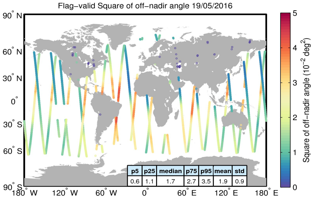
Figure 37. Geographical distribution of flag-valid mispointing data over oceans and lakes for 19/05/2016. The statistical values shown in the table refer to the mispointing in 10^{-2} \text{ deg}^2 and are calculated over all measurements shown in the figure.
