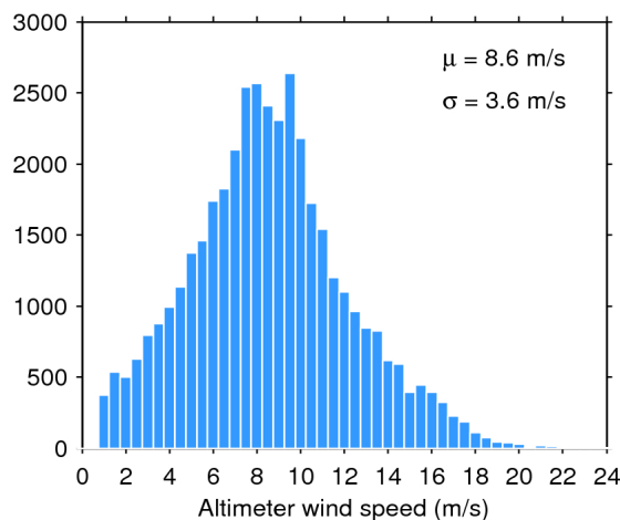
Figure 35. Histogram of science-valid wind over oceans and lakes for 19/05/2016. The mean ( \mu ) and standard deviation ( \sigma ) are also shown. Note that values larger than 24 m/s are excluded from the histogram for the sake of readability but not from the computation of \mu and \sigma .
