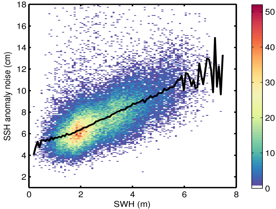
Figure 9. 2D histogram showing flag-valid SSH anomaly noise as a function of SWH for 19/05/2016. The black line denotes the median SSH anomaly noise as a function of SWH.
