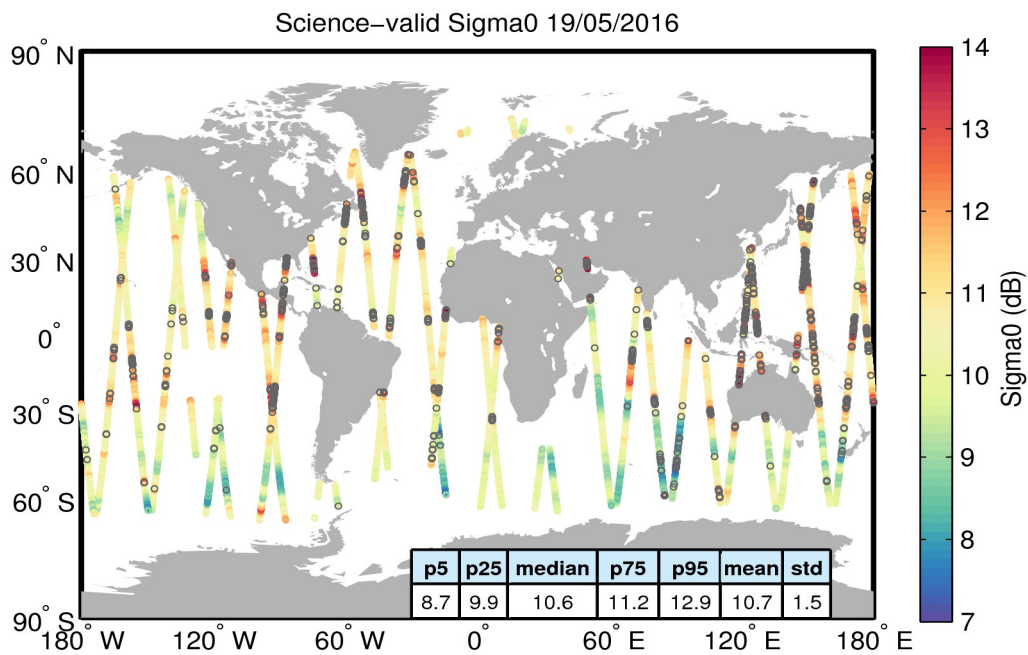
Figure 27. Geographical distribution of science-valid sigma0 data over oceans and lakes for 19/05/2016. The statistical values shown in the table refer to the sigma0 in dB and are calculated over all measurements shown in the figure. Gray circles denote records that have been rejected based on the editing criteria described in Table 4.
