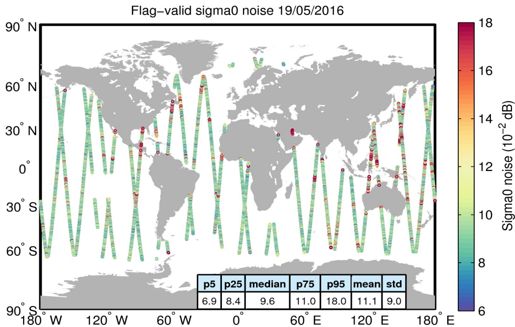
Figure 26. Geographical distribution of flag-valid 20-Hz sigma0 measurement noise over oceans and lakes for 19/05/2016. The statistical values shown in the table refer to the sigma0 noise and are calculated over all measurements shown in the figure.
