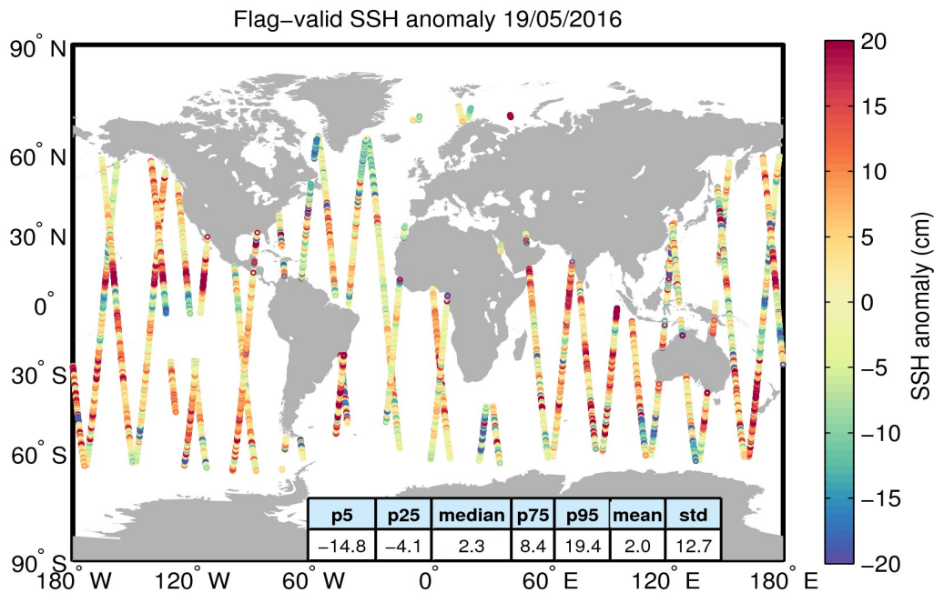
Figure 5. Geographical distribution of flag-valid 1-Hz SSH anomaly data over oceans and lakes for 19/05/2016. The statistical values shown in the table refer to the SSH anomaly in cm and are calculated over all measurements shown in the figure.
