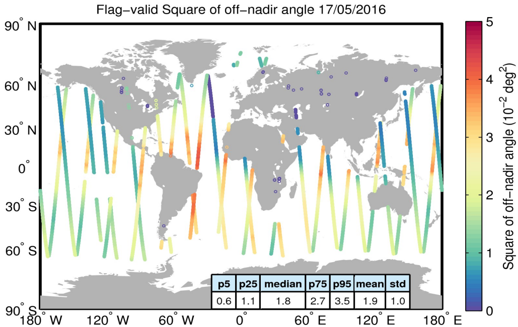
Figure 37. Geographical distribution of flag-valid mispointing data over oceans and lakes for 17/05/2016. The statistical values shown in the table refer to the mispointing in 10^{-2} \text{ deg}^2 and are calculated over all measurements shown in the figure.
