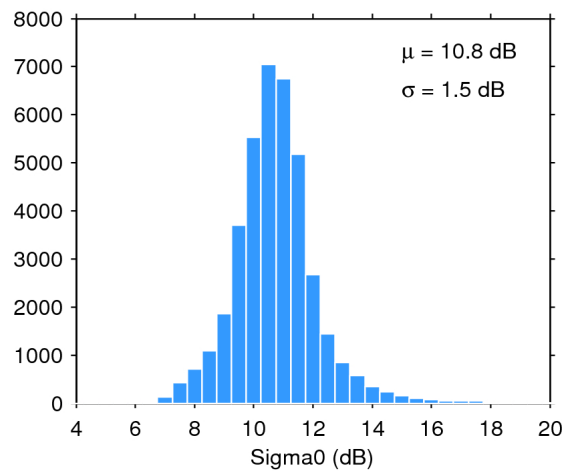
Figure 28. Histogram of science-valid sigma0 over oceans and lakes for 17/05/2016. The mean ( \mu ) and standard deviation ( \sigma ) are also shown. Note that values outside [4 20] dB are excluded from the histogram for the sake of readability but not from the computation of \mu and \sigma .
