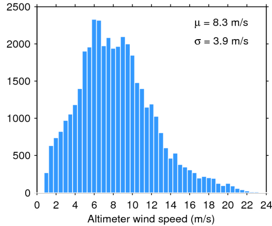
Figure 33. Histogram of flag-valid wind over oceans and lakes for 17/05/2016. The mean ( \mu ) and standard deviation ( \sigma ) are also shown. Note that values larger than 24 m/s are excluded from the histogram for the sake of readability but not from the computation of \mu and \sigma .
