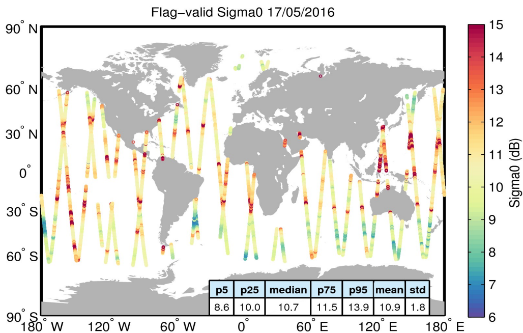
Figure 23. Geographical distribution of flag-valid sigma0 data over oceans and lakes for 17/05/2016. The statistical values shown in the table refer to the sigma0 in dB and are calculated over all measurements shown in the figure.
