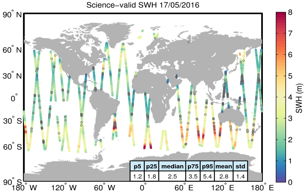
Figure 19. Geographical distribution of science-valid SWH data over oceans and lakes for 17/05/2016. The statistical values shown in the table refer to the SWH in m and are calculated over all measurements shown in the figure. Gray circles denote records that have been rejected based on the editing criteria described in Table 3.
