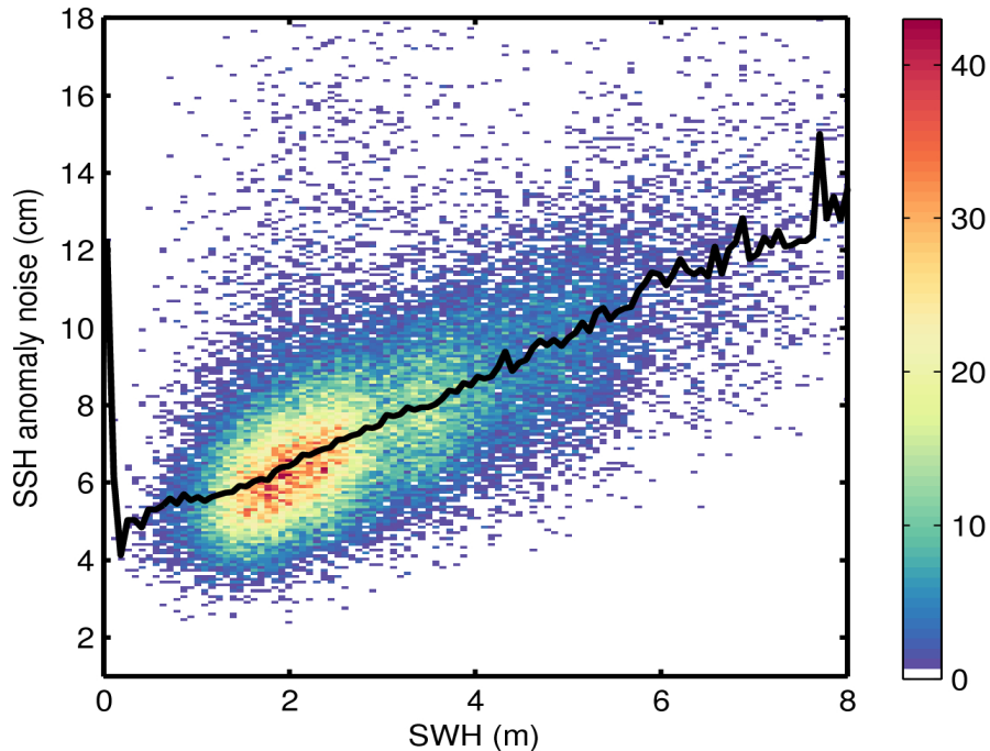
Figure 9. 2D histogram showing flag-valid SSH anomaly noise as a function of SWH for 17/05/2016. The black line denotes the median SSH anomaly noise as a function of SWH.
