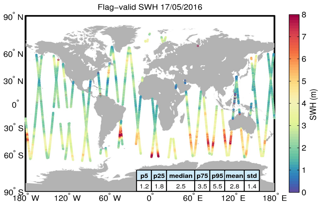
Figure 15. Geographical distribution of flag-valid SWH data over oceans and lakes for 17/05/2016. The statistical values shown in the table refer to the SWH in m and are calculated over all measurements shown in the figure.
