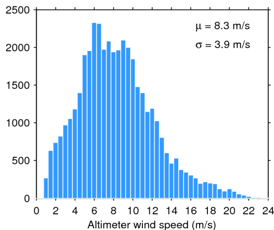
Figure 35. Histogram of science-valid wind over oceans and lakes for 17/05/2016. The mean ( \mu ) and standard deviation ( \sigma ) are also shown. Note that values larger than 24 m/s are excluded from the histogram for the sake of readability but not from the computation of \mu and \sigma .
