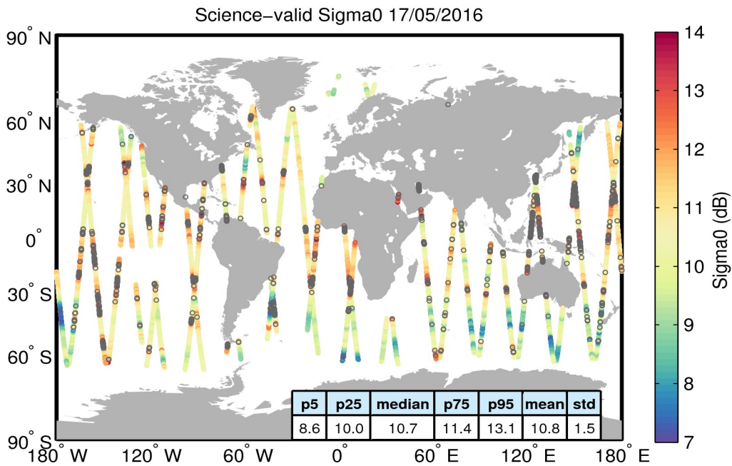
Figure 27. Geographical distribution of science-valid sigma0 data over oceans and lakes for 17/05/2016. The statistical values shown in the table refer to the sigma0 in dB and are calculated over all measurements shown in the figure. Gray circles denote records that have been rejected based on the editing criteria described in Table 4.
