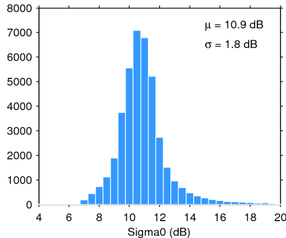
Figure 25. Histogram of flag-valid sigma0 over oceans and lakes for 17/05/2016. The mean ( \mu ) and standard deviation ( \sigma ) are also shown. Note that values outside [4 20] dB are excluded from the histogram for the sake of readability but not from the computation of \mu and \sigma .
