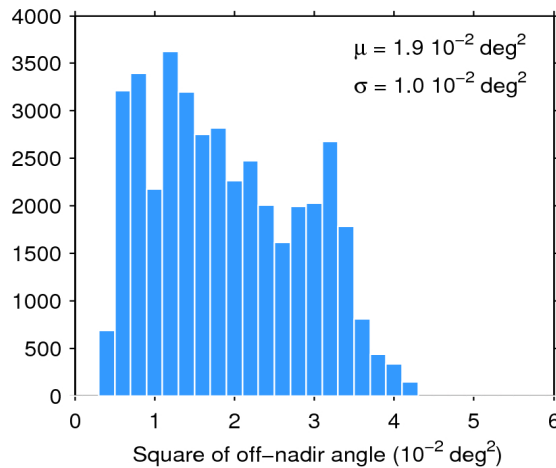
Figure 39. Histogram of flag-valid mispointing over oceans and lakes for 17/05/2016. The mean ( \mu ) and standard deviation ( \sigma ) are also shown. Note that values larger than 6 \cdot 10^{-2} \text{ deg}^2 are excluded from the histogram for the sake of readability but not from the computation of \mu and \sigma .
