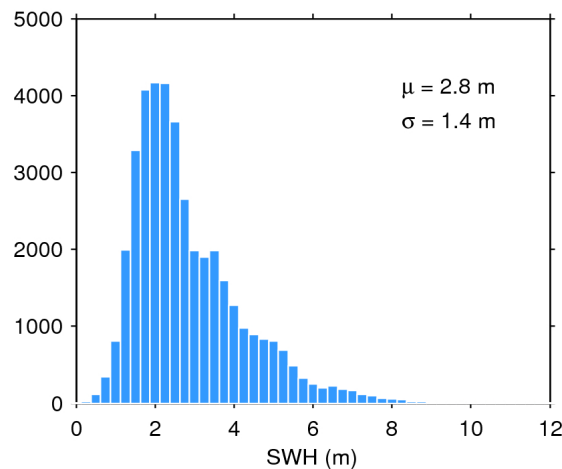
Figure 17. Histogram of flag-valid SWH over oceans and lakes for 17/05/2016. The mean ( \mu ) and standard deviation ( \sigma ) are also shown. Note that values larger than 12 m are excluded from the histogram for the sake of readability but not from the computation of \mu and \sigma .
