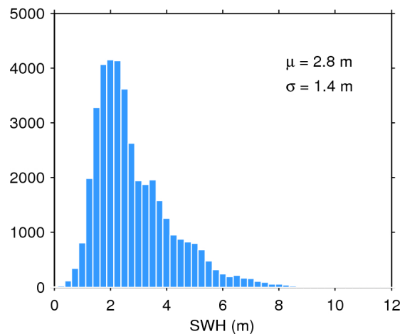
Figure 20. Histogram of science-valid SWH over oceans and lakes for 17/05/2016. The mean ( \mu ) and standard deviation ( \sigma ) are also shown. Note that values larger than 12 m are excluded from the histogram for the sake of readability but not from the computation of \mu and \sigma .
