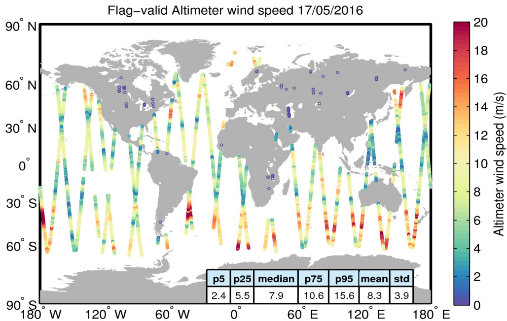
Figure 31. Geographical distribution of flag-valid wind data over oceans and lakes for 17/05/2016. The statistical values shown in the table refer to the wind in m/s and are calculated over all measurements shown in the figure.
