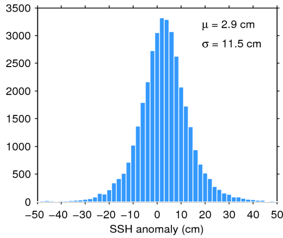
Figure 11. Histogram of science-valid SSH anomaly over oceans and lakes for 17/05/2016. The mean ( \mu ) and standard deviation ( \sigma ) are also shown. Note that values outside [-50 50] cm are excluded from the histogram for the sake of readability but not from the computation of \mu and \sigma .
