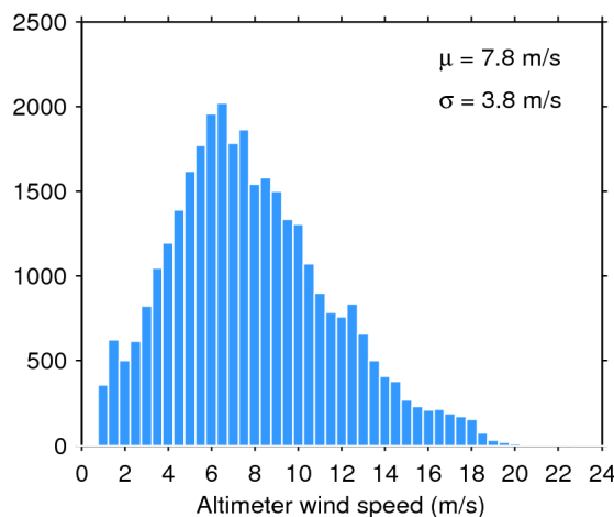
Figure 35. Histogram of science-valid wind over oceans and lakes for 16/05/2016. The mean ( \mu ) and standard deviation ( \sigma ) are also shown. Note that values larger than 24 m/s are excluded from the histogram for the sake of readability but not from the computation of \mu and \sigma .
