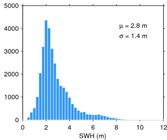
Figure 17. Histogram of flag-valid SWH over oceans and lakes for 16/05/2016. The mean ( \mu ) and standard deviation ( \sigma ) are also shown. Note that values larger than 12 m are excluded from the histogram for the sake of readability but not from the computation of \mu and \sigma .
