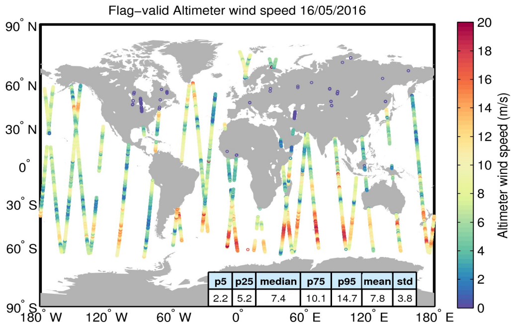
Figure 31. Geographical distribution of flag-valid wind data over oceans and lakes for 16/05/2016. The statistical values shown in the table refer to the wind in m/s and are calculated over all measurements shown in the figure.
