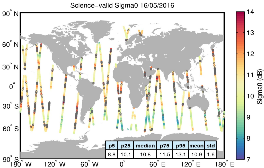
Figure 27. Geographical distribution of science-valid sigma0 data over oceans and lakes for 16/05/2016. The statistical values shown in the table refer to the sigma0 in dB and are calculated over all measurements shown in the figure. Gray circles denote records that have been rejected based on the editing criteria described in Table 4.
