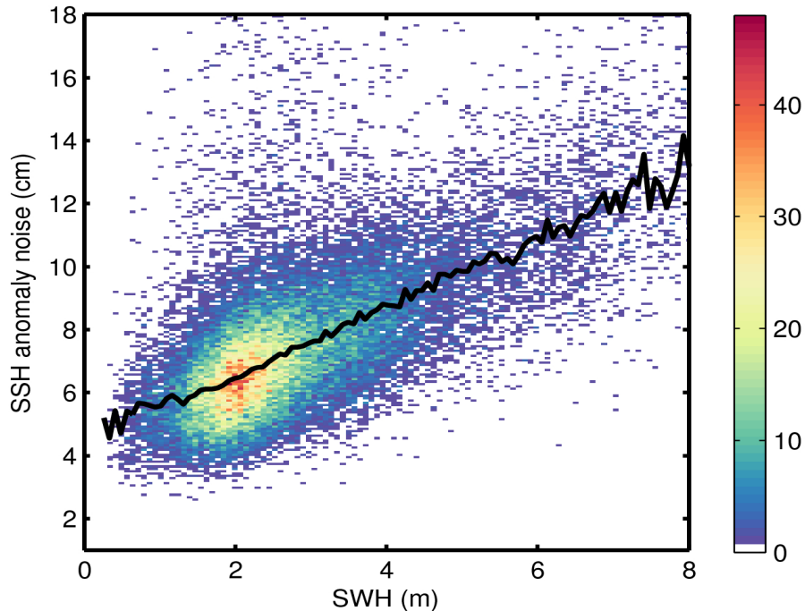
Figure 9. 2D histogram showing flag-valid SSH anomaly noise as a function of SWH for 16/05/2016. The black line denotes the median SSH anomaly noise as a function of SWH.
