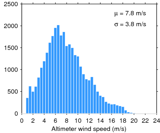
Figure 33. Histogram of flag-valid wind over oceans and lakes for 16/05/2016. The mean ( \mu ) and standard deviation ( \sigma ) are also shown. Note that values larger than 24 m/s are excluded from the histogram for the sake of readability but not from the computation of \mu and \sigma .
