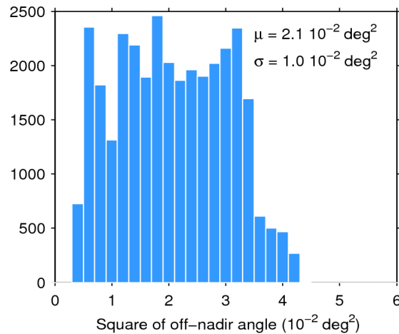
Figure 39. Histogram of flag-valid mispointing over oceans and lakes for 16/05/2016. The mean ( \mu ) and standard deviation ( \sigma ) are also shown. Note that values larger than 6 \cdot 10^{-2} \text{ deg}^2 are excluded from the histogram for the sake of readability but not from the computation of \mu and \sigma .
