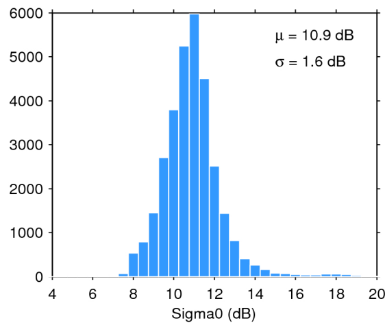
Figure 28. Histogram of science-valid sigma0 over oceans and lakes for 16/05/2016. The mean ( \mu ) and standard deviation ( \sigma ) are also shown. Note that values outside [4 20] dB are excluded from the histogram for the sake of readability but not from the computation of \mu and \sigma .
