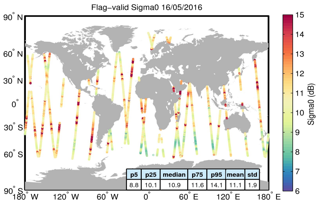
Figure 23. Geographical distribution of flag-valid sigma0 data over oceans and lakes for 16/05/2016. The statistical values shown in the table refer to the sigma0 in dB and are calculated over all measurements shown in the figure.
