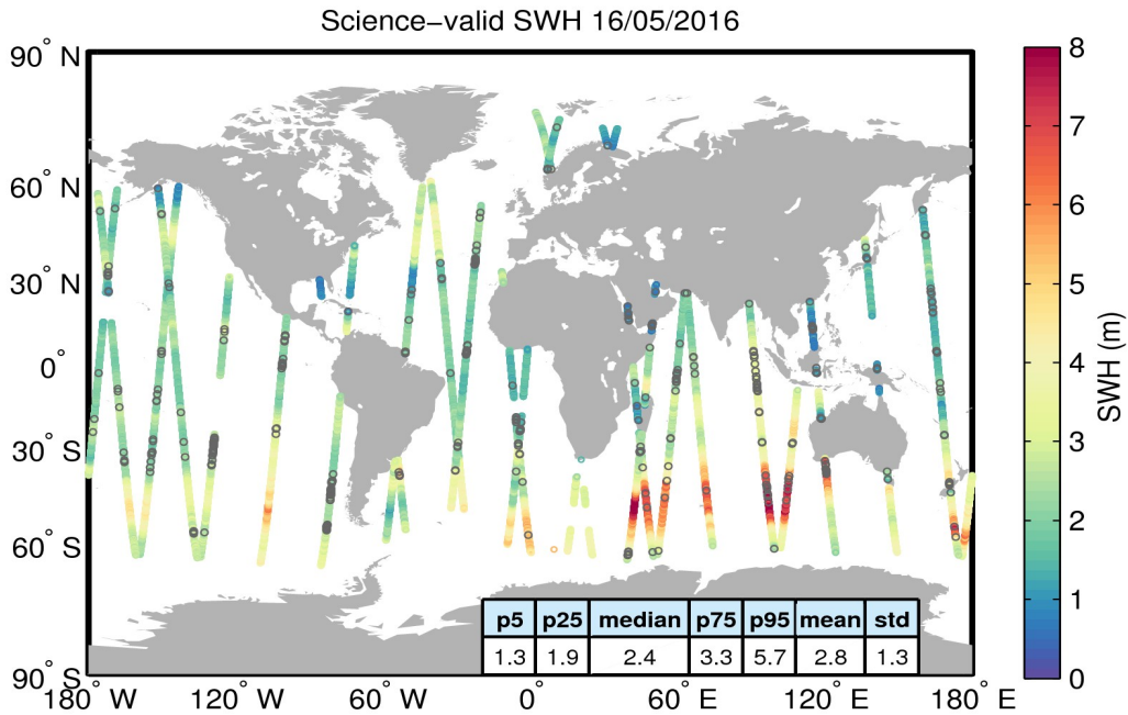
Figure 19. Geographical distribution of science-valid SWH data over oceans and lakes for 16/05/2016. The statistical values shown in the table refer to the SWH in m and are calculated over all measurements shown in the figure. Gray circles denote records that have been rejected based on the editing criteria described in Table 3.
