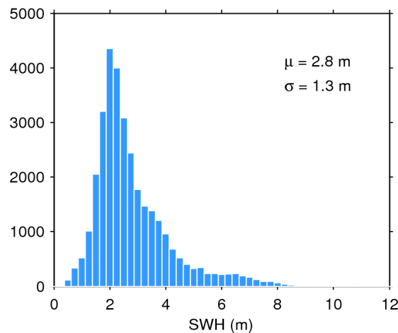
Figure 20. Histogram of science-valid SWH over oceans and lakes for 16/05/2016. The mean ( \mu ) and standard deviation ( \sigma ) are also shown. Note that values larger than 12 m are excluded from the histogram for the sake of readability but not from the computation of \mu and \sigma .
