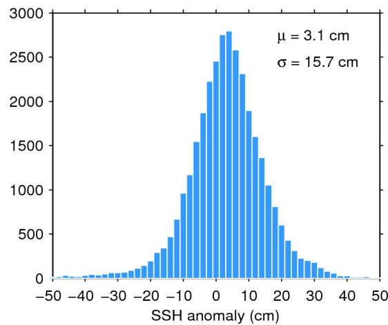
Figure 7. Histogram of flag-valid SSH anomaly over oceans and lakes for 16/05/2016. The mean ( \mu ) and standard deviation ( \sigma ) are also shown. Note that values outside [-50\ 50] cm are excluded from the histogram for the sake of readability but not from the computation of \mu and \sigma .
