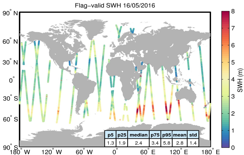
Figure 15. Geographical distribution of flag-valid SWH data over oceans and lakes for 16/05/2016. The statistical values shown in the table refer to the SWH in m and are calculated over all measurements shown in the figure.
