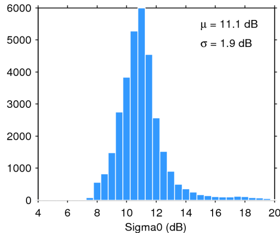
Figure 25. Histogram of flag-valid sigma0 over oceans and lakes for 16/05/2016. The mean ( \mu ) and standard deviation ( \sigma ) are also shown. Note that values outside [4 20] dB are excluded from the histogram for the sake of readability but not from the computation of \mu and \sigma .
