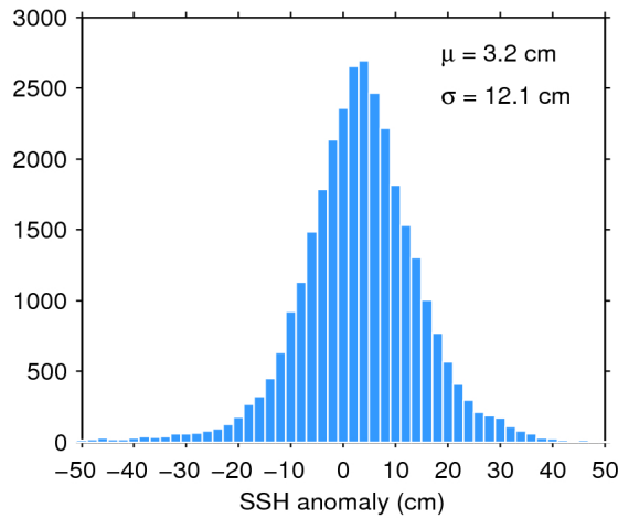
Figure 11. Histogram of science-valid SSH anomaly over oceans and lakes for 16/05/2016. The mean ( \mu ) and standard deviation ( \sigma ) are also shown. Note that values outside [-50 50] cm are excluded from the histogram for the sake of readability but not from the computation of \mu and \sigma .
