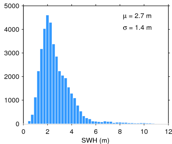
Figure 20. Histogram of science-valid SWH over oceans and lakes for 15/05/2016. The mean ( \mu ) and standard deviation ( \sigma ) are also shown. Note that values larger than 12 m are excluded from the histogram for the sake of readability but not from the computation of \mu and \sigma .
