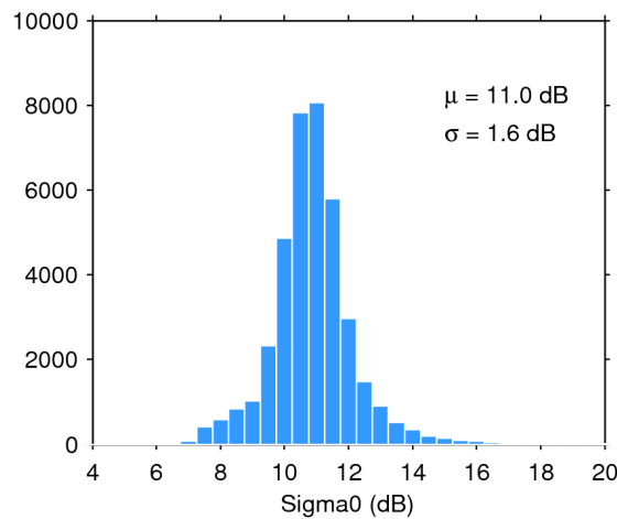
Figure 28. Histogram of science-valid sigma0 over oceans and lakes for 15/05/2016. The mean ( \mu ) and standard deviation ( \sigma ) are also shown. Note that values outside [4 20] dB are excluded from the histogram for the sake of readability but not from the computation of \mu and \sigma .
