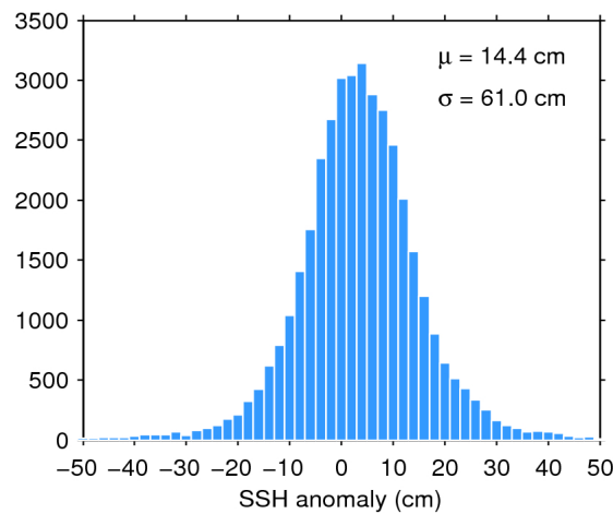
Figure 7. Histogram of flag-valid SSH anomaly over oceans and lakes for 15/05/2016. The mean ( \mu ) and standard deviation ( \sigma ) are also shown. Note that values outside [-50 50] cm are excluded from the histogram for the sake of readability but not from the computation of \mu and \sigma .
