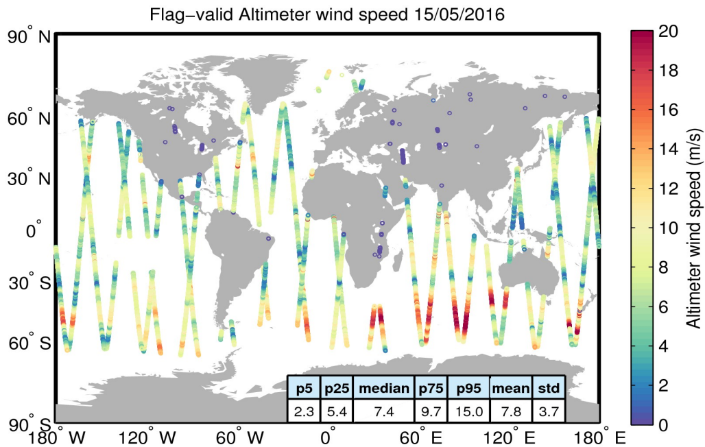
Figure 31. Geographical distribution of flag-valid wind data over oceans and lakes for 15/05/2016. The statistical values shown in the table refer to the wind in m/s and are calculated over all measurements shown in the figure.
