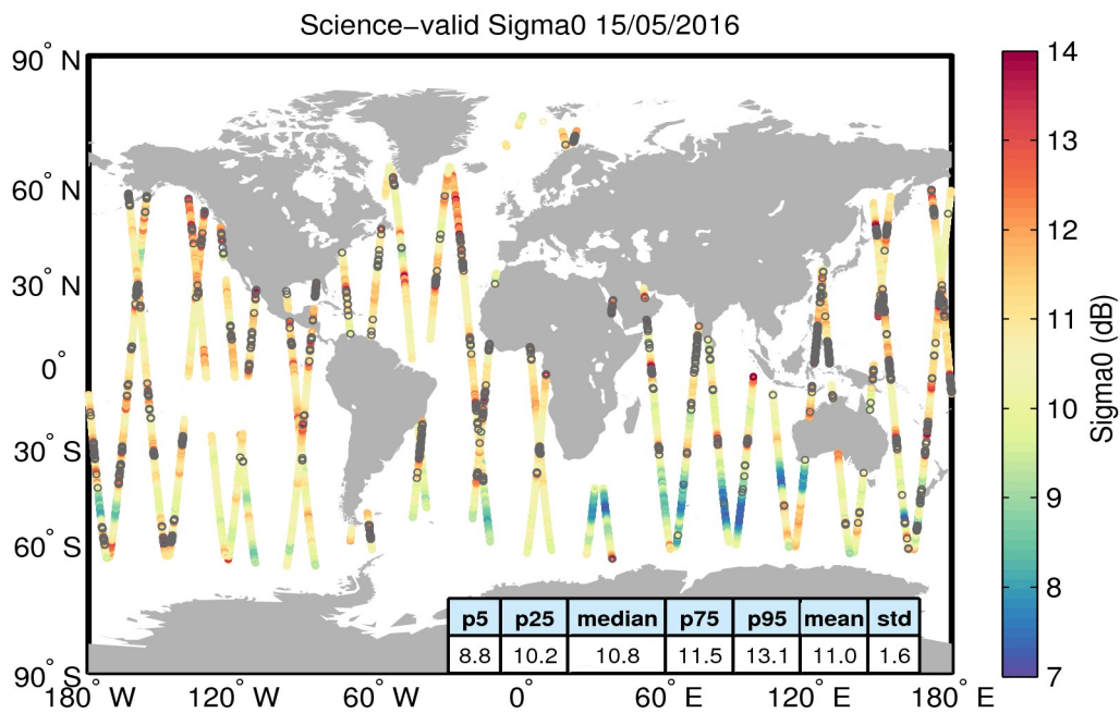
Figure 27. Geographical distribution of science-valid sigma0 data over oceans and lakes for 15/05/2016. The statistical values shown in the table refer to the sigma0 in dB and are calculated over all measurements shown in the figure. Gray circles denote records that have been rejected based on the editing criteria described in Table 4.
