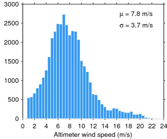
Figure 33. Histogram of flag-valid wind over oceans and lakes for 15/05/2016. The mean ( \mu ) and standard deviation ( \sigma ) are also shown. Note that values larger than 24 m/s are excluded from the histogram for the sake of readability but not from the computation of \mu and \sigma .
