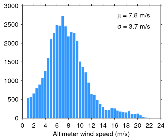
Figure 35. Histogram of science-valid wind over oceans and lakes for 15/05/2016. The mean ( \mu ) and standard deviation ( \sigma ) are also shown. Note that values larger than 24 m/s are excluded from the histogram for the sake of readability but not from the computation of \mu and \sigma .
