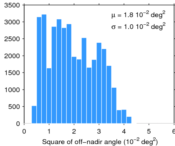
Figure 39. Histogram of flag-valid mispointing over oceans and lakes for 15/05/2016. The mean ( \mu ) and standard deviation ( \sigma ) are also shown. Note that values larger than 6 \cdot 10^{-2} \text{ deg}^2 are excluded from the histogram for the sake of readability but not from the computation of \mu and \sigma .
