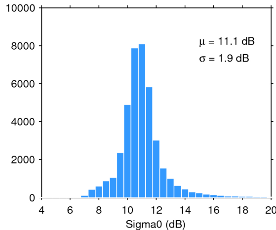
Figure 25. Histogram of flag-valid sigma0 over oceans and lakes for 15/05/2016. The mean ( \mu ) and standard deviation ( \sigma ) are also shown. Note that values outside [4 20] dB are excluded from the histogram for the sake of readability but not from the computation of \mu and \sigma .
