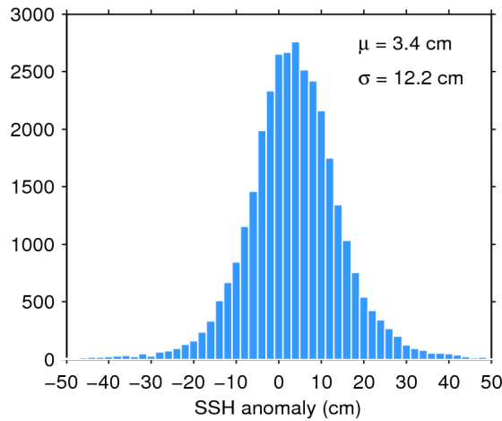
Figure 11. Histogram of science-valid SSH anomaly over oceans and lakes for 15/05/2016. The mean ( \mu ) and standard deviation ( \sigma ) are also shown. Note that values outside [-50 50] cm are excluded from the histogram for the sake of readability but not from the computation of \mu and \sigma .
