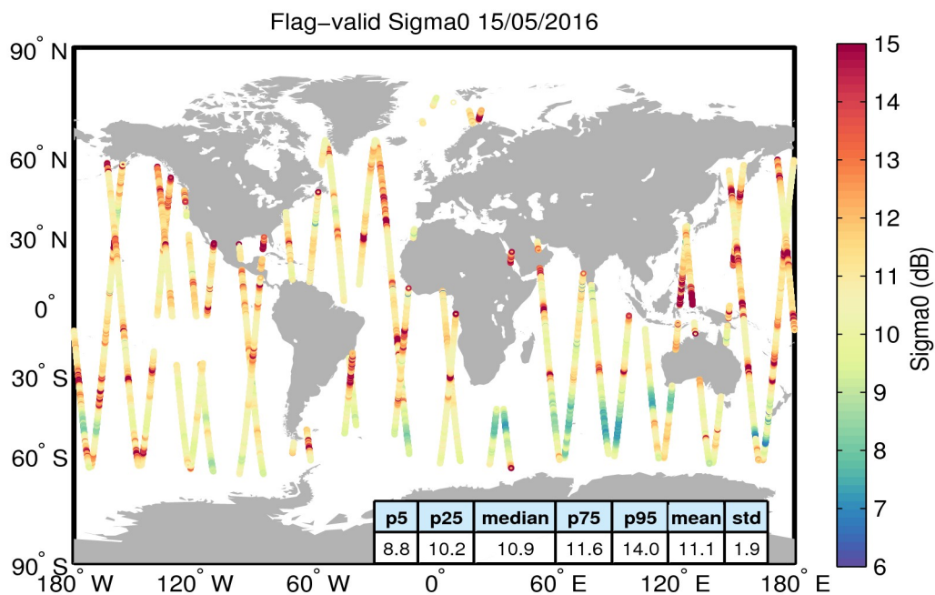
Figure 23. Geographical distribution of flag-valid sigma0 data over oceans and lakes for 15/05/2016. The statistical values shown in the table refer to the sigma0 in dB and are calculated over all measurements shown in the figure.
