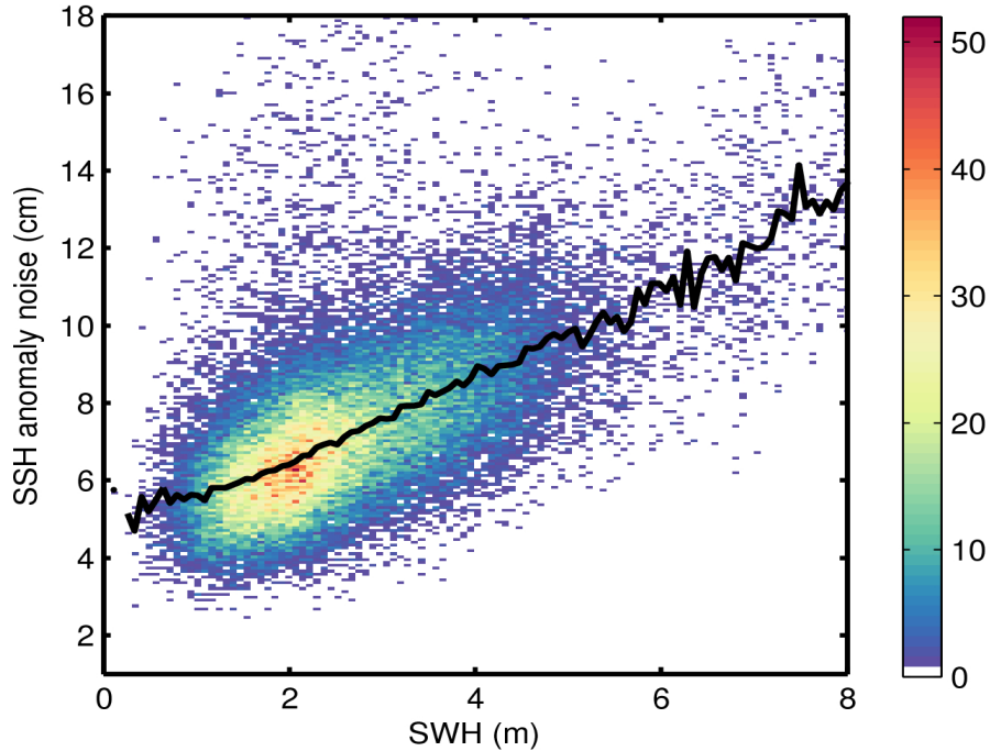
Figure 9. 2D histogram showing flag-valid SSH anomaly noise as a function of SWH for 15/05/2016. The black line denotes the median SSH anomaly noise as a function of SWH.
