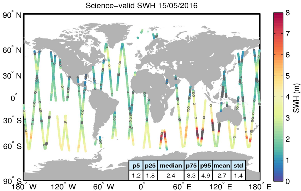
Figure 19. Geographical distribution of science-valid SWH data over oceans and lakes for 15/05/2016. The statistical values shown in the table refer to the SWH in m and are calculated over all measurements shown in the figure. Gray circles denote records that have been rejected based on the editing criteria described in Table 3.
