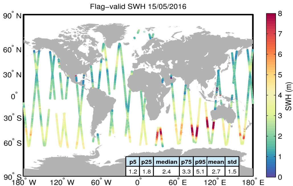
Figure 15. Geographical distribution of flag-valid SWH data over oceans and lakes for 15/05/2016. The statistical values shown in the table refer to the SWH in m and are calculated over all measurements shown in the figure.
