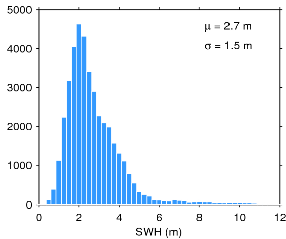
Figure 17. Histogram of flag-valid SWH over oceans and lakes for 15/05/2016. The mean ( \mu ) and standard deviation ( \sigma ) are also shown. Note that values larger than 12 m are excluded from the histogram for the sake of readability but not from the computation of \mu and \sigma .
