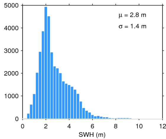
Figure 17. Histogram of flag-valid SWH over oceans and lakes for 14/05/2016. The mean ( \mu ) and standard deviation ( \sigma ) are also shown. Note that values larger than 12 m are excluded from the histogram for the sake of readability but not from the computation of \mu and \sigma .
