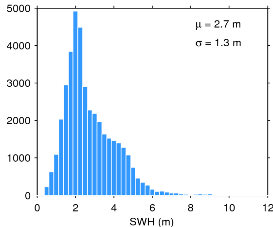
Figure 20. Histogram of science-valid SWH over oceans and lakes for 14/05/2016. The mean ( \mu ) and standard deviation ( \sigma ) are also shown. Note that values larger than 12 m are excluded from the histogram for the sake of readability but not from the computation of \mu and \sigma .
