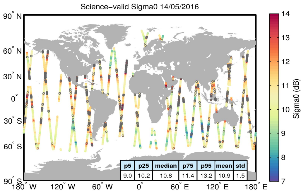
Figure 27. Geographical distribution of science-valid sigma0 data over oceans and lakes for 14/05/2016. The statistical values shown in the table refer to the sigma0 in dB and are calculated over all measurements shown in the figure. Gray circles denote records that have been rejected based on the editing criteria described in Table 4.
