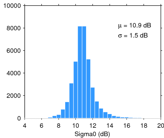
Figure 28. Histogram of science-valid sigma0 over oceans and lakes for 14/05/2016. The mean ( \mu ) and standard deviation ( \sigma ) are also shown. Note that values outside [4 20] dB are excluded from the histogram for the sake of readability but not from the computation of \mu and \sigma .
