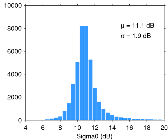
Figure 25. Histogram of flag-valid sigma0 over oceans and lakes for 14/05/2016. The mean ( \mu ) and standard deviation ( \sigma ) are also shown. Note that values outside [4 20] dB are excluded from the histogram for the sake of readability but not from the computation of \mu and \sigma .
