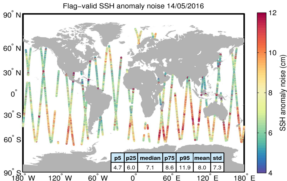
Figure 8. Geographical distribution of flag-valid 20-Hz SSH anomaly measurement noise over oceans and lakes for 14/05/2016. The statistical values shown in the table refer to the SSH anomaly noise and are calculated over all measurements shown in the figure.
