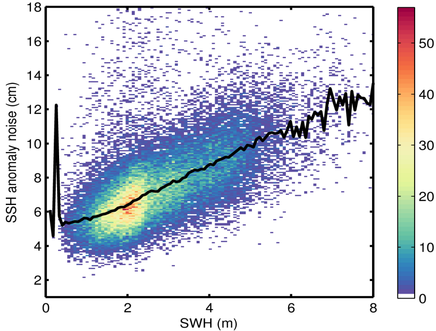
Figure 9. 2D histogram showing flag-valid SSH anomaly noise as a function of SWH for 14/05/2016. The black line denotes the median SSH anomaly noise as a function of SWH.
