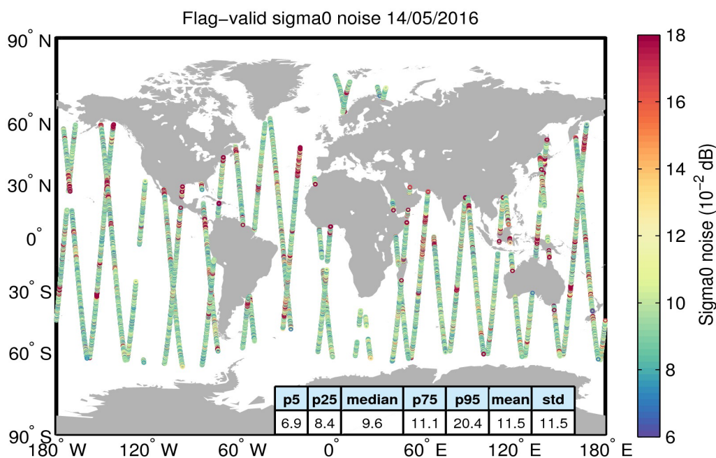
Figure 26. Geographical distribution of flag-valid 20-Hz sigma0 measurement noise over oceans and lakes for 14/05/2016. The statistical values shown in the table refer to the sigma0 noise and are calculated over all measurements shown in the figure.
