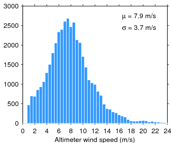
Figure 35. Histogram of science-valid wind over oceans and lakes for 14/05/2016. The mean ( \mu ) and standard deviation ( \sigma ) are also shown. Note that values larger than 24 m/s are excluded from the histogram for the sake of readability but not from the computation of \mu and \sigma .
