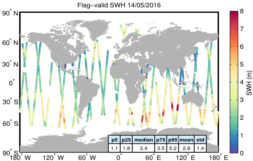
Figure 15. Geographical distribution of flag-valid SWH data over oceans and lakes for 14/05/2016. The statistical values shown in the table refer to the SWH in m and are calculated over all measurements shown in the figure.
