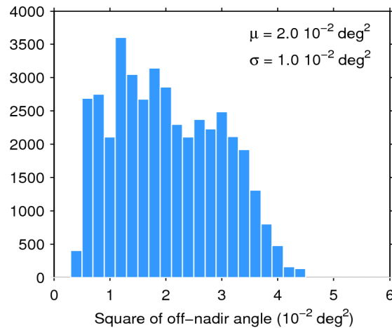
Figure 39. Histogram of flag-valid mispointing over oceans and lakes for 14/05/2016. The mean ( \mu ) and standard deviation ( \sigma ) are also shown. Note that values larger than 6 \cdot 10^{-2} \text{ deg}^2 are excluded from the histogram for the sake of readability but not from the computation of \mu and \sigma .
