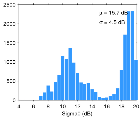
Figure 28. Histogram of science-valid sigma0 over oceans and lakes for 13/05/2016. The mean ( \mu ) and standard deviation ( \sigma ) are also shown. Note that values outside [4 20] dB are excluded from the histogram for the sake of readability but not from the computation of \mu and \sigma .
