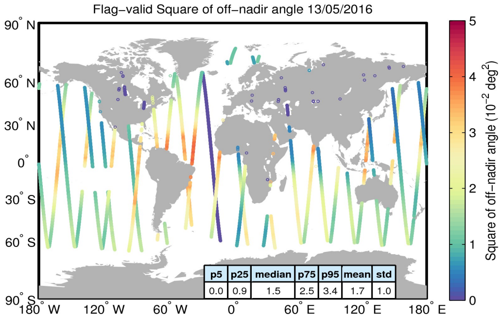
Figure 37. Geographical distribution of flag-valid mispointing data over oceans and lakes for 13/05/2016. The statistical values shown in the table refer to the mispointing in 10^{-2} deg 2 and are calculated over all measurements shown in the figure.
