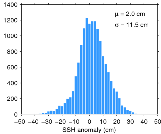
Figure 11. Histogram of science-valid SSH anomaly over oceans and lakes for 13/05/2016. The mean ( \mu ) and standard deviation ( \sigma ) are also shown. Note that values outside [-50 50] cm are excluded from the histogram for the sake of readability but not from the computation of \mu and \sigma .
