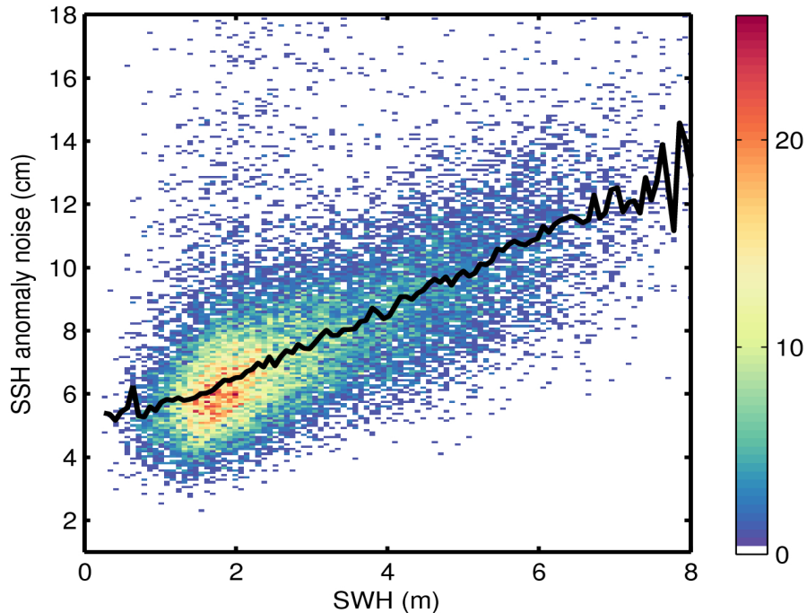
Figure 9. 2D histogram showing flag-valid SSH anomaly noise as a function of SWH for 13/05/2016. The black line denotes the median SSH anomaly noise as a function of SWH.
