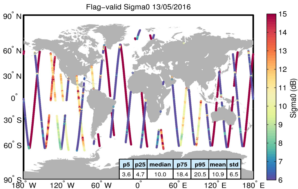
Figure 23. Geographical distribution of flag-valid sigma0 data over oceans and lakes for 13/05/2016. The statistical values shown in the table refer to the sigma0 in dB and are calculated over all measurements shown in the figure.
