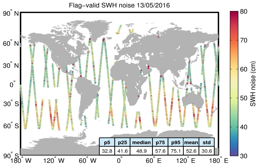
Figure 18. Geographical distribution of flag-valid 20-Hz SWH measurement noise over oceans and lakes for 13/05/2016. The statistical values shown in the table refer to the SWH noise and are calculated over all measurements shown in the figure.
