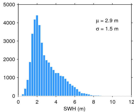
Figure 17. Histogram of flag-valid SWH over oceans and lakes for 13/05/2016. The mean ( \mu ) and standard deviation ( \sigma ) are also shown. Note that values larger than 12 m are excluded from the histogram for the sake of readability but not from the computation of \mu and \sigma .
