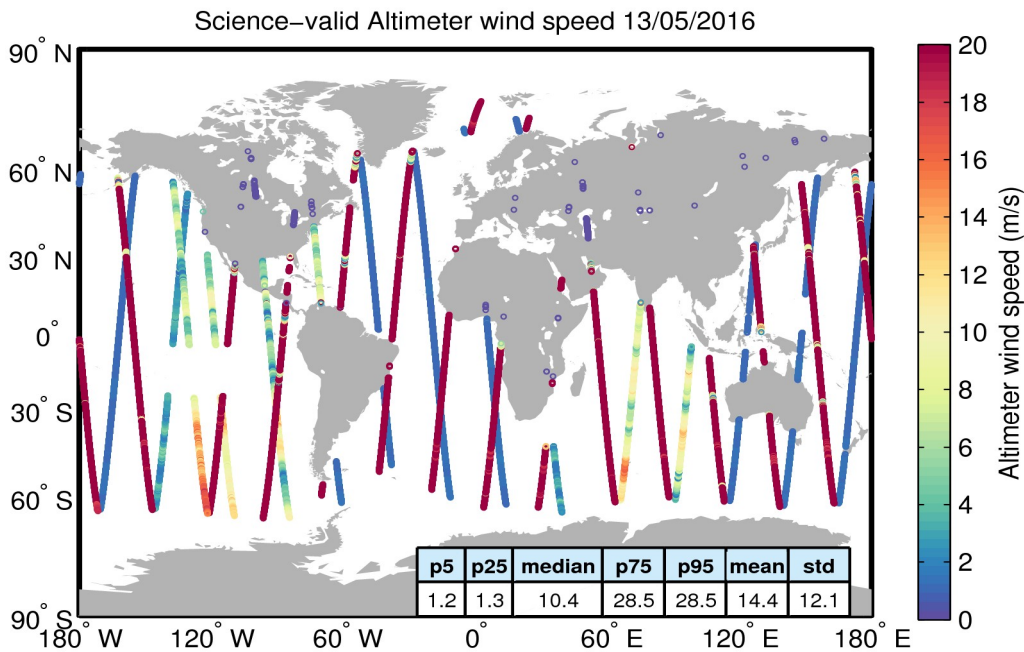
Figure 34. Geographical distribution of science-valid wind data over oceans and lakes for 13/05/2016. The statistical values shown in the table refer to the wind in m/s and are calculated over all measurements shown in the figure. Gray circles denote records that have been rejected based on the editing criteria described in Table 5.
