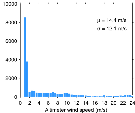
Figure 33. Histogram of flag-valid wind over oceans and lakes for 13/05/2016. The mean ( \mu ) and standard deviation ( \sigma ) are also shown. Note that values larger than 24 m/s are excluded from the histogram for the sake of readability but not from the computation of \mu and \sigma .
