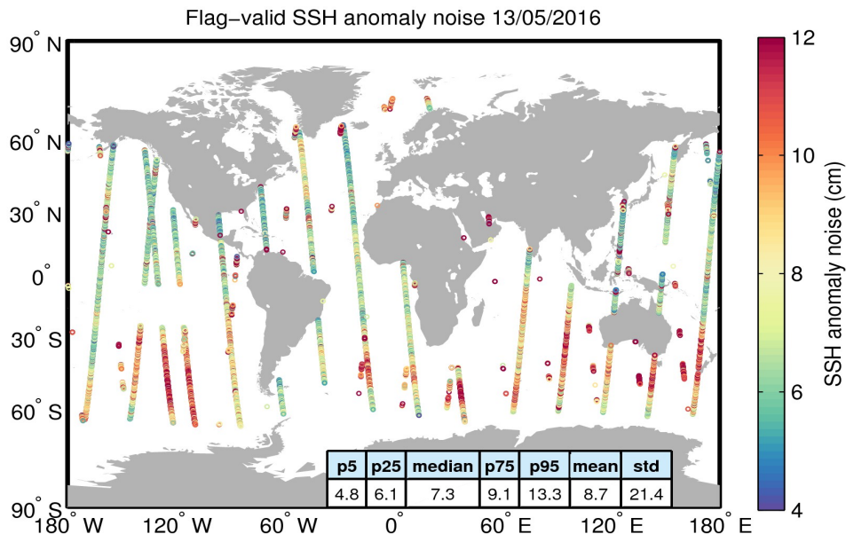
Figure 8. Geographical distribution of flag-valid 20-Hz SSH anomaly measurement noise over oceans and lakes for 13/05/2016. The statistical values shown in the table refer to the SSH anomaly noise and are calculated over all measurements shown in the figure.
