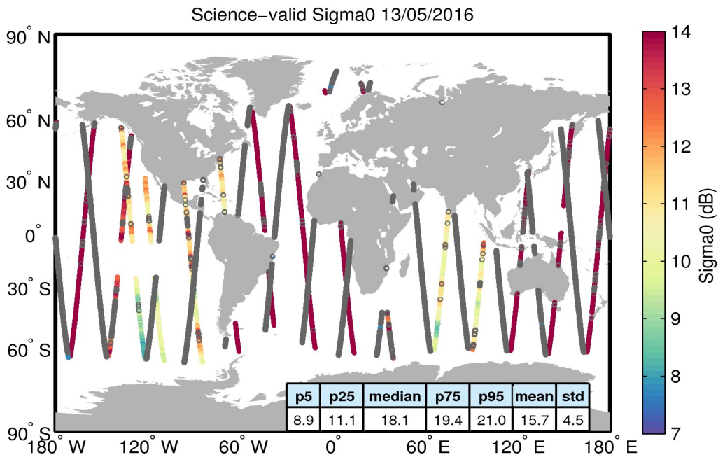
Figure 27. Geographical distribution of science-valid sigma0 data over oceans and lakes for 13/05/2016. The statistical values shown in the table refer to the sigma0 in dB and are calculated over all measurements shown in the figure. Gray circles denote records that have been rejected based on the editing criteria described in Table 4.
