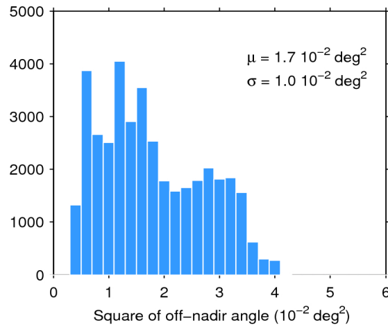
Figure 39. Histogram of flag-valid mispointing over oceans and lakes for 13/05/2016. The mean ( \mu ) and standard deviation ( \sigma ) are also shown. Note that values larger than 6 \cdot 10^{-2} \text{ deg}^2 are excluded from the histogram for the sake of readability but not from the computation of \mu and \sigma .
