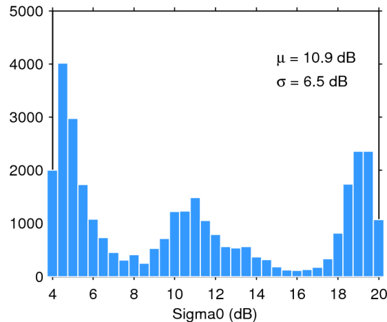
Figure 25. Histogram of flag-valid sigma0 over oceans and lakes for 13/05/2016. The mean ( \mu ) and standard deviation ( \sigma ) are also shown. Note that values outside [4 20] dB are excluded from the histogram for the sake of readability but not from the computation of \mu and \sigma .
