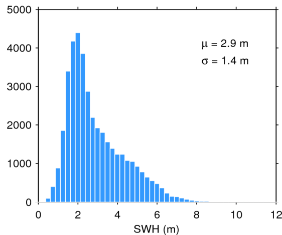
Figure 20. Histogram of science-valid SWH over oceans and lakes for 13/05/2016. The mean ( \mu ) and standard deviation ( \sigma ) are also shown. Note that values larger than 12 m are excluded from the histogram for the sake of readability but not from the computation of \mu and \sigma .
