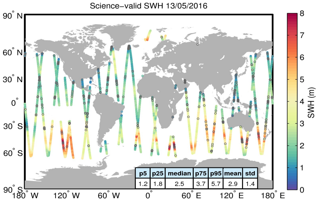
Figure 19. Geographical distribution of science-valid SWH data over oceans and lakes for 13/05/2016. The statistical values shown in the table refer to the SWH in m and are calculated over all measurements shown in the figure. Gray circles denote records that have been rejected based on the editing criteria described in Table 3.
