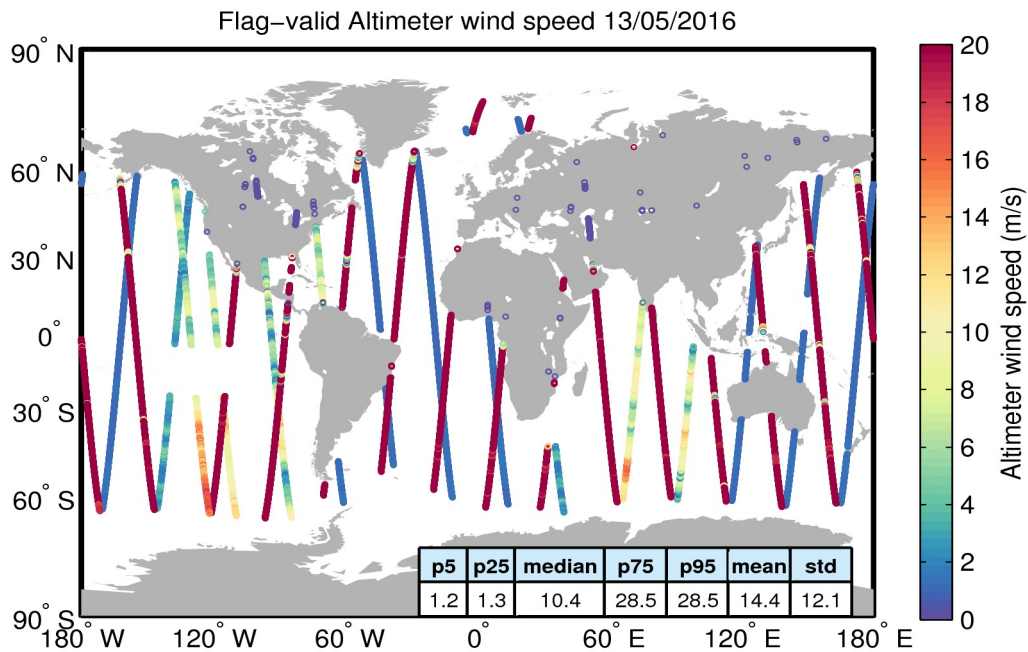
Figure 31. Geographical distribution of flag-valid wind data over oceans and lakes for 13/05/2016. The statistical values shown in the table refer to the wind in m/s and are calculated over all measurements shown in the figure.
