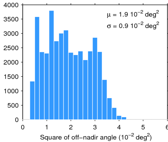
Figure 39. Histogram of flag-valid mispointing over oceans and lakes for 12/05/2016. The mean ( \mu ) and standard deviation ( \sigma ) are also shown. Note that values larger than 6 \cdot 10^{-2} \text{ deg}^2 are excluded from the histogram for the sake of readability but not from the computation of \mu and \sigma .
