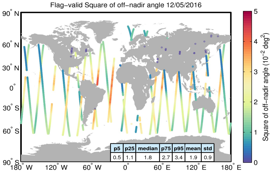
Figure 37. Geographical distribution of flag-valid mispointing data over oceans and lakes for 12/05/2016. The statistical values shown in the table refer to the mispointing in 10^{-2} deg 2 and are calculated over all measurements shown in the figure.
