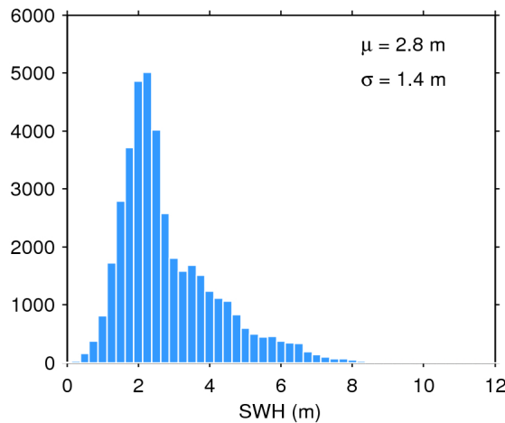
Figure 20. Histogram of science-valid SWH over oceans and lakes for 12/05/2016. The mean ( \mu ) and standard deviation ( \sigma ) are also shown. Note that values larger than 12 m are excluded from the histogram for the sake of readability but not from the computation of \mu and \sigma .
