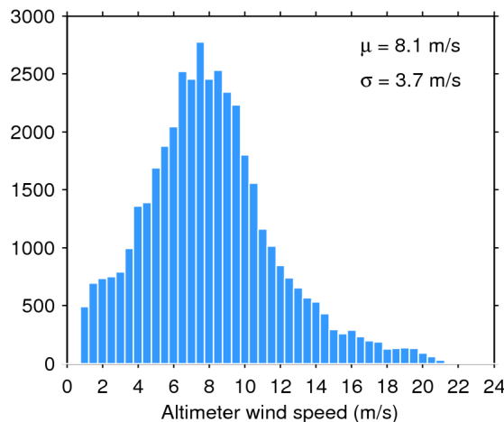
Figure 35. Histogram of science-valid wind over oceans and lakes for 12/05/2016. The mean ( \mu ) and standard deviation ( \sigma ) are also shown. Note that values larger than 24 m/s are excluded from the histogram for the sake of readability but not from the computation of \mu and \sigma .
