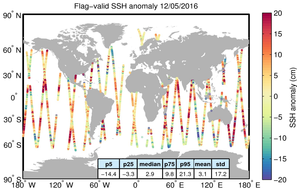
Figure 5. Geographical distribution of flag-valid 1-Hz SSH anomaly data over oceans and lakes for 12/05/2016. The statistical values shown in the table refer to the SSH anomaly in cm and are calculated over all measurements shown in the figure.
