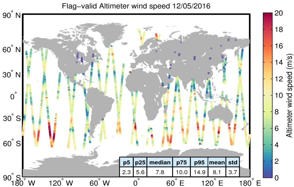
Figure 31. Geographical distribution of flag-valid wind data over oceans and lakes for 12/05/2016. The statistical values shown in the table refer to the wind in m/s and are calculated over all measurements shown in the figure.
