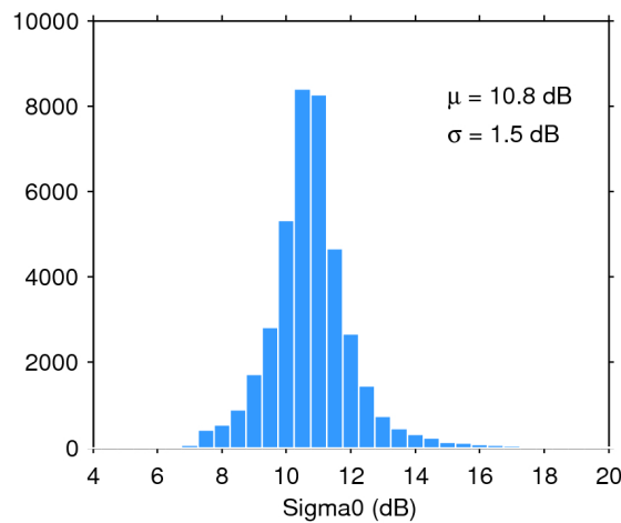
Figure 28. Histogram of science-valid sigma0 over oceans and lakes for 12/05/2016. The mean ( \mu ) and standard deviation ( \sigma ) are also shown. Note that values outside [4 20] dB are excluded from the histogram for the sake of readability but not from the computation of \mu and \sigma .
