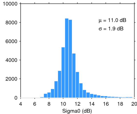
Figure 25. Histogram of flag-valid sigma0 over oceans and lakes for 12/05/2016. The mean ( \mu ) and standard deviation ( \sigma ) are also shown. Note that values outside [4 20] dB are excluded from the histogram for the sake of readability but not from the computation of \mu and \sigma .
