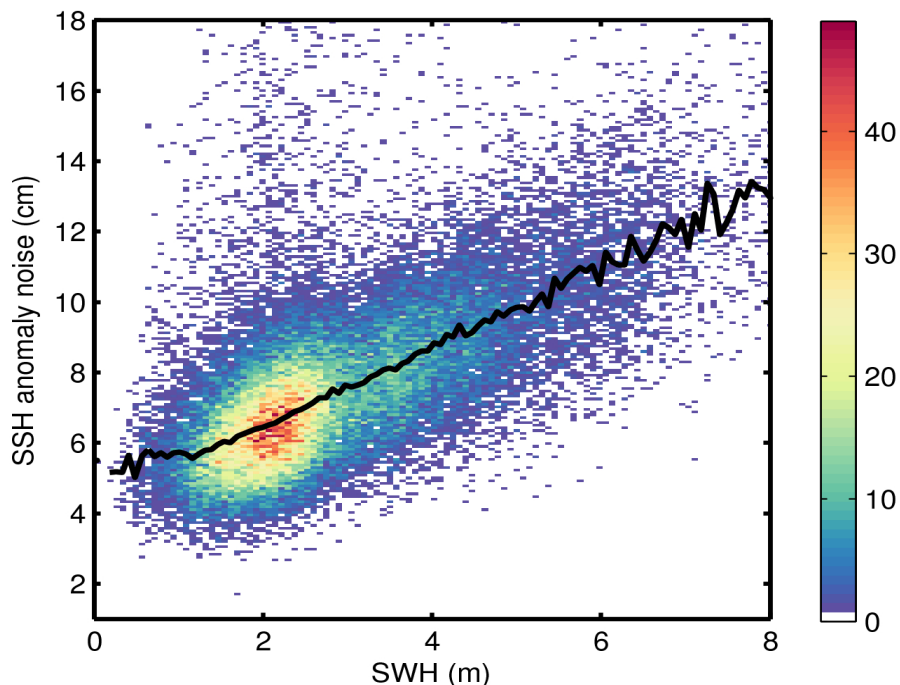
Figure 9. 2D histogram showing flag-valid SSH anomaly noise as a function of SWH for 12/05/2016. The black line denotes the median SSH anomaly noise as a function of SWH.
