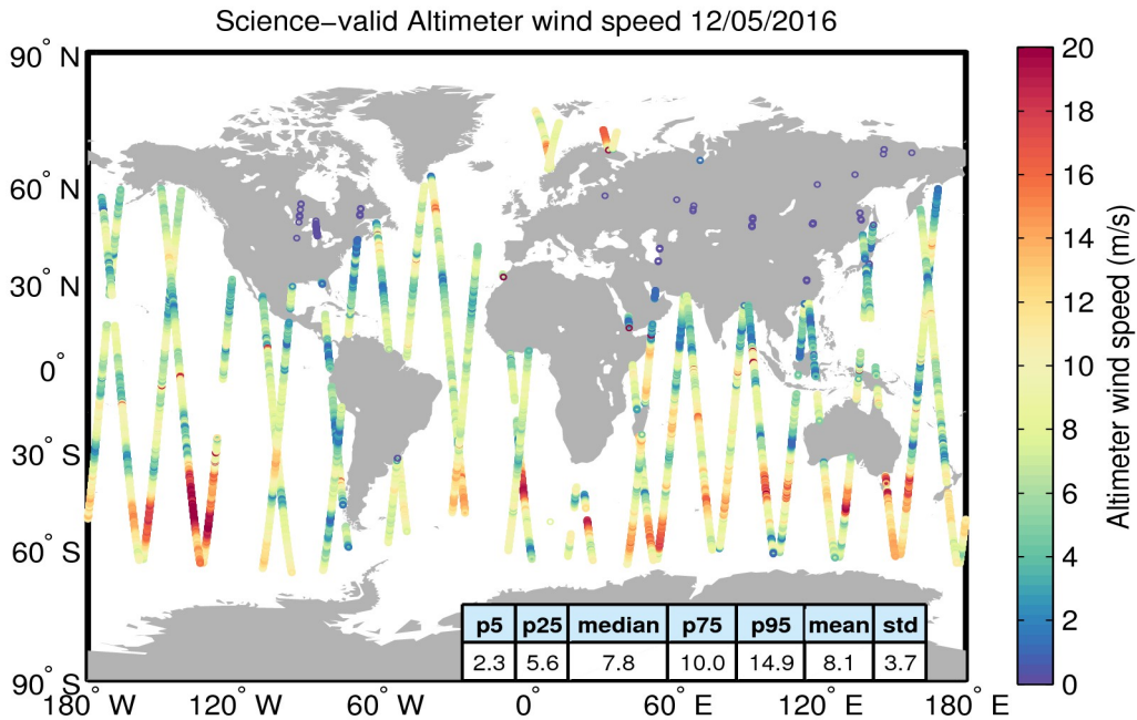
Figure 34. Geographical distribution of science-valid wind data over oceans and lakes for 12/05/2016. The statistical values shown in the table refer to the wind in m/s and are calculated over all measurements shown in the figure. Gray circles denote records that have been rejected based on the editing criteria described in Table 5.
