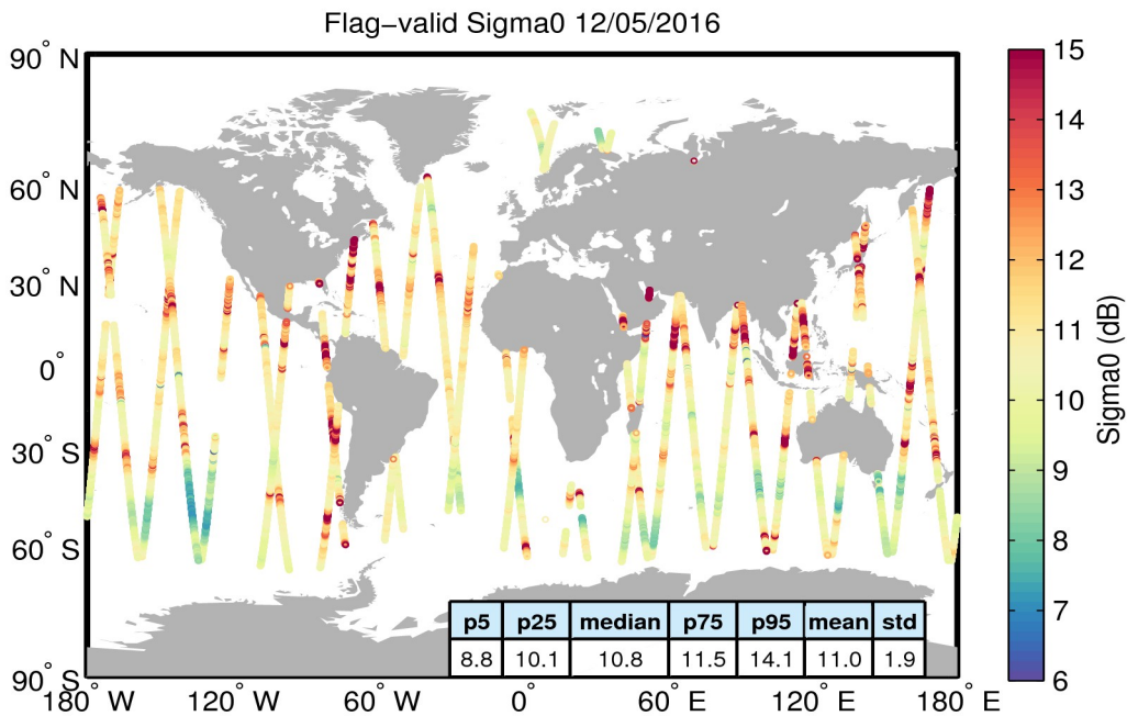
Figure 23. Geographical distribution of flag-valid sigma0 data over oceans and lakes for 12/05/2016. The statistical values shown in the table refer to the sigma0 in dB and are calculated over all measurements shown in the figure.
