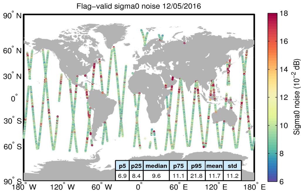
Figure 26. Geographical distribution of flag-valid 20-Hz sigma0 measurement noise over oceans and lakes for 12/05/2016. The statistical values shown in the table refer to the sigma0 noise and are calculated over all measurements shown in the figure.
