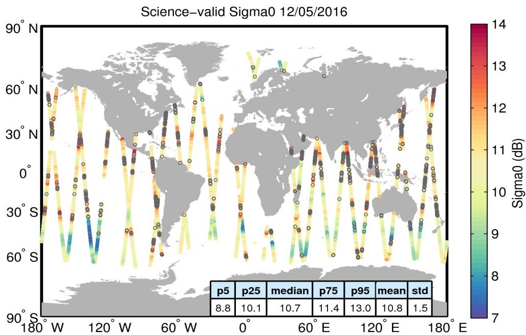
Figure 27. Geographical distribution of science-valid sigma0 data over oceans and lakes for 12/05/2016. The statistical values shown in the table refer to the sigma0 in dB and are calculated over all measurements shown in the figure. Gray circles denote records that have been rejected based on the editing criteria described in Table 4.
