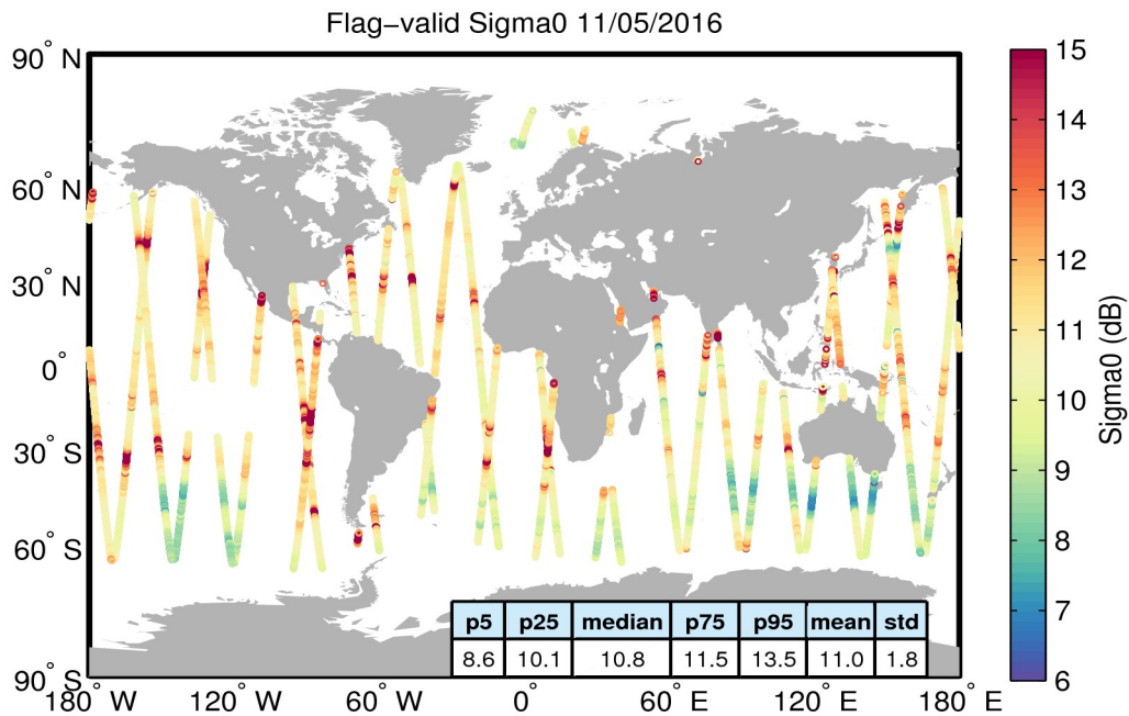
Figure 23. Geographical distribution of flag-valid sigma0 data over oceans and lakes for 11/05/2016. The statistical values shown in the table refer to the sigma0 in dB and are calculated over all measurements shown in the figure.
