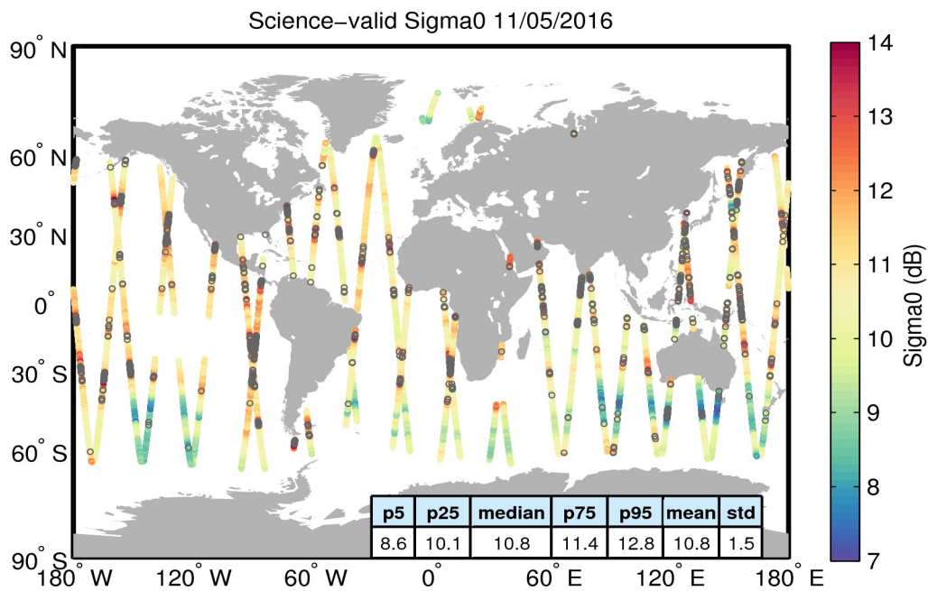
Figure 27. Geographical distribution of science-valid sigma0 data over oceans and lakes for 11/05/2016. The statistical values shown in the table refer to the sigma0 in dB and are calculated over all measurements shown in the figure. Gray circles denote records that have been rejected based on the editing criteria described in Table 4.
