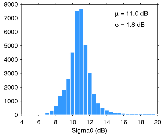
Figure 25. Histogram of flag-valid sigma0 over oceans and lakes for 11/05/2016. The mean ( \mu ) and standard deviation ( \sigma ) are also shown. Note that values outside [4 20] dB are excluded from the histogram for the sake of readability but not from the computation of \mu and \sigma .
