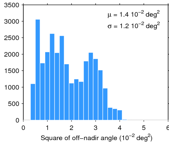
Figure 39. Histogram of flag-valid mispointing over oceans and lakes for 11/05/2016. The mean ( \mu ) and standard deviation ( \sigma ) are also shown. Note that values larger than 6 \cdot 10^{-2} \text{ deg}^2 are excluded from the histogram for the sake of readability but not from the computation of \mu and \sigma .
