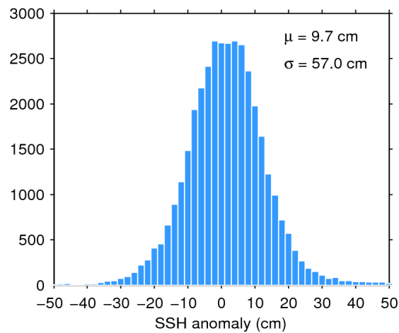
Figure 7. Histogram of flag-valid SSH anomaly over oceans and lakes for 11/05/2016. The mean ( \mu ) and standard deviation ( \sigma ) are also shown. Note that values outside [-50 50] cm are excluded from the histogram for the sake of readability but not from the computation of \mu and \sigma .
