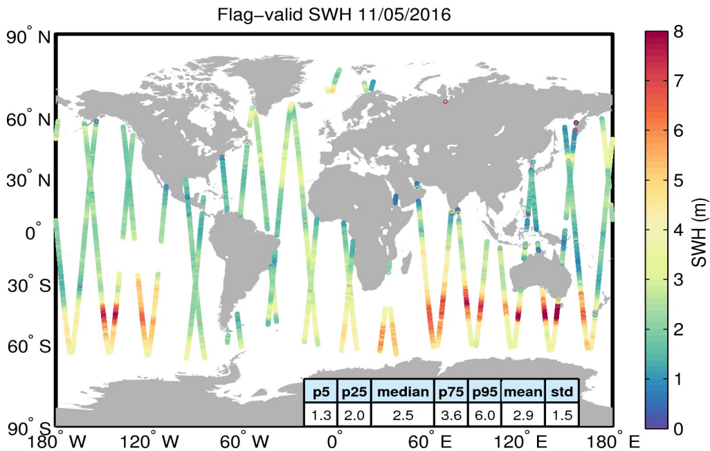
Figure 15. Geographical distribution of flag-valid SWH data over oceans and lakes for 11/05/2016. The statistical values shown in the table refer to the SWH in m and are calculated over all measurements shown in the figure.
