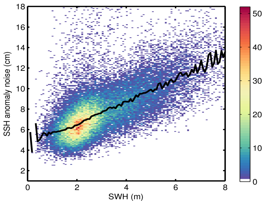
Figure 9. 2D histogram showing flag-valid SSH anomaly noise as a function of SWH for 11/05/2016. The black line denotes the median SSH anomaly noise as a function of SWH.
