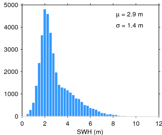
Figure 20. Histogram of science-valid SWH over oceans and lakes for 11/05/2016. The mean ( \mu ) and standard deviation ( \sigma ) are also shown. Note that values larger than 12 m are excluded from the histogram for the sake of readability but not from the computation of \mu and \sigma .
