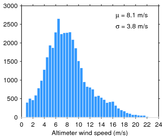
Figure 35. Histogram of science-valid wind over oceans and lakes for 11/05/2016. The mean ( \mu ) and standard deviation ( \sigma ) are also shown. Note that values larger than 24 m/s are excluded from the histogram for the sake of readability but not from the computation of \mu and \sigma .
