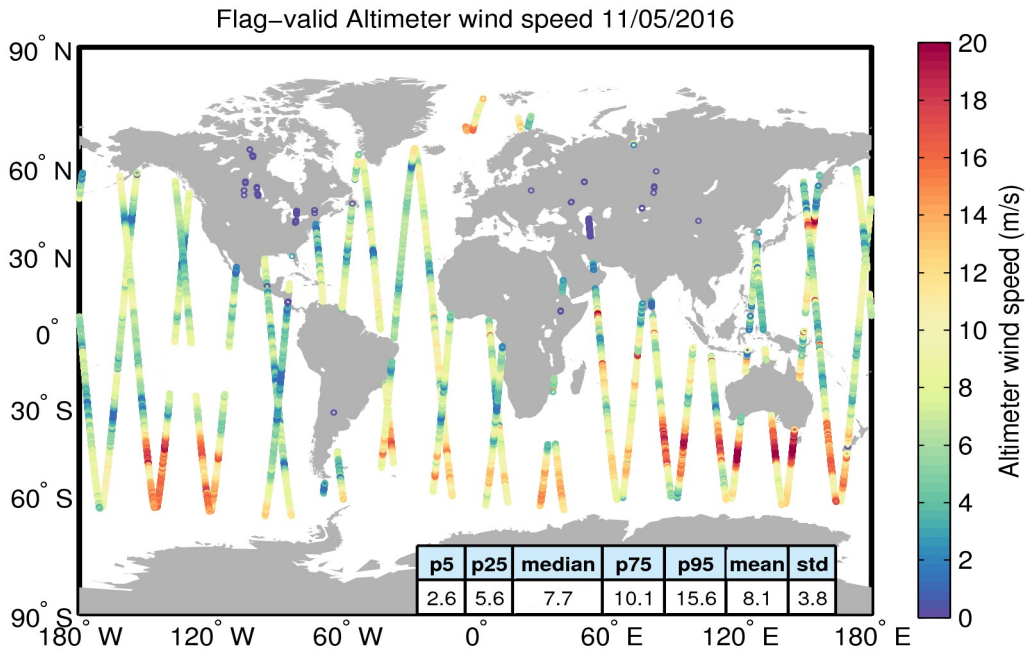
Figure 31. Geographical distribution of flag-valid wind data over oceans and lakes for 11/05/2016. The statistical values shown in the table refer to the wind in m/s and are calculated over all measurements shown in the figure.
