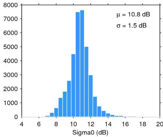
Figure 28. Histogram of science-valid sigma0 over oceans and lakes for 11/05/2016. The mean ( \mu ) and standard deviation ( \sigma ) are also shown. Note that values outside [4 20] dB are excluded from the histogram for the sake of readability but not from the computation of \mu and \sigma .
