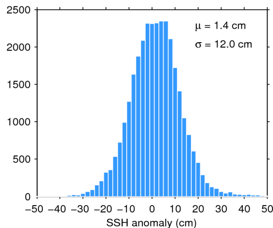
Figure 11. Histogram of science-valid SSH anomaly over oceans and lakes for 11/05/2016. The mean ( \mu ) and standard deviation ( \sigma ) are also shown. Note that values outside [-50 50] cm are excluded from the histogram for the sake of readability but not from the computation of \mu and \sigma .
