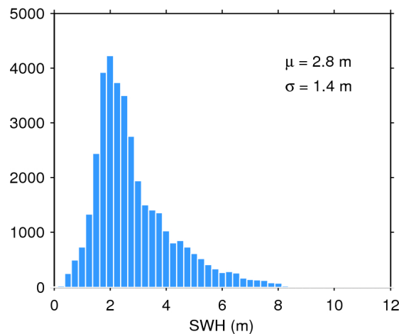
Figure 20. Histogram of science-valid SWH over oceans and lakes for 10/05/2016. The mean ( \mu ) and standard deviation ( \sigma ) are also shown. Note that values larger than 12 m are excluded from the histogram for the sake of readability but not from the computation of \mu and \sigma .
