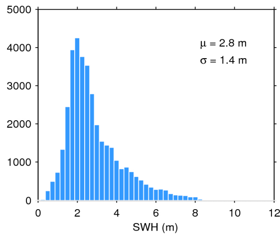
Figure 17. Histogram of flag-valid SWH over oceans and lakes for 10/05/2016. The mean ( \mu ) and standard deviation ( \sigma ) are also shown. Note that values larger than 12 m are excluded from the histogram for the sake of readability but not from the computation of \mu and \sigma .
