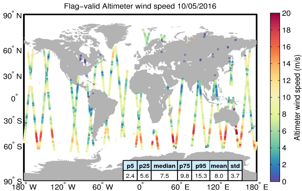
Figure 31. Geographical distribution of flag-valid wind data over oceans and lakes for 10/05/2016. The statistical values shown in the table refer to the wind in m/s and are calculated over all measurements shown in the figure.
