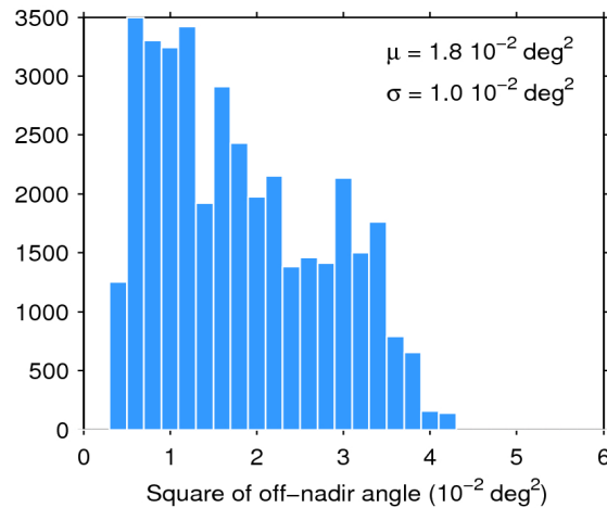
Figure 39. Histogram of flag-valid mispointing over oceans and lakes for 10/05/2016. The mean ( \mu ) and standard deviation ( \sigma ) are also shown. Note that values larger than 6 \cdot 10^{-2} \text{ deg}^2 are excluded from the histogram for the sake of readability but not from the computation of \mu and \sigma .
