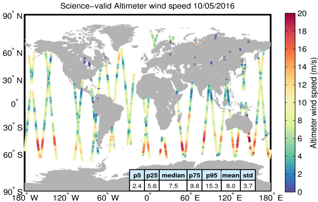
Figure 34. Geographical distribution of science-valid wind data over oceans and lakes for 10/05/2016. The statistical values shown in the table refer to the wind in m/s and are calculated over all measurements shown in the figure. Gray circles denote records that have been rejected based on the editing criteria described in Table 5.
