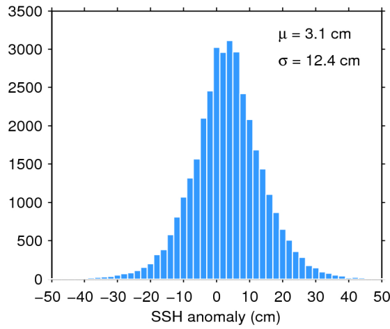
Figure 11. Histogram of science-valid SSH anomaly over oceans and lakes for 10/05/2016. The mean ( \mu ) and standard deviation ( \sigma ) are also shown. Note that values outside [-50 50] cm are excluded from the histogram for the sake of readability but not from the computation of \mu and \sigma .
