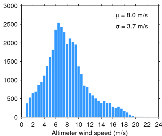
Figure 35. Histogram of science-valid wind over oceans and lakes for 10/05/2016. The mean ( \mu ) and standard deviation ( \sigma ) are also shown. Note that values larger than 24 m/s are excluded from the histogram for the sake of readability but not from the computation of \mu and \sigma .
