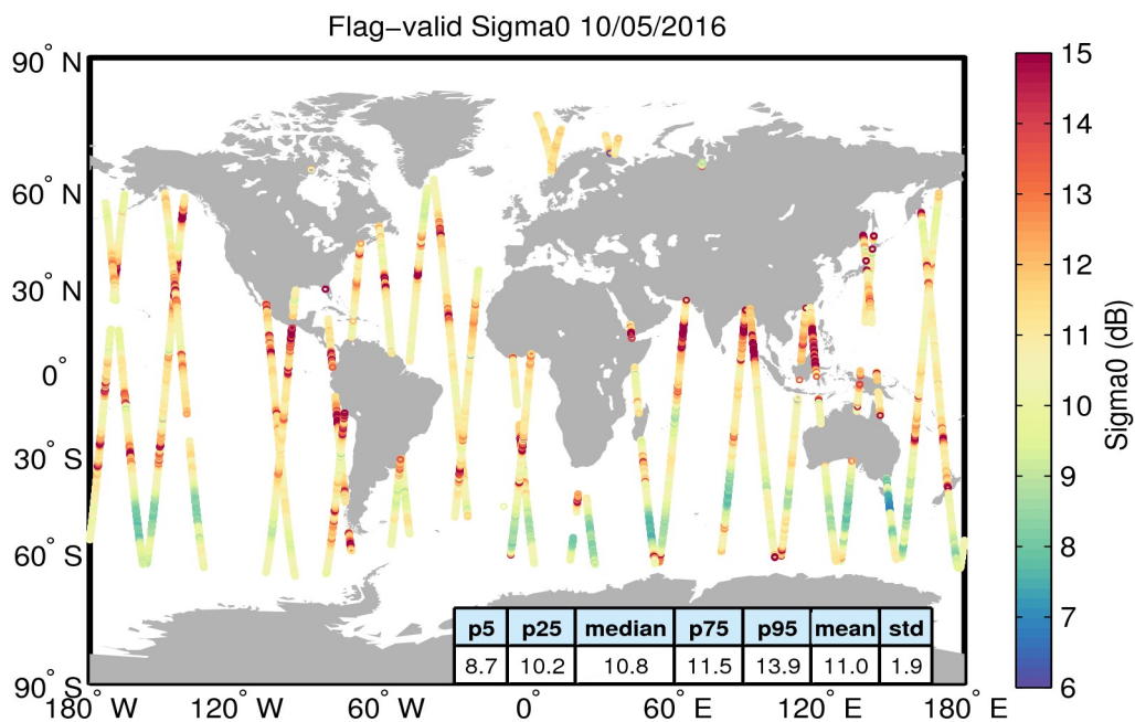
Figure 23. Geographical distribution of flag-valid sigma0 data over oceans and lakes for 10/05/2016. The statistical values shown in the table refer to the sigma0 in dB and are calculated over all measurements shown in the figure.
