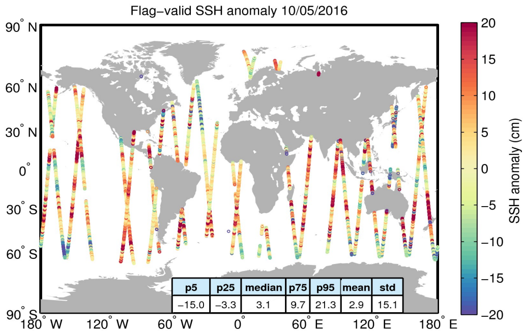
Figure 5. Geographical distribution of flag-valid 1-Hz SSH anomaly data over oceans and lakes for 10/05/2016. The statistical values shown in the table refer to the SSH anomaly in cm and are calculated over all measurements shown in the figure.
