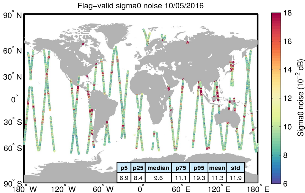
Figure 26. Geographical distribution of flag-valid 20-Hz sigma0 measurement noise over oceans and lakes for 10/05/2016. The statistical values shown in the table refer to the sigma0 noise and are calculated over all measurements shown in the figure.
