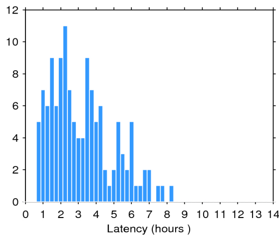
Figure 2. Histogram of the data latency for 10/05/2016. The y-axis denotes the number of files that are made available with a delay of x-hours with respect to the mean time of the records stored in the file.
