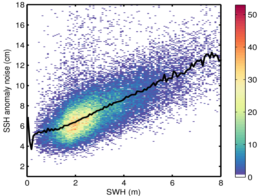
Figure 9. 2D histogram showing flag-valid SSH anomaly noise as a function of SWH for 10/05/2016. The black line denotes the median SSH anomaly noise as a function of SWH.
