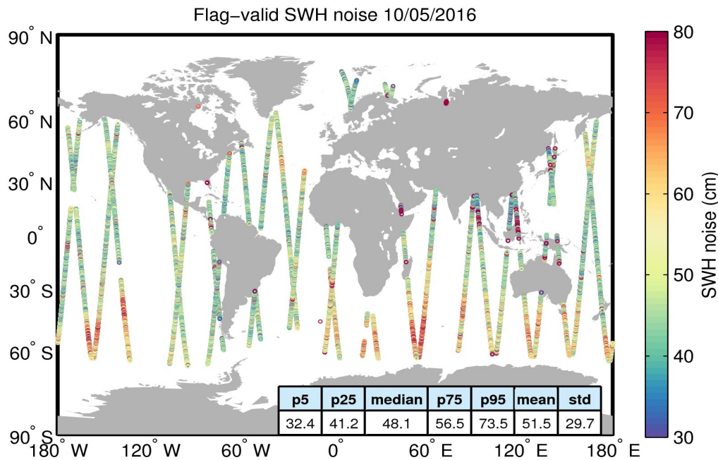
Figure 18. Geographical distribution of flag-valid 20-Hz SWH measurement noise over oceans and lakes for 10/05/2016. The statistical values shown in the figure refer to the SWH noise and are calculated over all measurements shown in the figure.
