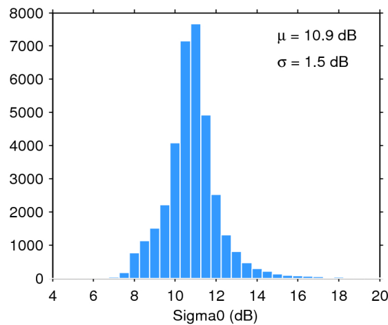
Figure 28. Histogram of science-valid sigma0 over oceans and lakes for 10/05/2016. The mean ( \mu ) and standard deviation ( \sigma ) are also shown. Note that values outside [4 20] dB are excluded from the histogram for the sake of readability but not from the computation of \mu and \sigma .
