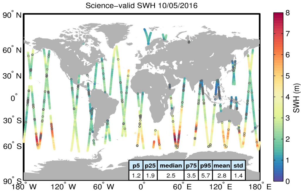
Figure 19. Geographical distribution of science-valid SWH data over oceans and lakes for 10/05/2016. The statistical values shown in the table refer to the SWH in m and are calculated over all measurements shown in the figure. Gray circles denote records that have been rejected based on the editing criteria described in Table 3.
