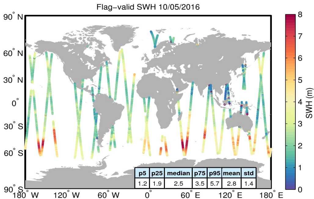
Figure 15. Geographical distribution of flag-valid SWH data over oceans and lakes for 10/05/2016. The statistical values shown in the table refer to the SWH in m and are calculated over all measurements shown in the figure.
