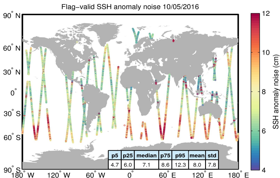
Figure 8. Geographical distribution of flag-valid 20-Hz SSH anomaly measurement noise over oceans and lakes for 10/05/2016. The statistical values shown in the table refer to the SSH anomaly noise and are calculated over all measurements shown in the figure.
