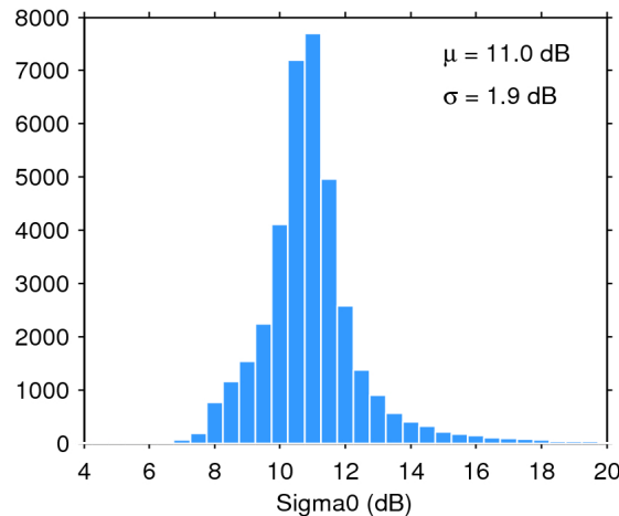
Figure 25. Histogram of flag-valid sigma0 over oceans and lakes for 10/05/2016. The mean ( \mu ) and standard deviation ( \sigma ) are also shown. Note that values outside [4 20] dB are excluded from the histogram for the sake of readability but not from the computation of \mu and \sigma .
