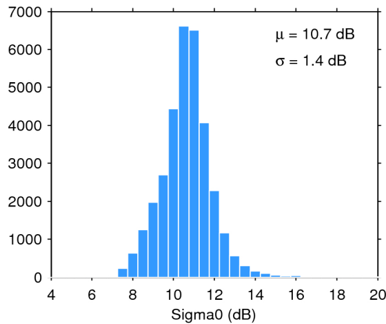
Figure 28. Histogram of science-valid sigma0 over oceans and lakes for 09/05/2016. The mean ( \mu ) and standard deviation ( \sigma ) are also shown. Note that values outside [4 20] dB are excluded from the histogram for the sake of readability but not from the computation of \mu and \sigma .
