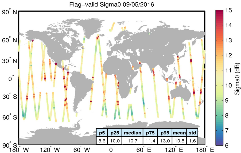
Figure 23. Geographical distribution of flag-valid sigma0 data over oceans and lakes for 09/05/2016. The statistical values shown in the table refer to the sigma0 in dB and are calculated over all measurements shown in the figure.
