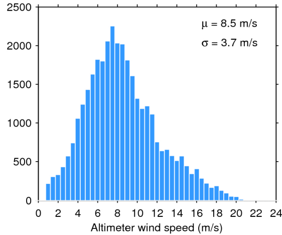
Figure 33. Histogram of flag-valid wind over oceans and lakes for 09/05/2016. The mean ( \mu ) and standard deviation ( \sigma ) are also shown. Note that values larger than 24 m/s are excluded from the histogram for the sake of readability but not from the computation of \mu and \sigma .
