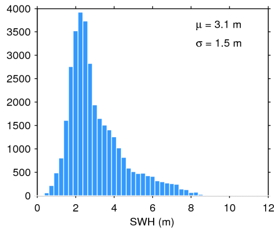
Figure 17. Histogram of flag-valid SWH over oceans and lakes for 09/05/2016. The mean ( \mu ) and standard deviation ( \sigma ) are also shown. Note that values larger than 12 m are excluded from the histogram for the sake of readability but not from the computation of \mu and \sigma .
