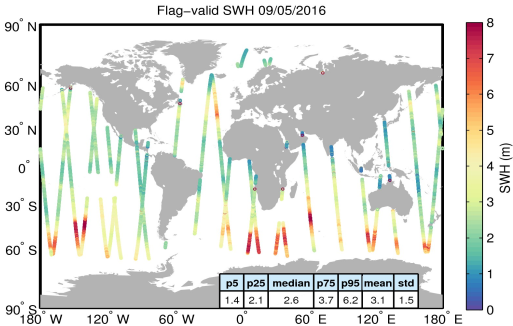
Figure 15. Geographical distribution of flag-valid SWH data over oceans and lakes for 09/05/2016. The statistical values shown in the table refer to the SWH in m and are calculated over all measurements shown in the figure.
