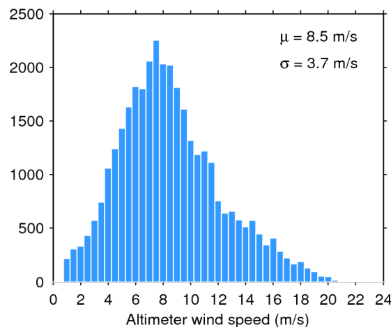
Figure 35. Histogram of science-valid wind over oceans and lakes for 09/05/2016. The mean ( \mu ) and standard deviation ( \sigma ) are also shown. Note that values larger than 24 m/s are excluded from the histogram for the sake of readability but not from the computation of \mu and \sigma .
