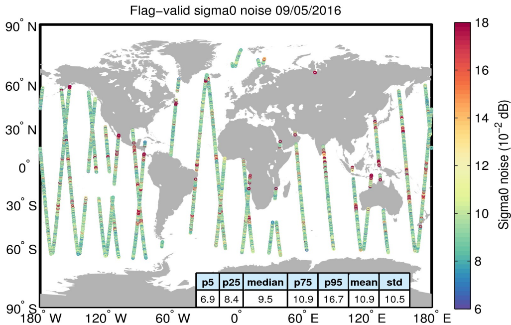
Figure 26. Geographical distribution of flag-valid 20-Hz sigma0 measurement noise over oceans and lakes for 09/05/2016. The statistical values shown in the table refer to the sigma0 noise and are calculated over all measurements shown in the figure.
