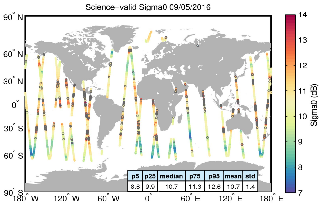
Figure 27. Geographical distribution of science-valid sigma0 data over oceans and lakes for 09/05/2016. The statistical values shown in the table refer to the sigma0 in dB and are calculated over all measurements shown in the figure. Gray circles denote records that have been rejected based on the editing criteria described in Table 4.
