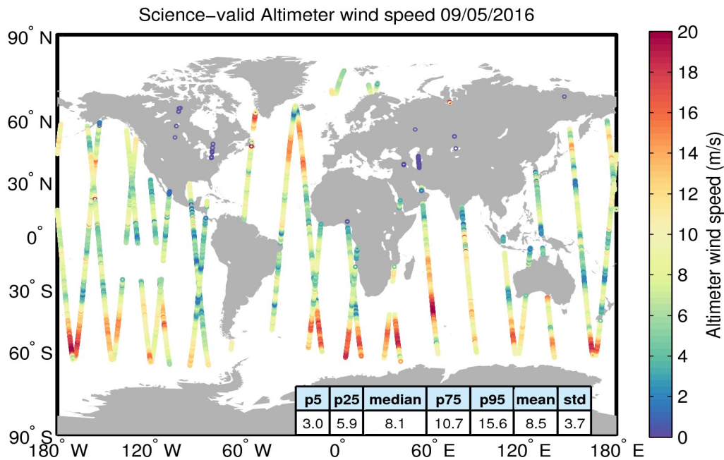
Figure 34. Geographical distribution of science-valid wind data over oceans and lakes for 09/05/2016. The statistical values shown in the table refer to the wind in m/s and are calculated over all measurements shown in the figure. Gray circles denote records that have been rejected based on the editing criteria described in Table 5.
