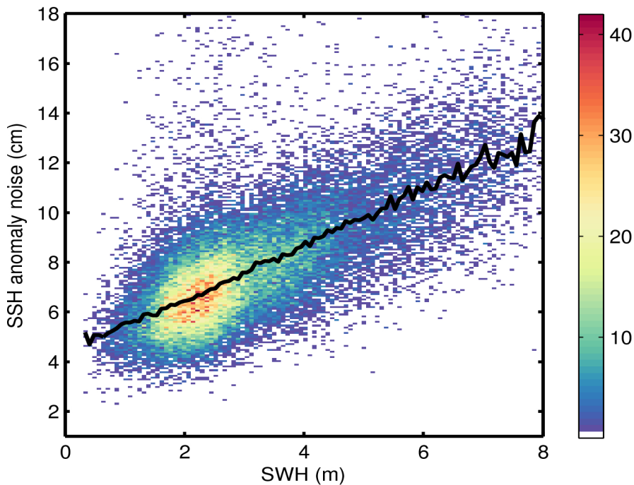
Figure 9. 2D histogram showing flag-valid SSH anomaly noise as a function of SWH for 09/05/2016. The black line denotes the median SSH anomaly noise as a function of SWH.
