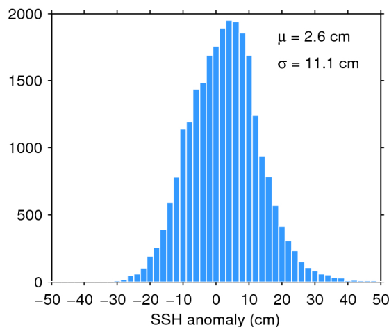
Figure 11. Histogram of science-valid SSH anomaly over oceans and lakes for 09/05/2016. The mean ( \mu ) and standard deviation ( \sigma ) are also shown. Note that values outside [-50 50] cm are excluded from the histogram for the sake of readability but not from the computation of \mu and \sigma .
