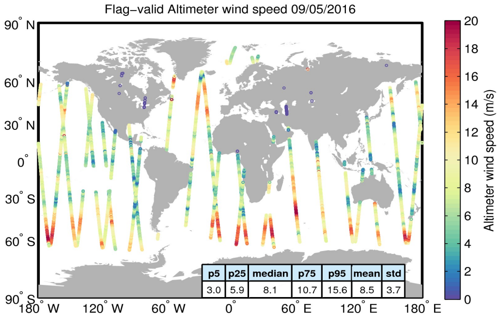
Figure 31. Geographical distribution of flag-valid wind data over oceans and lakes for 09/05/2016. The statistical values shown in the table refer to the wind in m/s and are calculated over all measurements shown in the figure.
