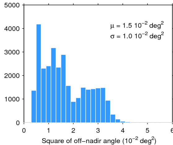
Figure 39. Histogram of flag-valid mispointing over oceans and lakes for 09/05/2016. The mean ( \mu ) and standard deviation ( \sigma ) are also shown. Note that values larger than 6 \cdot 10^{-2} \text{ deg}^2 are excluded from the histogram for the sake of readability but not from the computation of \mu and \sigma .
