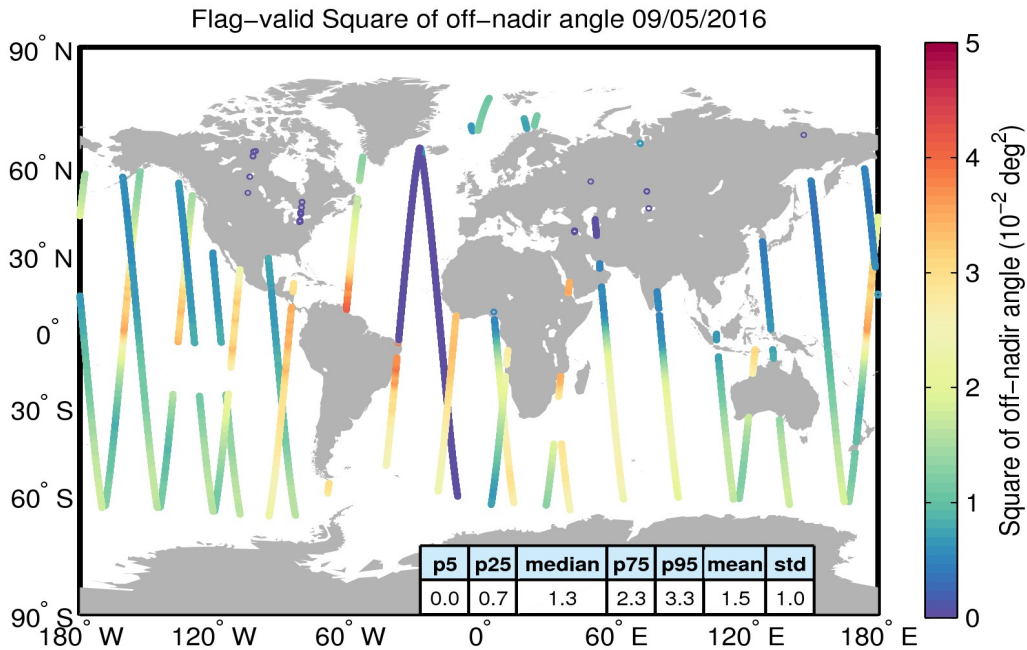
Figure 37. Geographical distribution of flag-valid mispointing data over oceans and lakes for 09/05/2016. The statistical values shown in the table refer to the mispointing in 10^{-2} \text{ deg}^2 and are calculated over all measurements shown in the figure.
