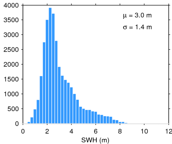
Figure 20. Histogram of science-valid SWH over oceans and lakes for 09/05/2016. The mean ( \mu ) and standard deviation ( \sigma ) are also shown. Note that values larger than 12 m are excluded from the histogram for the sake of readability but not from the computation of \mu and \sigma .
