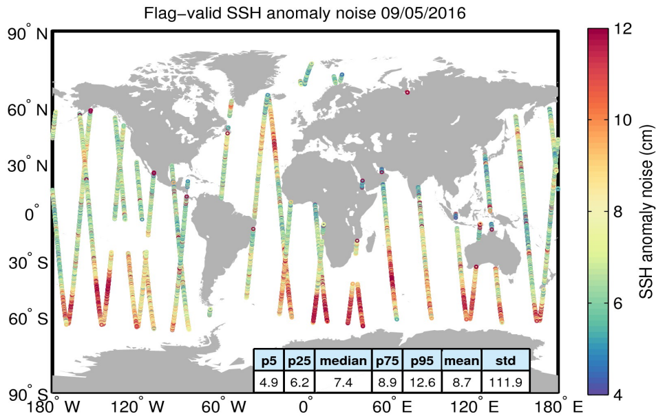
Figure 8. Geographical distribution of flag-valid 20-Hz SSH anomaly measurement noise over oceans and lakes for 09/05/2016. The statistical values shown in the table refer to the SSH anomaly noise and are calculated over all measurements shown in the figure.
