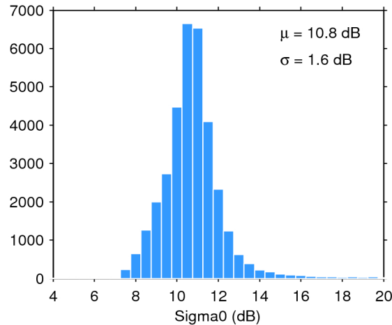
Figure 25. Histogram of flag-valid sigma0 over oceans and lakes for 09/05/2016. The mean ( \mu ) and standard deviation ( \sigma ) are also shown. Note that values outside [4 20] dB are excluded from the histogram for the sake of readability but not from the computation of \mu and \sigma .
