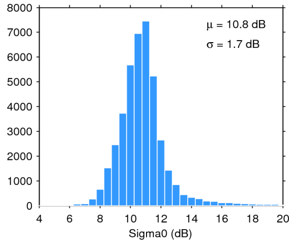
Figure 25. Histogram of flag-valid sigma0 over oceans and lakes for 07/05/2016. The mean ( \mu ) and standard deviation ( \sigma ) are also shown. Note that values outside [4 20] dB are excluded from the histogram for the sake of readability but not from the computation of \mu and \sigma .
