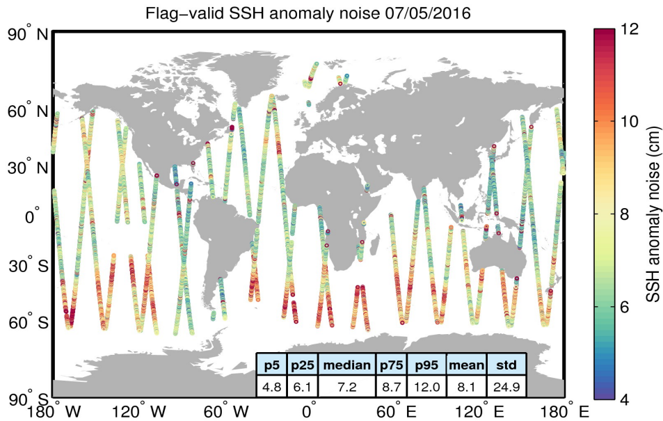
Figure 8. Geographical distribution of flag-valid 20-Hz SSH anomaly measurement noise over oceans and lakes for 07/05/2016. The statistical values shown in the table refer to the SSH anomaly noise and are calculated over all measurements shown in the figure.
