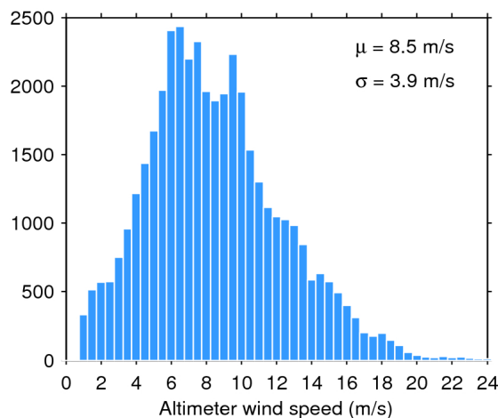
Figure 35. Histogram of science-valid wind over oceans and lakes for 07/05/2016. The mean ( \mu ) and standard deviation ( \sigma ) are also shown. Note that values larger than 24 m/s are excluded from the histogram for the sake of readability but not from the computation of \mu and \sigma .
