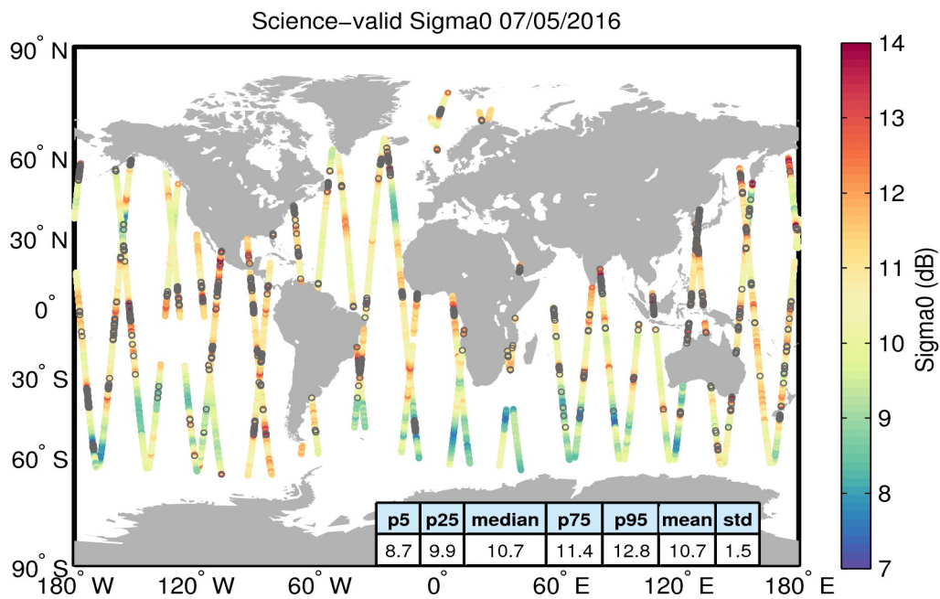
Figure 27. Geographical distribution of science-valid sigma0 data over oceans and lakes for 07/05/2016. The statistical values shown in the table refer to the sigma0 in dB and are calculated over all measurements shown in the figure. Gray circles denote records that have been rejected based on the editing criteria described in Table 4.
