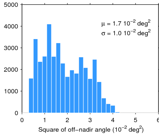
Figure 39. Histogram of flag-valid mispointing over oceans and lakes for 07/05/2016. The mean ( \mu ) and standard deviation ( \sigma ) are also shown. Note that values larger than 6 \cdot 10^{-2} \text{ deg}^2 are excluded from the histogram for the sake of readability but not from the computation of \mu and \sigma .
