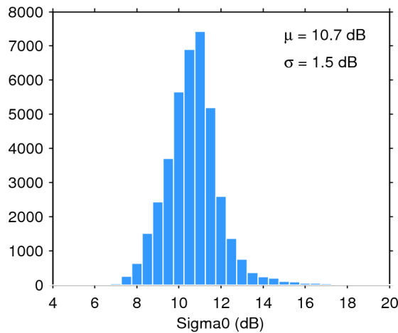
Figure 28. Histogram of science-valid sigma0 over oceans and lakes for 07/05/2016. The mean ( \mu ) and standard deviation ( \sigma ) are also shown. Note that values outside [4 20] dB are excluded from the histogram for the sake of readability but not from the computation of \mu and \sigma .
