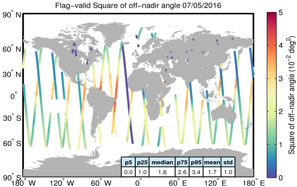
Figure 37. Geographical distribution of flag-valid mispointing data over oceans and lakes for 07/05/2016. The statistical values shown in the table refer to the mispointing in 10^{-2} \text{ deg}^2 and are calculated over all measurements shown in the figure.
