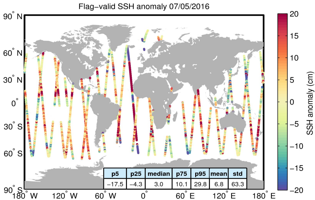
Figure 5. Geographical distribution of flag-valid 1-Hz SSH anomaly data over oceans and lakes for 07/05/2016. The statistical values shown in the table refer to the SSH anomaly in cm and are calculated over all measurements shown in the figure.
