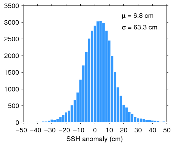
Figure 7. Histogram of flag-valid SSH anomaly over oceans and lakes for 07/05/2016. The mean ( \mu ) and standard deviation ( \sigma ) are also shown. Note that values outside [-50 50] cm are excluded from the histogram for the sake of readability but not from the computation of \mu and \sigma .
