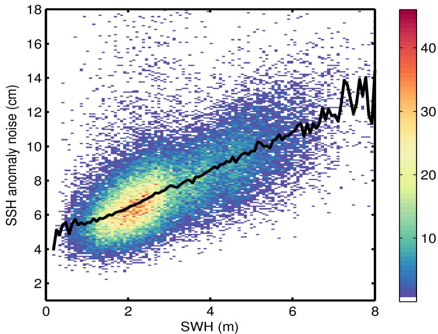
Figure 9. 2D histogram showing flag-valid SSH anomaly noise as a function of SWH for 07/05/2016. The black line denotes the median SSH anomaly noise as a function of SWH.
