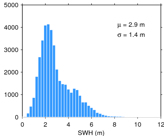
Figure 20. Histogram of science-valid SWH over oceans and lakes for 07/05/2016. The mean ( \mu ) and standard deviation ( \sigma ) are also shown. Note that values larger than 12 m are excluded from the histogram for the sake of readability but not from the computation of \mu and \sigma .
