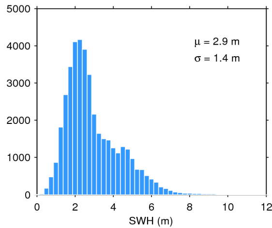
Figure 17. Histogram of flag-valid SWH over oceans and lakes for 07/05/2016. The mean ( \mu ) and standard deviation ( \sigma ) are also shown. Note that values larger than 12 m are excluded from the histogram for the sake of readability but not from the computation of \mu and \sigma .
