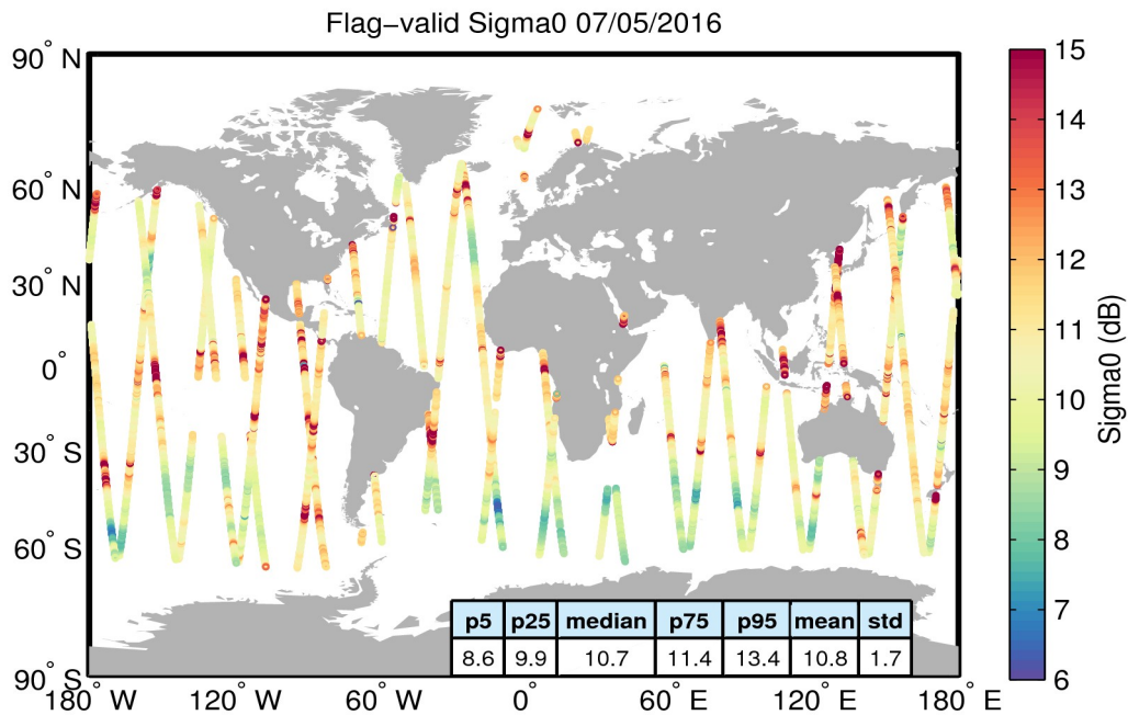
Figure 23. Geographical distribution of flag-valid sigma0 data over oceans and lakes for 07/05/2016. The statistical values shown in the table refer to the sigma0 in dB and are calculated over all measurements shown in the figure.
