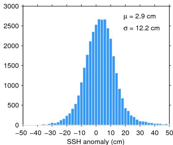
Figure 11. Histogram of science-valid SSH anomaly over oceans and lakes for 07/05/2016. The mean ( \mu ) and standard deviation ( \sigma ) are also shown. Note that values outside [-50 50] cm are excluded from the histogram for the sake of readability but not from the computation of \mu and \sigma .
