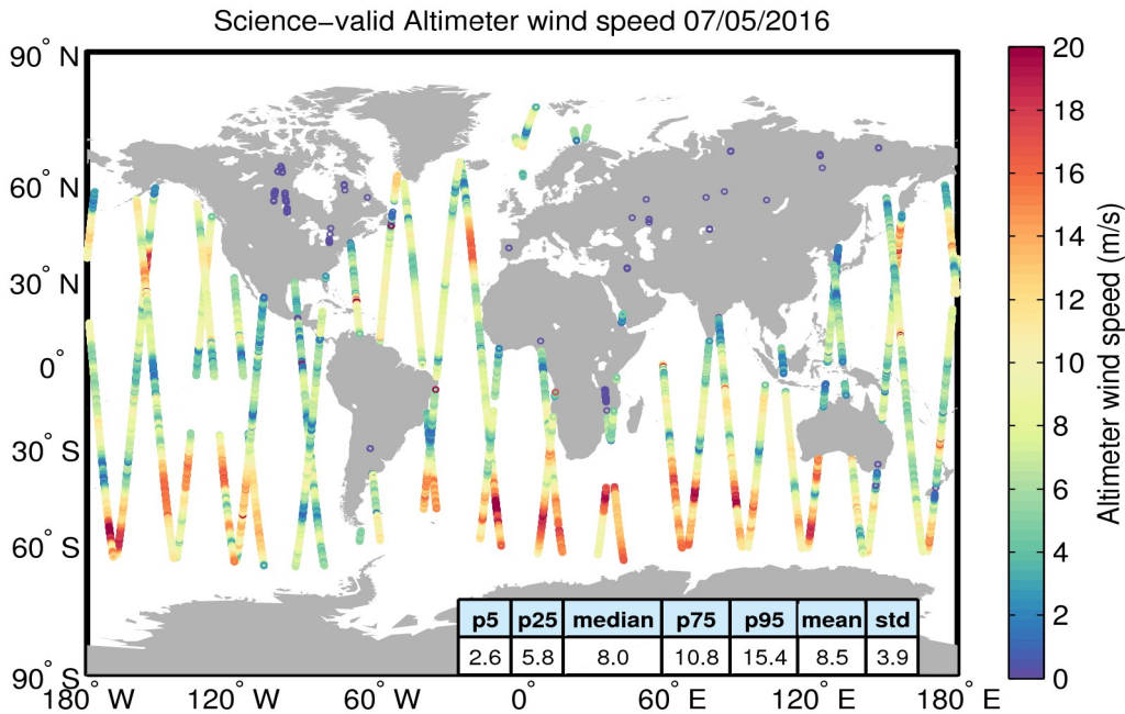
Figure 34. Geographical distribution of science-valid wind data over oceans and lakes for 07/05/2016. The statistical values shown in the table refer to the wind in m/s and are calculated over all measurements shown in the figure. Gray circles denote records that have been rejected based on the editing criteria described in Table 5.
