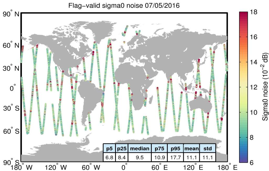
Figure 26. Geographical distribution of flag-valid 20-Hz sigma0 measurement noise over oceans and lakes for 07/05/2016. The statistical values shown in the table refer to the sigma0 noise and are calculated over all measurements shown in the figure.
