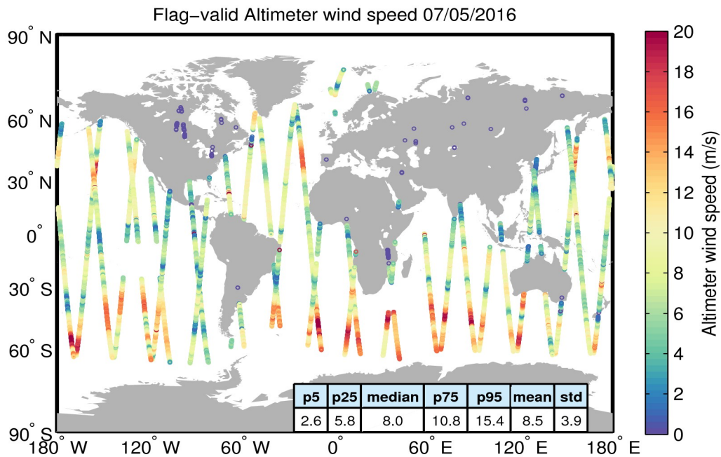
Figure 31. Geographical distribution of flag-valid wind data over oceans and lakes for 07/05/2016. The statistical values shown in the table refer to the wind in m/s and are calculated over all measurements shown in the figure.
