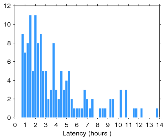
Figure 2. Histogram of the data latency for 07/05/2016. The y-axis denotes the number of files that are made available with a delay of x-hours with respect to the mean time of the records stored in the file.
