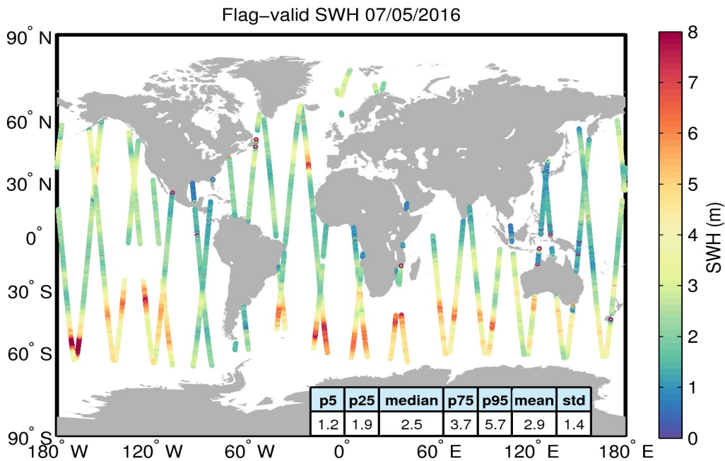
Figure 15. Geographical distribution of flag-valid SWH data over oceans and lakes for 07/05/2016. The statistical values shown in the table refer to the SWH in m and are calculated over all measurements shown in the figure.
