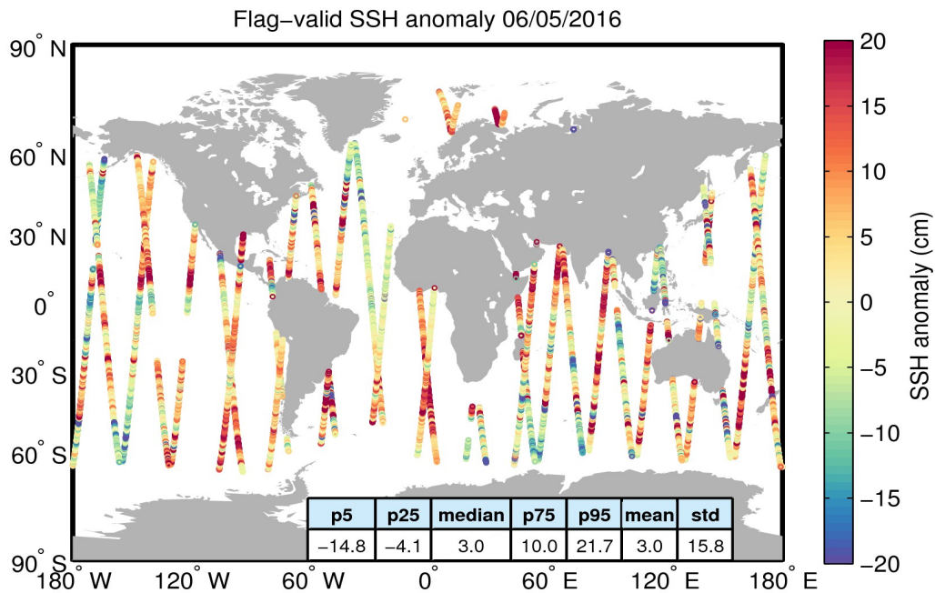
Figure 5. Geographical distribution of flag-valid 1-Hz SSH anomaly data over oceans and lakes for 06/05/2016. The statistical values shown in the table refer to the SSH anomaly in cm and are calculated over all measurements shown in the figure.
