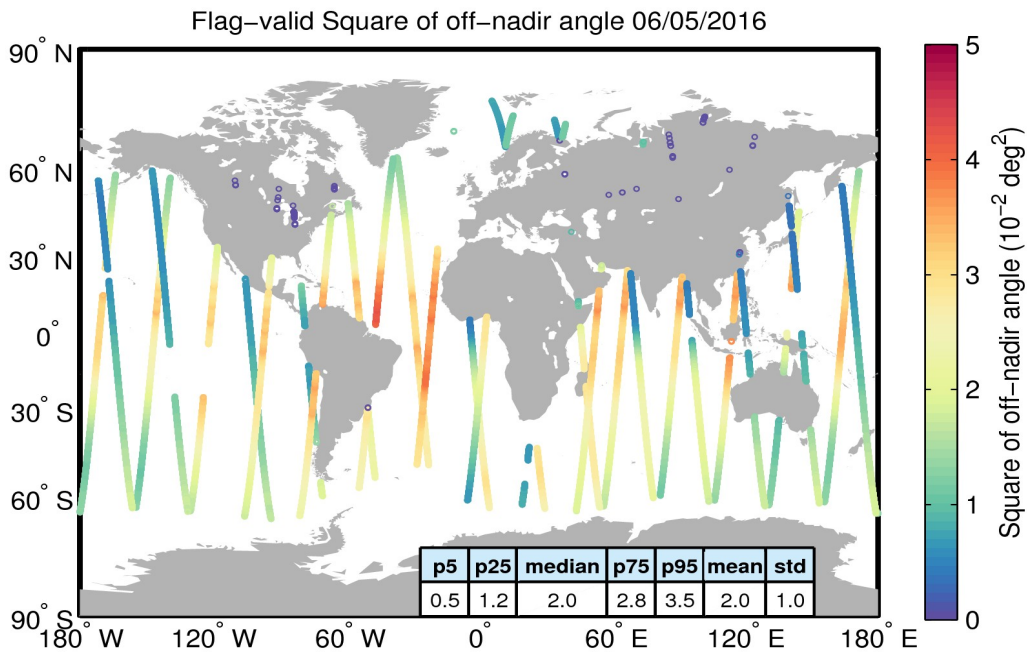
Figure 37. Geographical distribution of flag-valid mispointing data over oceans and lakes for 06/05/2016. The statistical values shown in the table refer to the mispointing in 10^{-2} deg 2 and are calculated over all measurements shown in the figure.
