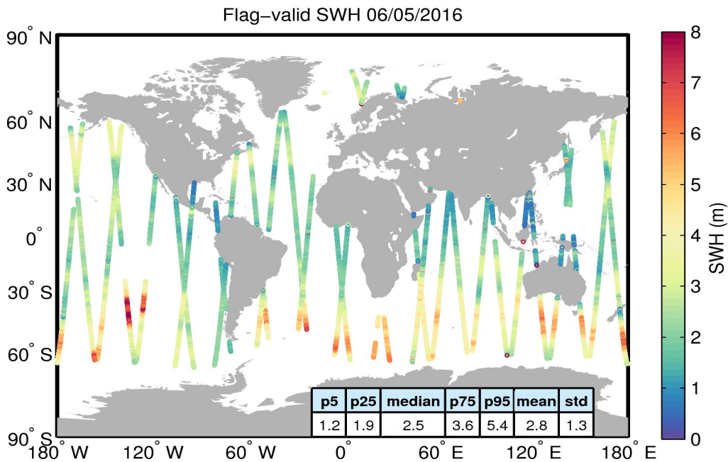
Figure 15. Geographical distribution of flag-valid SWH data over oceans and lakes for 06/05/2016. The statistical values shown in the table refer to the SWH in m and are calculated over all measurements shown in the figure.
