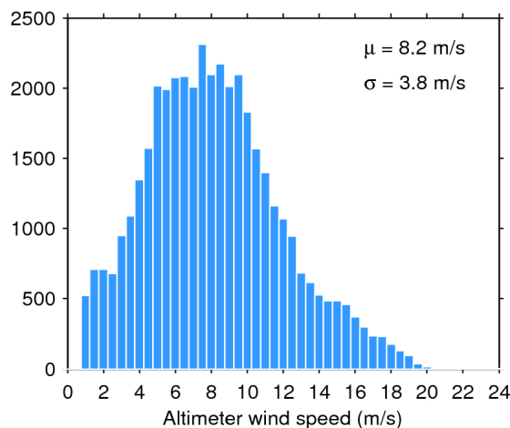
Figure 35. Histogram of science-valid wind over oceans and lakes for 06/05/2016. The mean ( \mu ) and standard deviation ( \sigma ) are also shown. Note that values larger than 24 m/s are excluded from the histogram for the sake of readability but not from the computation of \mu and \sigma .
