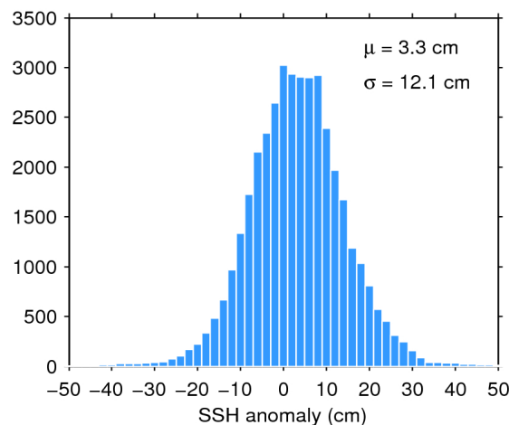
Figure 11. Histogram of science-valid SSH anomaly over oceans and lakes for 06/05/2016. The mean ( \mu ) and standard deviation ( \sigma ) are also shown. Note that values outside [-50 50] cm are excluded from the histogram for the sake of readability but not from the computation of \mu and \sigma .
