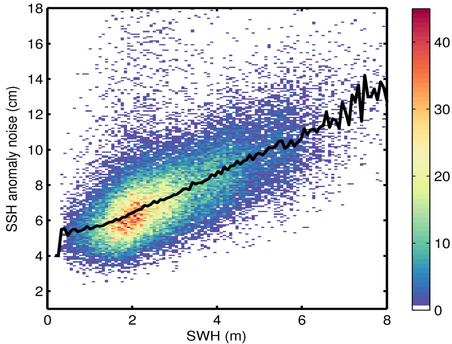
Figure 9. 2D histogram showing flag-valid SSH anomaly noise as a function of SWH for 06/05/2016. The black line denotes the median SSH anomaly noise as a function of SWH.
