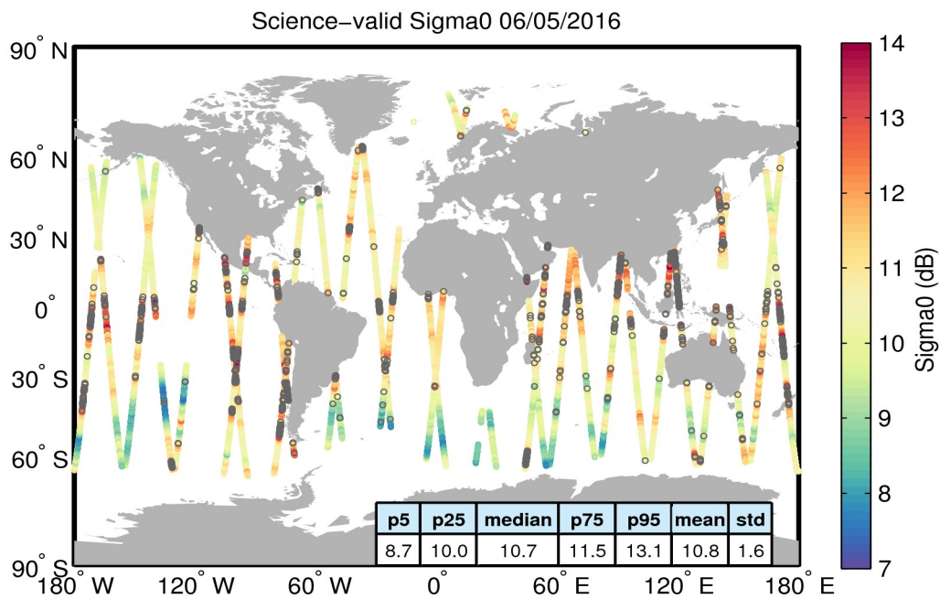
Figure 27. Geographical distribution of science-valid sigma0 data over oceans and lakes for 06/05/2016. The statistical values shown in the table refer to the sigma0 in dB and are calculated over all measurements shown in the figure. Gray circles denote records that have been rejected based on the editing criteria described in Table 4.
