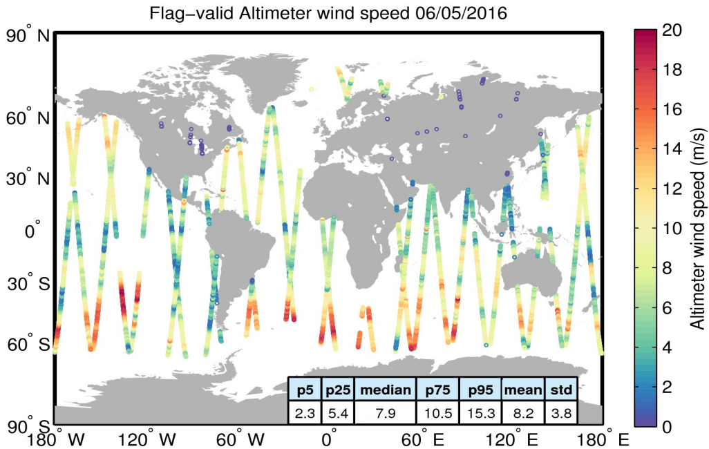
Figure 31. Geographical distribution of flag-valid wind data over oceans and lakes for 06/05/2016. The statistical values shown in the table refer to the wind in m/s and are calculated over all measurements shown in the figure.
