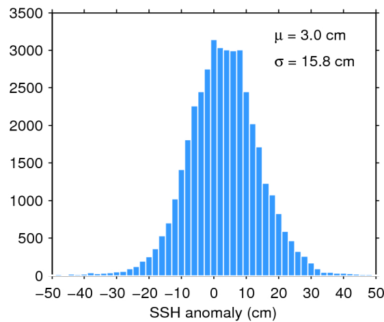
Figure 7. Histogram of flag-valid SSH anomaly over oceans and lakes for 06/05/2016. The mean ( \mu ) and standard deviation ( \sigma ) are also shown. Note that values outside [-50\ 50] cm are excluded from the histogram for the sake of readability but not from the computation of \mu and \sigma .
