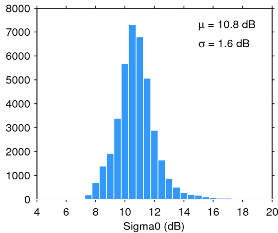
Figure 28. Histogram of science-valid sigma0 over oceans and lakes for 06/05/2016. The mean ( \mu ) and standard deviation ( \sigma ) are also shown. Note that values outside [4 20] dB are excluded from the histogram for the sake of readability but not from the computation of \mu and \sigma .
