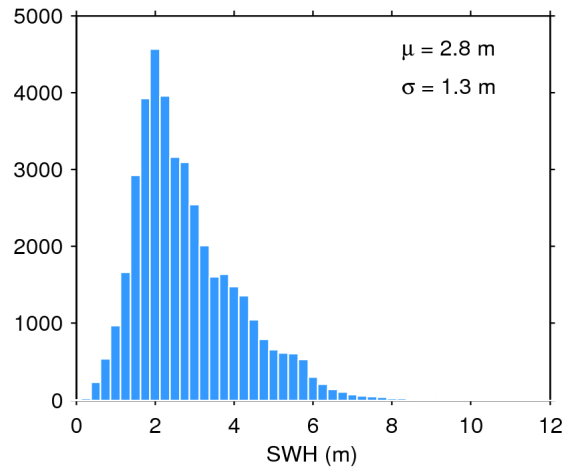
Figure 17. Histogram of flag-valid SWH over oceans and lakes for 06/05/2016. The mean ( \mu ) and standard deviation ( \sigma ) are also shown. Note that values larger than 12 m are excluded from the histogram for the sake of readability but not from the computation of \mu and \sigma .
