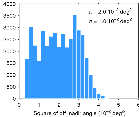
Figure 39. Histogram of flag-valid mispointing over oceans and lakes for 06/05/2016. The mean ( \mu ) and standard deviation ( \sigma ) are also shown. Note that values larger than 6 \cdot 10^{-2} \text{ deg}^2 are excluded from the histogram for the sake of readability but not from the computation of \mu and \sigma .
