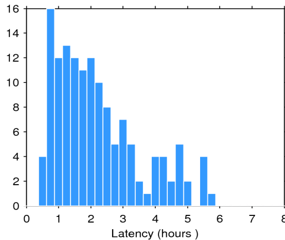
Figure 2. Histogram of the data latency for 06/05/2016. The y-axis denotes the number of files that are made available with a delay of x-hours with respect to the mean time of the records stored in the file.
