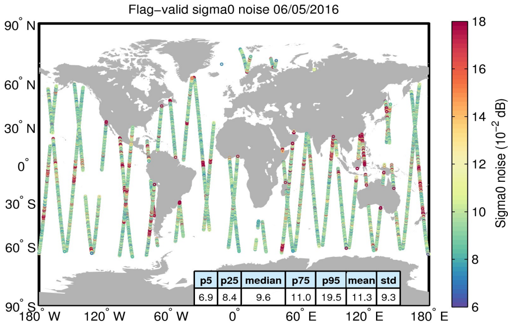
Figure 26. Geographical distribution of flag-valid 20-Hz sigma0 measurement noise over oceans and lakes for 06/05/2016. The statistical values shown in the table refer to the sigma0 noise and are calculated over all measurements shown in the figure.
