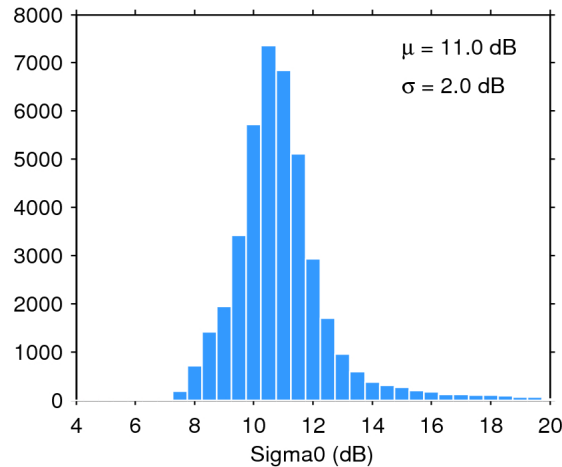
Figure 25. Histogram of flag-valid sigma0 over oceans and lakes for 06/05/2016. The mean ( \mu ) and standard deviation ( \sigma ) are also shown. Note that values outside [4 20] dB are excluded from the histogram for the sake of readability but not from the computation of \mu and \sigma .
