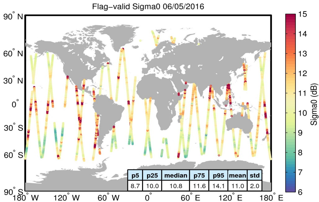
Figure 23. Geographical distribution of flag-valid sigma0 data over oceans and lakes for 06/05/2016. The statistical values shown in the table refer to the sigma0 in dB and are calculated over all measurements shown in the figure.
