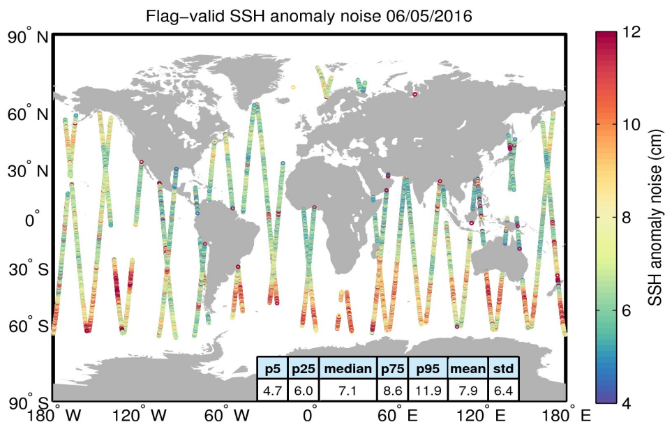
Figure 8. Geographical distribution of flag-valid 20-Hz SSH anomaly measurement noise over oceans and lakes for 06/05/2016. The statistical values shown in the table refer to the SSH anomaly noise and are calculated over all measurements shown in the figure.
