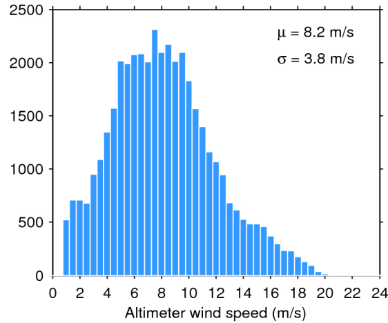
Figure 33. Histogram of flag-valid wind over oceans and lakes for 06/05/2016. The mean ( \mu ) and standard deviation ( \sigma ) are also shown. Note that values larger than 24 m/s are excluded from the histogram for the sake of readability but not from the computation of \mu and \sigma .
