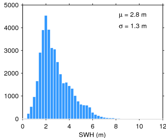
Figure 20. Histogram of science-valid SWH over oceans and lakes for 06/05/2016. The mean ( \mu ) and standard deviation ( \sigma ) are also shown. Note that values larger than 12 m are excluded from the histogram for the sake of readability but not from the computation of \mu and \sigma .
