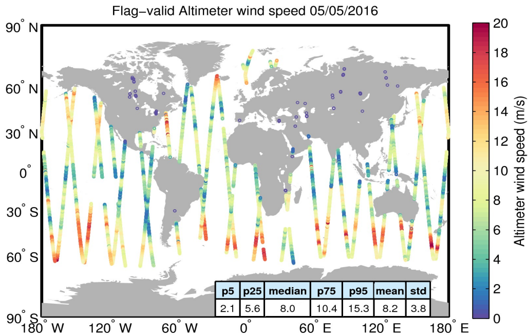
Figure 31. Geographical distribution of flag-valid wind data over oceans and lakes for 05/05/2016. The statistical values shown in the table refer to the wind in m/s and are calculated over all measurements shown in the figure.
