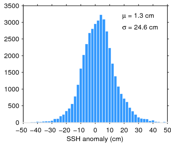
Figure 7. Histogram of flag-valid SSH anomaly over oceans and lakes for 05/05/2016. The mean ( \mu ) and standard deviation ( \sigma ) are also shown. Note that values outside [-50\ 50] cm are excluded from the histogram for the sake of readability but not from the computation of \mu and \sigma .
