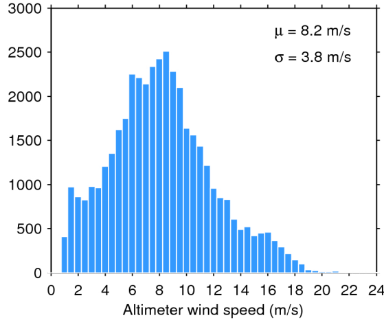
Figure 33. Histogram of flag-valid wind over oceans and lakes for 05/05/2016. The mean ( \mu ) and standard deviation ( \sigma ) are also shown. Note that values larger than 24 m/s are excluded from the histogram for the sake of readability but not from the computation of \mu and \sigma .
