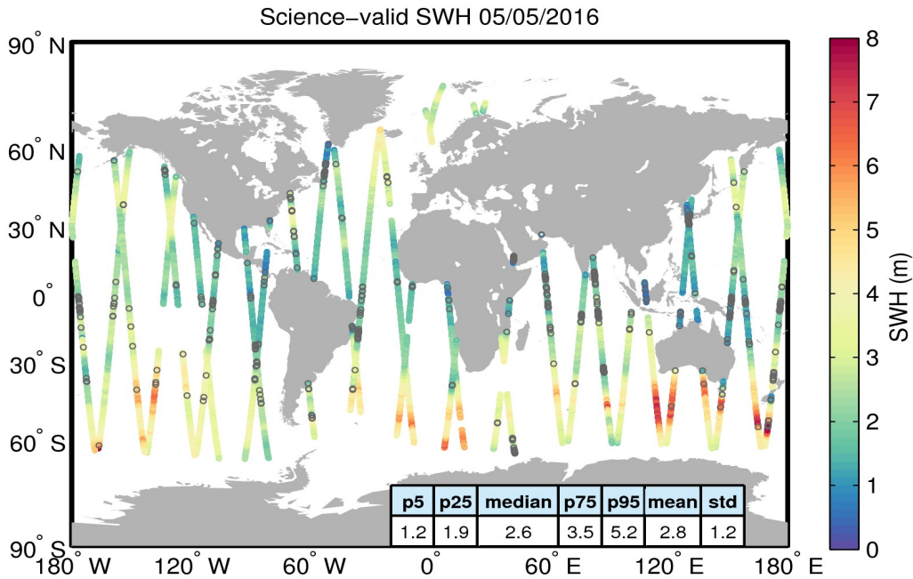
Figure 19. Geographical distribution of science-valid SWH data over oceans and lakes for 05/05/2016. The statistical values shown in the table refer to the SWH in m and are calculated over all measurements shown in the figure. Gray circles denote records that have been rejected based on the editing criteria described in Table 3.
