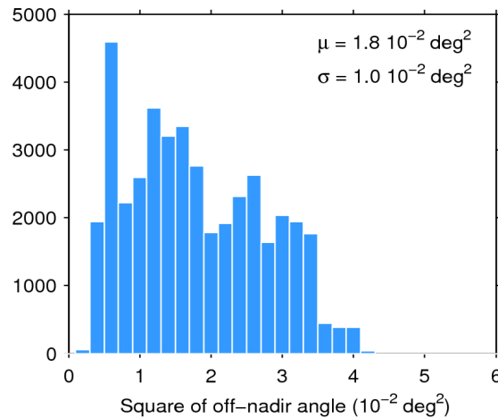
Figure 39. Histogram of flag-valid mispointing over oceans and lakes for 05/05/2016. The mean ( \mu ) and standard deviation ( \sigma ) are also shown. Note that values larger than 6 \cdot 10^{-2} \text{ deg}^2 are excluded from the histogram for the sake of readability but not from the computation of \mu and \sigma .
