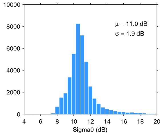
Figure 25. Histogram of flag-valid sigma0 over oceans and lakes for 05/05/2016. The mean ( \mu ) and standard deviation ( \sigma ) are also shown. Note that values outside [4 20] dB are excluded from the histogram for the sake of readability but not from the computation of \mu and \sigma .
