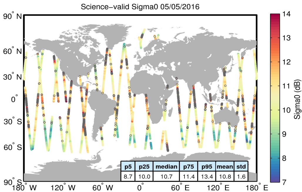
Figure 27. Geographical distribution of science-valid sigma0 data over oceans and lakes for 05/05/2016. The statistical values shown in the table refer to the sigma0 in dB and are calculated over all measurements shown in the figure. Gray circles denote records that have been rejected based on the editing criteria described in Table 4.
