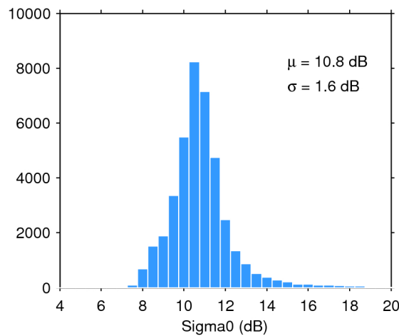
Figure 28. Histogram of science-valid sigma0 over oceans and lakes for 05/05/2016. The mean ( \mu ) and standard deviation ( \sigma ) are also shown. Note that values outside [4 20] dB are excluded from the histogram for the sake of readability but not from the computation of \mu and \sigma .
