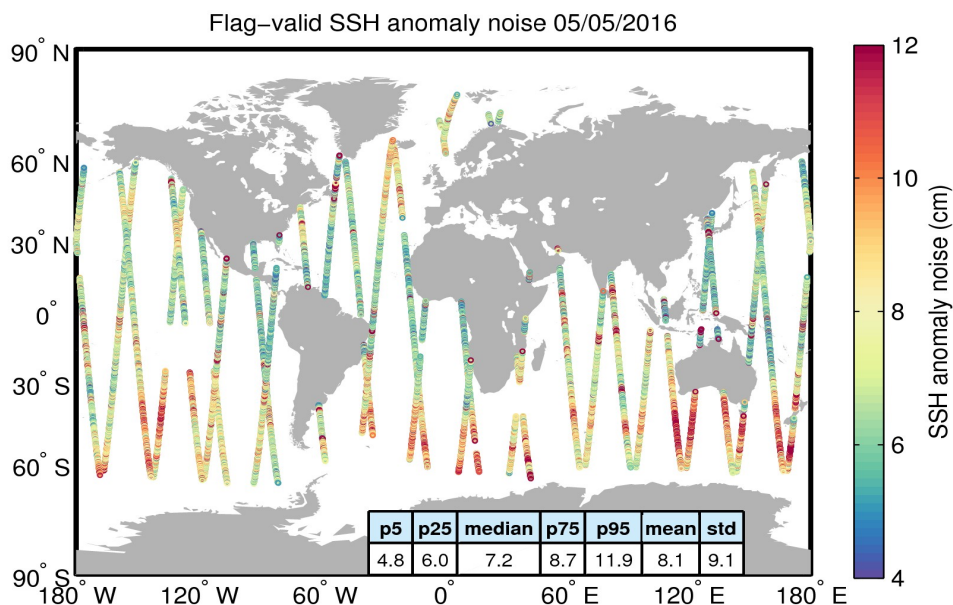
Figure 8. Geographical distribution of flag-valid 20-Hz SSH anomaly measurement noise over oceans and lakes for 05/05/2016. The statistical values shown in the table refer to the SSH anomaly noise and are calculated over all measurements shown in the figure.
