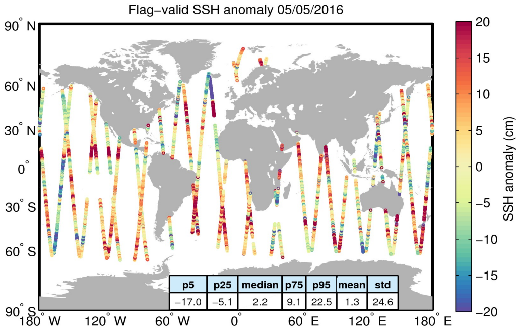
Figure 5. Geographical distribution of flag-valid 1-Hz SSH anomaly data over oceans and lakes for 05/05/2016. The statistical values shown in the table refer to the SSH anomaly in cm and are calculated over all measurements shown in the figure.
