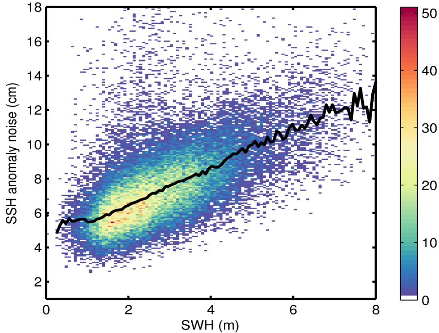
Figure 9. 2D histogram showing flag-valid SSH anomaly noise as a function of SWH for 05/05/2016. The black line denotes the median SSH anomaly noise as a function of SWH.
