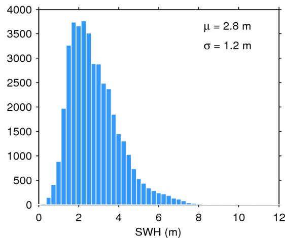
Figure 20. Histogram of science-valid SWH over oceans and lakes for 05/05/2016. The mean ( \mu ) and standard deviation ( \sigma ) are also shown. Note that values larger than 12 m are excluded from the histogram for the sake of readability but not from the computation of \mu and \sigma .
