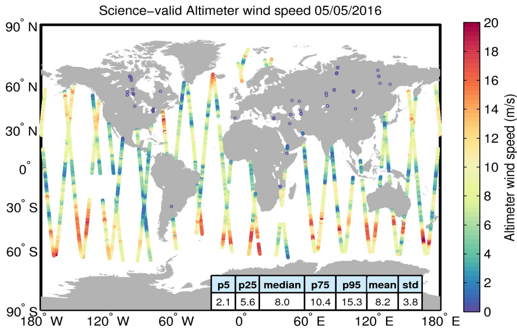
Figure 34. Geographical distribution of science-valid wind data over oceans and lakes for 05/05/2016. The statistical values shown in the table refer to the wind in m/s and are calculated over all measurements shown in the figure. Gray circles denote records that have been rejected based on the editing criteria described in Table 5.
