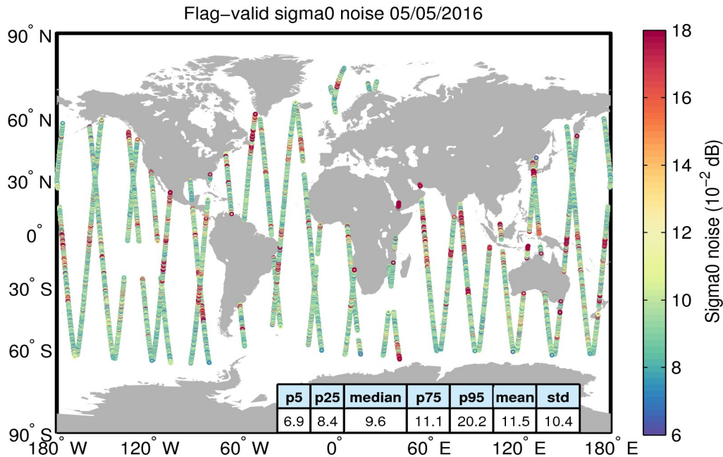
Figure 26. Geographical distribution of flag-valid 20-Hz sigma0 measurement noise over oceans and lakes for 05/05/2016. The statistical values shown in the table refer to the sigma0 noise and are calculated over all measurements shown in the figure.
