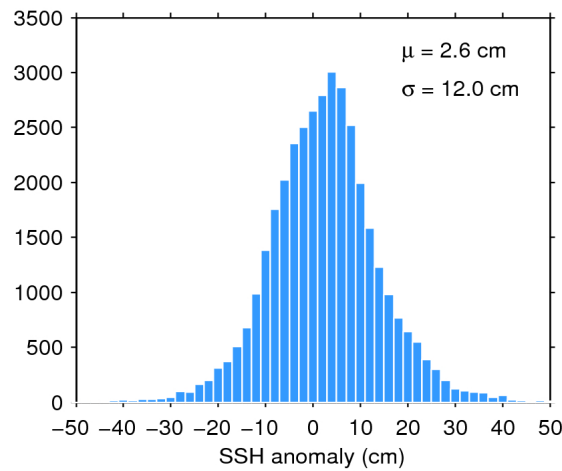
Figure 11. Histogram of science-valid SSH anomaly over oceans and lakes for 05/05/2016. The mean ( \mu ) and standard deviation ( \sigma ) are also shown. Note that values outside [-50 50] cm are excluded from the histogram for the sake of readability but not from the computation of \mu and \sigma .
