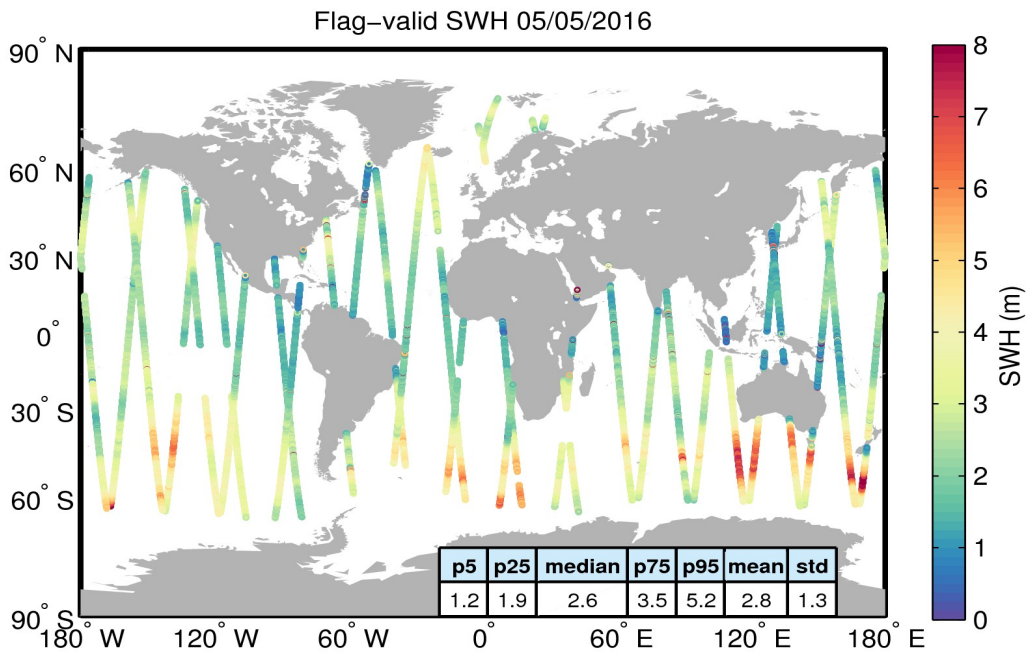
Figure 15. Geographical distribution of flag-valid SWH data over oceans and lakes for 05/05/2016. The statistical values shown in the table refer to the SWH in m and are calculated over all measurements shown in the figure.
