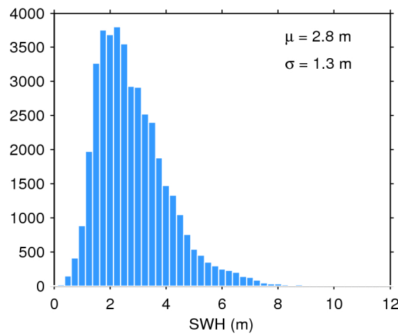
Figure 17. Histogram of flag-valid SWH over oceans and lakes for 05/05/2016. The mean ( \mu ) and standard deviation ( \sigma ) are also shown. Note that values larger than 12 m are excluded from the histogram for the sake of readability but not from the computation of \mu and \sigma .
