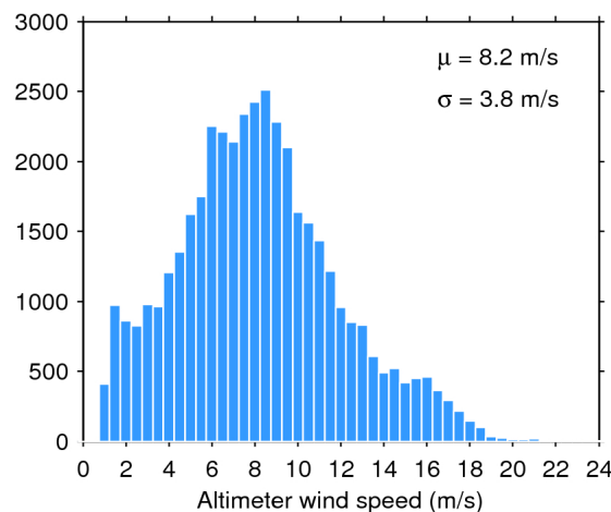
Figure 35. Histogram of science-valid wind over oceans and lakes for 05/05/2016. The mean ( \mu ) and standard deviation ( \sigma ) are also shown. Note that values larger than 24 m/s are excluded from the histogram for the sake of readability but not from the computation of \mu and \sigma .
