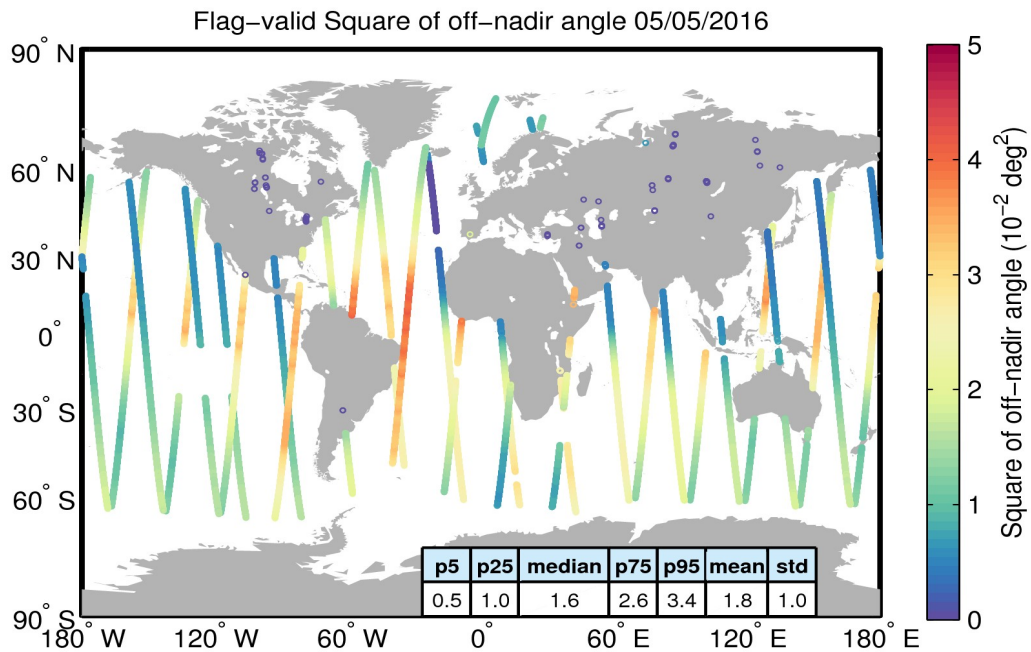
Figure 37. Geographical distribution of flag-valid mispointing data over oceans and lakes for 05/05/2016. The statistical values shown in the table refer to the mispointing in 10^{-2} \text{ deg}^2 and are calculated over all measurements shown in the figure.
