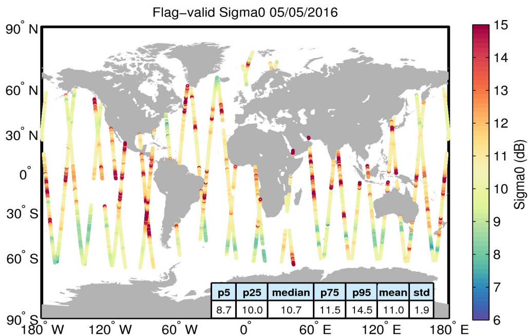
Figure 23. Geographical distribution of flag-valid sigma0 data over oceans and lakes for 05/05/2016. The statistical values shown in the table refer to the sigma0 in dB and are calculated over all measurements shown in the figure.
