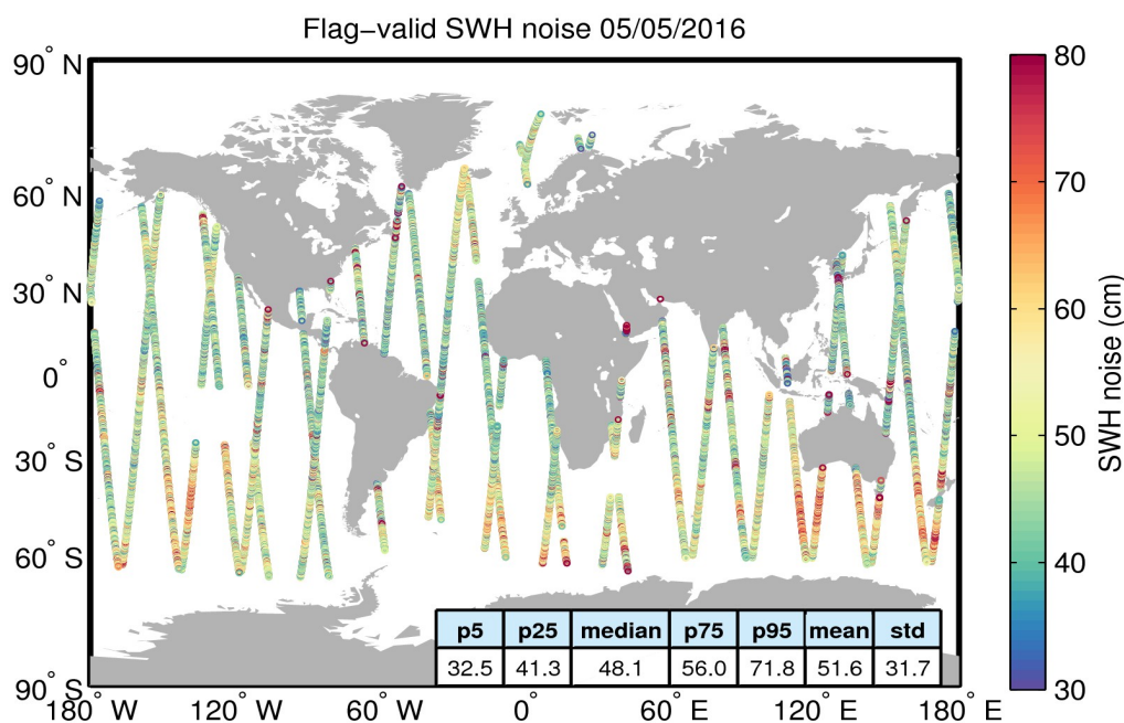
Figure 18. Geographical distribution of flag-valid 20-Hz SWH measurement noise over oceans and lakes for 05/05/2016. The statistical values shown in the table refer to the SWH noise and are calculated over all measurements shown in the figure.
