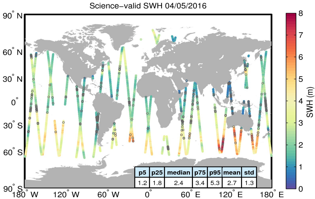
Figure 19. Geographical distribution of science-valid SWH data over oceans and lakes for 04/05/2016. The statistical values shown in the table refer to the SWH in m and are calculated over all measurements shown in the figure. Gray circles denote records that have been rejected based on the editing criteria described in Table 3.
