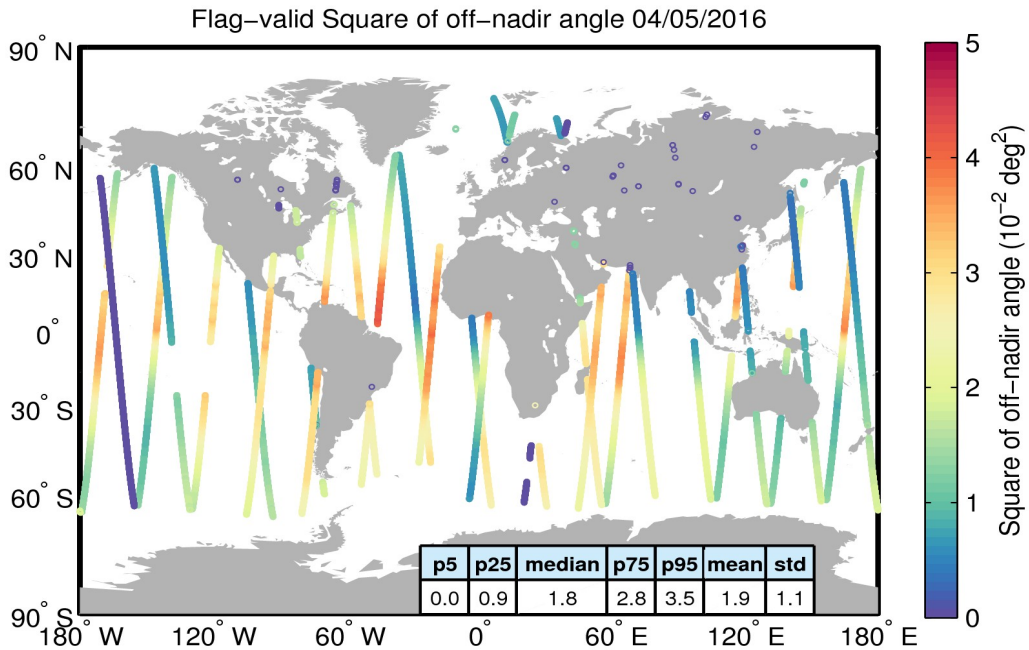
Figure 37. Geographical distribution of flag-valid mispointing data over oceans and lakes for 04/05/2016. The statistical values shown in the table refer to the mispointing in 10^{-2} \text{ deg}^2 and are calculated over all measurements shown in the figure.
