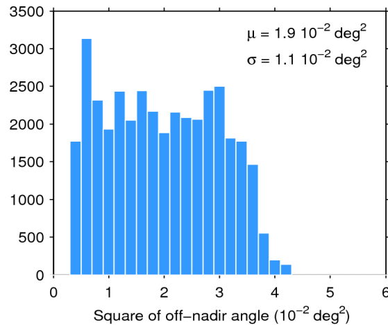
Figure 39. Histogram of flag-valid mispointing over oceans and lakes for 04/05/2016. The mean ( \mu ) and standard deviation ( \sigma ) are also shown. Note that values larger than 6 \cdot 10^{-2} \text{ deg}^2 are excluded from the histogram for the sake of readability but not from the computation of \mu and \sigma .
