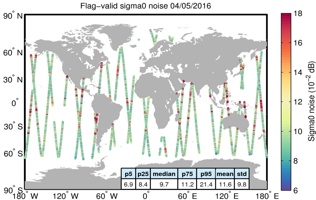
Figure 26. Geographical distribution of flag-valid 20-Hz sigma0 measurement noise over oceans and lakes for 04/05/2016. The statistical values shown in the table refer to the sigma0 noise and are calculated over all measurements shown in the figure.
