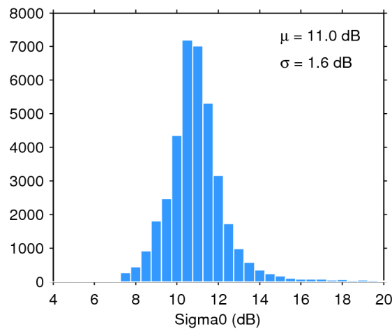
Figure 28. Histogram of science-valid sigma0 over oceans and lakes for 04/05/2016. The mean ( \mu ) and standard deviation ( \sigma ) are also shown. Note that values outside [4 20] dB are excluded from the histogram for the sake of readability but not from the computation of \mu and \sigma .
