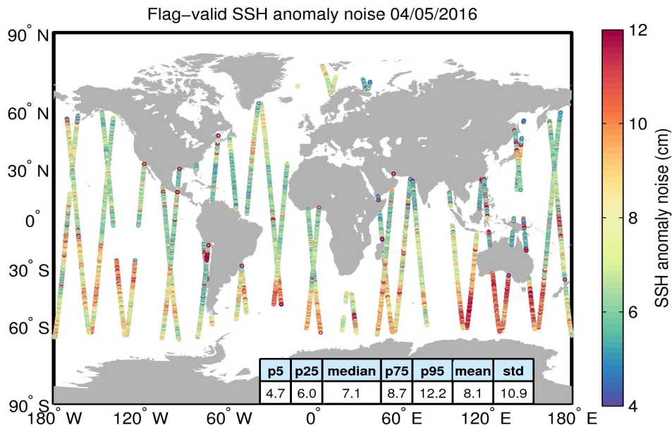
Figure 8. Geographical distribution of flag-valid 20-Hz SSH anomaly measurement noise over oceans and lakes for 04/05/2016. The statistical values shown in the table refer to the SSH anomaly noise and are calculated over all measurements shown in the figure.
