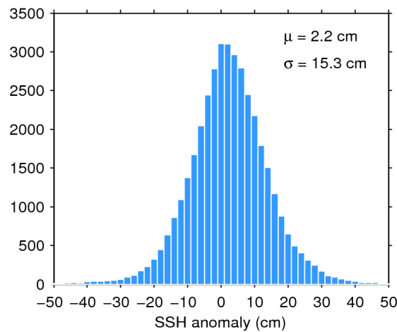
Figure 7. Histogram of flag-valid SSH anomaly over oceans and lakes for 04/05/2016. The mean ( \mu ) and standard deviation ( \sigma ) are also shown. Note that values outside [-50\ 50] cm are excluded from the histogram for the sake of readability but not from the computation of \mu and \sigma .
