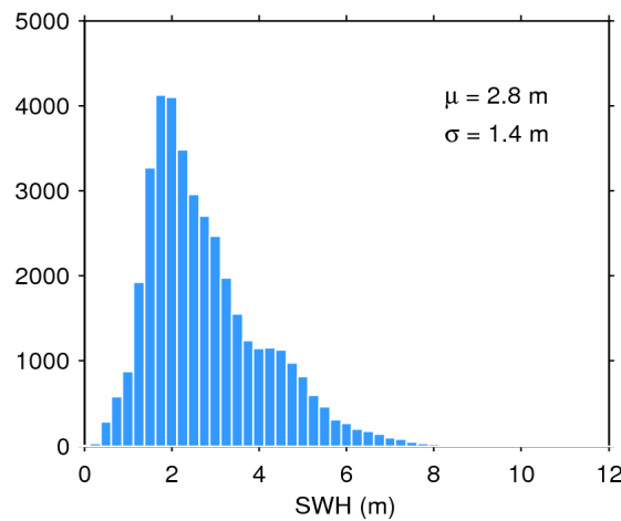
Figure 17. Histogram of flag-valid SWH over oceans and lakes for 04/05/2016. The mean ( \mu ) and standard deviation ( \sigma ) are also shown. Note that values larger than 12 m are excluded from the histogram for the sake of readability but not from the computation of \mu and \sigma .
