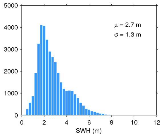
Figure 20. Histogram of science-valid SWH over oceans and lakes for 04/05/2016. The mean ( \mu ) and standard deviation ( \sigma ) are also shown. Note that values larger than 12 m are excluded from the histogram for the sake of readability but not from the computation of \mu and \sigma .
