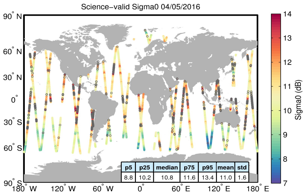
Figure 27. Geographical distribution of science-valid sigma0 data over oceans and lakes for 04/05/2016. The statistical values shown in the table refer to the sigma0 in dB and are calculated over all measurements shown in the figure. Gray circles denote records that have been rejected based on the editing criteria described in Table 4.
