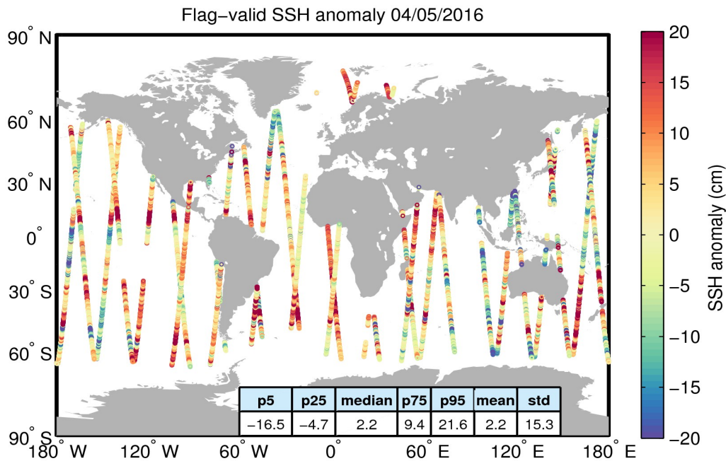
Figure 5. Geographical distribution of flag-valid 1-Hz SSH anomaly data over oceans and lakes for 04/05/2016. The statistical values shown in the table refer to the SSH anomaly in cm and are calculated over all measurements shown in the figure.
