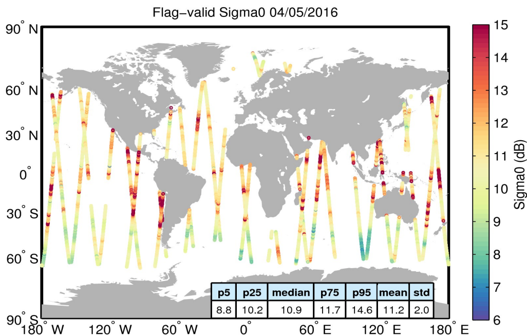
Figure 23. Geographical distribution of flag-valid sigma0 data over oceans and lakes for 04/05/2016. The statistical values shown in the table refer to the sigma0 in dB and are calculated over all measurements shown in the figure.
