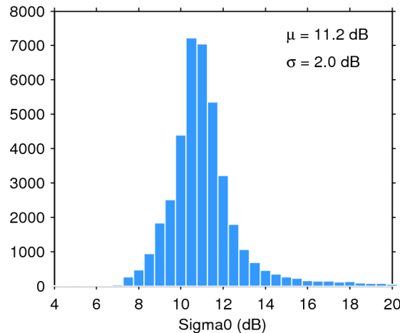
Figure 25. Histogram of flag-valid sigma0 over oceans and lakes for 04/05/2016. The mean ( \mu ) and standard deviation ( \sigma ) are also shown. Note that values outside [4 20] dB are excluded from the histogram for the sake of readability but not from the computation of \mu and \sigma .
