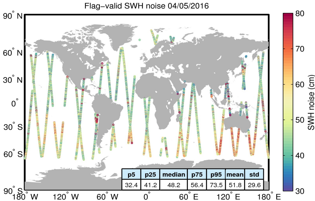
Figure 18. Geographical distribution of flag-valid 20-Hz SWH measurement noise over oceans and lakes for 04/05/2016. The statistical values shown in the table refer to the SWH noise and are calculated over all measurements shown in the figure.
