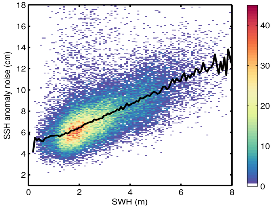
Figure 9. 2D histogram showing flag-valid SSH anomaly noise as a function of SWH for 04/05/2016. The black line denotes the median SSH anomaly noise as a function of SWH.
