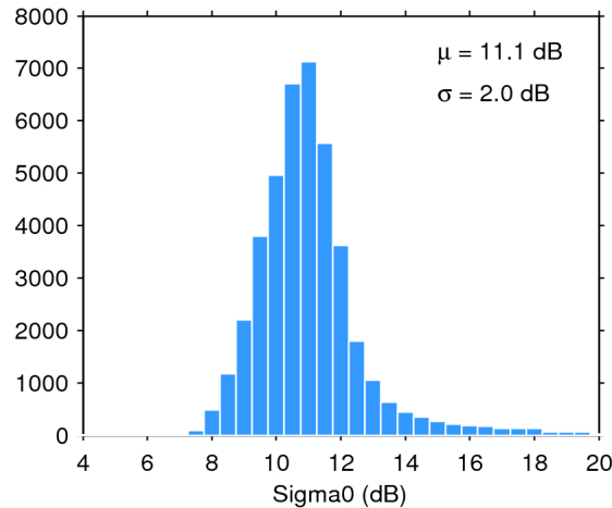
Figure 25. Histogram of flag-valid sigma0 over oceans and lakes for 03/05/2016. The mean ( \mu ) and standard deviation ( \sigma ) are also shown. Note that values outside [4 20] dB are excluded from the histogram for the sake of readability but not from the computation of \mu and \sigma .
