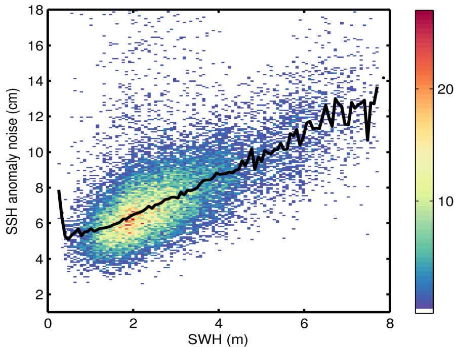
Figure 9. 2D histogram showing flag-valid SSH anomaly noise as a function of SWH for 03/05/2016. The black line denotes the median SSH anomaly noise as a function of SWH.
