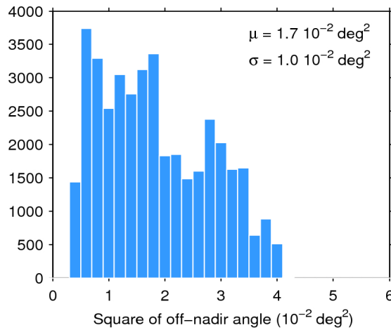
Figure 39. Histogram of flag-valid mispointing over oceans and lakes for 03/05/2016. The mean ( \mu ) and standard deviation ( \sigma ) are also shown. Note that values larger than 6 \cdot 10^{-2} \text{ deg}^2 are excluded from the histogram for the sake of readability but not from the computation of \mu and \sigma .
