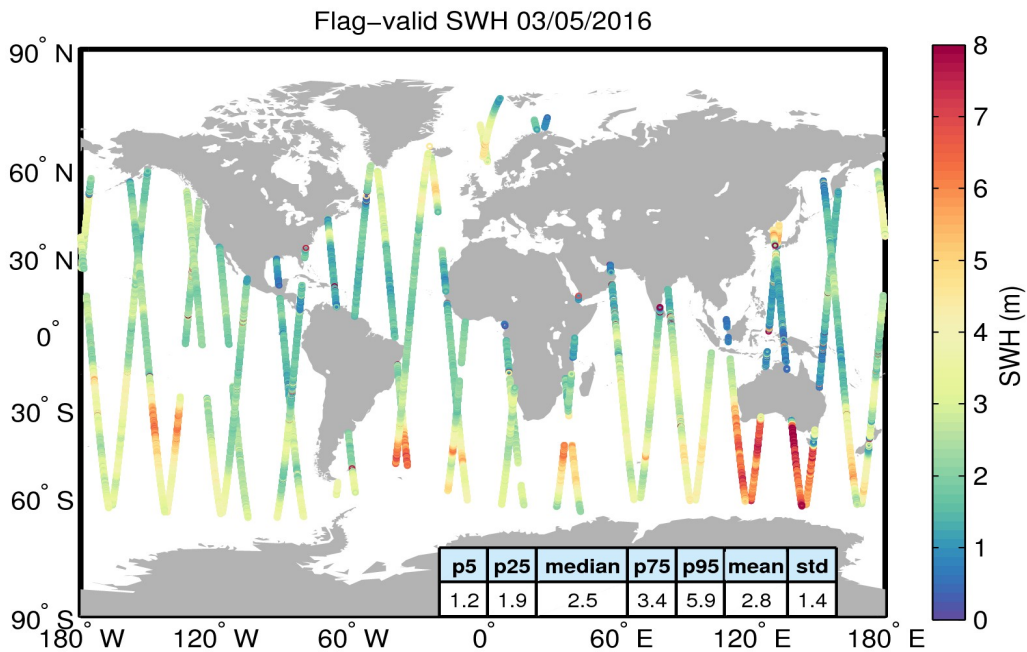
Figure 15. Geographical distribution of flag-valid SWH data over oceans and lakes for 03/05/2016. The statistical values shown in the table refer to the SWH in m and are calculated over all measurements shown in the figure.
