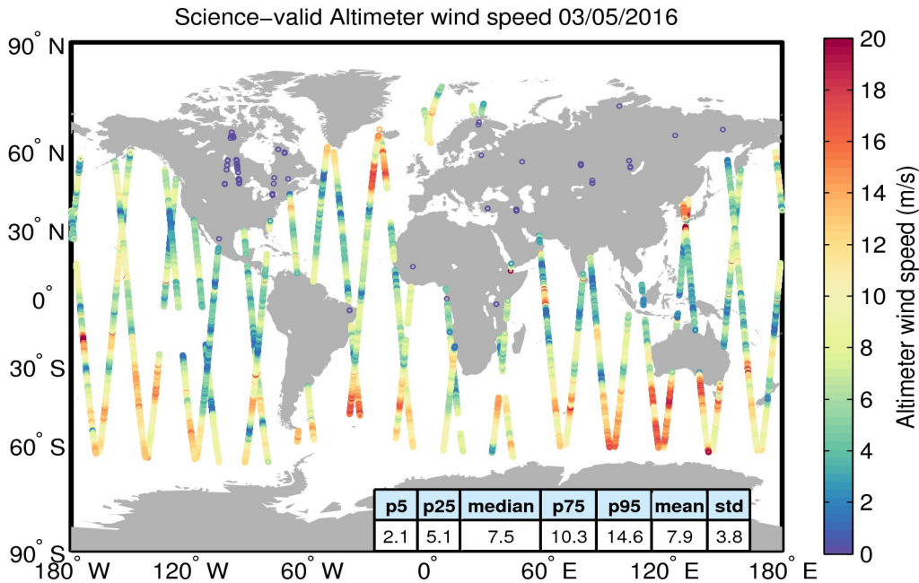
Figure 34. Geographical distribution of science-valid wind data over oceans and lakes for 03/05/2016. The statistical values shown in the table refer to the wind in m/s and are calculated over all measurements shown in the figure. Gray circles denote records that have been rejected based on the editing criteria described in Table 5.
