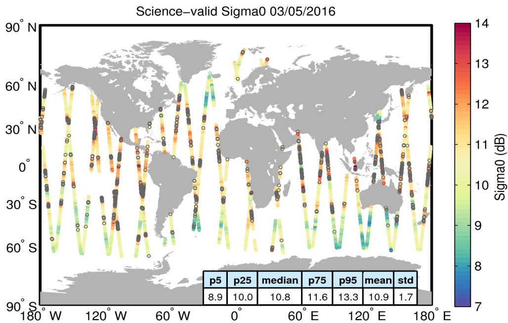
Figure 27. Geographical distribution of science-valid sigma0 data over oceans and lakes for 03/05/2016. The statistical values shown in the table refer to the sigma0 in dB and are calculated over all measurements shown in the figure. Gray circles denote records that have been rejected based on the editing criteria described in Table 4.
