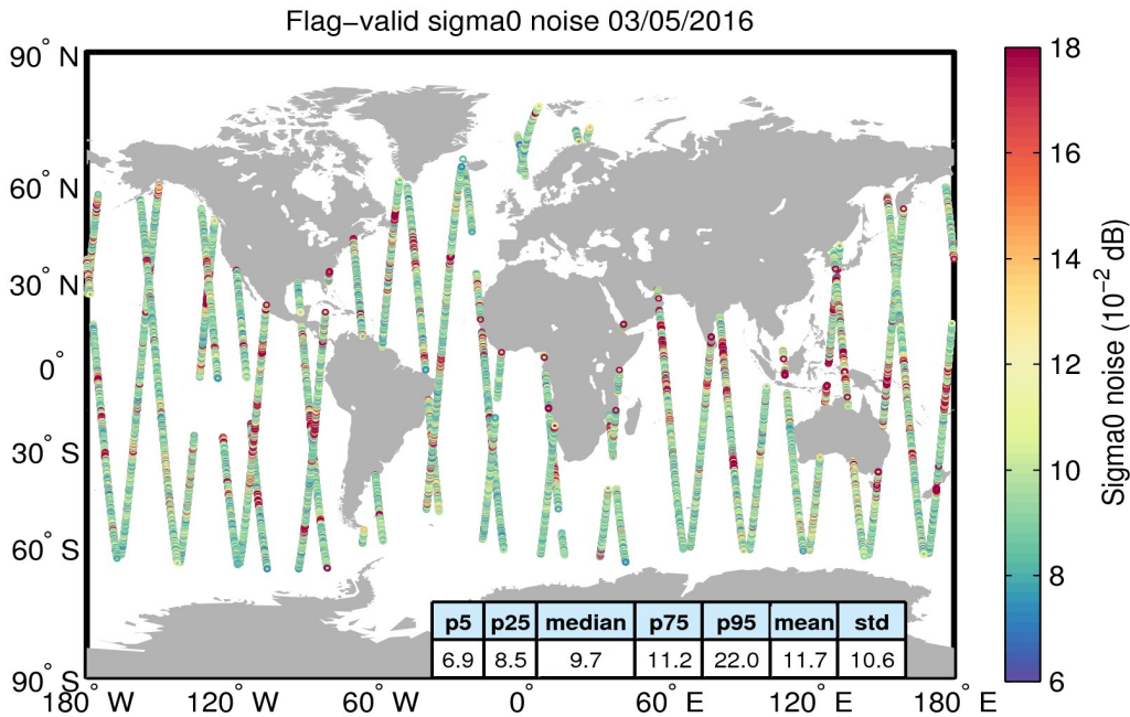
Figure 26. Geographical distribution of flag-valid 20-Hz sigma0 measurement noise over oceans and lakes for 03/05/2016. The statistical values shown in the table refer to the sigma0 noise and are calculated over all measurements shown in the figure.
