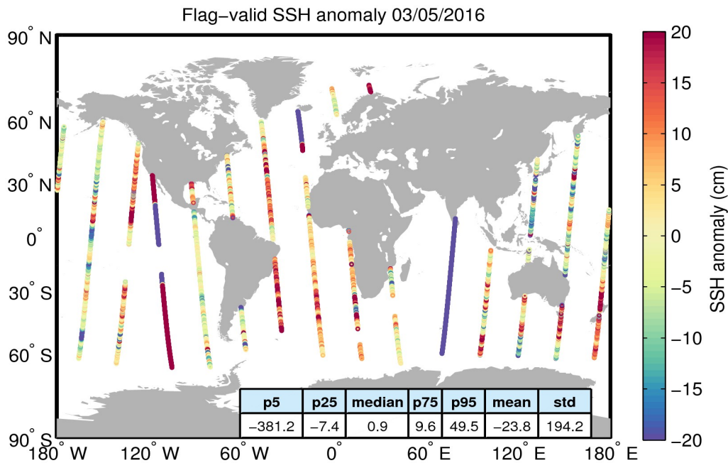
Figure 5. Geographical distribution of flag-valid 1-Hz SSH anomaly data over oceans and lakes for 03/05/2016. The statistical values shown in the table refer to the SSH anomaly in cm and are calculated over all measurements shown in the figure.
