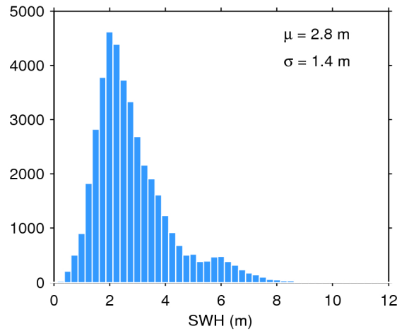
Figure 17. Histogram of flag-valid SWH over oceans and lakes for 03/05/2016. The mean ( \mu ) and standard deviation ( \sigma ) are also shown. Note that values larger than 12 m are excluded from the histogram for the sake of readability but not from the computation of \mu and \sigma .
