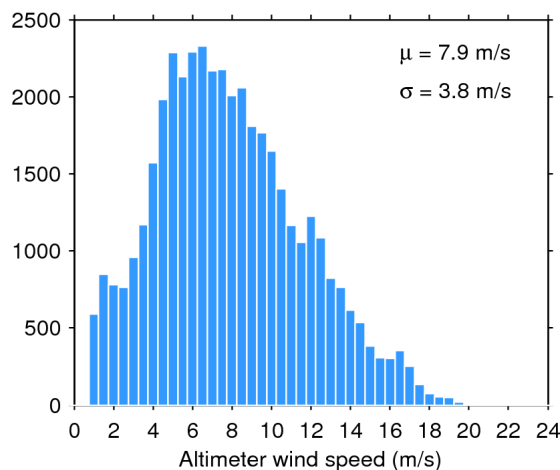
Figure 35. Histogram of science-valid wind over oceans and lakes for 03/05/2016. The mean ( \mu ) and standard deviation ( \sigma ) are also shown. Note that values larger than 24 m/s are excluded from the histogram for the sake of readability but not from the computation of \mu and \sigma .
