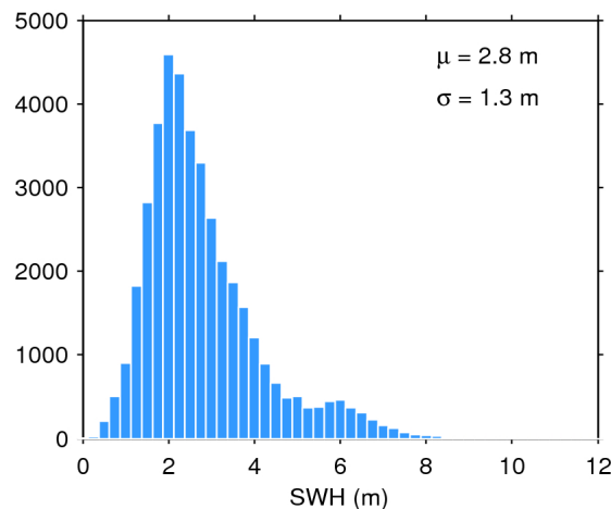
Figure 20. Histogram of science-valid SWH over oceans and lakes for 03/05/2016. The mean ( \mu ) and standard deviation ( \sigma ) are also shown. Note that values larger than 12 m are excluded from the histogram for the sake of readability but not from the computation of \mu and \sigma .
