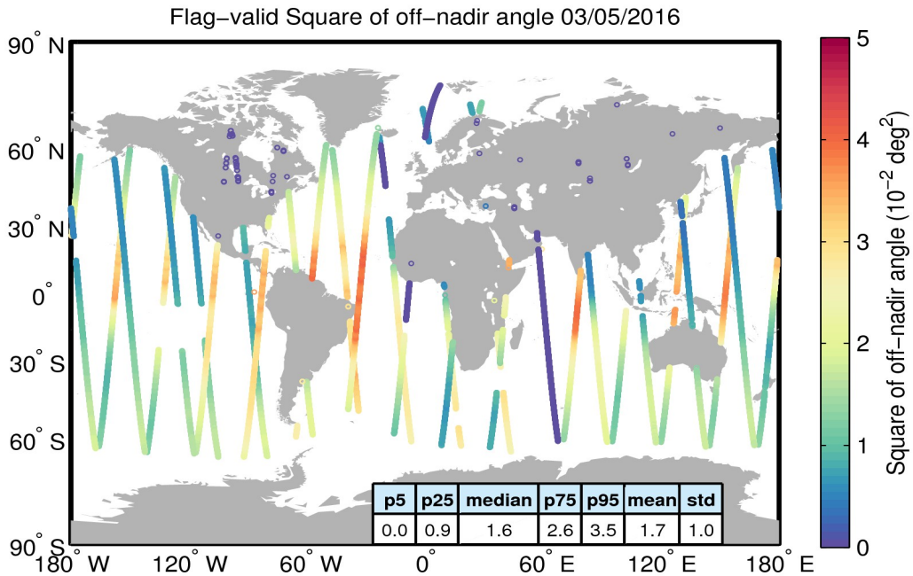
Figure 37. Geographical distribution of flag-valid mispointing data over oceans and lakes for 03/05/2016. The statistical values shown in the table refer to the mispointing in 10^{-2} \text{ deg}^2 and are calculated over all measurements shown in the figure.
