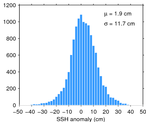
Figure 11. Histogram of science-valid SSH anomaly over oceans and lakes for 03/05/2016. The mean ( \mu ) and standard deviation ( \sigma ) are also shown. Note that values outside [-50 50] cm are excluded from the histogram for the sake of readability but not from the computation of \mu and \sigma .
