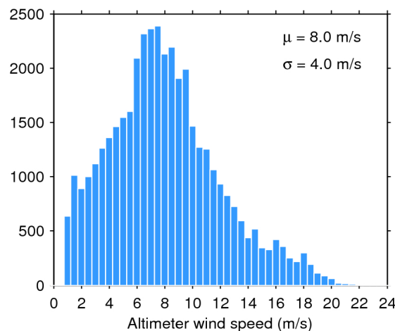
Figure 35. Histogram of science-valid wind over oceans and lakes for 02/05/2016. The mean ( \mu ) and standard deviation ( \sigma ) are also shown. Note that values larger than 24 m/s are excluded from the histogram for the sake of readability but not from the computation of \mu and \sigma .
