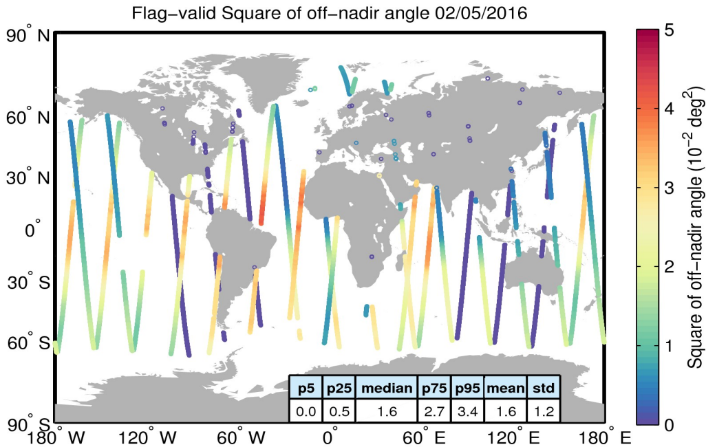
Figure 37. Geographical distribution of flag-valid mispointing data over oceans and lakes for 02/05/2016. The statistical values shown in the table refer to the mispointing in 10^{-2} \text{ deg}^2 and are calculated over all measurements shown in the figure.
