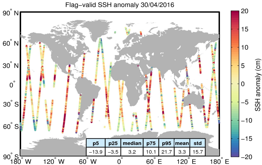
Figure 5. Geographical distribution of flag-valid 1-Hz SSH anomaly data over oceans and lakes for 30/04/2016. The statistical values shown in the table refer to the SSH anomaly in cm and are calculated over all measurements shown in the figure.
