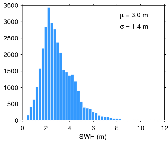
Figure 17. Histogram of flag-valid SWH over oceans and lakes for 30/04/2016. The mean ( \mu ) and standard deviation ( \sigma ) are also shown. Note that values larger than 12 m are excluded from the histogram for the sake of readability but not from the computation of \mu and \sigma .
