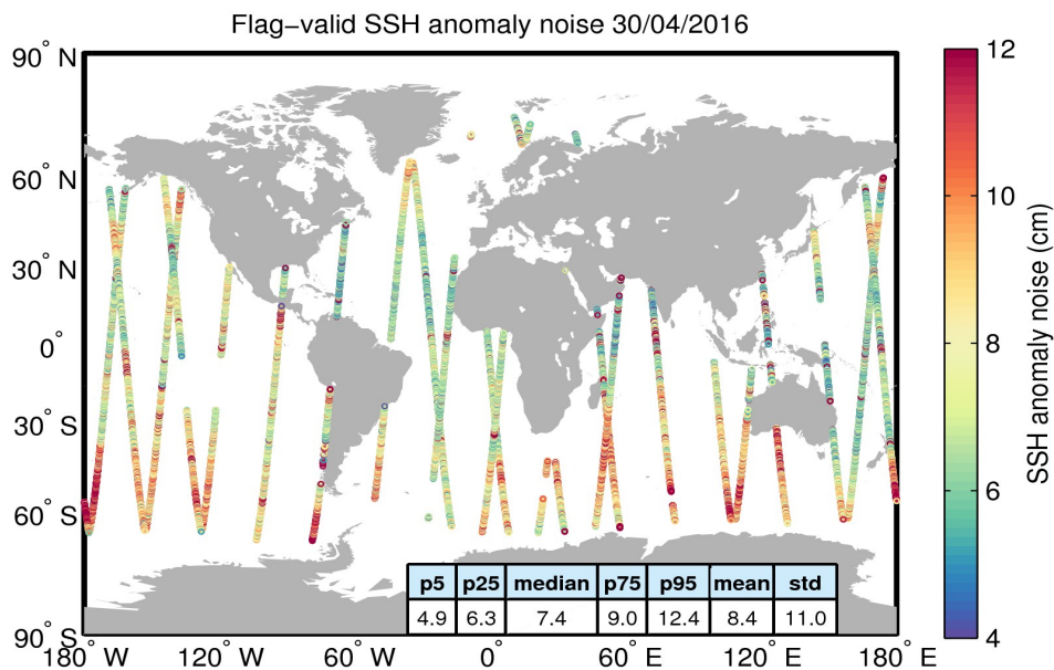
Figure 8. Geographical distribution of flag-valid 20-Hz SSH anomaly measurement noise over oceans and lakes for 30/04/2016. The statistical values shown in the table refer to the SSH anomaly noise and are calculated over all measurements shown in the figure.
