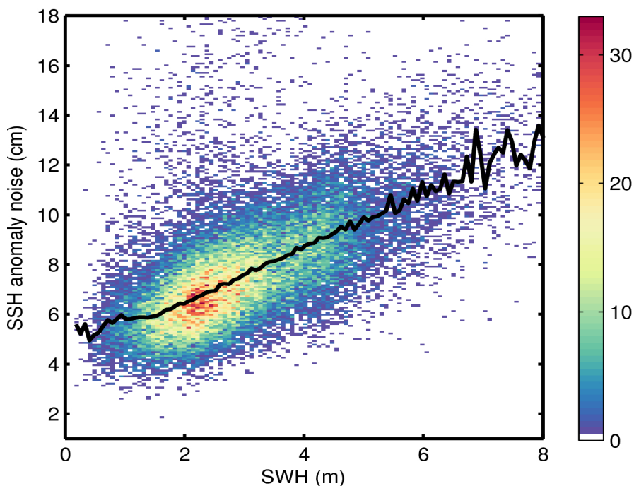
Figure 9. 2D histogram showing flag-valid SSH anomaly noise as a function of SWH for 30/04/2016. The black line denotes the median SSH anomaly noise as a function of SWH.
