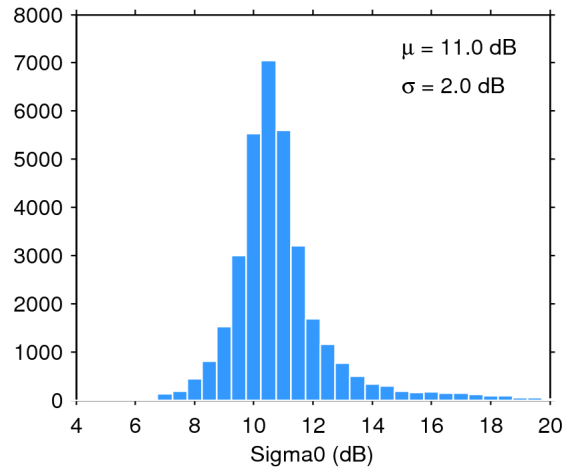
Figure 25. Histogram of flag-valid sigma0 over oceans and lakes for 30/04/2016. The mean ( \mu ) and standard deviation ( \sigma ) are also shown. Note that values outside [4 20] dB are excluded from the histogram for the sake of readability but not from the computation of \mu and \sigma .
