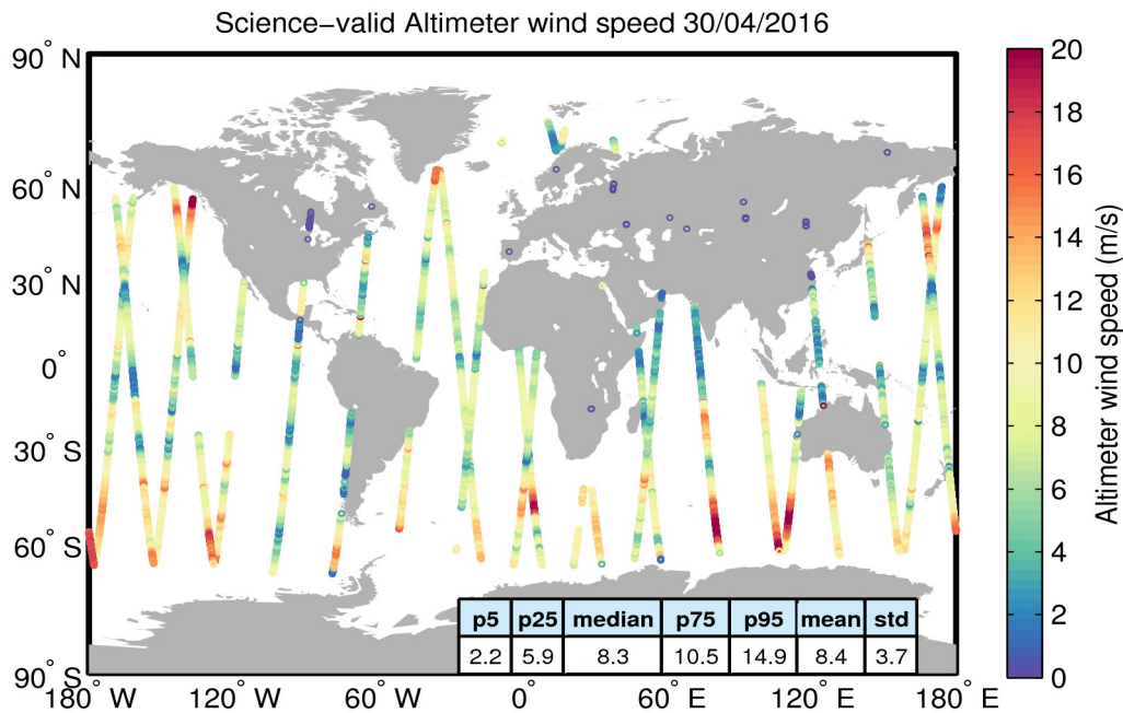
Figure 34. Geographical distribution of science-valid wind data over oceans and lakes for 30/04/2016. The statistical values shown in the table refer to the wind in m/s and are calculated over all measurements shown in the figure. Gray circles denote records that have been rejected based on the editing criteria described in Table 5.
