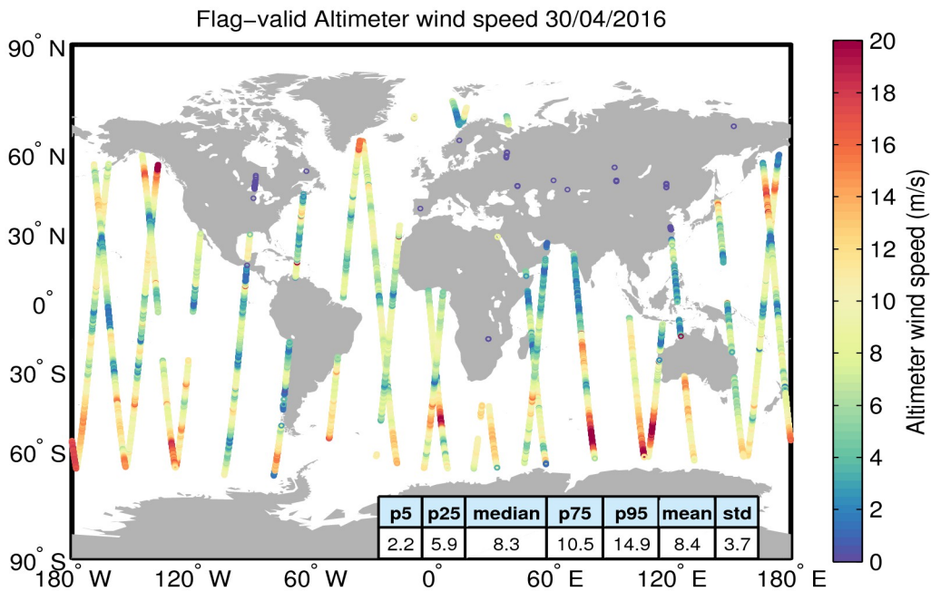
Figure 31. Geographical distribution of flag-valid wind data over oceans and lakes for 30/04/2016. The statistical values shown in the table refer to the wind in m/s and are calculated over all measurements shown in the figure.
