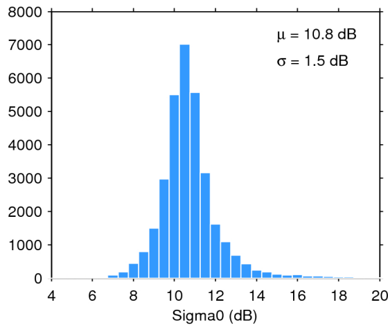
Figure 28. Histogram of science-valid sigma0 over oceans and lakes for 30/04/2016. The mean ( \mu ) and standard deviation ( \sigma ) are also shown. Note that values outside [4 20] dB are excluded from the histogram for the sake of readability but not from the computation of \mu and \sigma .
