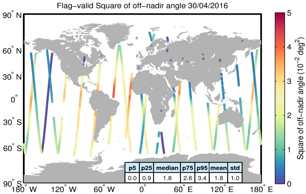
Figure 37. Geographical distribution of flag-valid mispointing data over oceans and lakes for 30/04/2016. The statistical values shown in the table refer to the mispointing in 10^{-2} deg 2 and are calculated over all measurements shown in the figure.
