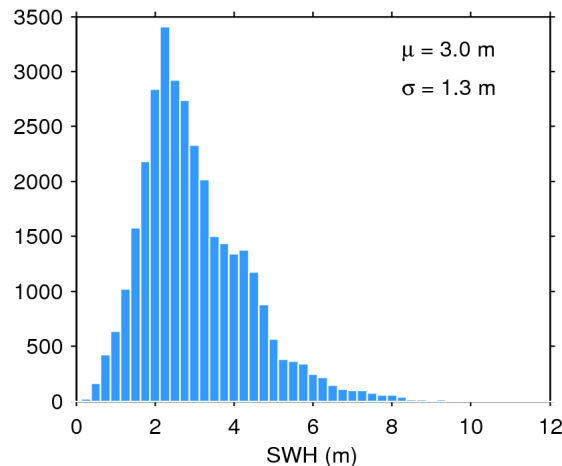
Figure 20. Histogram of science-valid SWH over oceans and lakes for 30/04/2016. The mean ( \mu ) and standard deviation ( \sigma ) are also shown. Note that values larger than 12 m are excluded from the histogram for the sake of readability but not from the computation of \mu and \sigma .
