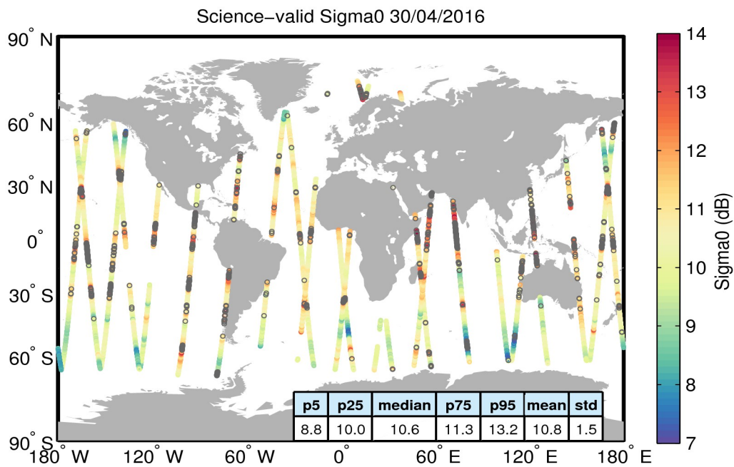
Figure 27. Geographical distribution of science-valid sigma0 data over oceans and lakes for 30/04/2016. The statistical values shown in the table refer to the sigma0 in dB and are calculated over all measurements shown in the figure. Gray circles denote records that have been rejected based on the editing criteria described in Table 4.
