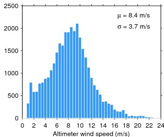
Figure 35. Histogram of science-valid wind over oceans and lakes for 30/04/2016. The mean ( \mu ) and standard deviation ( \sigma ) are also shown. Note that values larger than 24 m/s are excluded from the histogram for the sake of readability but not from the computation of \mu and \sigma .
