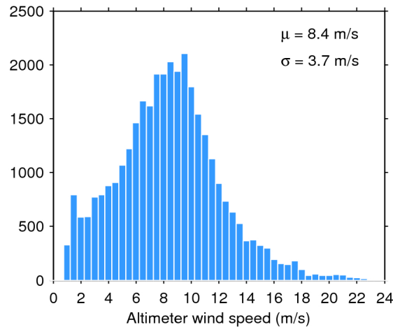
Figure 33. Histogram of flag-valid wind over oceans and lakes for 30/04/2016. The mean ( \mu ) and standard deviation ( \sigma ) are also shown. Note that values larger than 24 m/s are excluded from the histogram for the sake of readability but not from the computation of \mu and \sigma .
