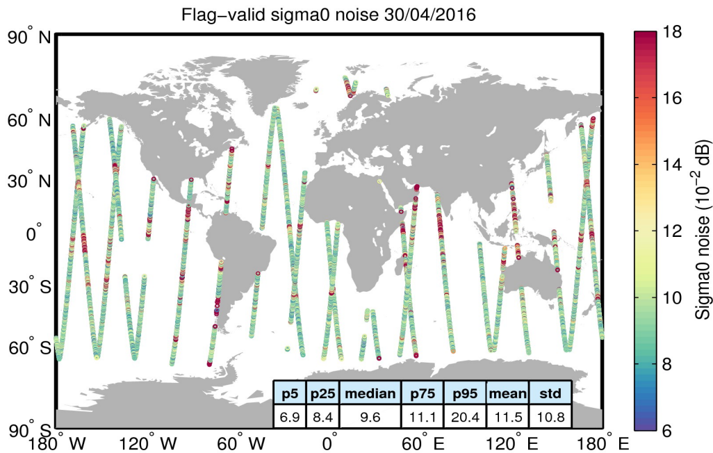
Figure 26. Geographical distribution of flag-valid 20-Hz sigma0 measurement noise over oceans and lakes for 30/04/2016. The statistical values shown in the table refer to the sigma0 noise and are calculated over all measurements shown in the figure.
