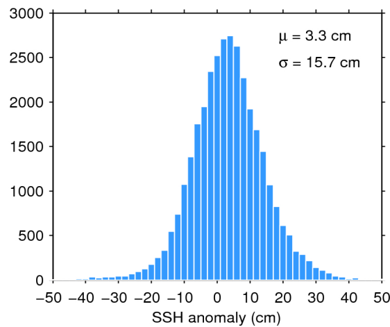
Figure 7. Histogram of flag-valid SSH anomaly over oceans and lakes for 30/04/2016. The mean ( \mu ) and standard deviation ( \sigma ) are also shown. Note that values outside [-50 50] cm are excluded from the histogram for the sake of readability but not from the computation of \mu and \sigma .
