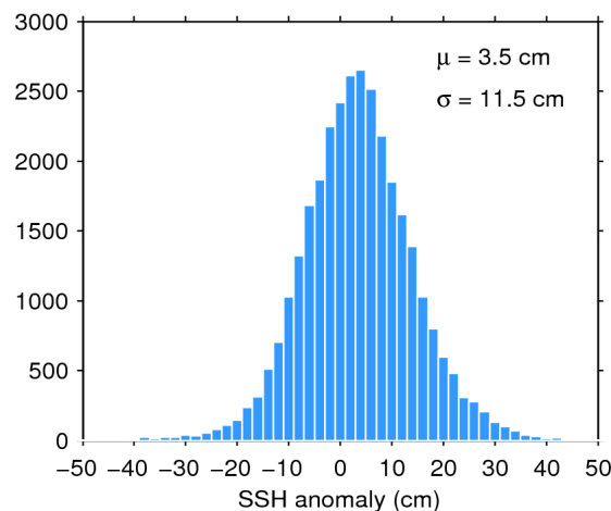
Figure 11. Histogram of science-valid SSH anomaly over oceans and lakes for 30/04/2016. The mean ( \mu ) and standard deviation ( \sigma ) are also shown. Note that values outside [-50 50] cm are excluded from the histogram for the sake of readability but not from the computation of \mu and \sigma .
