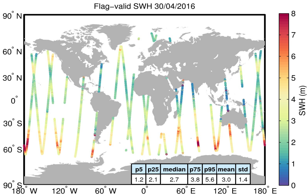
Figure 15. Geographical distribution of flag-valid SWH data over oceans and lakes for 30/04/2016. The statistical values shown in the table refer to the SWH in m and are calculated over all measurements shown in the figure.
