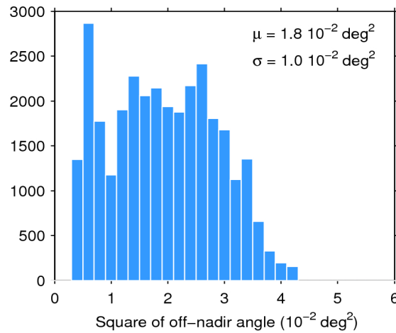
Figure 39. Histogram of flag-valid mispointing over oceans and lakes for 30/04/2016. The mean ( \mu ) and standard deviation ( \sigma ) are also shown. Note that values larger than 6 \cdot 10^{-2} \text{ deg}^2 are excluded from the histogram for the sake of readability but not from the computation of \mu and \sigma .
