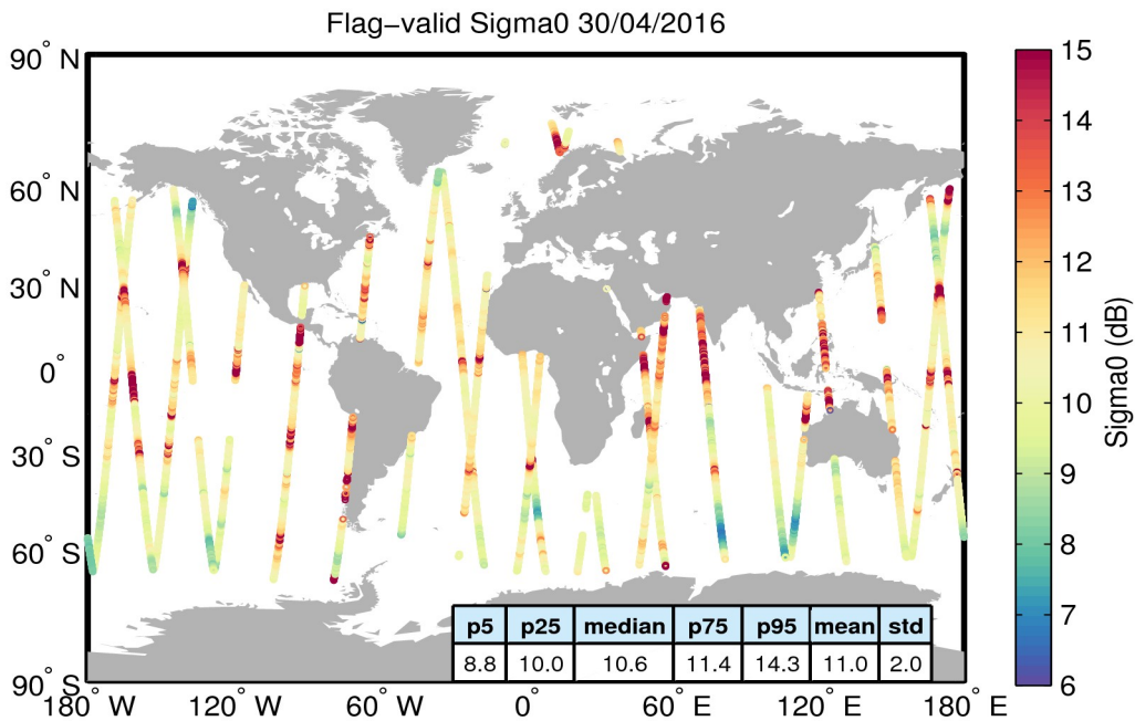
Figure 23. Geographical distribution of flag-valid sigma0 data over oceans and lakes for 30/04/2016. The statistical values shown in the table refer to the sigma0 in dB and are calculated over all measurements shown in the figure.
