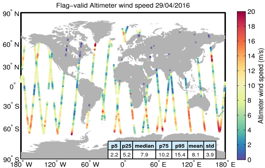
Figure 31. Geographical distribution of flag-valid wind data over oceans and lakes for 29/04/2016. The statistical values shown in the table refer to the wind in m/s and are calculated over all measurements shown in the figure.
