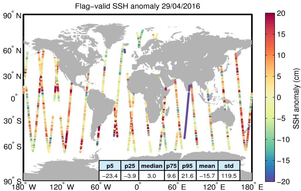
Figure 5. Geographical distribution of flag-valid 1-Hz SSH anomaly data over oceans and lakes for 29/04/2016. The statistical values shown in the table refer to the SSH anomaly in cm and are calculated over all measurements shown in the figure.
