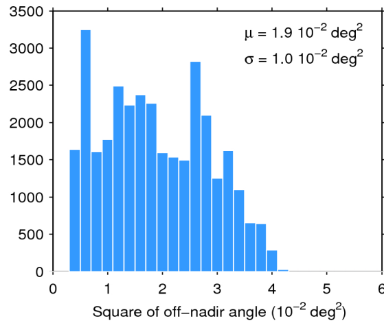
Figure 39. Histogram of flag-valid mispointing over oceans and lakes for 29/04/2016. The mean ( \mu ) and standard deviation ( \sigma ) are also shown. Note that values larger than 6 \cdot 10^{-2} \text{ deg}^2 are excluded from the histogram for the sake of readability but not from the computation of \mu and \sigma .
