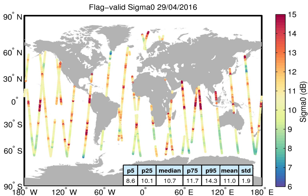
Figure 23. Geographical distribution of flag-valid sigma0 data over oceans and lakes for 29/04/2016. The statistical values shown in the table refer to the sigma0 in dB and are calculated over all measurements shown in the figure.
