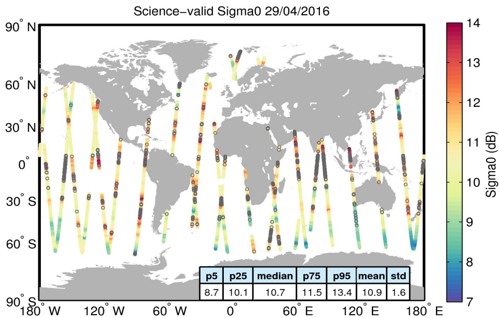
Figure 27. Geographical distribution of science-valid sigma0 data over oceans and lakes for 29/04/2016. The statistical values shown in the table refer to the sigma0 in dB and are calculated over all measurements shown in the figure. Gray circles denote records that have been rejected based on the editing criteria described in Table 4.
