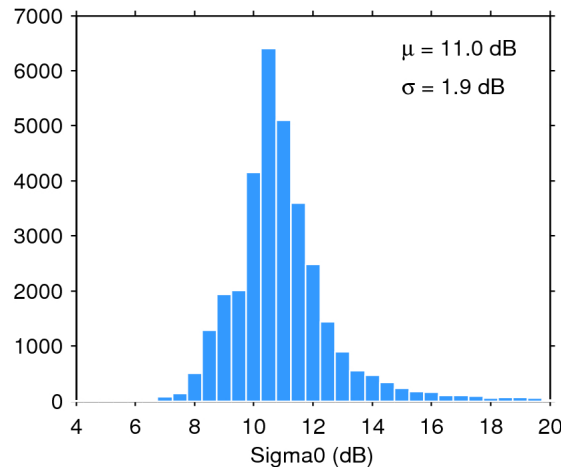
Figure 25. Histogram of flag-valid sigma0 over oceans and lakes for 29/04/2016. The mean ( \mu ) and standard deviation ( \sigma ) are also shown. Note that values outside [4 20] dB are excluded from the histogram for the sake of readability but not from the computation of \mu and \sigma .
