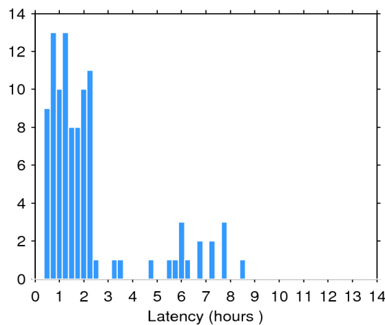
Figure 2. Histogram of the data latency for 29/04/2016. The y-axis denotes the number of files that are made available with a delay of x-hours with respect to the mean time of the records stored in the file.
