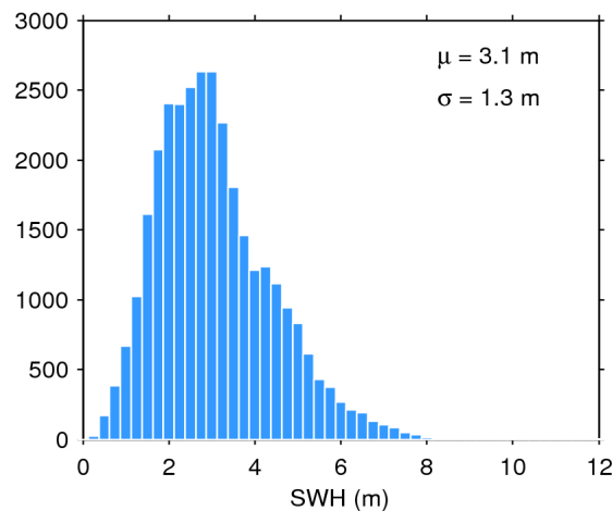
Figure 20. Histogram of science-valid SWH over oceans and lakes for 29/04/2016. The mean ( \mu ) and standard deviation ( \sigma ) are also shown. Note that values larger than 12 m are excluded from the histogram for the sake of readability but not from the computation of \mu and \sigma .
