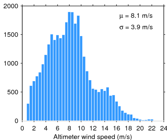
Figure 35. Histogram of science-valid wind over oceans and lakes for 29/04/2016. The mean ( \mu ) and standard deviation ( \sigma ) are also shown. Note that values larger than 24 m/s are excluded from the histogram for the sake of readability but not from the computation of \mu and \sigma .
