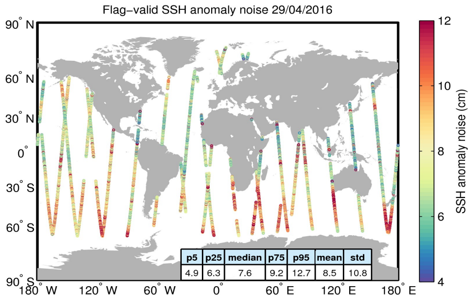
Figure 8. Geographical distribution of flag-valid 20-Hz SSH anomaly measurement noise over oceans and lakes for 29/04/2016. The statistical values shown in the table refer to the SSH anomaly noise and are calculated over all measurements shown in the figure.
