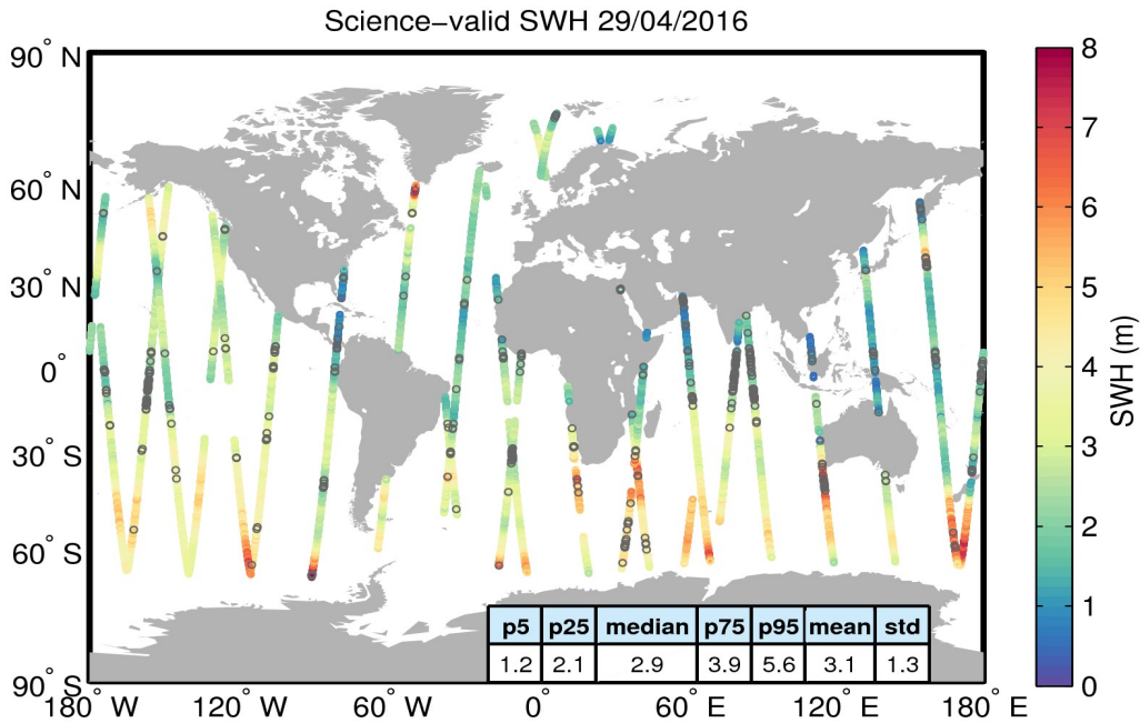
Figure 19. Geographical distribution of science-valid SWH data over oceans and lakes for 29/04/2016. The statistical values shown in the table refer to the SWH in m and are calculated over all measurements shown in the figure. Gray circles denote records that have been rejected based on the editing criteria described in Table 3.
