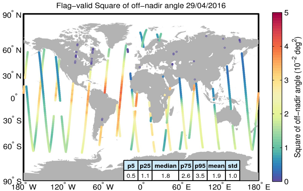
Figure 37. Geographical distribution of flag-valid mispointing data over oceans and lakes for 29/04/2016. The statistical values shown in the table refer to the mispointing in 10^{-2} \text{ deg}^2 and are calculated over all measurements shown in the figure.
