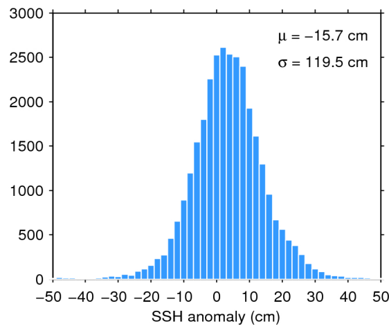
Figure 7. Histogram of flag-valid SSH anomaly over oceans and lakes for 29/04/2016. The mean ( \mu ) and standard deviation ( \sigma ) are also shown. Note that values outside [-50\ 50] cm are excluded from the histogram for the sake of readability but not from the computation of \mu and \sigma .
