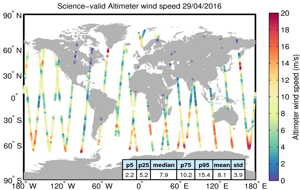
Figure 34. Geographical distribution of science-valid wind data over oceans and lakes for 29/04/2016. The statistical values shown in the table refer to the wind in m/s and are calculated over all measurements shown in the figure. Gray circles denote records that have been rejected based on the editing criteria described in Table 5.
