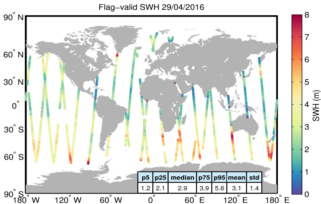
Figure 15. Geographical distribution of flag-valid SWH data over oceans and lakes for 29/04/2016. The statistical values shown in the table refer to the SWH in m and are calculated over all measurements shown in the figure.
