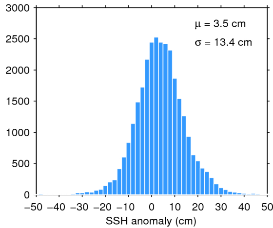
Figure 11. Histogram of science-valid SSH anomaly over oceans and lakes for 29/04/2016. The mean ( \mu ) and standard deviation ( \sigma ) are also shown. Note that values outside [-50 50] cm are excluded from the histogram for the sake of readability but not from the computation of \mu and \sigma .
