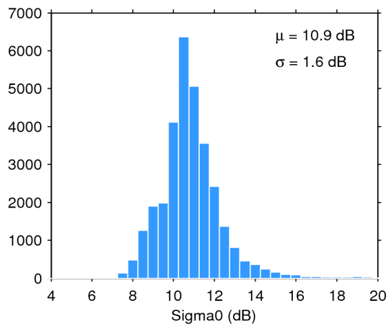
Figure 28. Histogram of science-valid sigma0 over oceans and lakes for 29/04/2016. The mean ( \mu ) and standard deviation ( \sigma ) are also shown. Note that values outside [4 20] dB are excluded from the histogram for the sake of readability but not from the computation of \mu and \sigma .
