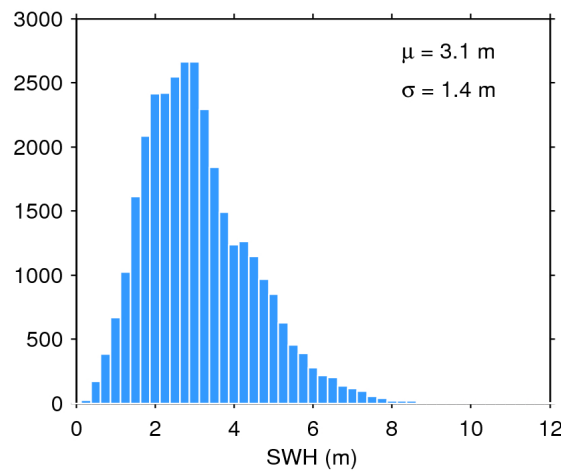
Figure 17. Histogram of flag-valid SWH over oceans and lakes for 29/04/2016. The mean ( \mu ) and standard deviation ( \sigma ) are also shown. Note that values larger than 12 m are excluded from the histogram for the sake of readability but not from the computation of \mu and \sigma .
