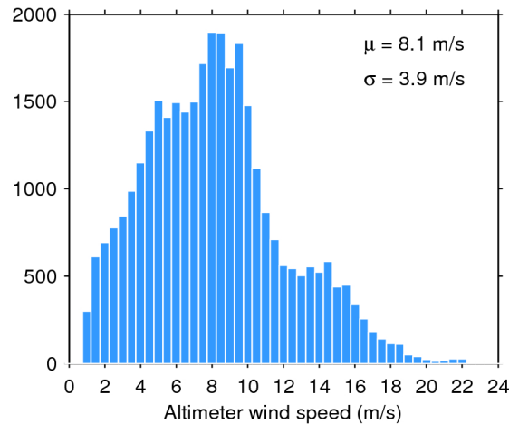
Figure 33. Histogram of flag-valid wind over oceans and lakes for 29/04/2016. The mean ( \mu ) and standard deviation ( \sigma ) are also shown. Note that values larger than 24 m/s are excluded from the histogram for the sake of readability but not from the computation of \mu and \sigma .
