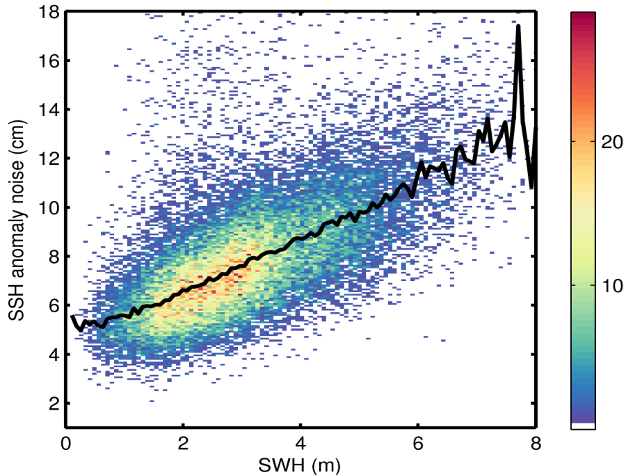
Figure 9. 2D histogram showing flag-valid SSH anomaly noise as a function of SWH for 29/04/2016. The black line denotes the median SSH anomaly noise as a function of SWH.
