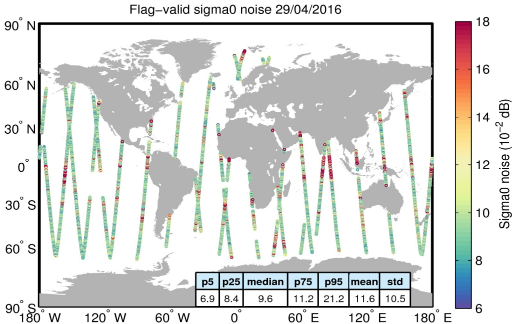
Figure 26. Geographical distribution of flag-valid 20-Hz sigma0 measurement noise over oceans and lakes for 29/04/2016. The statistical values shown in the table refer to the sigma0 noise and are calculated over all measurements shown in the figure.
