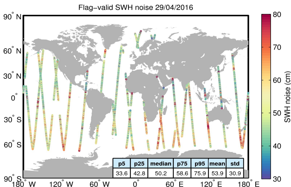
Figure 18. Geographical distribution of flag-valid 20-Hz SWH measurement noise over oceans and lakes for 29/04/2016. The statistical values shown in the table refer to the SWH noise and are calculated over all measurements shown in the figure.
