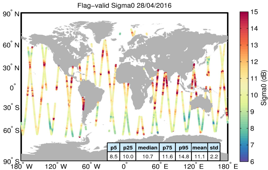
Figure 23. Geographical distribution of flag-valid sigma0 data over oceans and lakes for 28/04/2016. The statistical values shown in the table refer to the sigma0 in dB and are calculated over all measurements shown in the figure.
