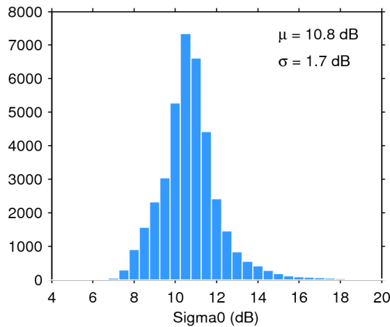
Figure 28. Histogram of science-valid sigma0 over oceans and lakes for 28/04/2016. The mean ( \mu ) and standard deviation ( \sigma ) are also shown. Note that values outside [4 20] dB are excluded from the histogram for the sake of readability but not from the computation of \mu and \sigma .
