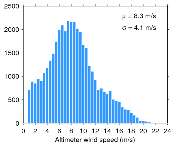
Figure 35. Histogram of science-valid wind over oceans and lakes for 28/04/2016. The mean ( \mu ) and standard deviation ( \sigma ) are also shown. Note that values larger than 24 m/s are excluded from the histogram for the sake of readability but not from the computation of \mu and \sigma .
