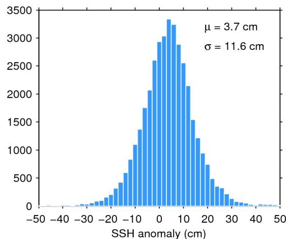
Figure 11. Histogram of science-valid SSH anomaly over oceans and lakes for 28/04/2016. The mean ( \mu ) and standard deviation ( \sigma ) are also shown. Note that values outside [-50 50] cm are excluded from the histogram for the sake of readability but not from the computation of \mu and \sigma .
