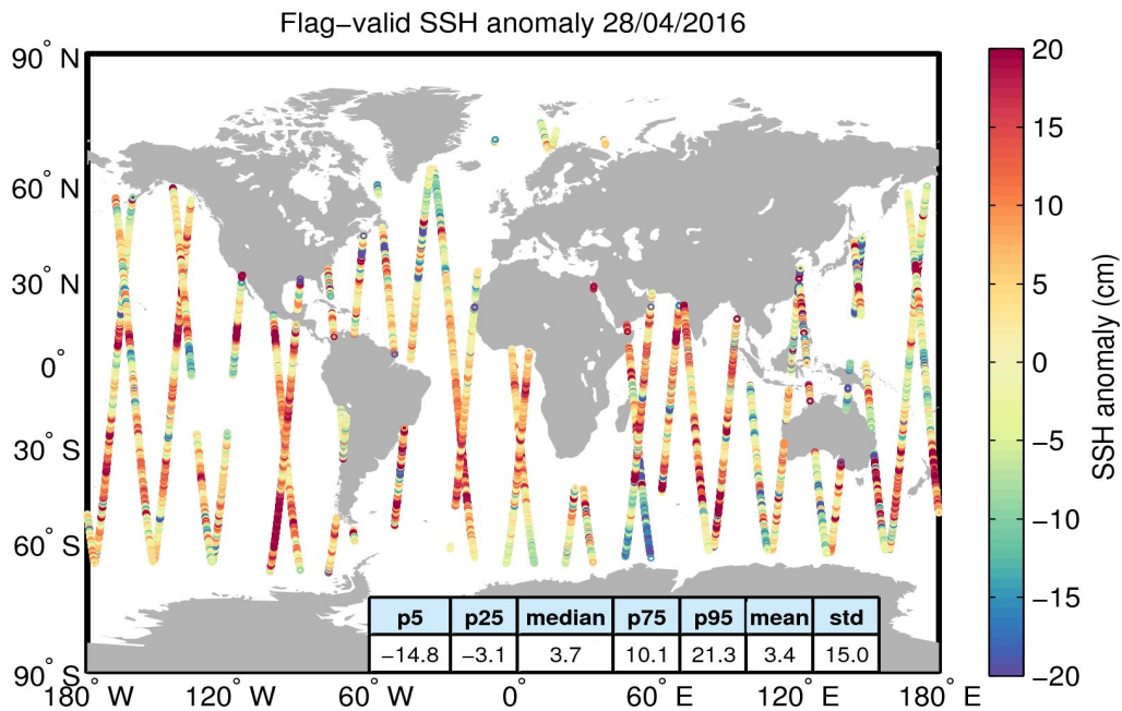
Figure 5. Geographical distribution of flag-valid 1-Hz SSH anomaly data over oceans and lakes for 28/04/2016. The statistical values shown in the table refer to the SSH anomaly in cm and are calculated over all measurements shown in the figure.
