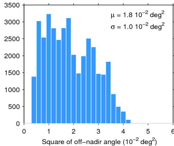
Figure 39. Histogram of flag-valid mispointing over oceans and lakes for 28/04/2016. The mean ( \mu ) and standard deviation ( \sigma ) are also shown. Note that values larger than 6 \cdot 10^{-2} \text{ deg}^2 are excluded from the histogram for the sake of readability but not from the computation of \mu and \sigma .
