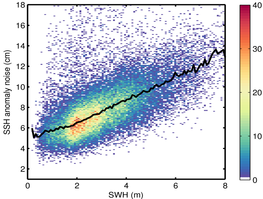
Figure 9. 2D histogram showing flag-valid SSH anomaly noise as a function of SWH for 28/04/2016. The black line denotes the median SSH anomaly noise as a function of SWH.
