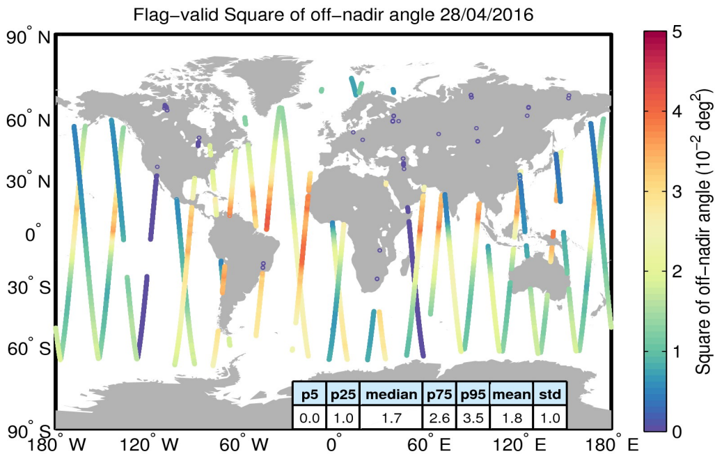
Figure 37. Geographical distribution of flag-valid mispointing data over oceans and lakes for 28/04/2016. The statistical values shown in the table refer to the mispointing in 10^{-2} \text{ deg}^2 and are calculated over all measurements shown in the figure.
