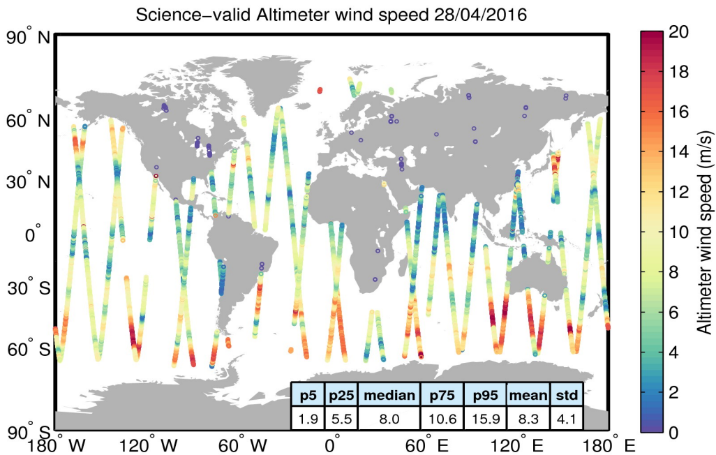
Figure 34. Geographical distribution of science-valid wind data over oceans and lakes for 28/04/2016. The statistical values shown in the table refer to the wind in m/s and are calculated over all measurements shown in the figure. Gray circles denote records that have been rejected based on the editing criteria described in Table 5.
