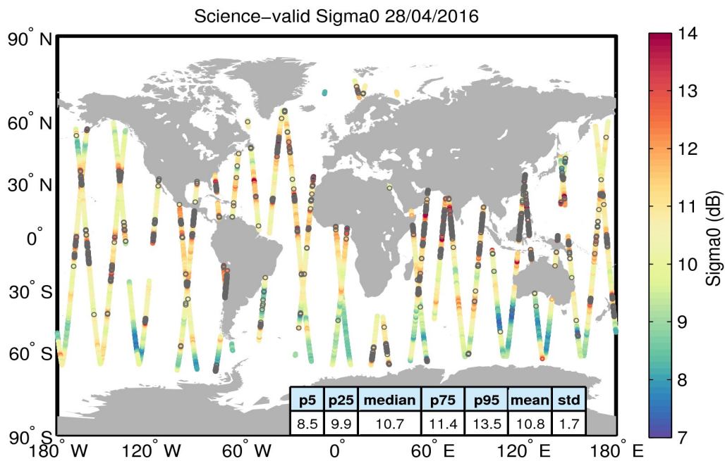
Figure 27. Geographical distribution of science-valid sigma0 data over oceans and lakes for 28/04/2016. The statistical values shown in the table refer to the sigma0 in dB and are calculated over all measurements shown in the figure. Gray circles denote records that have been rejected based on the editing criteria described in Table 4.
