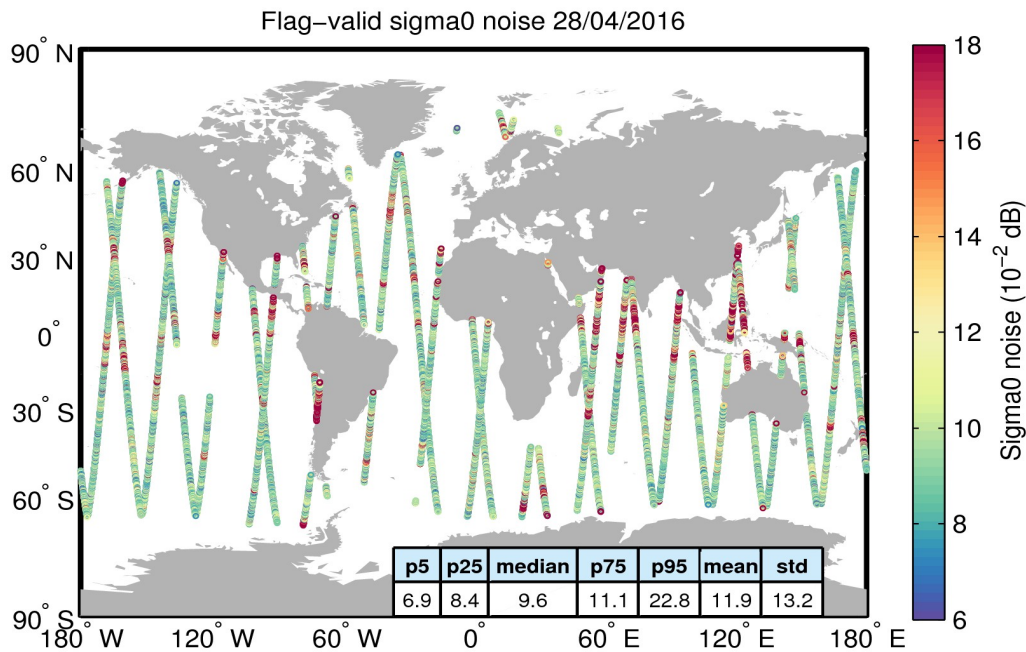
Figure 26. Geographical distribution of flag-valid 20-Hz sigma0 measurement noise over oceans and lakes for 28/04/2016. The statistical values shown in the table refer to the sigma0 noise and are calculated over all measurements shown in the figure.
