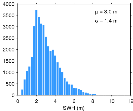
Figure 20. Histogram of science-valid SWH over oceans and lakes for 28/04/2016. The mean ( \mu ) and standard deviation ( \sigma ) are also shown. Note that values larger than 12 m are excluded from the histogram for the sake of readability but not from the computation of \mu and \sigma .
