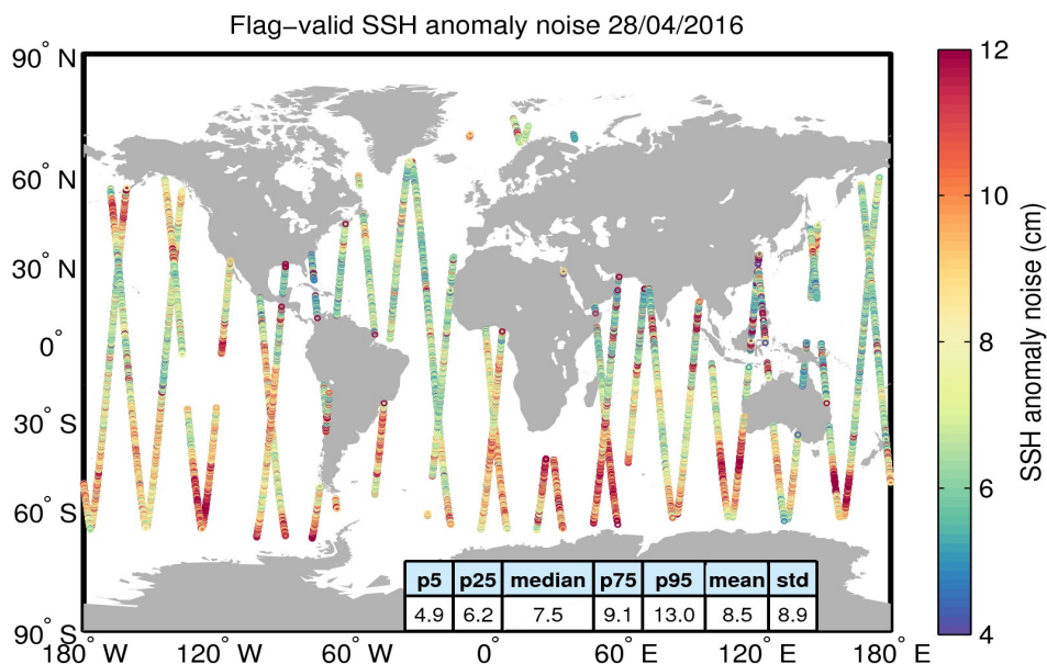
Figure 8. Geographical distribution of flag-valid 20-Hz SSH anomaly measurement noise over oceans and lakes for 28/04/2016. The statistical values shown in the table refer to the SSH anomaly noise and are calculated over all measurements shown in the figure.
