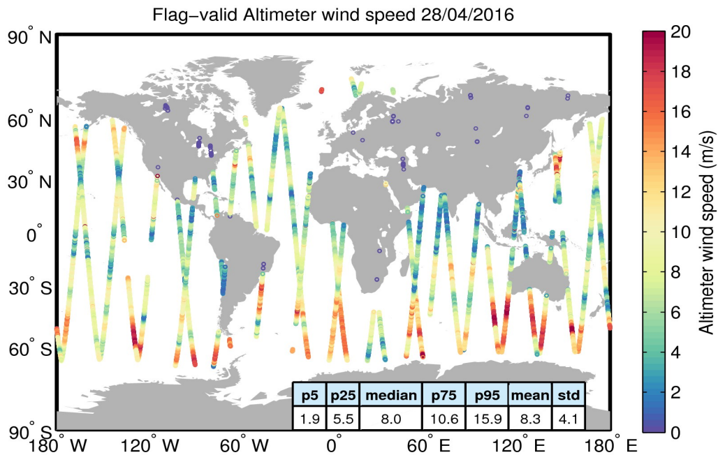
Figure 31. Geographical distribution of flag-valid wind data over oceans and lakes for 28/04/2016. The statistical values shown in the table refer to the wind in m/s and are calculated over all measurements shown in the figure.
