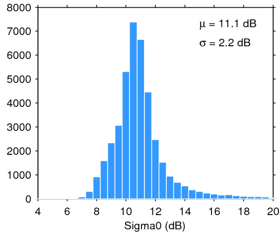
Figure 25. Histogram of flag-valid sigma0 over oceans and lakes for 28/04/2016. The mean ( \mu ) and standard deviation ( \sigma ) are also shown. Note that values outside [4 20] dB are excluded from the histogram for the sake of readability but not from the computation of \mu and \sigma .
