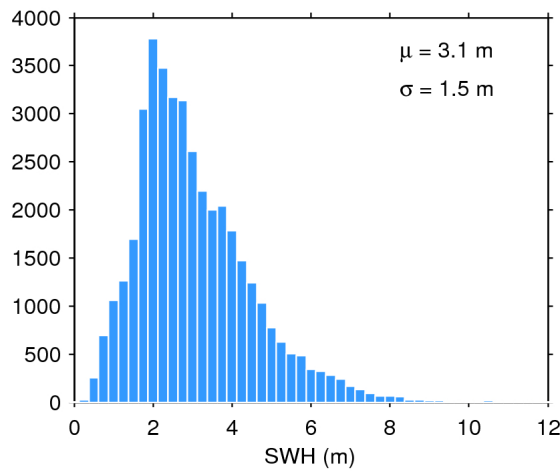
Figure 17. Histogram of flag-valid SWH over oceans and lakes for 28/04/2016. The mean ( \mu ) and standard deviation ( \sigma ) are also shown. Note that values larger than 12 m are excluded from the histogram for the sake of readability but not from the computation of \mu and \sigma .
