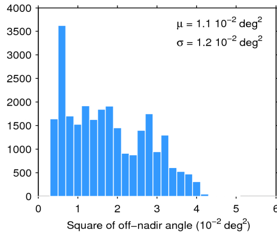
Figure 39. Histogram of flag-valid mispointing over oceans and lakes for 27/04/2016. The mean ( \mu ) and standard deviation ( \sigma ) are also shown. Note that values larger than 6 \cdot 10^{-2} \text{ deg}^2 are excluded from the histogram for the sake of readability but not from the computation of \mu and \sigma .
