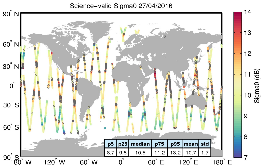
Figure 27. Geographical distribution of science-valid sigma0 data over oceans and lakes for 27/04/2016. The statistical values shown in the table refer to the sigma0 in dB and are calculated over all measurements shown in the figure. Gray circles denote records that have been rejected based on the editing criteria described in Table 4.
