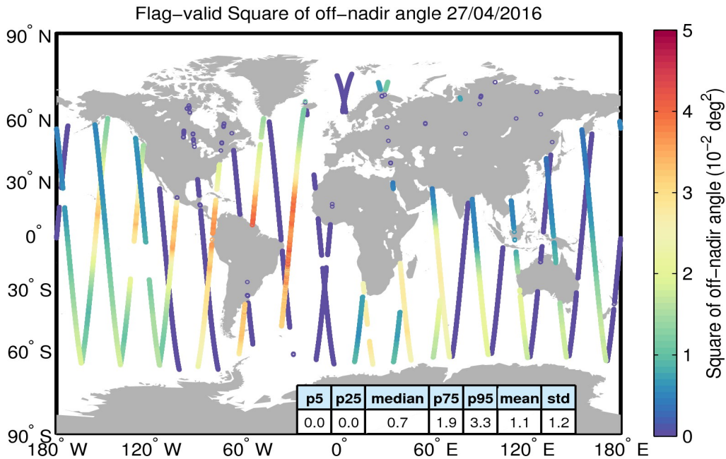
Figure 37. Geographical distribution of flag-valid mispointing data over oceans and lakes for 27/04/2016. The statistical values shown in the table refer to the mispointing in 10^{-2} \text{ deg}^2 and are calculated over all measurements shown in the figure.
