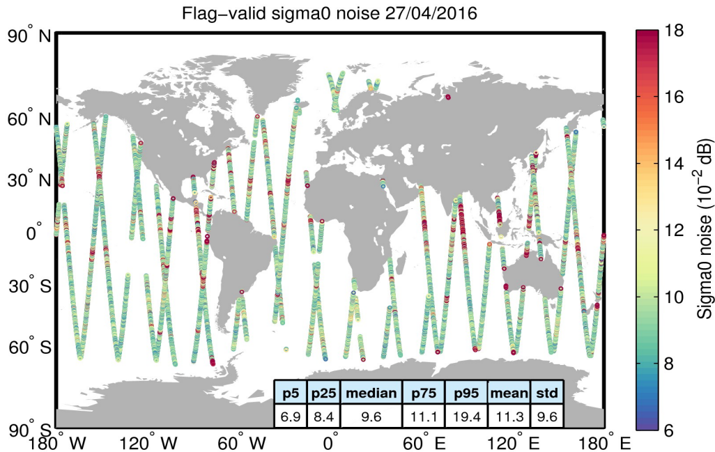
Figure 26. Geographical distribution of flag-valid 20-Hz sigma0 measurement noise over oceans and lakes for 27/04/2016. The statistical values shown in the table refer to the sigma0 noise and are calculated over all measurements shown in the figure.
