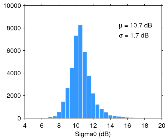
Figure 28. Histogram of science-valid sigma0 over oceans and lakes for 27/04/2016. The mean ( \mu ) and standard deviation ( \sigma ) are also shown. Note that values outside [4 20] dB are excluded from the histogram for the sake of readability but not from the computation of \mu and \sigma .
