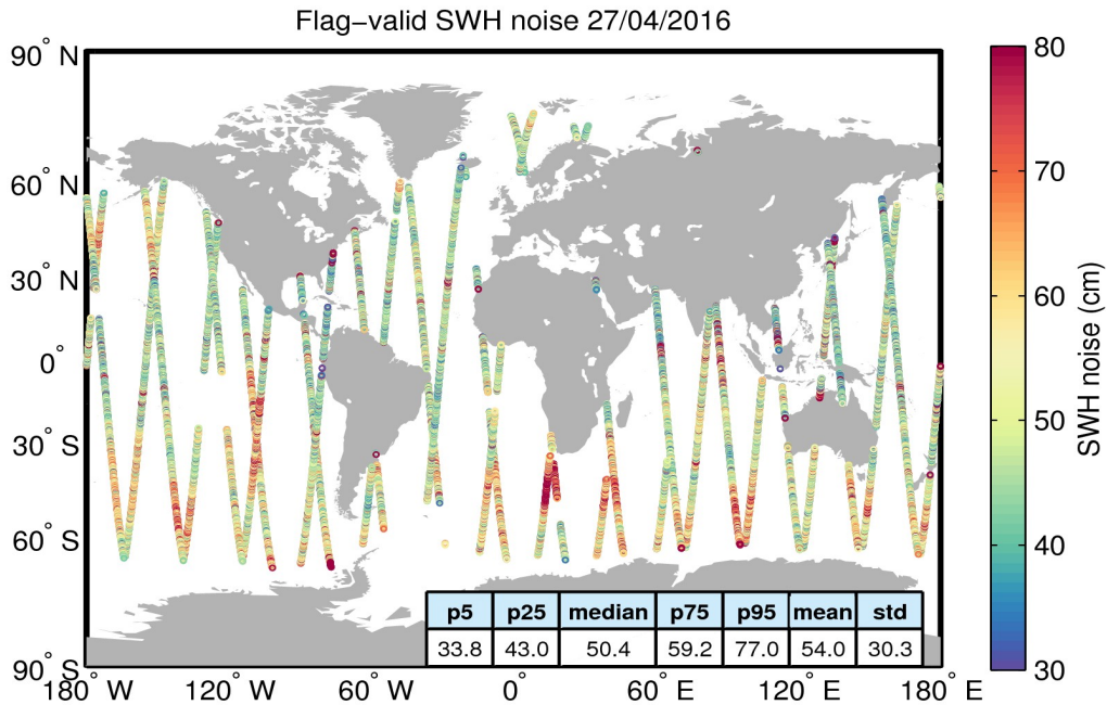
Figure 18. Geographical distribution of flag-valid 20-Hz SWH measurement noise over oceans and lakes for 27/04/2016. The statistical values shown in the table refer to the SWH noise and are calculated over all measurements shown in the figure.
