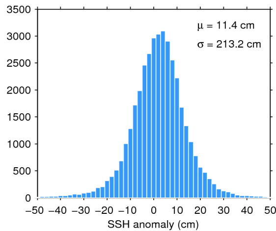
Figure 7. Histogram of flag-valid SSH anomaly over oceans and lakes for 27/04/2016. The mean ( \mu ) and standard deviation ( \sigma ) are also shown. Note that values outside [-50 50] cm are excluded from the histogram for the sake of readability but not from the computation of \mu and \sigma .
