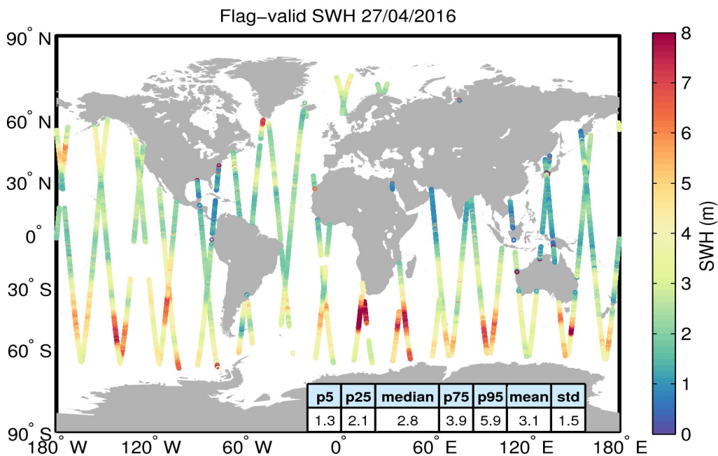
Figure 15. Geographical distribution of flag-valid SWH data over oceans and lakes for 27/04/2016. The statistical values shown in the table refer to the SWH in m and are calculated over all measurements shown in the figure.
