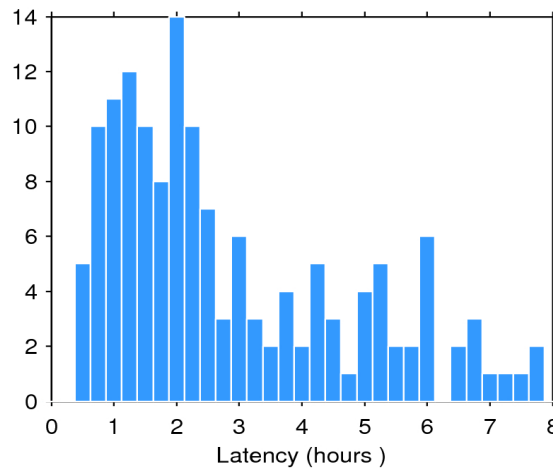
Figure 2. Histogram of the data latency for 27/04/2016. The y-axis denotes the number of files that are made available with a delay of x-hours with respect to the mean time of the records stored in the file.
