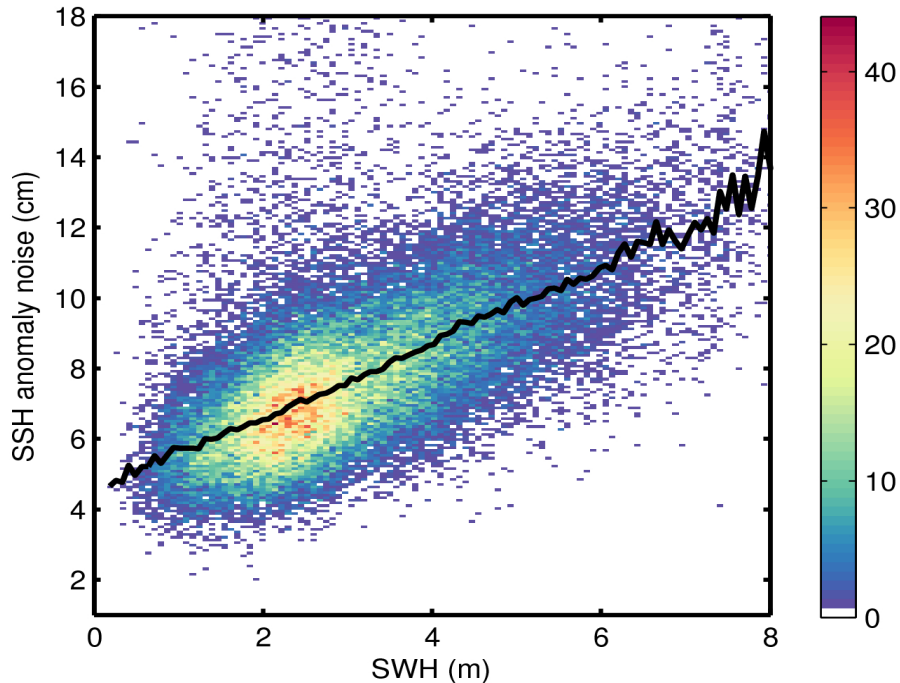
Figure 9. 2D histogram showing flag-valid SSH anomaly noise as a function of SWH for 27/04/2016. The black line denotes the median SSH anomaly noise as a function of SWH.
