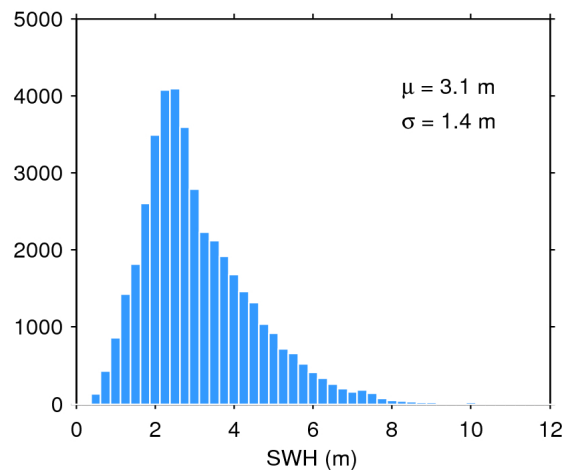
Figure 20. Histogram of science-valid SWH over oceans and lakes for 27/04/2016. The mean ( \mu ) and standard deviation ( \sigma ) are also shown. Note that values larger than 12 m are excluded from the histogram for the sake of readability but not from the computation of \mu and \sigma .
