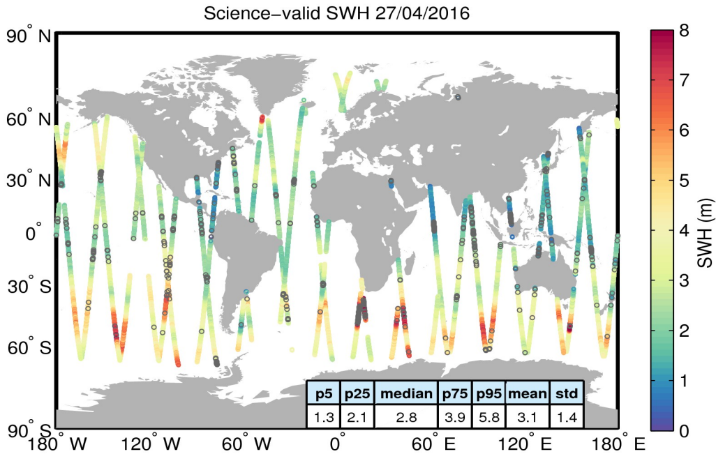
Figure 19. Geographical distribution of science-valid SWH data over oceans and lakes for 27/04/2016. The statistical values shown in the table refer to the SWH in m and are calculated over all measurements shown in the figure. Gray circles denote records that have been rejected based on the editing criteria described in Table 3.
