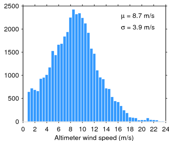
Figure 35. Histogram of science-valid wind over oceans and lakes for 27/04/2016. The mean ( \mu ) and standard deviation ( \sigma ) are also shown. Note that values larger than 24 m/s are excluded from the histogram for the sake of readability but not from the computation of \mu and \sigma .
