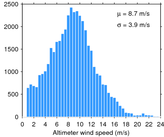
Figure 33. Histogram of flag-valid wind over oceans and lakes for 27/04/2016. The mean ( \mu ) and standard deviation ( \sigma ) are also shown. Note that values larger than 24 m/s are excluded from the histogram for the sake of readability but not from the computation of \mu and \sigma .
