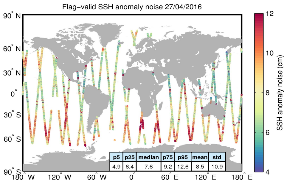
Figure 8. Geographical distribution of flag-valid 20-Hz SSH anomaly measurement noise over oceans and lakes for 27/04/2016. The statistical values shown in the table refer to the SSH anomaly noise and are calculated over all measurements shown in the figure.
