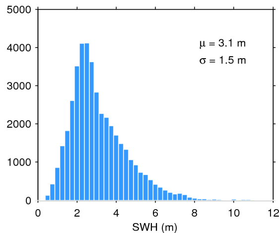
Figure 17. Histogram of flag-valid SWH over oceans and lakes for 27/04/2016. The mean ( \mu ) and standard deviation ( \sigma ) are also shown. Note that values larger than 12 m are excluded from the histogram for the sake of readability but not from the computation of \mu and \sigma .
