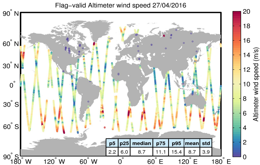
Figure 31. Geographical distribution of flag-valid wind data over oceans and lakes for 27/04/2016. The statistical values shown in the table refer to the wind in m/s and are calculated over all measurements shown in the figure.
