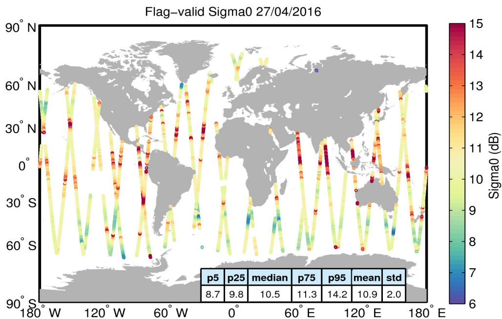
Figure 23. Geographical distribution of flag-valid sigma0 data over oceans and lakes for 27/04/2016. The statistical values shown in the table refer to the sigma0 in dB and are calculated over all measurements shown in the figure.
