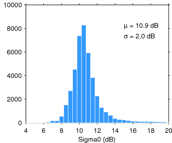
Figure 25. Histogram of flag-valid sigma0 over oceans and lakes for 27/04/2016. The mean ( \mu ) and standard deviation ( \sigma ) are also shown. Note that values outside [4 20] dB are excluded from the histogram for the sake of readability but not from the computation of \mu and \sigma .
