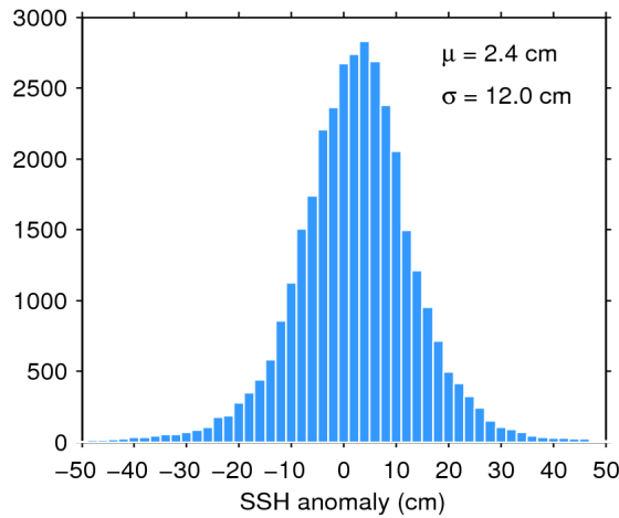
Figure 11. Histogram of science-valid SSH anomaly over oceans and lakes for 27/04/2016. The mean ( \mu ) and standard deviation ( \sigma ) are also shown. Note that values outside [-50 50] cm are excluded from the histogram for the sake of readability but not from the computation of \mu and \sigma .
