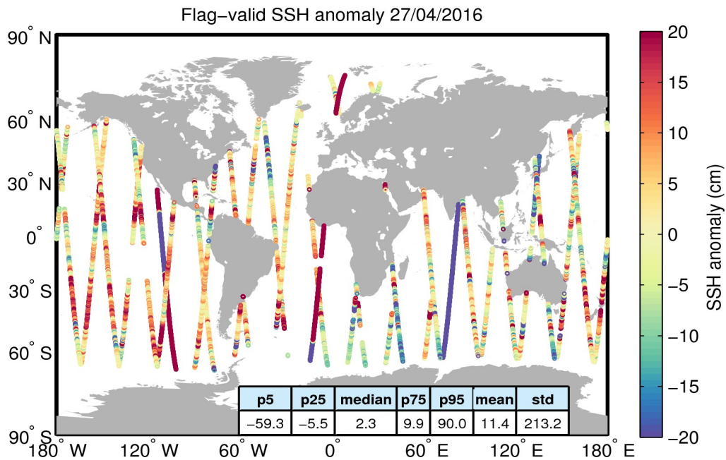
Figure 5. Geographical distribution of flag-valid 1-Hz SSH anomaly data over oceans and lakes for 27/04/2016. The statistical values shown in the table refer to the SSH anomaly in cm and are calculated over all measurements shown in the figure.
