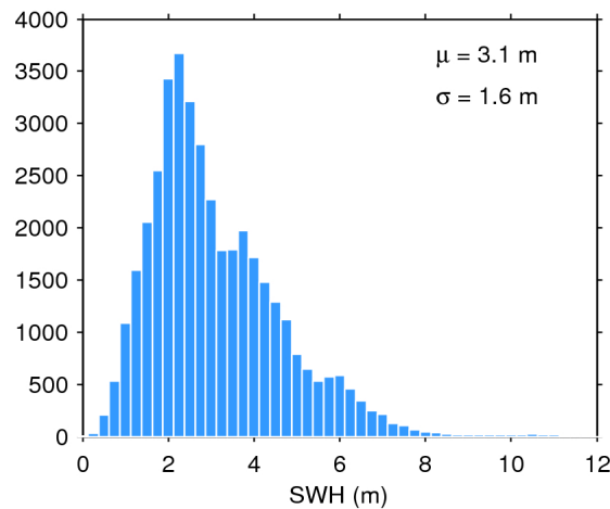
Figure 17. Histogram of flag-valid SWH over oceans and lakes for 26/04/2016. The mean ( \mu ) and standard deviation ( \sigma ) are also shown. Note that values larger than 12 m are excluded from the histogram for the sake of readability but not from the computation of \mu and \sigma .
