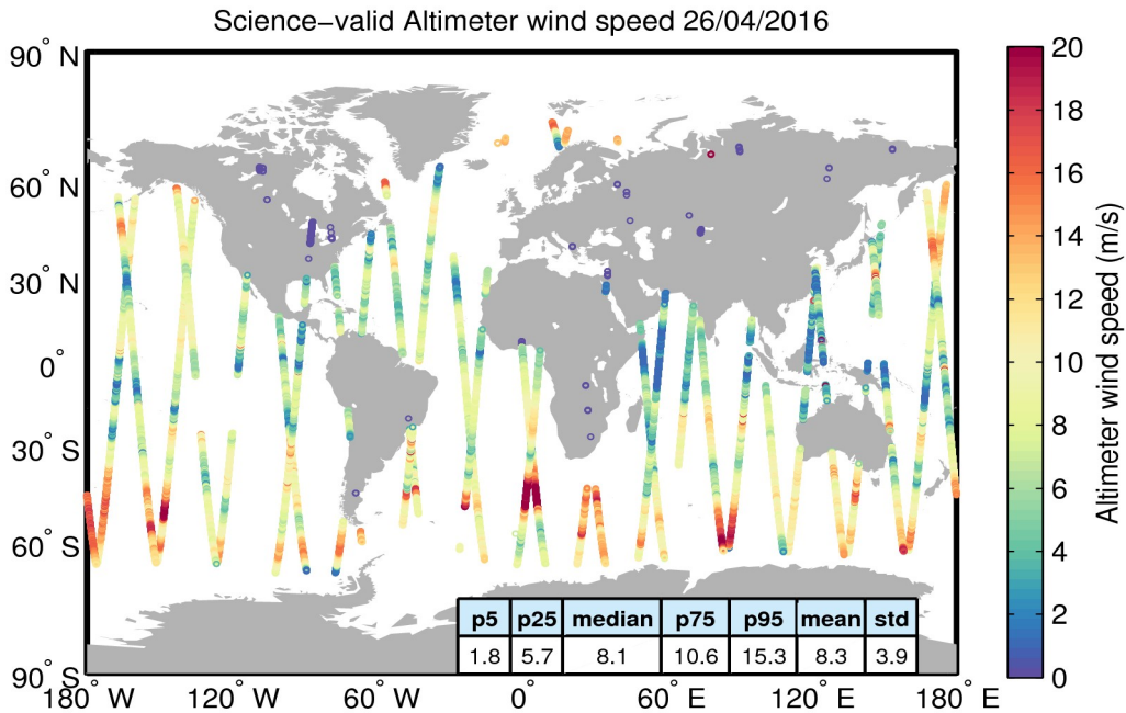
Figure 34. Geographical distribution of science-valid wind data over oceans and lakes for 26/04/2016. The statistical values shown in the table refer to the wind in m/s and are calculated over all measurements shown in the figure. Gray circles denote records that have been rejected based on the editing criteria described in Table 5.
