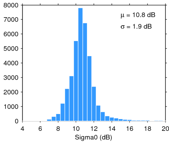
Figure 28. Histogram of science-valid sigma0 over oceans and lakes for 26/04/2016. The mean ( \mu ) and standard deviation ( \sigma ) are also shown. Note that values outside [4 20] dB are excluded from the histogram for the sake of readability but not from the computation of \mu and \sigma .
