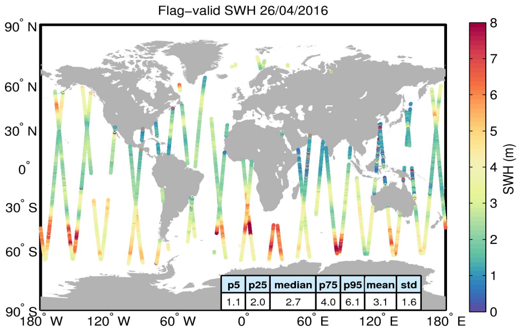
Figure 15. Geographical distribution of flag-valid SWH data over oceans and lakes for 26/04/2016. The statistical values shown in the table refer to the SWH in m and are calculated over all measurements shown in the figure.
