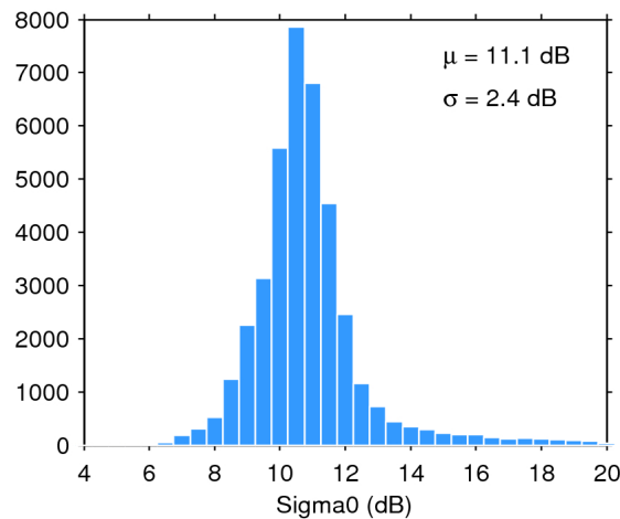
Figure 25. Histogram of flag-valid sigma0 over oceans and lakes for 26/04/2016. The mean ( \mu ) and standard deviation ( \sigma ) are also shown. Note that values outside [4 20] dB are excluded from the histogram for the sake of readability but not from the computation of \mu and \sigma .
