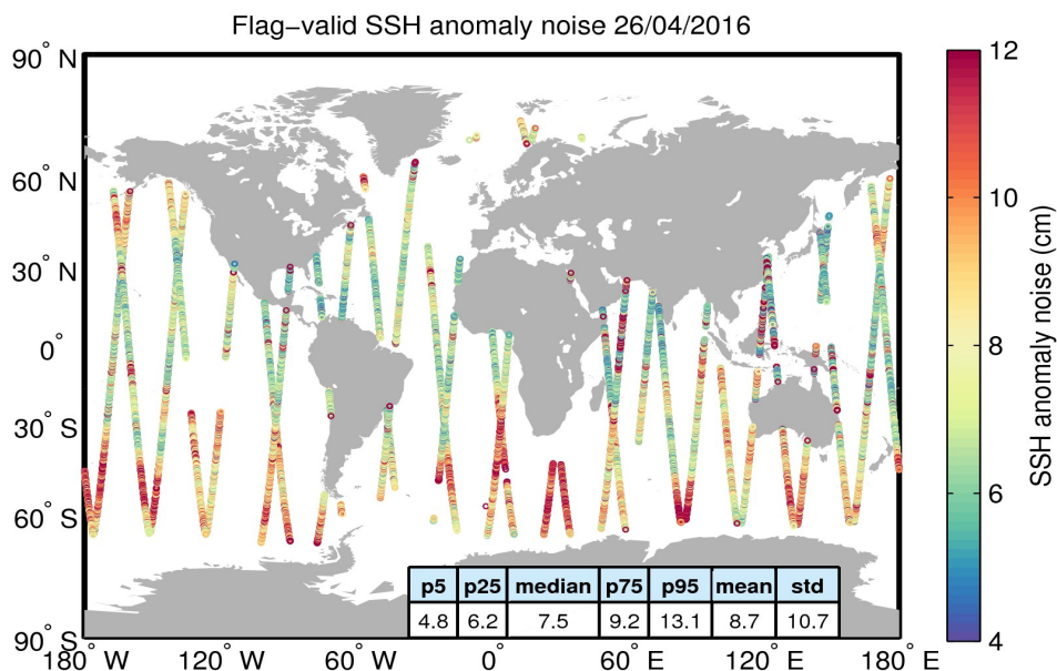
Figure 8. Geographical distribution of flag-valid 20-Hz SSH anomaly measurement noise over oceans and lakes for 26/04/2016. The statistical values shown in the table refer to the SSH anomaly noise and are calculated over all measurements shown in the figure.
