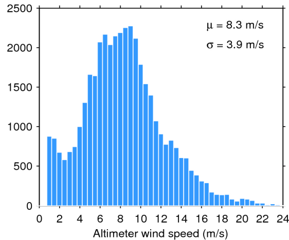
Figure 33. Histogram of flag-valid wind over oceans and lakes for 26/04/2016. The mean ( \mu ) and standard deviation ( \sigma ) are also shown. Note that values larger than 24 m/s are excluded from the histogram for the sake of readability but not from the computation of \mu and \sigma .
