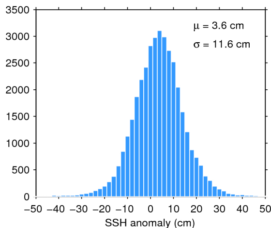
Figure 11. Histogram of science-valid SSH anomaly over oceans and lakes for 26/04/2016. The mean ( \mu ) and standard deviation ( \sigma ) are also shown. Note that values outside [-50 50] cm are excluded from the histogram for the sake of readability but not from the computation of \mu and \sigma .
