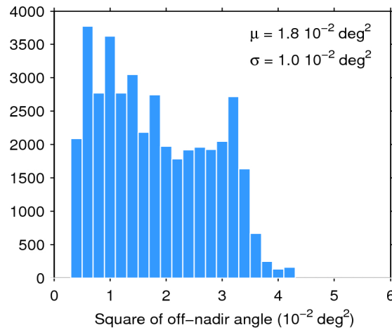
Figure 39. Histogram of flag-valid mispointing over oceans and lakes for 26/04/2016. The mean ( \mu ) and standard deviation ( \sigma ) are also shown. Note that values larger than 6 \cdot 10^{-2} \text{ deg}^2 are excluded from the histogram for the sake of readability but not from the computation of \mu and \sigma .
