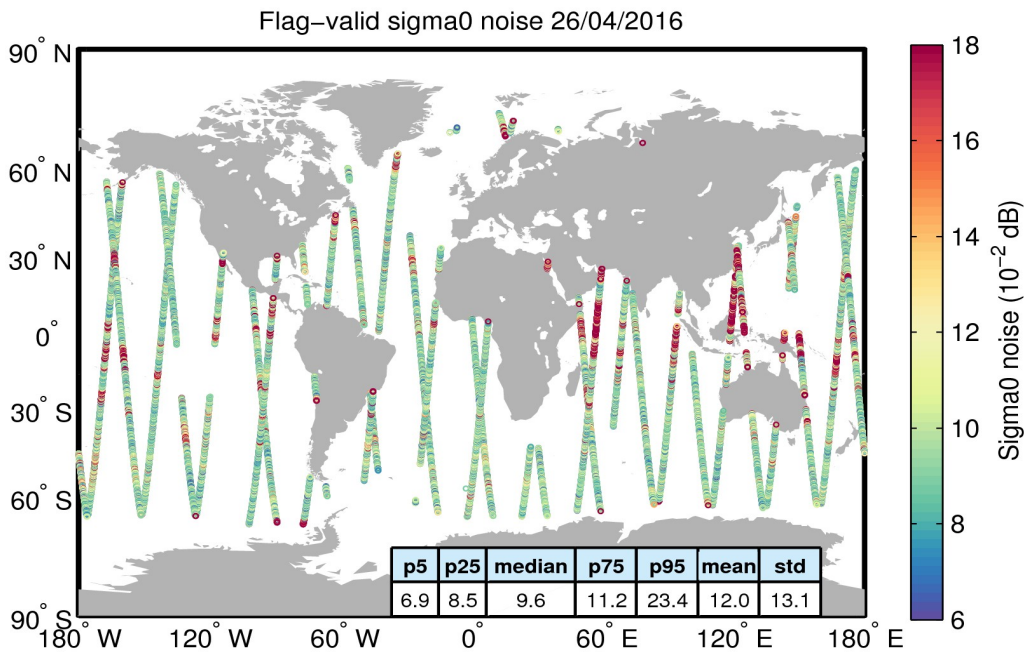
Figure 26. Geographical distribution of flag-valid 20-Hz sigma0 measurement noise over oceans and lakes for 26/04/2016. The statistical values shown in the table refer to the sigma0 noise and are calculated over all measurements shown in the figure.
