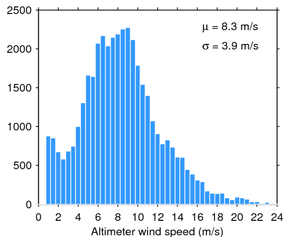
Figure 35. Histogram of science-valid wind over oceans and lakes for 26/04/2016. The mean ( \mu ) and standard deviation ( \sigma ) are also shown. Note that values larger than 24 m/s are excluded from the histogram for the sake of readability but not from the computation of \mu and \sigma .
