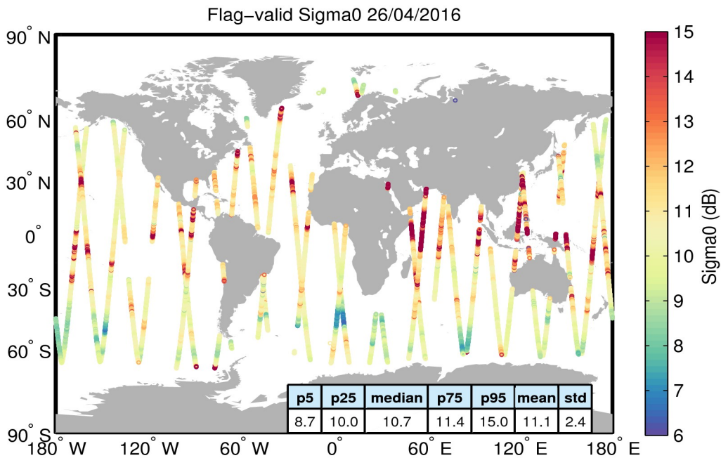
Figure 23. Geographical distribution of flag-valid sigma0 data over oceans and lakes for 26/04/2016. The statistical values shown in the table refer to the sigma0 in dB and are calculated over all measurements shown in the figure.
