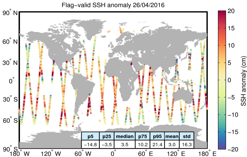
Figure 5. Geographical distribution of flag-valid 1-Hz SSH anomaly data over oceans and lakes for 26/04/2016. The statistical values shown in the table refer to the SSH anomaly in cm and are calculated over all measurements shown in the figure.
