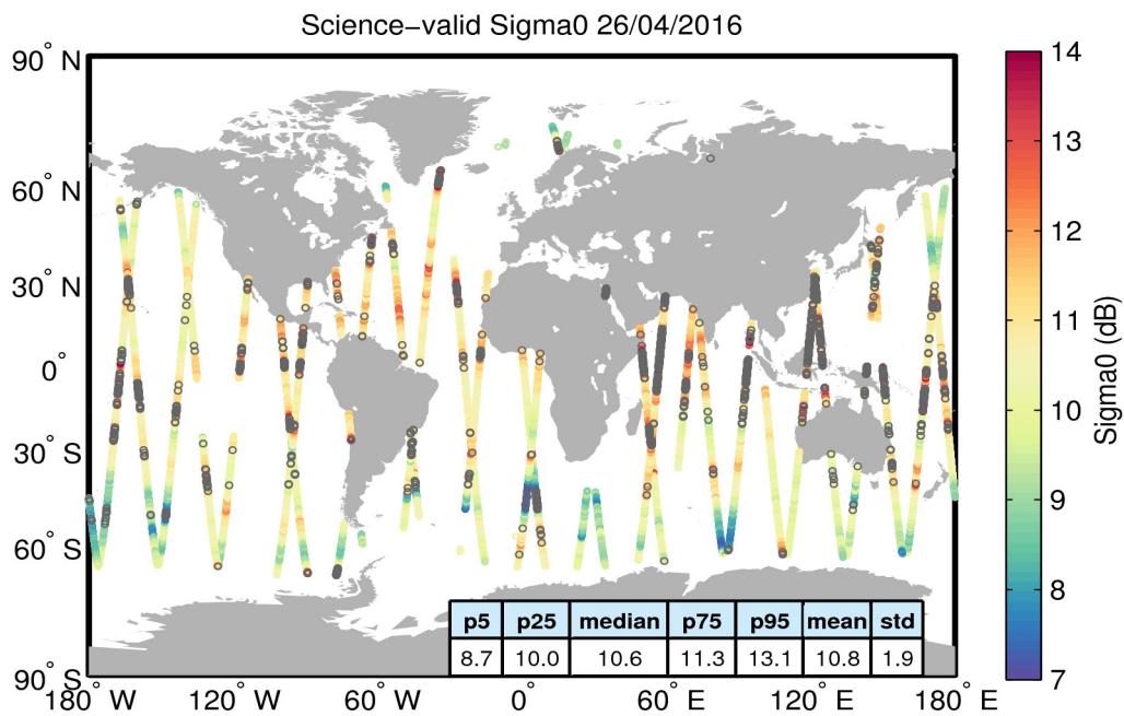
Figure 27. Geographical distribution of science-valid sigma0 data over oceans and lakes for 26/04/2016. The statistical values shown in the table refer to the sigma0 in dB and are calculated over all measurements shown in the figure. Gray circles denote records that have been rejected based on the editing criteria described in Table 4.
