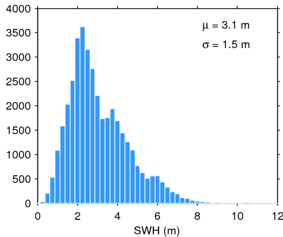
Figure 20. Histogram of science-valid SWH over oceans and lakes for 26/04/2016. The mean ( \mu ) and standard deviation ( \sigma ) are also shown. Note that values larger than 12 m are excluded from the histogram for the sake of readability but not from the computation of \mu and \sigma .
