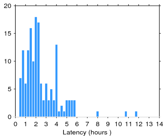
Figure 2. Histogram of the data latency for 26/04/2016. The y-axis denotes the number of files that are made available with a delay of x-hours with respect to the mean time of the records stored in the file.
