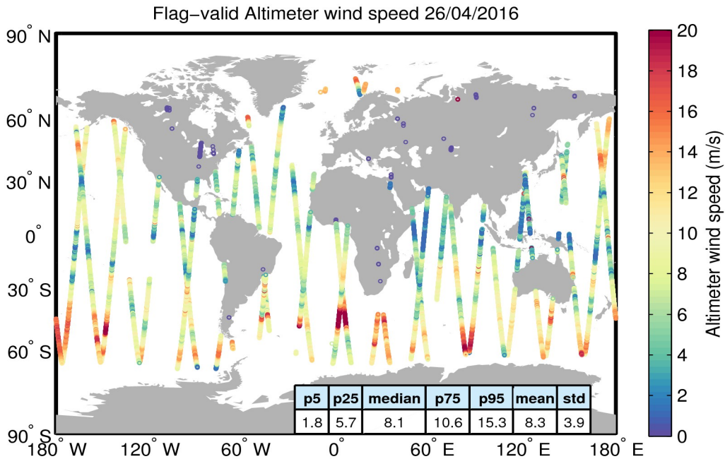
Figure 31. Geographical distribution of flag-valid wind data over oceans and lakes for 26/04/2016. The statistical values shown in the table refer to the wind in m/s and are calculated over all measurements shown in the figure.
