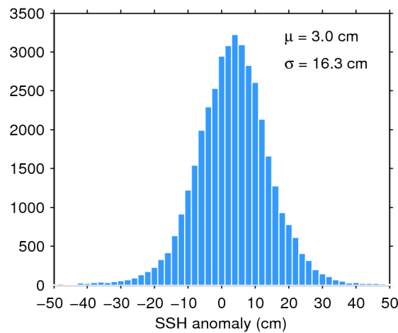
Figure 7. Histogram of flag-valid SSH anomaly over oceans and lakes for 26/04/2016. The mean ( \mu ) and standard deviation ( \sigma ) are also shown. Note that values outside [-50 50] cm are excluded from the histogram for the sake of readability but not from the computation of \mu and \sigma .
