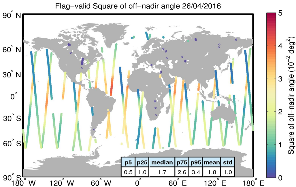
Figure 37. Geographical distribution of flag-valid mispointing data over oceans and lakes for 26/04/2016. The statistical values shown in the table refer to the mispointing in 10^{-2} \text{ deg}^2 and are calculated over all measurements shown in the figure.
