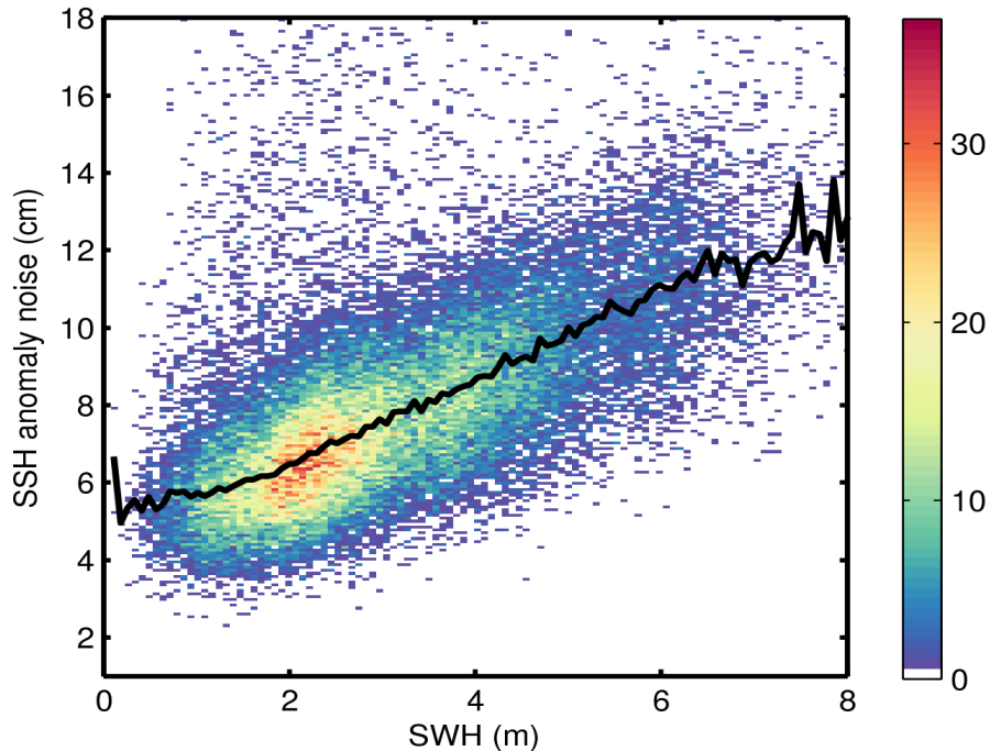
Figure 9. 2D histogram showing flag-valid SSH anomaly noise as a function of SWH for 26/04/2016. The black line denotes the median SSH anomaly noise as a function of SWH.
