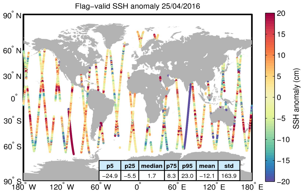
Figure 5. Geographical distribution of flag-valid 1-Hz SSH anomaly data over oceans and lakes for 25/04/2016. The statistical values shown in the table refer to the SSH anomaly in cm and are calculated over all measurements shown in the figure.
