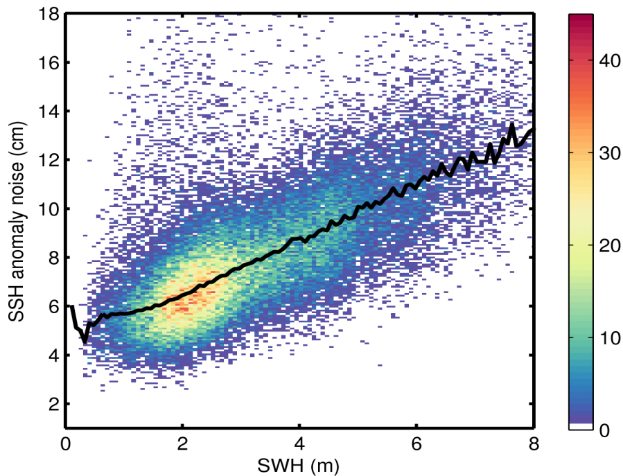
Figure 9. 2D histogram showing flag-valid SSH anomaly noise as a function of SWH for 25/04/2016. The black line denotes the median SSH anomaly noise as a function of SWH.
