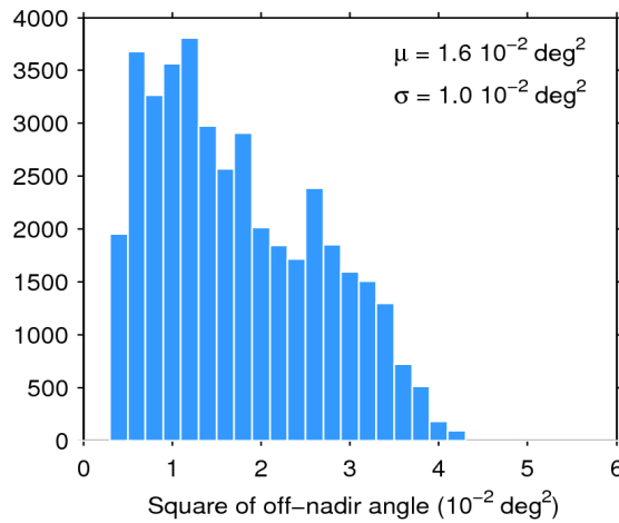
Figure 39. Histogram of flag-valid mispointing over oceans and lakes for 25/04/2016. The mean ( \mu ) and standard deviation ( \sigma ) are also shown. Note that values larger than 6 \cdot 10^{-2} \text{ deg}^2 are excluded from the histogram for the sake of readability but not from the computation of \mu and \sigma .
