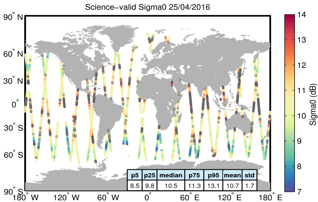
Figure 27. Geographical distribution of science-valid sigma0 data over oceans and lakes for 25/04/2016. The statistical values shown in the table refer to the sigma0 in dB and are calculated over all measurements shown in the figure. Gray circles denote records that have been rejected based on the editing criteria described in Table 4.
