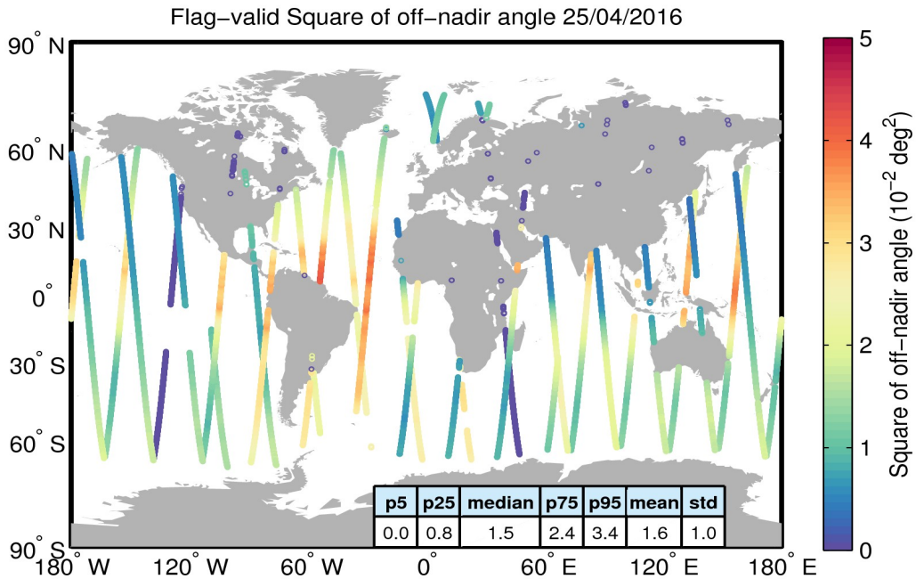
Figure 37. Geographical distribution of flag-valid mispointing data over oceans and lakes for 25/04/2016. The statistical values shown in the table refer to the mispointing in 10^{-2} \text{ deg}^2 and are calculated over all measurements shown in the figure.
