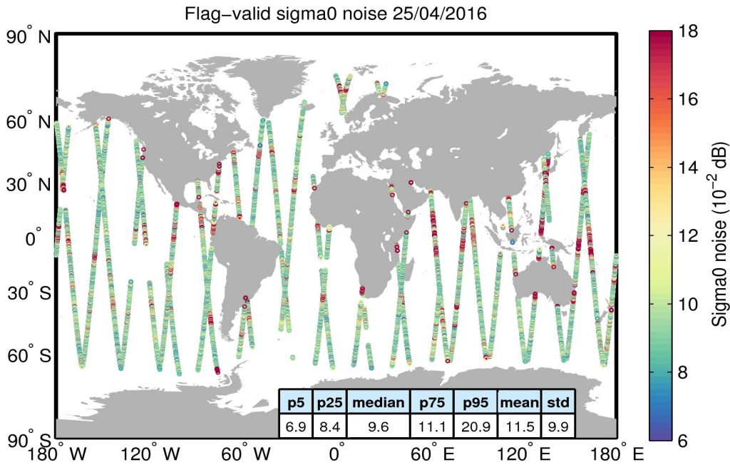
Figure 26. Geographical distribution of flag-valid 20-Hz sigma0 measurement noise over oceans and lakes for 25/04/2016. The statistical values shown in the table refer to the sigma0 noise and are calculated over all measurements shown in the figure.
