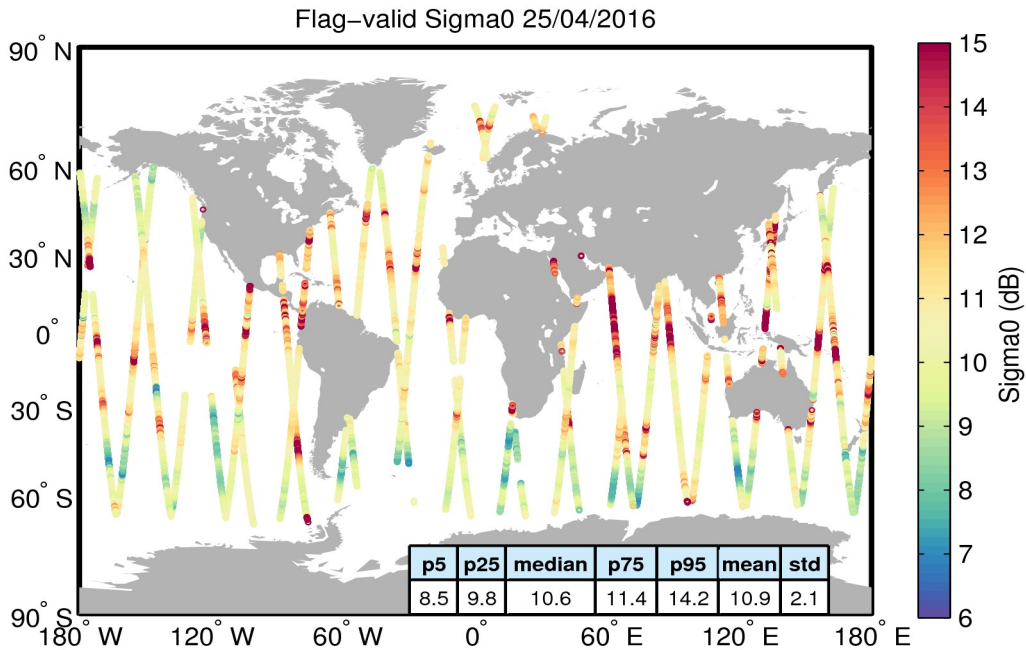
Figure 23. Geographical distribution of flag-valid sigma0 data over oceans and lakes for 25/04/2016. The statistical values shown in the table refer to the sigma0 in dB and are calculated over all measurements shown in the figure.
