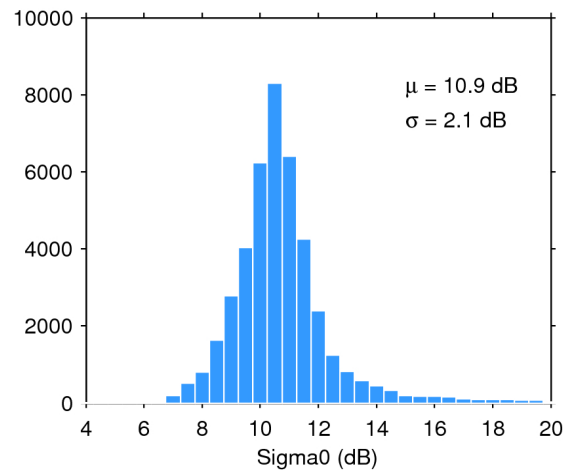
Figure 25. Histogram of flag-valid sigma0 over oceans and lakes for 25/04/2016. The mean ( \mu ) and standard deviation ( \sigma ) are also shown. Note that values outside [4 20] dB are excluded from the histogram for the sake of readability but not from the computation of \mu and \sigma .
