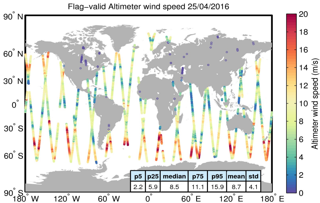
Figure 31. Geographical distribution of flag-valid wind data over oceans and lakes for 25/04/2016. The statistical values shown in the table refer to the wind in m/s and are calculated over all measurements shown in the figure.
