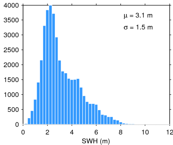
Figure 20. Histogram of science-valid SWH over oceans and lakes for 25/04/2016. The mean ( \mu ) and standard deviation ( \sigma ) are also shown. Note that values larger than 12 m are excluded from the histogram for the sake of readability but not from the computation of \mu and \sigma .
