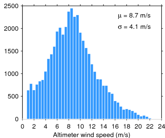
Figure 35. Histogram of science-valid wind over oceans and lakes for 25/04/2016. The mean ( \mu ) and standard deviation ( \sigma ) are also shown. Note that values larger than 24 m/s are excluded from the histogram for the sake of readability but not from the computation of \mu and \sigma .
