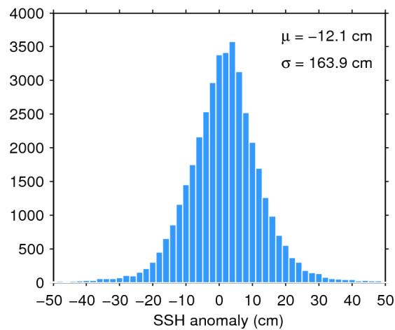
Figure 7. Histogram of flag-valid SSH anomaly over oceans and lakes for 25/04/2016. The mean ( \mu ) and standard deviation ( \sigma ) are also shown. Note that values outside [-50 50] cm are excluded from the histogram for the sake of readability but not from the computation of \mu and \sigma .
