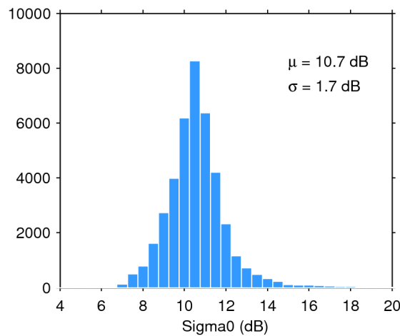
Figure 28. Histogram of science-valid sigma0 over oceans and lakes for 25/04/2016. The mean ( \mu ) and standard deviation ( \sigma ) are also shown. Note that values outside [4 20] dB are excluded from the histogram for the sake of readability but not from the computation of \mu and \sigma .
