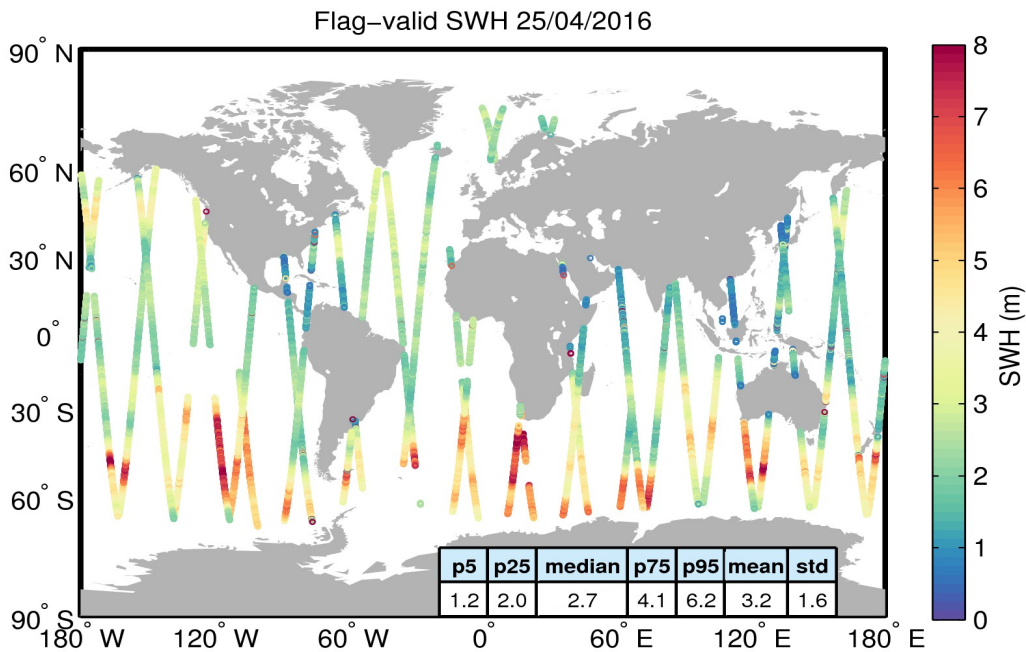
Figure 15. Geographical distribution of flag-valid SWH data over oceans and lakes for 25/04/2016. The statistical values shown in the table refer to the SWH in m and are calculated over all measurements shown in the figure.
