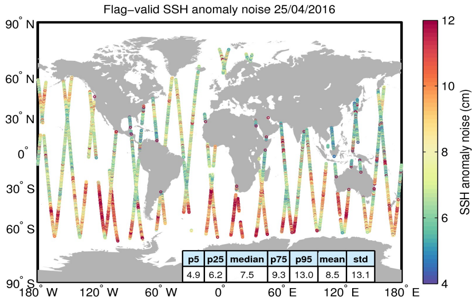
Figure 8. Geographical distribution of flag-valid 20-Hz SSH anomaly measurement noise over oceans and lakes for 25/04/2016. The statistical values shown in the table refer to the SSH anomaly noise and are calculated over all measurements shown in the figure.
