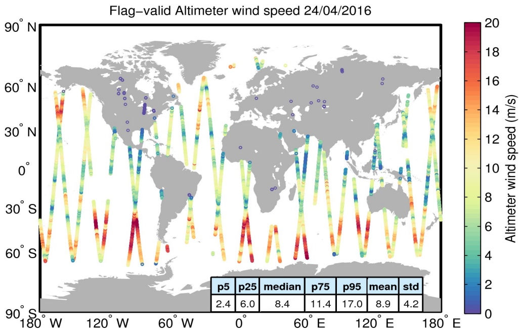
Figure 31. Geographical distribution of flag-valid wind data over oceans and lakes for 24/04/2016. The statistical values shown in the table refer to the wind in m/s and are calculated over all measurements shown in the figure.
