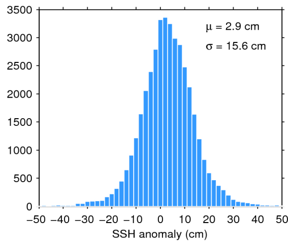
Figure 7. Histogram of flag-valid SSH anomaly over oceans and lakes for 24/04/2016. The mean ( \mu ) and standard deviation ( \sigma ) are also shown. Note that values outside [-50\ 50] cm are excluded from the histogram for the sake of readability but not from the computation of \mu and \sigma .
