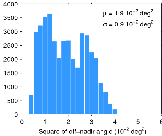
Figure 39. Histogram of flag-valid mispointing over oceans and lakes for 24/04/2016. The mean ( \mu ) and standard deviation ( \sigma ) are also shown. Note that values larger than 6 \cdot 10^{-2} \text{ deg}^2 are excluded from the histogram for the sake of readability but not from the computation of \mu and \sigma .
