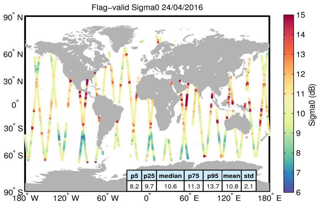
Figure 23. Geographical distribution of flag-valid sigma0 data over oceans and lakes for 24/04/2016. The statistical values shown in the table refer to the sigma0 in dB and are calculated over all measurements shown in the figure.
