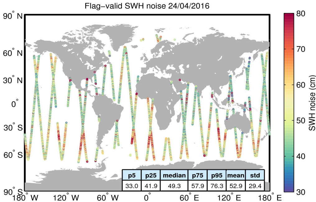
Figure 18. Geographical distribution of flag-valid 20-Hz SWH measurement noise over oceans and lakes for 24/04/2016. The statistical values shown in the figure refer to the SWH noise and are calculated over all measurements shown in the figure.
