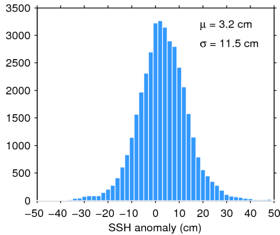
Figure 11. Histogram of science-valid SSH anomaly over oceans and lakes for 24/04/2016. The mean ( \mu ) and standard deviation ( \sigma ) are also shown. Note that values outside [-50 50] cm are excluded from the histogram for the sake of readability but not from the computation of \mu and \sigma .
