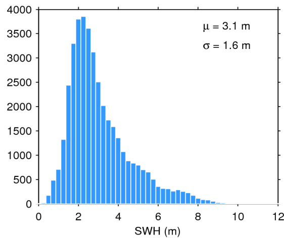
Figure 17. Histogram of flag-valid SWH over oceans and lakes for 24/04/2016. The mean ( \mu ) and standard deviation ( \sigma ) are also shown. Note that values larger than 12 m are excluded from the histogram for the sake of readability but not from the computation of \mu and \sigma .
