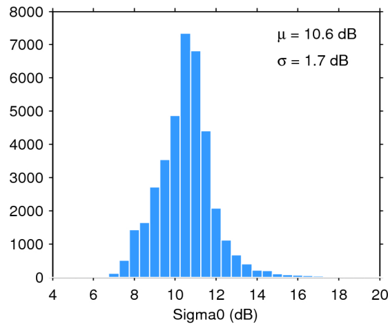
Figure 28. Histogram of science-valid sigma0 over oceans and lakes for 24/04/2016. The mean ( \mu ) and standard deviation ( \sigma ) are also shown. Note that values outside [4 20] dB are excluded from the histogram for the sake of readability but not from the computation of \mu and \sigma .
