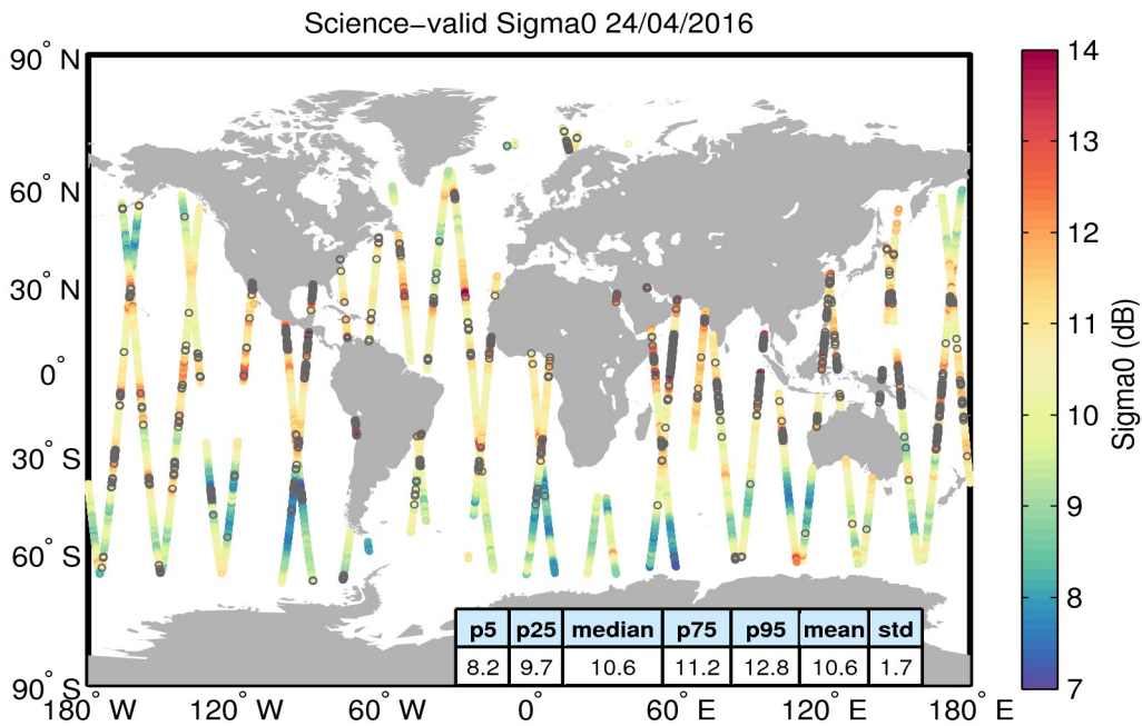
Figure 27. Geographical distribution of science-valid sigma0 data over oceans and lakes for 24/04/2016. The statistical values shown in the table refer to the sigma0 in dB and are calculated over all measurements shown in the figure. Gray circles denote records that have been rejected based on the editing criteria described in Table 4.
