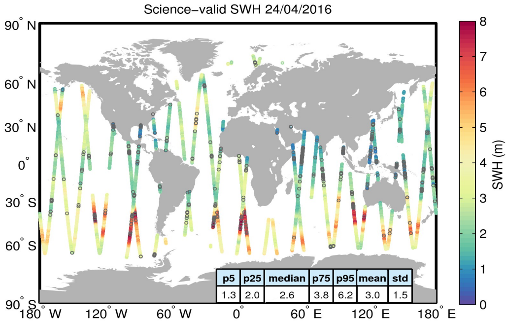
Figure 19. Geographical distribution of science-valid SWH data over oceans and lakes for 24/04/2016. The statistical values shown in the table refer to the SWH in m and are calculated over all measurements shown in the figure. Gray circles denote records that have been rejected based on the editing criteria described in Table 3.
