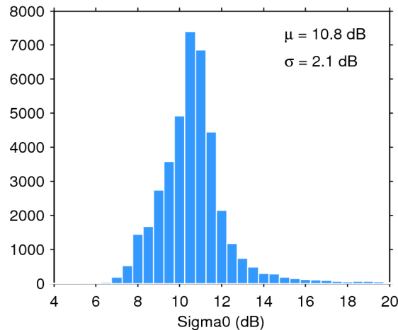
Figure 25. Histogram of flag-valid sigma0 over oceans and lakes for 24/04/2016. The mean ( \mu ) and standard deviation ( \sigma ) are also shown. Note that values outside [4 20] dB are excluded from the histogram for the sake of readability but not from the computation of \mu and \sigma .
