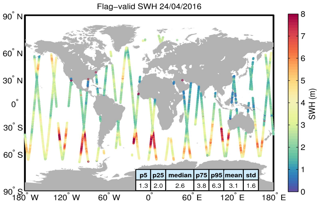
Figure 15. Geographical distribution of flag-valid SWH data over oceans and lakes for 24/04/2016. The statistical values shown in the table refer to the SWH in m and are calculated over all measurements shown in the figure.
