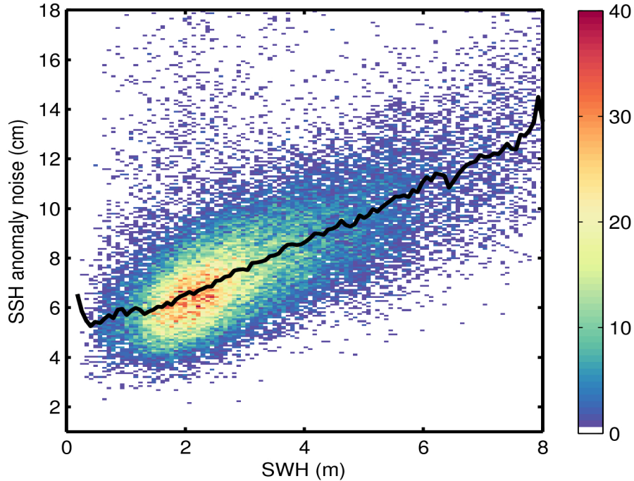
Figure 9. 2D histogram showing flag-valid SSH anomaly noise as a function of SWH for 24/04/2016. The black line denotes the median SSH anomaly noise as a function of SWH.
