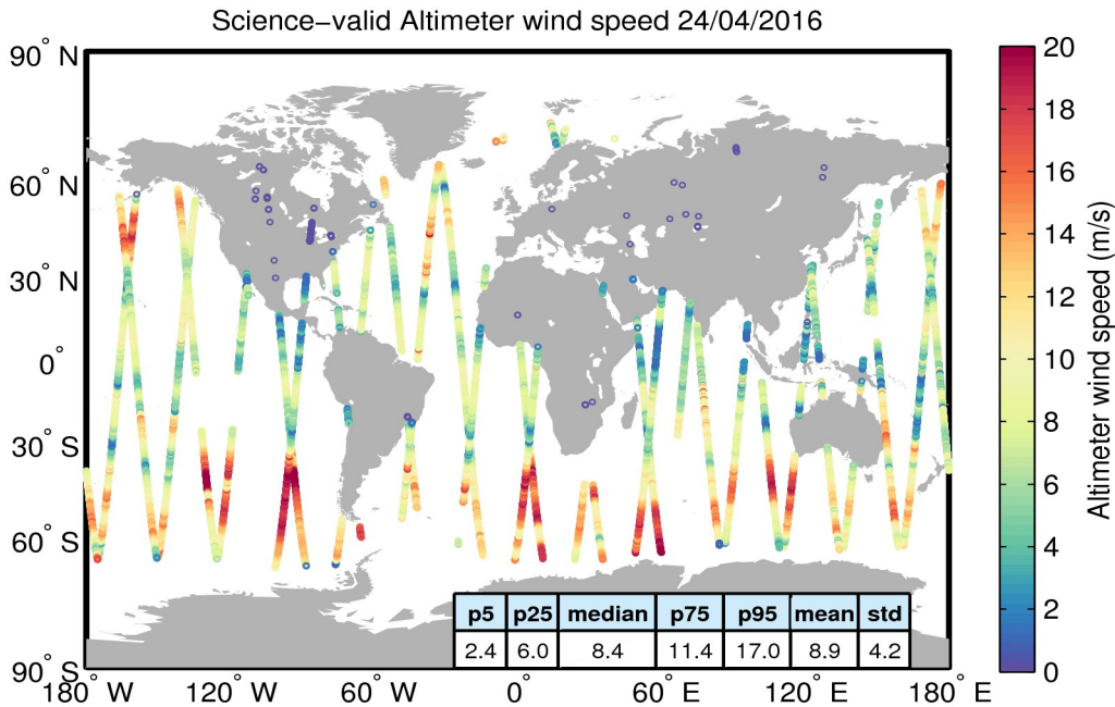
Figure 34. Geographical distribution of science-valid wind data over oceans and lakes for 24/04/2016. The statistical values shown in the table refer to the wind in m/s and are calculated over all measurements shown in the figure. Gray circles denote records that have been rejected based on the editing criteria described in Table 5.
