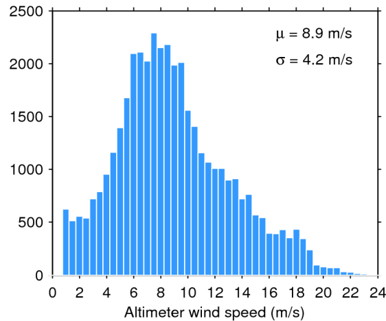
Figure 33. Histogram of flag-valid wind over oceans and lakes for 24/04/2016. The mean ( \mu ) and standard deviation ( \sigma ) are also shown. Note that values larger than 24 m/s are excluded from the histogram for the sake of readability but not from the computation of \mu and \sigma .
