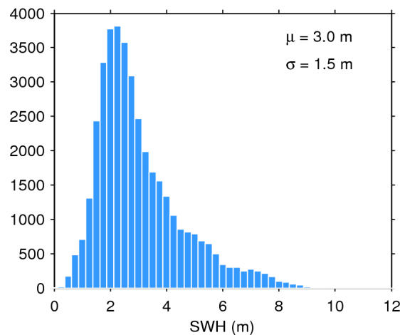
Figure 20. Histogram of science-valid SWH over oceans and lakes for 24/04/2016. The mean ( \mu ) and standard deviation ( \sigma ) are also shown. Note that values larger than 12 m are excluded from the histogram for the sake of readability but not from the computation of \mu and \sigma .
