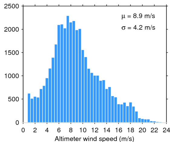
Figure 35. Histogram of science-valid wind over oceans and lakes for 24/04/2016. The mean ( \mu ) and standard deviation ( \sigma ) are also shown. Note that values larger than 24 m/s are excluded from the histogram for the sake of readability but not from the computation of \mu and \sigma .
