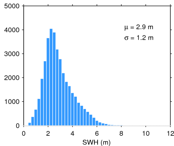
Figure 20. Histogram of science-valid SWH over oceans and lakes for 22/04/2016. The mean ( \mu ) and standard deviation ( \sigma ) are also shown. Note that values larger than 12 m are excluded from the histogram for the sake of readability but not from the computation of \mu and \sigma .
