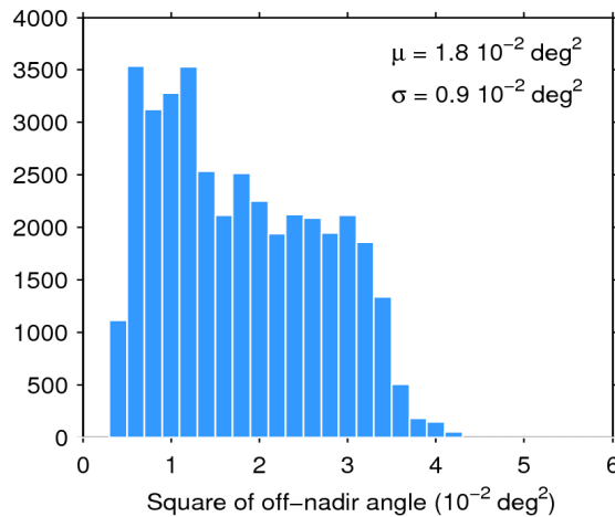
Figure 39. Histogram of flag-valid mispointing over oceans and lakes for 22/04/2016. The mean ( \mu ) and standard deviation ( \sigma ) are also shown. Note that values larger than 6 \cdot 10^{-2} \text{ deg}^2 are excluded from the histogram for the sake of readability but not from the computation of \mu and \sigma .
