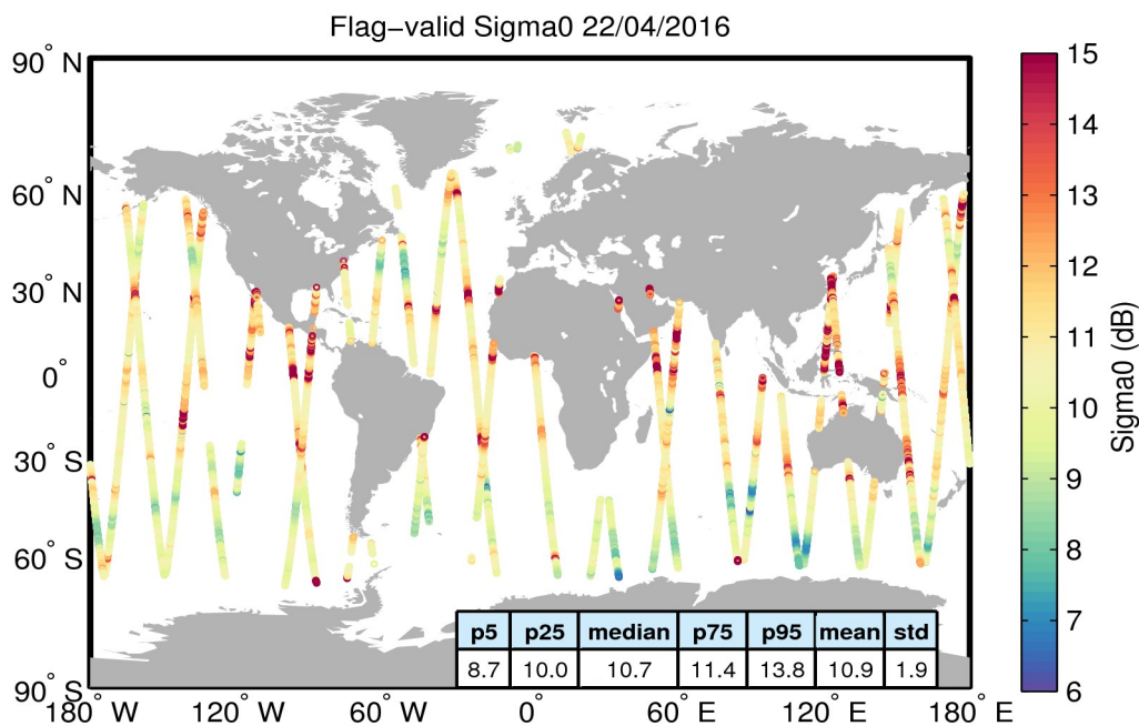
Figure 23. Geographical distribution of flag-valid sigma0 data over oceans and lakes for 22/04/2016. The statistical values shown in the table refer to the sigma0 in dB and are calculated over all measurements shown in the figure.
