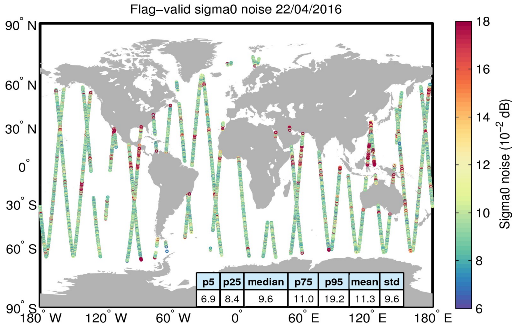
Figure 26. Geographical distribution of flag-valid 20-Hz sigma0 measurement noise over oceans and lakes for 22/04/2016. The statistical values shown in the table refer to the sigma0 noise and are calculated over all measurements shown in the figure.
