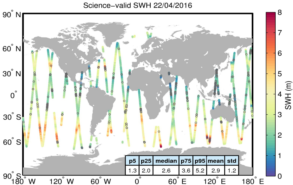
Figure 19. Geographical distribution of science-valid SWH data over oceans and lakes for 22/04/2016. The statistical values shown in the table refer to the SWH in m and are calculated over all measurements shown in the figure. Gray circles denote records that have been rejected based on the editing criteria described in Table 3.
