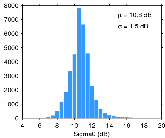
Figure 28. Histogram of science-valid sigma0 over oceans and lakes for 22/04/2016. The mean ( \mu ) and standard deviation ( \sigma ) are also shown. Note that values outside [4 20] dB are excluded from the histogram for the sake of readability but not from the computation of \mu and \sigma .
