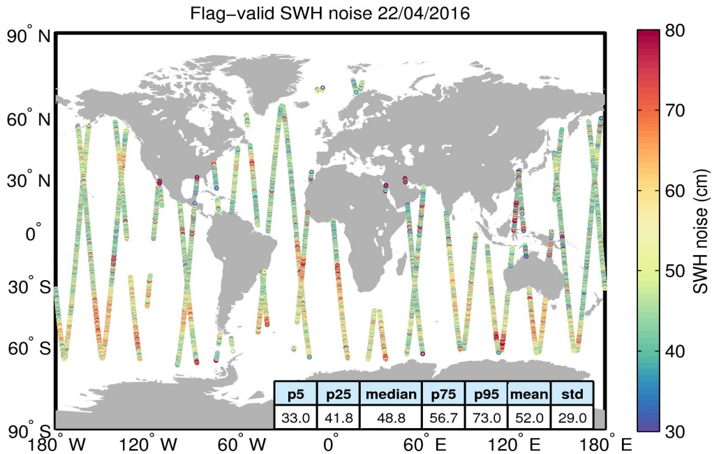
Figure 18. Geographical distribution of flag-valid 20-Hz SWH measurement noise over oceans and lakes for 22/04/2016. The statistical values shown in the figure refer to the SWH noise and are calculated over all measurements shown in the figure.
