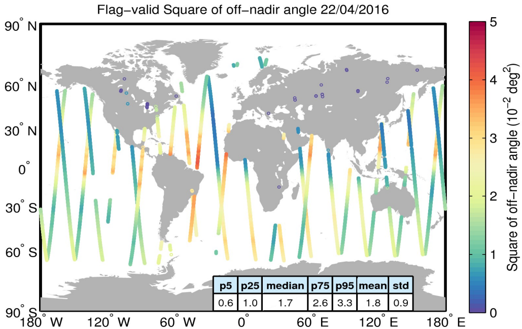
Figure 37. Geographical distribution of flag-valid mispointing data over oceans and lakes for 22/04/2016. The statistical values shown in the table refer to the mispointing in 10^{-2} \text{ deg}^2 and are calculated over all measurements shown in the figure.
