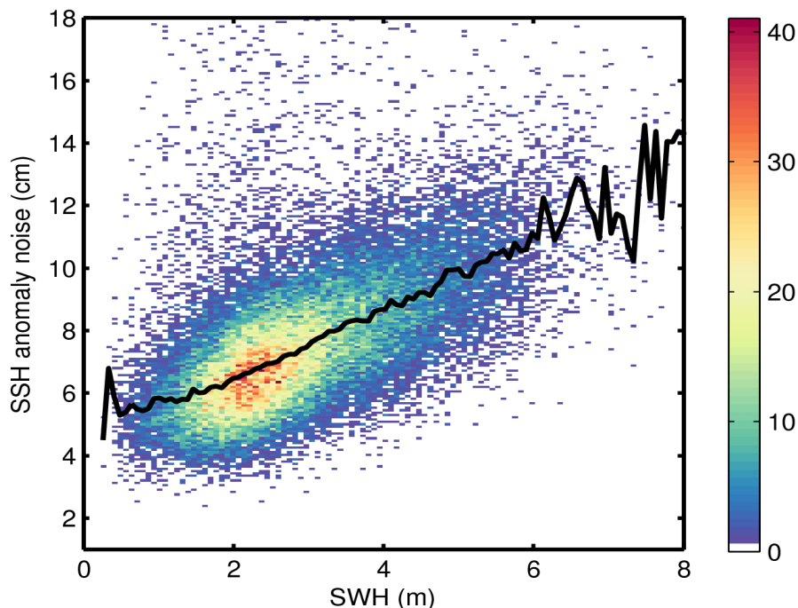
Figure 9. 2D histogram showing flag-valid SSH anomaly noise as a function of SWH for 22/04/2016. The black line denotes the median SSH anomaly noise as a function of SWH.
