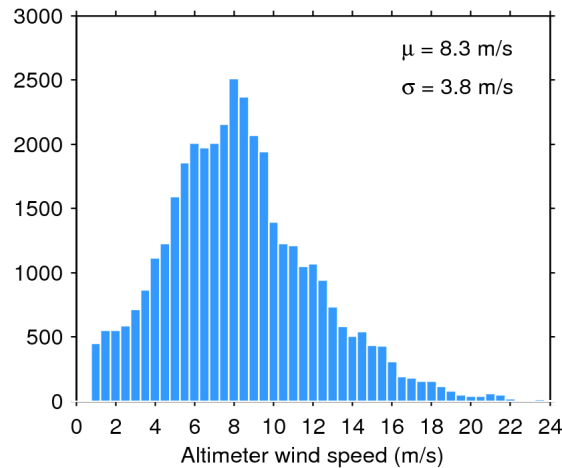
Figure 33. Histogram of flag-valid wind over oceans and lakes for 22/04/2016. The mean ( \mu ) and standard deviation ( \sigma ) are also shown. Note that values larger than 24 m/s are excluded from the histogram for the sake of readability but not from the computation of \mu and \sigma .
