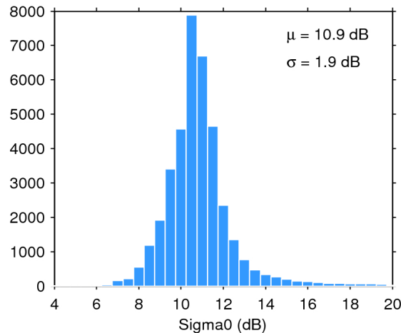
Figure 25. Histogram of flag-valid sigma0 over oceans and lakes for 22/04/2016. The mean ( \mu ) and standard deviation ( \sigma ) are also shown. Note that values outside [4 20] dB are excluded from the histogram for the sake of readability but not from the computation of \mu and \sigma .
