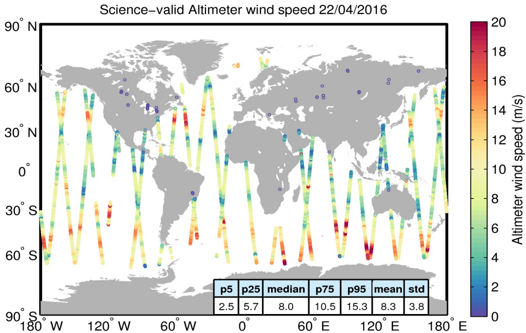
Figure 34. Geographical distribution of science-valid wind data over oceans and lakes for 22/04/2016. The statistical values shown in the table refer to the wind in m/s and are calculated over all measurements shown in the figure. Gray circles denote records that have been rejected based on the editing criteria described in Table 5.
