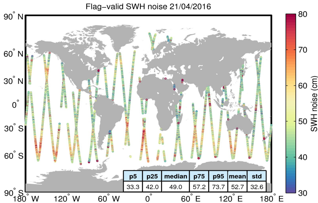
Figure 18. Geographical distribution of flag-valid 20-Hz SWH measurement noise over oceans and lakes for 21/04/2016. The statistical values shown in the figure refer to the SWH noise and are calculated over all measurements shown in the figure.
