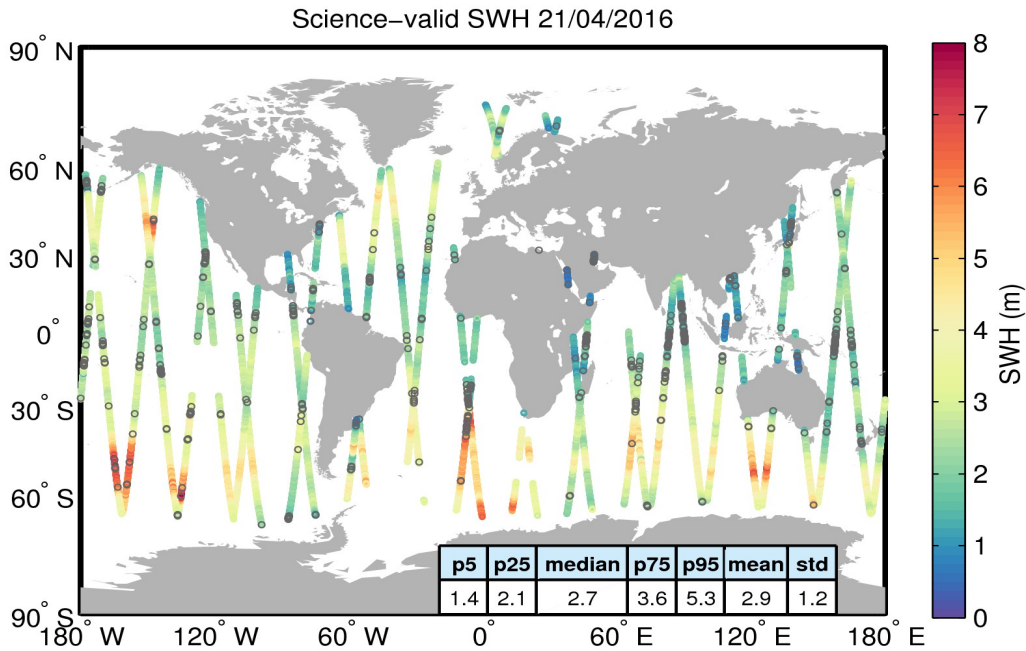
Figure 19. Geographical distribution of science-valid SWH data over oceans and lakes for 21/04/2016. The statistical values shown in the table refer to the SWH in m and are calculated over all measurements shown in the figure. Gray circles denote records that have been rejected based on the editing criteria described in Table 3.
