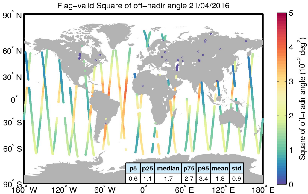
Figure 37. Geographical distribution of flag-valid mispointing data over oceans and lakes for 21/04/2016. The statistical values shown in the table refer to the mispointing in 10^{-2} \text{ deg}^2 and are calculated over all measurements shown in the figure.
