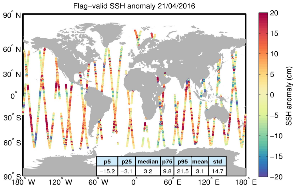
Figure 5. Geographical distribution of flag-valid 1-Hz SSH anomaly data over oceans and lakes for 21/04/2016. The statistical values shown in the table refer to the SSH anomaly in cm and are calculated over all measurements shown in the figure.
