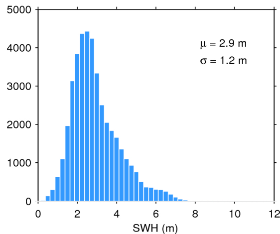
Figure 20. Histogram of science-valid SWH over oceans and lakes for 21/04/2016. The mean ( \mu ) and standard deviation ( \sigma ) are also shown. Note that values larger than 12 m are excluded from the histogram for the sake of readability but not from the computation of \mu and \sigma .
