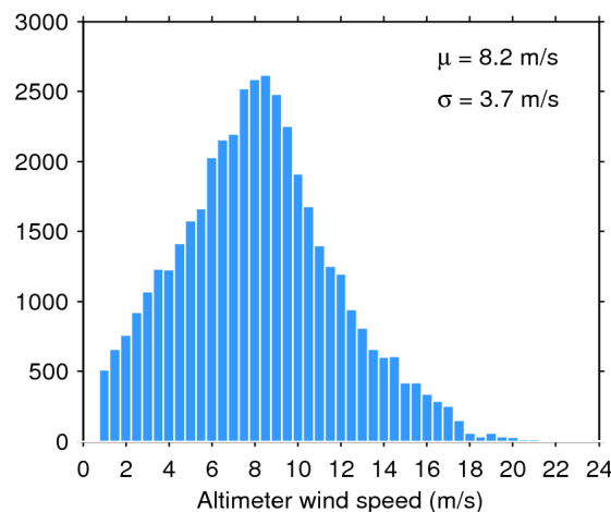
Figure 35. Histogram of science-valid wind over oceans and lakes for 21/04/2016. The mean ( \mu ) and standard deviation ( \sigma ) are also shown. Note that values larger than 24 m/s are excluded from the histogram for the sake of readability but not from the computation of \mu and \sigma .
