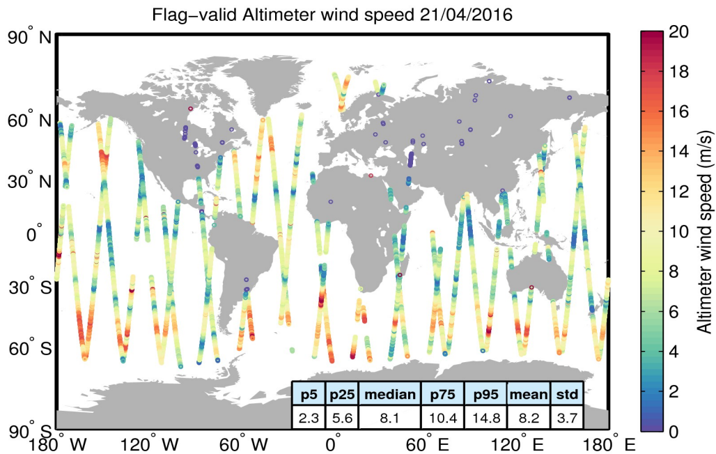
Figure 31. Geographical distribution of flag-valid wind data over oceans and lakes for 21/04/2016. The statistical values shown in the table refer to the wind in m/s and are calculated over all measurements shown in the figure.
