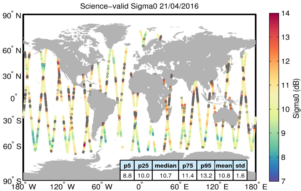
Figure 27. Geographical distribution of science-valid sigma0 data over oceans and lakes for 21/04/2016. The statistical values shown in the table refer to the sigma0 in dB and are calculated over all measurements shown in the figure. Gray circles denote records that have been rejected based on the editing criteria described in Table 4.
