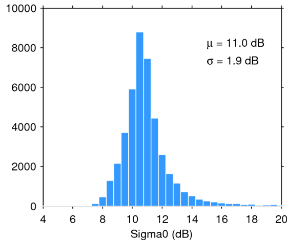
Figure 25. Histogram of flag-valid sigma0 over oceans and lakes for 21/04/2016. The mean ( \mu ) and standard deviation ( \sigma ) are also shown. Note that values outside [4 20] dB are excluded from the histogram for the sake of readability but not from the computation of \mu and \sigma .
