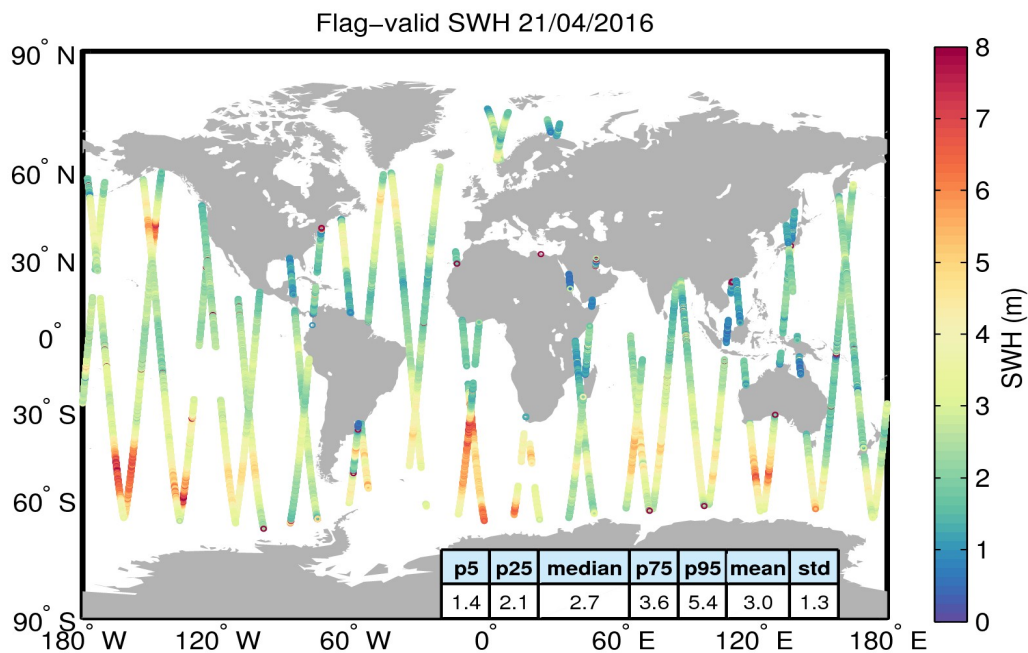
Figure 15. Geographical distribution of flag-valid SWH data over oceans and lakes for 21/04/2016. The statistical values shown in the table refer to the SWH in m and are calculated over all measurements shown in the figure.
