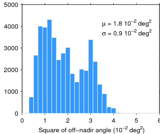
Figure 39. Histogram of flag-valid mispointing over oceans and lakes for 21/04/2016. The mean ( \mu ) and standard deviation ( \sigma ) are also shown. Note that values larger than 6 \cdot 10^{-2} \text{ deg}^2 are excluded from the histogram for the sake of readability but not from the computation of \mu and \sigma .
