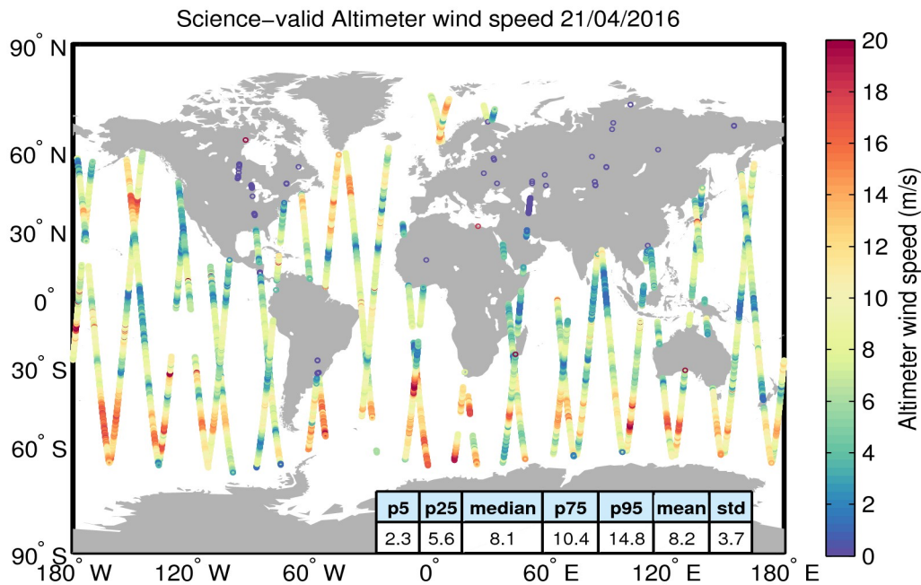
Figure 34. Geographical distribution of science-valid wind data over oceans and lakes for 21/04/2016. The statistical values shown in the table refer to the wind in m/s and are calculated over all measurements shown in the figure. Gray circles denote records that have been rejected based on the editing criteria described in Table 5.
