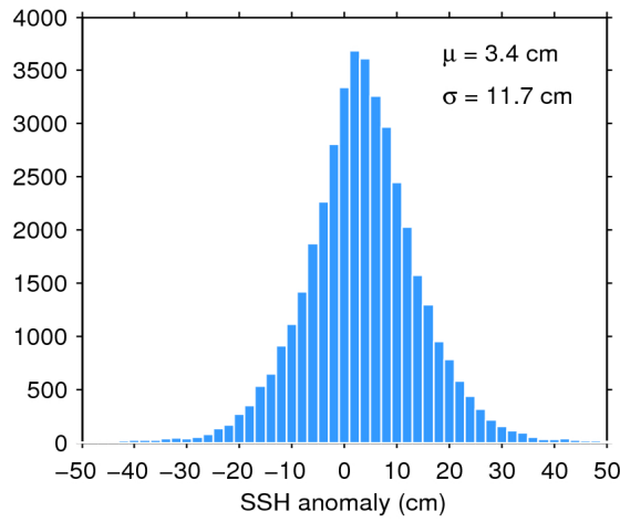
Figure 11. Histogram of science-valid SSH anomaly over oceans and lakes for 21/04/2016. The mean ( \mu ) and standard deviation ( \sigma ) are also shown. Note that values outside [-50 50] cm are excluded from the histogram for the sake of readability but not from the computation of \mu and \sigma .
