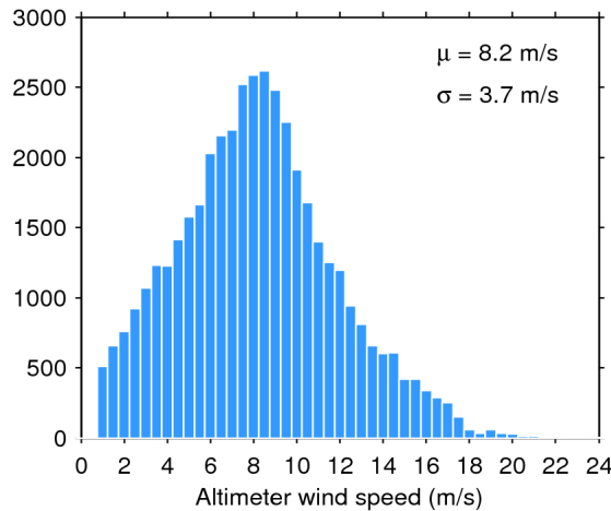
Figure 33. Histogram of flag-valid wind over oceans and lakes for 21/04/2016. The mean ( \mu ) and standard deviation ( \sigma ) are also shown. Note that values larger than 24 m/s are excluded from the histogram for the sake of readability but not from the computation of \mu and \sigma .
