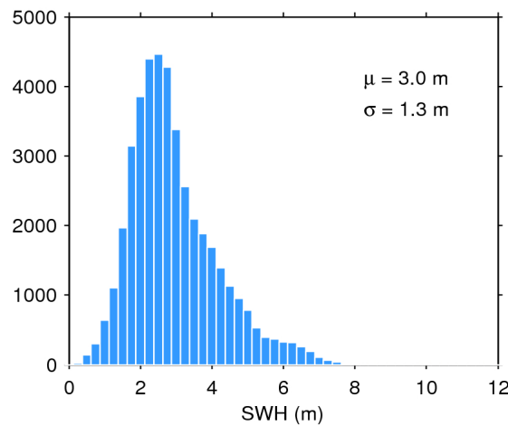
Figure 17. Histogram of flag-valid SWH over oceans and lakes for 21/04/2016. The mean ( \mu ) and standard deviation ( \sigma ) are also shown. Note that values larger than 12 m are excluded from the histogram for the sake of readability but not from the computation of \mu and \sigma .
