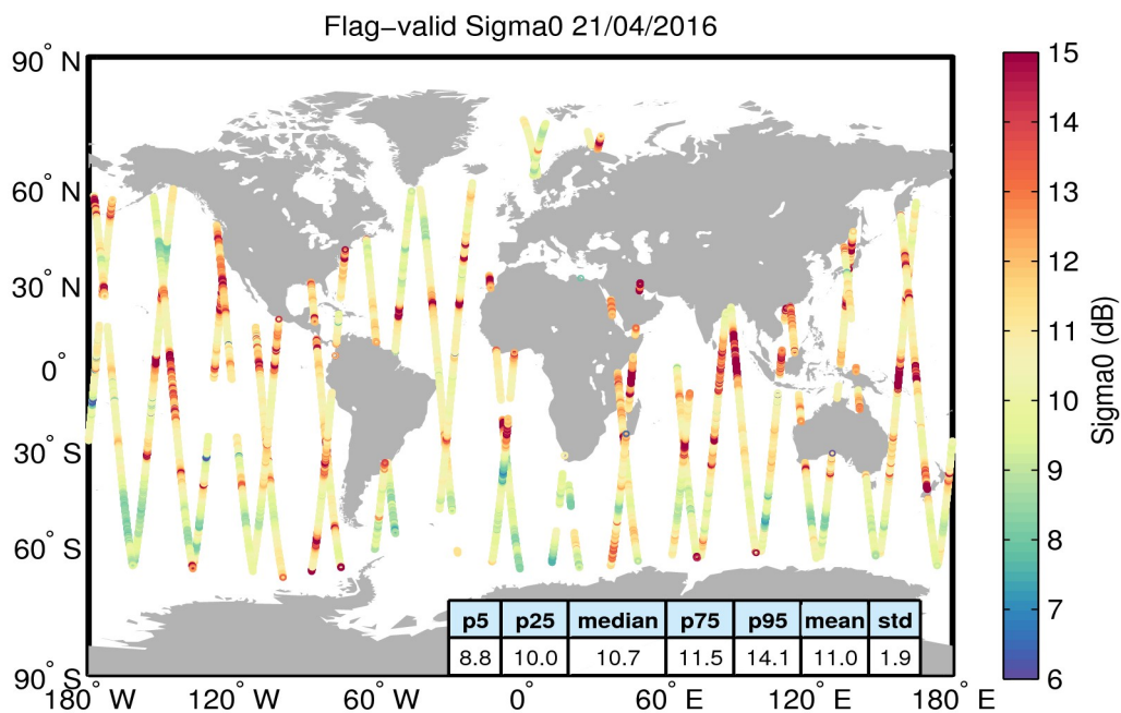
Figure 23. Geographical distribution of flag-valid sigma0 data over oceans and lakes for 21/04/2016. The statistical values shown in the table refer to the sigma0 in dB and are calculated over all measurements shown in the figure.
