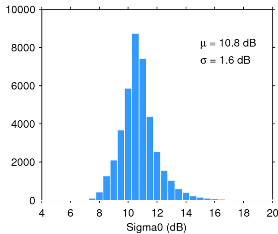
Figure 28. Histogram of science-valid sigma0 over oceans and lakes for 21/04/2016. The mean ( \mu ) and standard deviation ( \sigma ) are also shown. Note that values outside [4 20] dB are excluded from the histogram for the sake of readability but not from the computation of \mu and \sigma .
