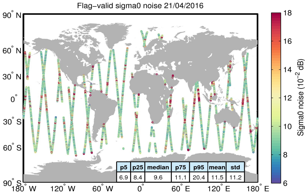
Figure 26. Geographical distribution of flag-valid 20-Hz sigma0 measurement noise over oceans and lakes for 21/04/2016. The statistical values shown in the table refer to the sigma0 noise and are calculated over all measurements shown in the figure.
