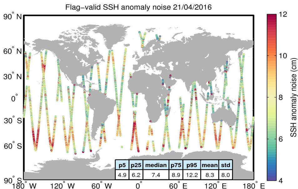
Figure 8. Geographical distribution of flag-valid 20-Hz SSH anomaly measurement noise over oceans and lakes for 21/04/2016. The statistical values shown in the table refer to the SSH anomaly noise and are calculated over all measurements shown in the figure.
