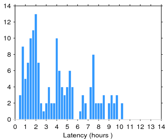
Figure 2. Histogram of the data latency for 21/04/2016. The y-axis denotes the number of files that are made available with a delay of x-hours with respect to the mean time of the records stored in the file.
