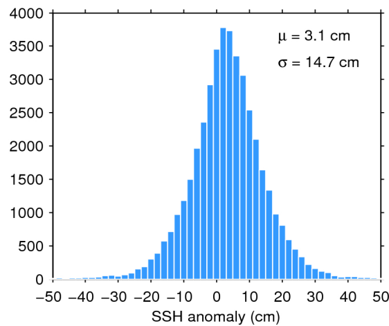
Figure 7. Histogram of flag-valid SSH anomaly over oceans and lakes for 21/04/2016. The mean ( \mu ) and standard deviation ( \sigma ) are also shown. Note that values outside [-50\ 50] cm are excluded from the histogram for the sake of readability but not from the computation of \mu and \sigma .
