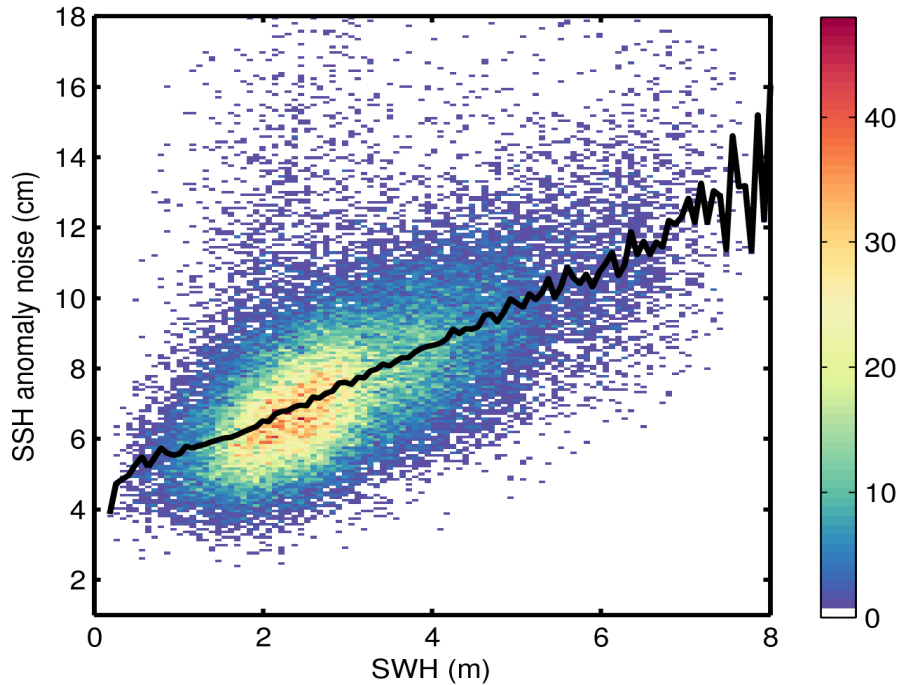
Figure 9. 2D histogram showing flag-valid SSH anomaly noise as a function of SWH for 21/04/2016. The black line denotes the median SSH anomaly noise as a function of SWH.
