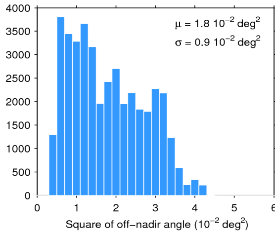
Figure 39. Histogram of flag-valid mispointing over oceans and lakes for 20/04/2016. The mean ( \mu ) and standard deviation ( \sigma ) are also shown. Note that values larger than 6 \cdot 10^{-2} \text{ deg}^2 are excluded from the histogram for the sake of readability but not from the computation of \mu and \sigma .
