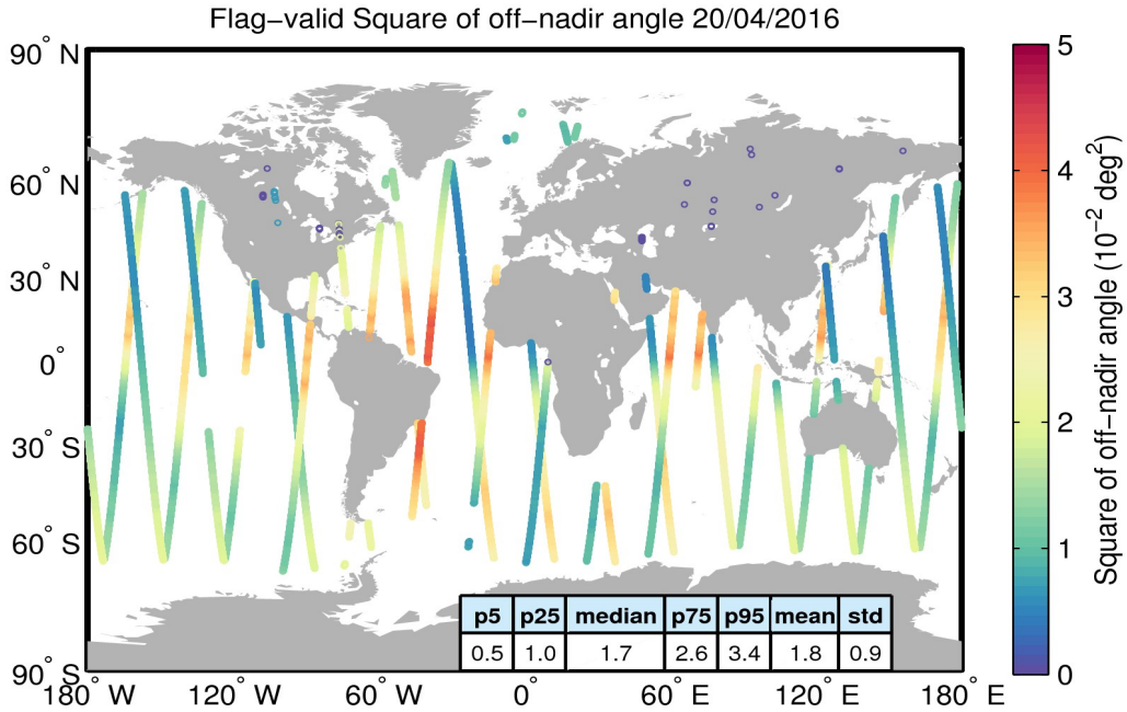
Figure 37. Geographical distribution of flag-valid mispointing data over oceans and lakes for 20/04/2016. The statistical values shown in the table refer to the mispointing in 10^{-2} deg 2 and are calculated over all measurements shown in the figure.
