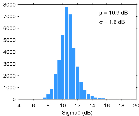
Figure 28. Histogram of science-valid sigma0 over oceans and lakes for 20/04/2016. The mean ( \mu ) and standard deviation ( \sigma ) are also shown. Note that values outside [4 20] dB are excluded from the histogram for the sake of readability but not from the computation of \mu and \sigma .
