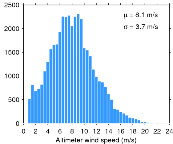
Figure 33. Histogram of flag-valid wind over oceans and lakes for 20/04/2016. The mean ( \mu ) and standard deviation ( \sigma ) are also shown. Note that values larger than 24 m/s are excluded from the histogram for the sake of readability but not from the computation of \mu and \sigma .
