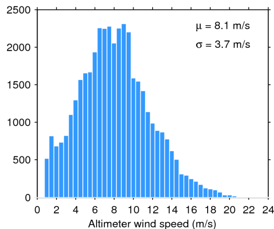
Figure 35. Histogram of science-valid wind over oceans and lakes for 20/04/2016. The mean ( \mu ) and standard deviation ( \sigma ) are also shown. Note that values larger than 24 m/s are excluded from the histogram for the sake of readability but not from the computation of \mu and \sigma .
