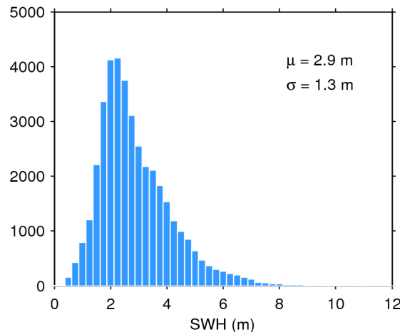
Figure 20. Histogram of science-valid SWH over oceans and lakes for 20/04/2016. The mean ( \mu ) and standard deviation ( \sigma ) are also shown. Note that values larger than 12 m are excluded from the histogram for the sake of readability but not from the computation of \mu and \sigma .
