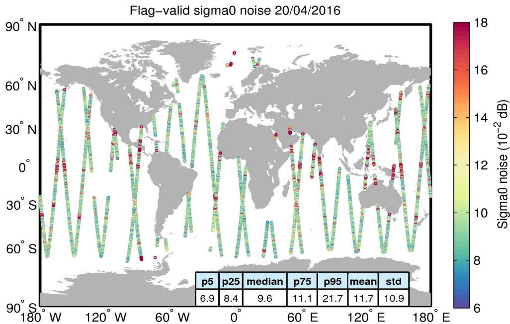
Figure 26. Geographical distribution of flag-valid 20-Hz sigma0 measurement noise over oceans and lakes for 20/04/2016. The statistical values shown in the table refer to the sigma0 noise and are calculated over all measurements shown in the figure.
