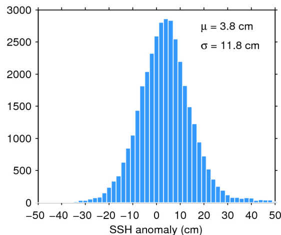
Figure 11. Histogram of science-valid SSH anomaly over oceans and lakes for 20/04/2016. The mean ( \mu ) and standard deviation ( \sigma ) are also shown. Note that values outside [-50 50] cm are excluded from the histogram for the sake of readability but not from the computation of \mu and \sigma .
