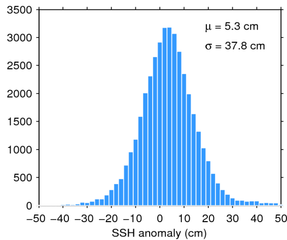
Figure 7. Histogram of flag-valid SSH anomaly over oceans and lakes for 20/04/2016. The mean ( \mu ) and standard deviation ( \sigma ) are also shown. Note that values outside [-50\ 50] cm are excluded from the histogram for the sake of readability but not from the computation of \mu and \sigma .
