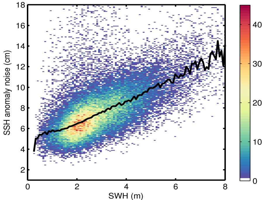
Figure 9. 2D histogram showing flag-valid SSH anomaly noise as a function of SWH for 20/04/2016. The black line denotes the median SSH anomaly noise as a function of SWH.
