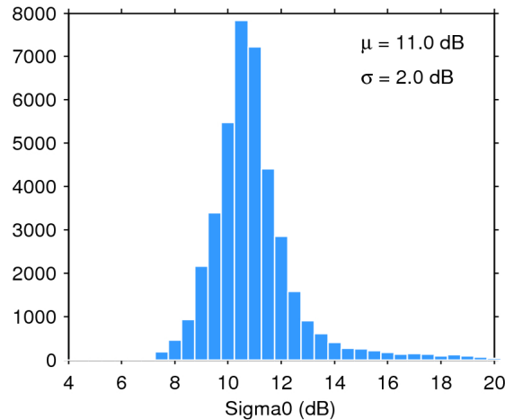
Figure 25. Histogram of flag-valid sigma0 over oceans and lakes for 20/04/2016. The mean ( \mu ) and standard deviation ( \sigma ) are also shown. Note that values outside [4 20] dB are excluded from the histogram for the sake of readability but not from the computation of \mu and \sigma .
