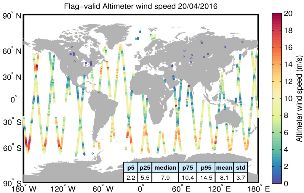
Figure 31. Geographical distribution of flag-valid wind data over oceans and lakes for 20/04/2016. The statistical values shown in the table refer to the wind in m/s and are calculated over all measurements shown in the figure.
