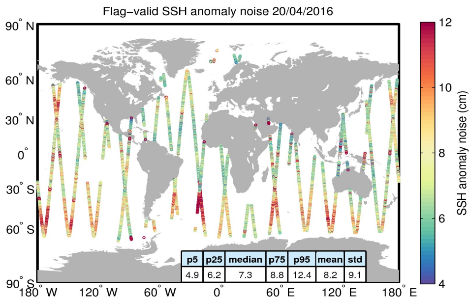
Figure 8. Geographical distribution of flag-valid 20-Hz SSH anomaly measurement noise over oceans and lakes for 20/04/2016. The statistical values shown in the table refer to the SSH anomaly noise and are calculated over all measurements shown in the figure.
