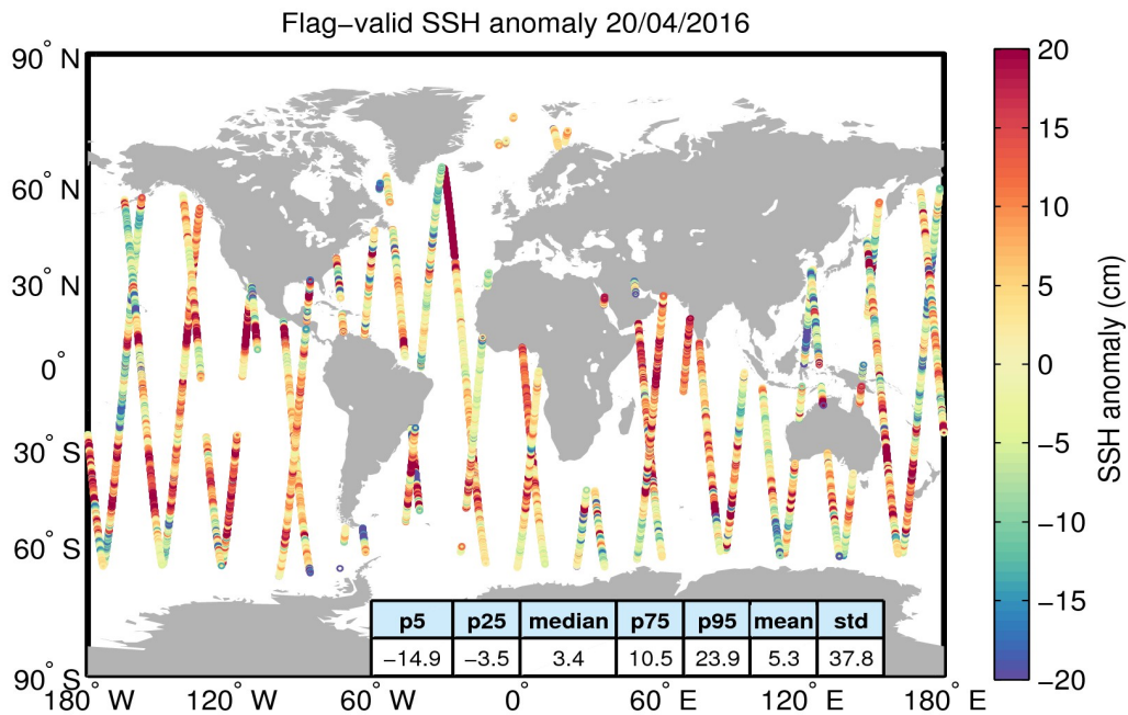
Figure 5. Geographical distribution of flag-valid 1-Hz SSH anomaly data over oceans and lakes for 20/04/2016. The statistical values shown in the table refer to the SSH anomaly in cm and are calculated over all measurements shown in the figure.
