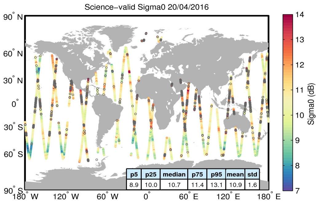
Figure 27. Geographical distribution of science-valid sigma0 data over oceans and lakes for 20/04/2016. The statistical values shown in the table refer to the sigma0 in dB and are calculated over all measurements shown in the figure. Gray circles denote records that have been rejected based on the editing criteria described in Table 4.
