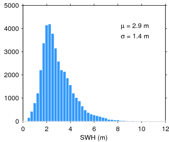
Figure 17. Histogram of flag-valid SWH over oceans and lakes for 20/04/2016. The mean ( \mu ) and standard deviation ( \sigma ) are also shown. Note that values larger than 12 m are excluded from the histogram for the sake of readability but not from the computation of \mu and \sigma .
