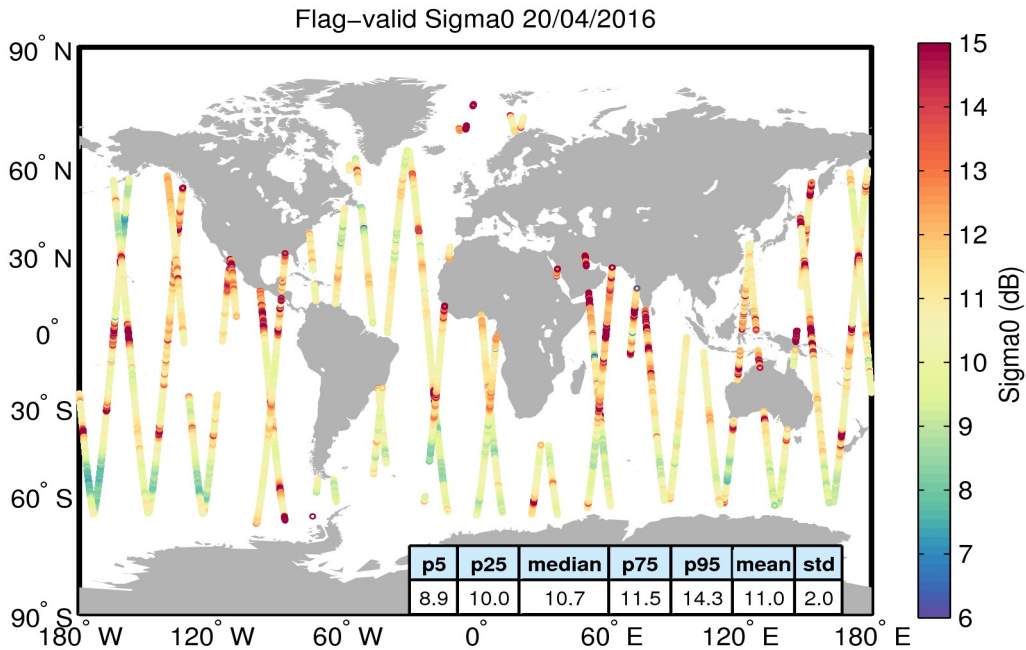
Figure 23. Geographical distribution of flag-valid sigma0 data over oceans and lakes for 20/04/2016. The statistical values shown in the table refer to the sigma0 in dB and are calculated over all measurements shown in the figure.
