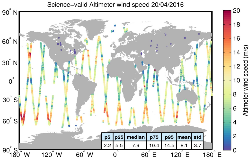
Figure 34. Geographical distribution of science-valid wind data over oceans and lakes for 20/04/2016. The statistical values shown in the table refer to the wind in m/s and are calculated over all measurements shown in the figure. Gray circles denote records that have been rejected based on the editing criteria described in Table 5.
