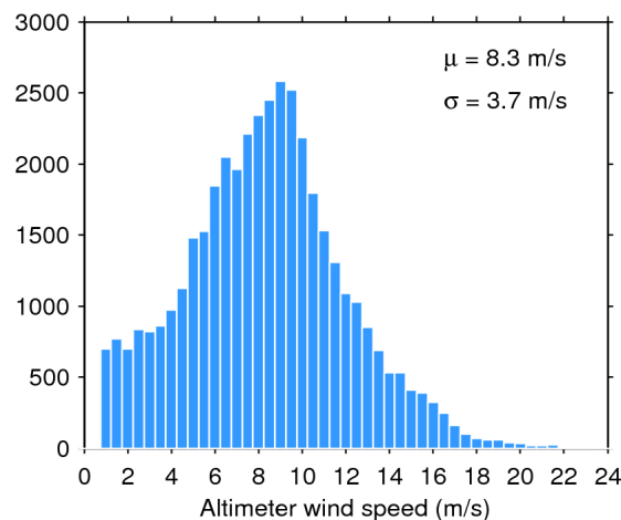
Figure 35. Histogram of science-valid wind over oceans and lakes for 19/04/2016. The mean ( \mu ) and standard deviation ( \sigma ) are also shown. Note that values larger than 24 m/s are excluded from the histogram for the sake of readability but not from the computation of \mu and \sigma .
