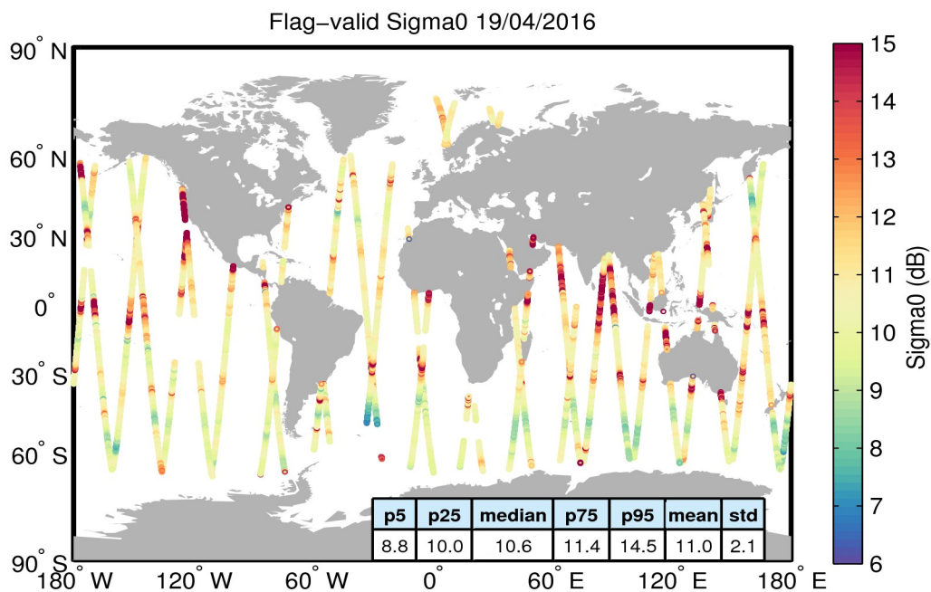
Figure 23. Geographical distribution of flag-valid sigma0 data over oceans and lakes for 19/04/2016. The statistical values shown in the table refer to the sigma0 in dB and are calculated over all measurements shown in the figure.
