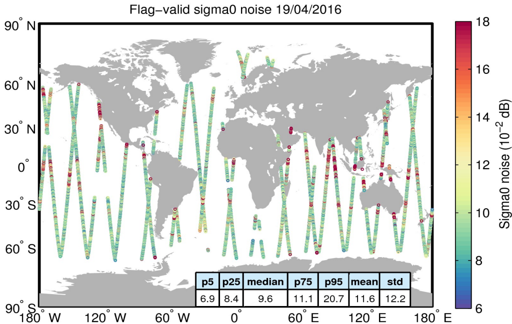
Figure 26. Geographical distribution of flag-valid 20-Hz sigma0 measurement noise over oceans and lakes for 19/04/2016. The statistical values shown in the table refer to the sigma0 noise and are calculated over all measurements shown in the figure.
