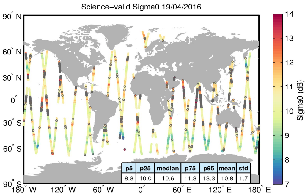
Figure 27. Geographical distribution of science-valid sigma0 data over oceans and lakes for 19/04/2016. The statistical values shown in the table refer to the sigma0 in dB and are calculated over all measurements shown in the figure. Gray circles denote records that have been rejected based on the editing criteria described in Table 4.
