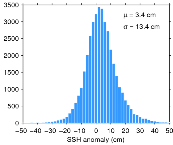
Figure 11. Histogram of science-valid SSH anomaly over oceans and lakes for 19/04/2016. The mean ( \mu ) and standard deviation ( \sigma ) are also shown. Note that values outside [-50 50] cm are excluded from the histogram for the sake of readability but not from the computation of \mu and \sigma .
