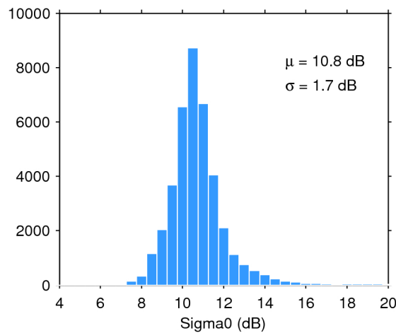
Figure 28. Histogram of science-valid sigma0 over oceans and lakes for 19/04/2016. The mean ( \mu ) and standard deviation ( \sigma ) are also shown. Note that values outside [4 20] dB are excluded from the histogram for the sake of readability but not from the computation of \mu and \sigma .
