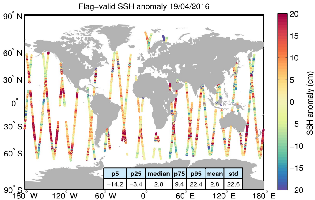
Figure 5. Geographical distribution of flag-valid 1-Hz SSH anomaly data over oceans and lakes for 19/04/2016. The statistical values shown in the table refer to the SSH anomaly in cm and are calculated over all measurements shown in the figure.
