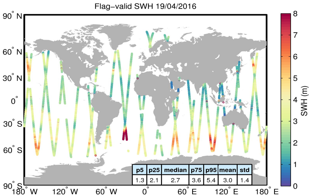
Figure 15. Geographical distribution of flag-valid SWH data over oceans and lakes for 19/04/2016. The statistical values shown in the table refer to the SWH in m and are calculated over all measurements shown in the figure.
