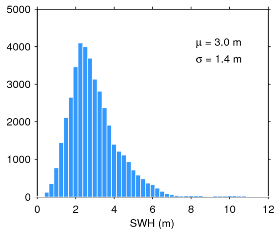
Figure 17. Histogram of flag-valid SWH over oceans and lakes for 19/04/2016. The mean ( \mu ) and standard deviation ( \sigma ) are also shown. Note that values larger than 12 m are excluded from the histogram for the sake of readability but not from the computation of \mu and \sigma .
