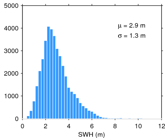
Figure 20. Histogram of science-valid SWH over oceans and lakes for 19/04/2016. The mean ( \mu ) and standard deviation ( \sigma ) are also shown. Note that values larger than 12 m are excluded from the histogram for the sake of readability but not from the computation of \mu and \sigma .
