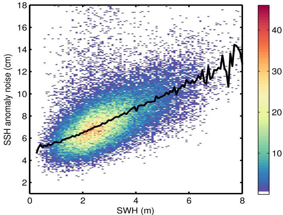
Figure 9. 2D histogram showing flag-valid SSH anomaly noise as a function of SWH for 19/04/2016. The black line denotes the median SSH anomaly noise as a function of SWH.
