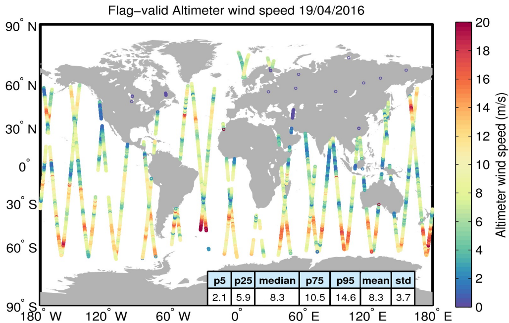
Figure 31. Geographical distribution of flag-valid wind data over oceans and lakes for 19/04/2016. The statistical values shown in the table refer to the wind in m/s and are calculated over all measurements shown in the figure.
