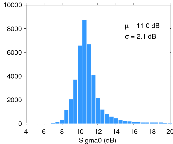
Figure 25. Histogram of flag-valid sigma0 over oceans and lakes for 19/04/2016. The mean ( \mu ) and standard deviation ( \sigma ) are also shown. Note that values outside [4 20] dB are excluded from the histogram for the sake of readability but not from the computation of \mu and \sigma .
