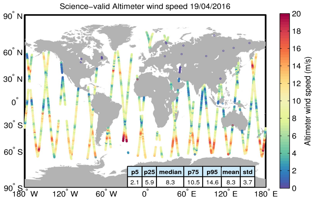
Figure 34. Geographical distribution of science-valid wind data over oceans and lakes for 19/04/2016. The statistical values shown in the table refer to the wind in m/s and are calculated over all measurements shown in the figure. Gray circles denote records that have been rejected based on the editing criteria described in Table 5.
