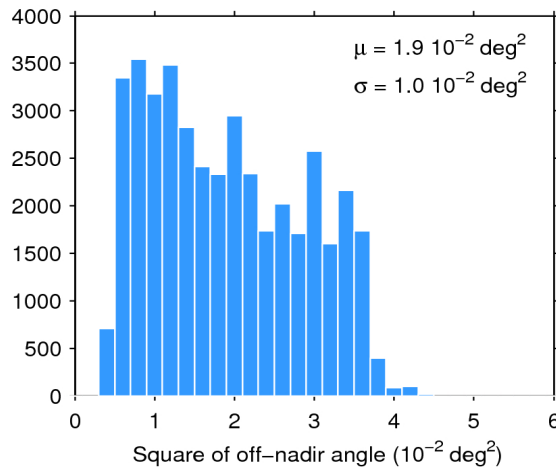
Figure 39. Histogram of flag-valid mispointing over oceans and lakes for 19/04/2016. The mean ( \mu ) and standard deviation ( \sigma ) are also shown. Note that values larger than 6 \cdot 10^{-2} \text{ deg}^2 are excluded from the histogram for the sake of readability but not from the computation of \mu and \sigma .
