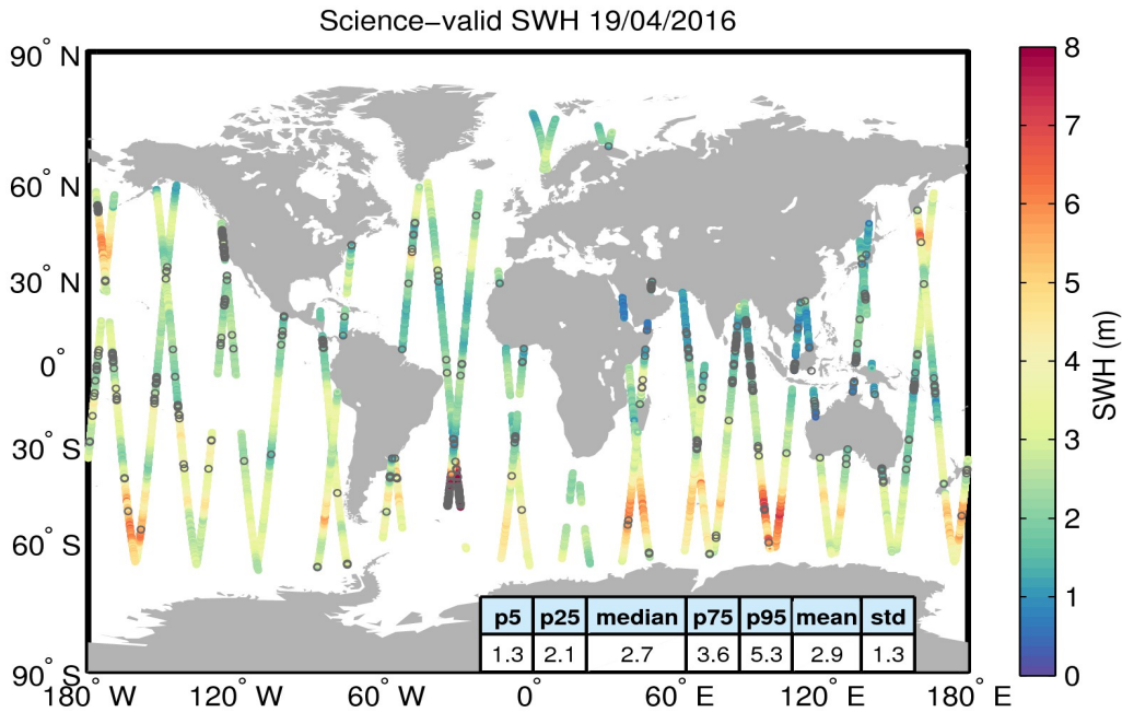
Figure 19. Geographical distribution of science-valid SWH data over oceans and lakes for 19/04/2016. The statistical values shown in the table refer to the SWH in m and are calculated over all measurements shown in the figure. Gray circles denote records that have been rejected based on the editing criteria described in Table 3.
