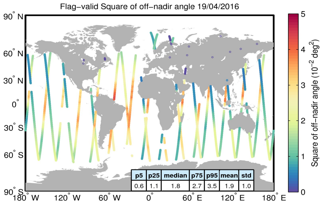
Figure 37. Geographical distribution of flag-valid mispointing data over oceans and lakes for 19/04/2016. The statistical values shown in the table refer to the mispointing in 10^{-2} deg 2 and are calculated over all measurements shown in the figure.
